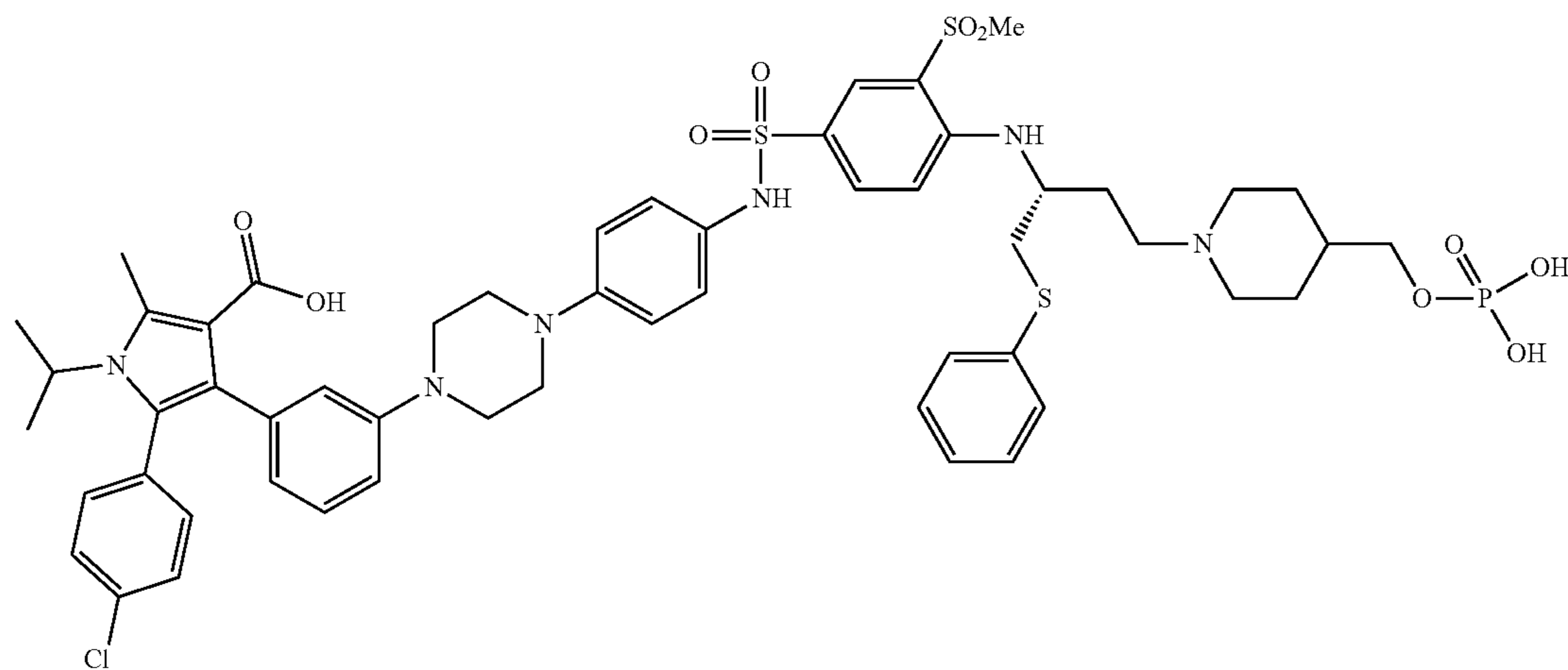
(R)-5-(4-chlorophenyl)-1-isopropyl-2-methyl-4-(3-(4-(4-((3-(methylsulfonyl)-4-((1-(phenylthio)-4-(4-((phosphonooxy)methyl)piperidin-1-yl)butan-2-yl)amino)phenyl)sulfonamido)phenyl)piperazin-1-yl)phenyl)-1H-pyrrole-3-carboxylic acid
