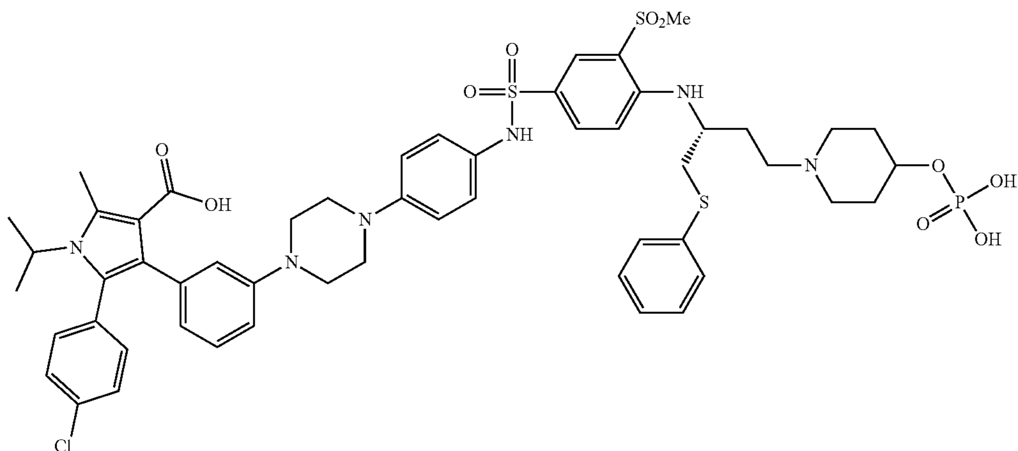
(R)-5-(4-chlorophenyl)-1-isopropyl-2-methyl-4-(3-(4-(4-((3-(methylsulfonyl)-4-((1-(phenylthio)-4-(4-phosphonoxy)piperidin-1-yl)butan-2-yl)amino)phenyl)sulfonamido)phenyl)piperazin-1-yl)phenyl)-1H-pyrrole-3-carboxylic acid
