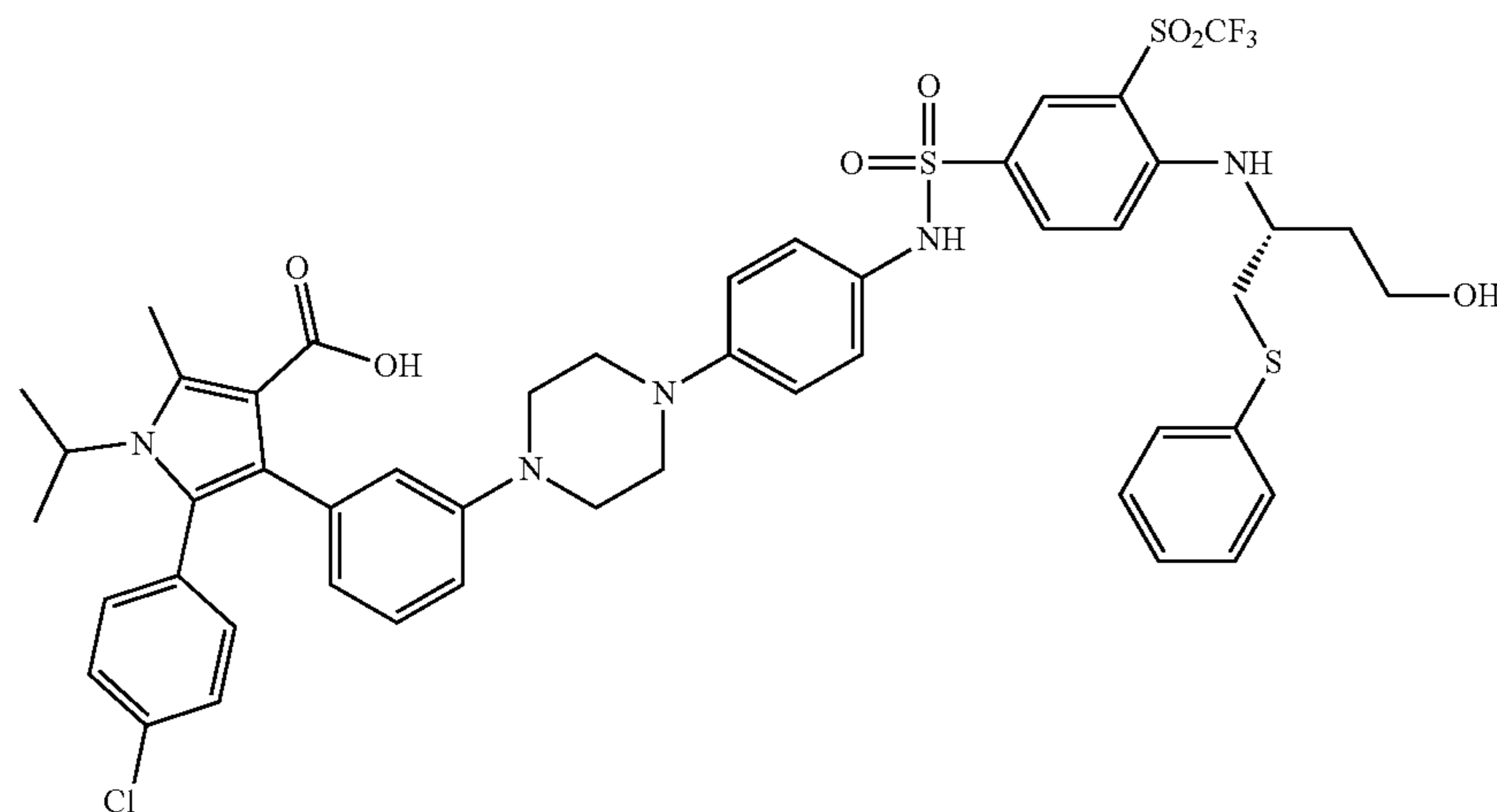
(R)-5-(4-chlorophenyl)-4-(3-(4-(4-((4-(4-(hydroxy-1-(phenylthio)butan-2-yl)amino)-3-(trifluoromethyl)sulfonyl)phenyl)sulfonamido)phenyl)piperazin-1-yl)phenyl)-1-isopropyl-2-methyl-1H-pyrrole-3-carboxylic acid
