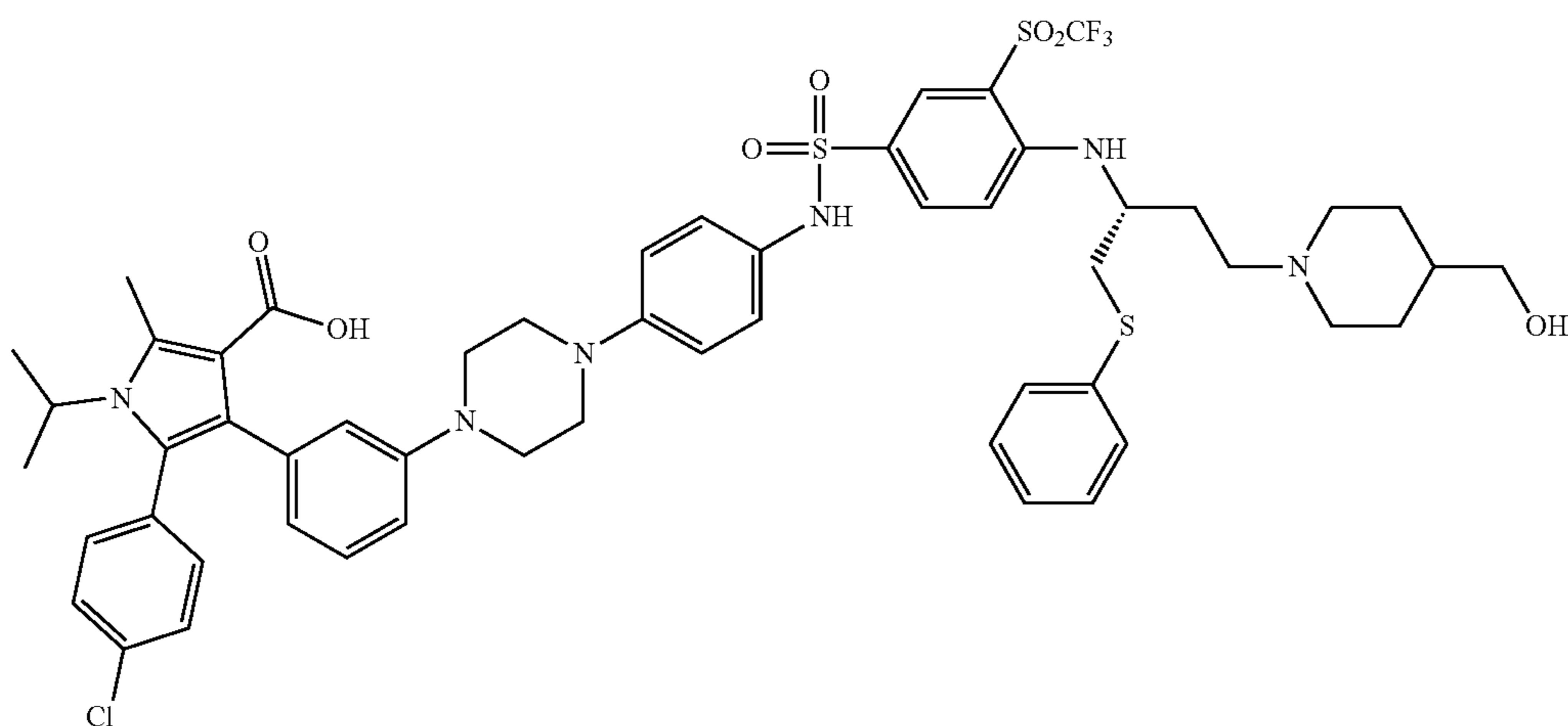
(R)-5-(4-chlorophenyl)-4-(3-(4-(4-((4-(4-(hydroxymethyl)piperidin-1-yl)-1-(phenylthio)butan-2-yl)amino)-3-((trifluoromethyl)sulfonyl)phenyl)sulfonamido)phenyl)piperazin-1-yl)phenyl)-1-isopropyl-2-methyl-1H-pyrrole-3-carboxylic acid
