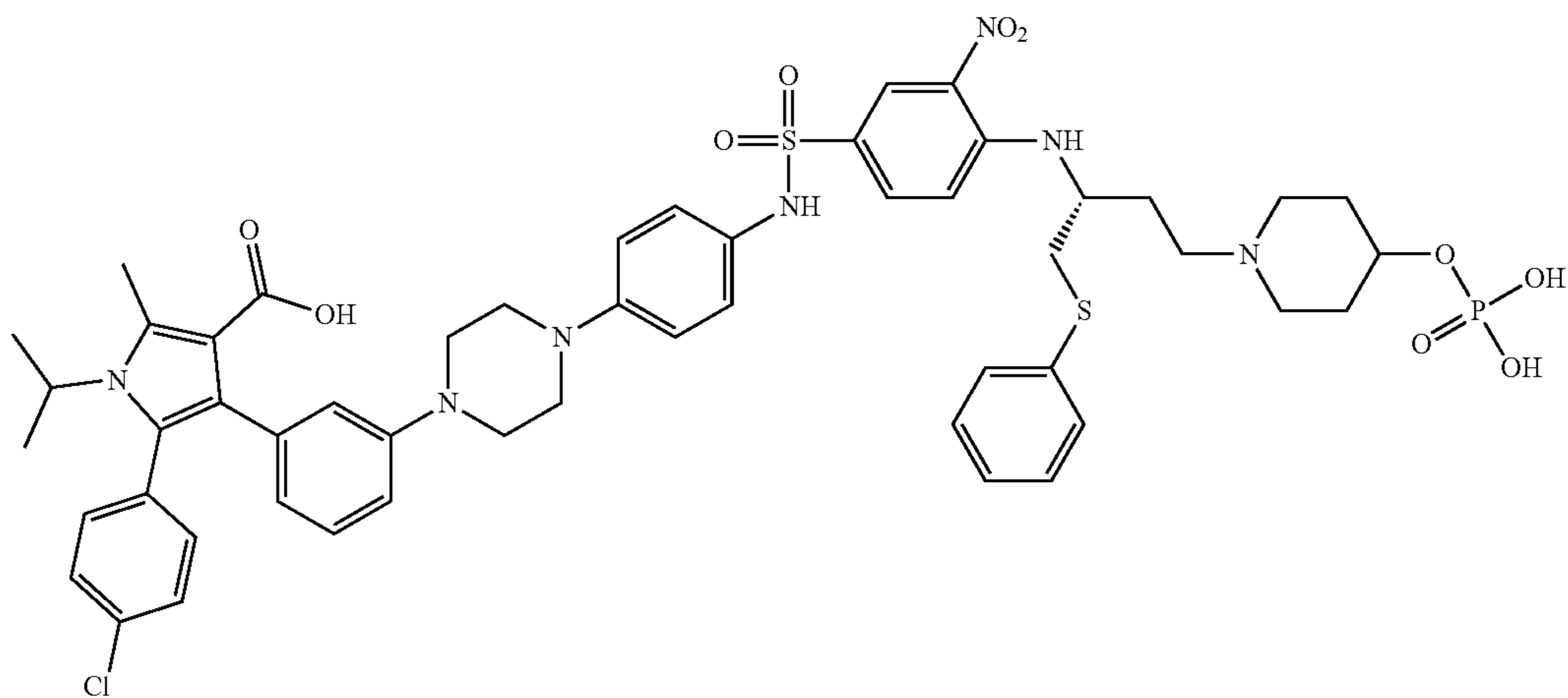
(R)-5-(4-chlorophenyl)-1-isopropyl-2-methyl-4-(3-(4-(4-((3-nitro-4-((1-(phenylthio)-4-(4-(phosphonoxy)piperidin-1-yl)butan-2-yl)amino)phenyl)sulfonamido)phenyl)piperazin-1-yl)phenyl)-1H-pyrrole-3-carboxylic acid
