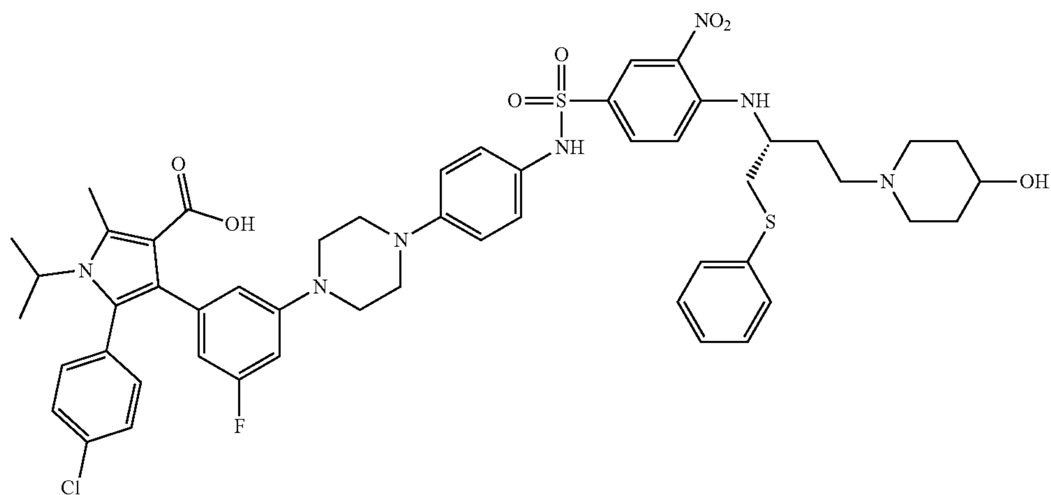
(R)-5-(4-chlorophenyl)-4-(3-fluoro-5-(4-(4-((4-(4-hydroxypiperidin-1-yl)-1-(phenylthio)butan-2-yl)amino)-3-nitrophenyl)sulfonamido)phenyl)piperazin-1-yl)phenyl)-1-isopropyl-2-methyl-1H-pyrrole-3-carboxylic acid
