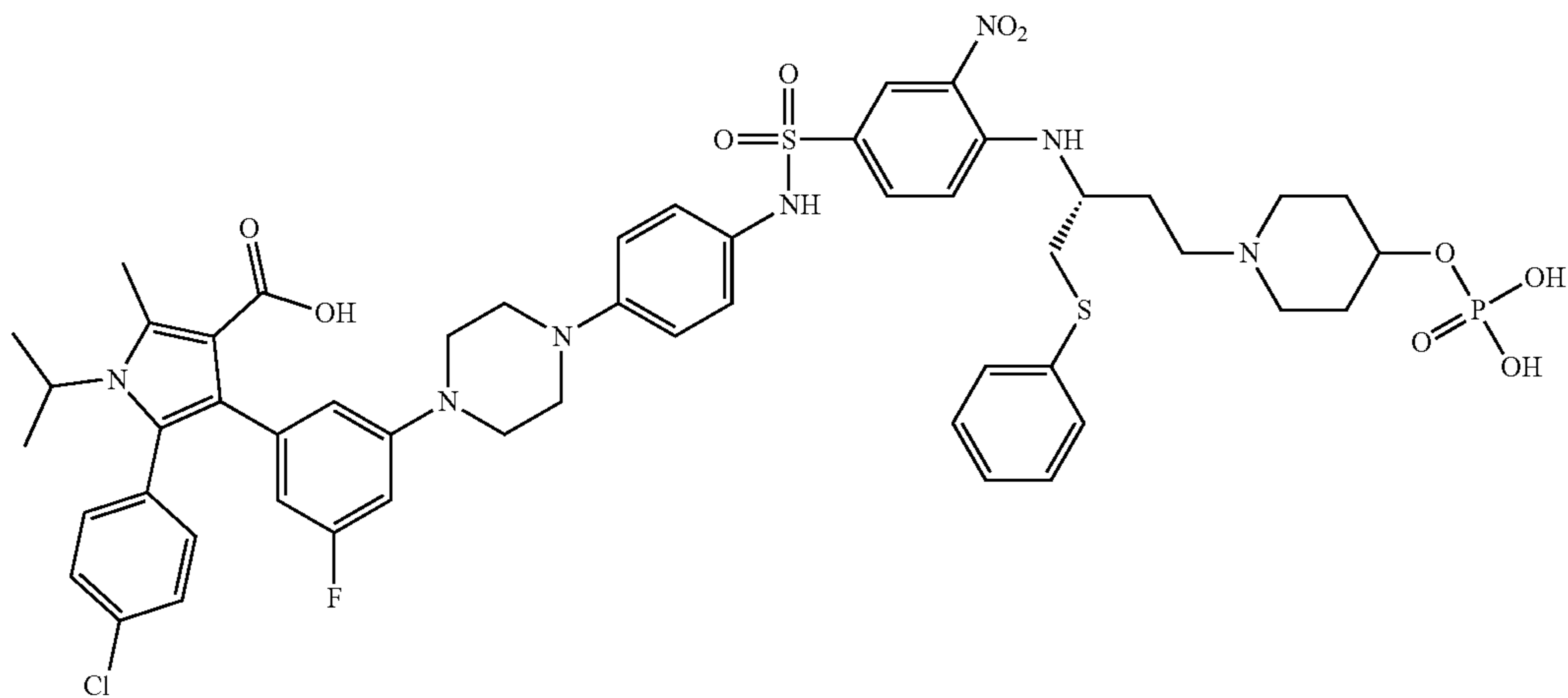
(R)-5-(4-chlorophenyl)-4-(3-fluoro-5-(4-(4-((3-nitro-4-((1-(phenylthio)-4-(4-(phosphonoxy)piperidin-1-yl)butan-2-yl)amino)phenyl)sulfonamido)phenyl)piperazin-1-yl)phenyl)-1-isopropyl-2-methyl-1H-pyrrole-3-carboxylic acid
