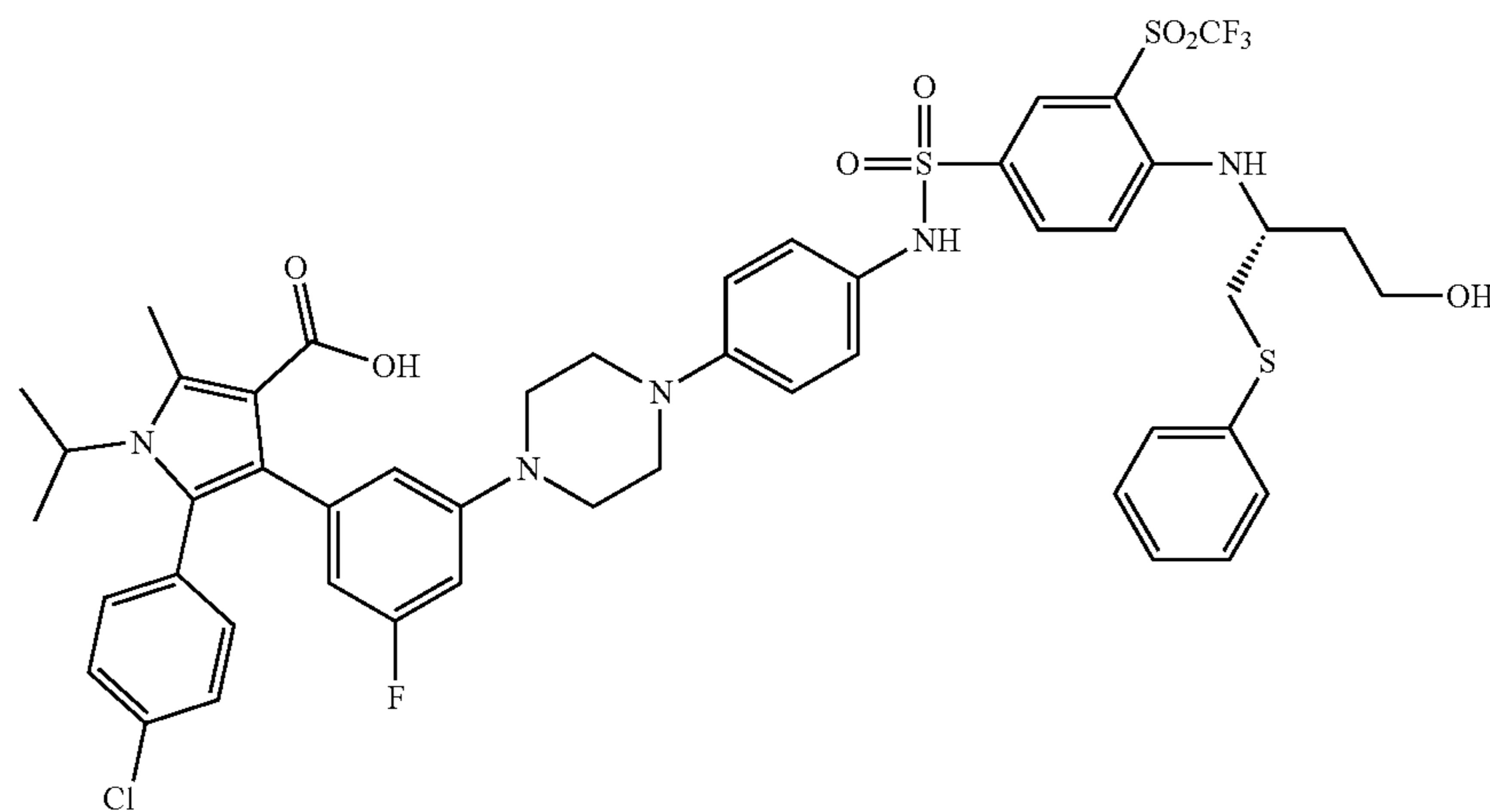
(R)-5-(4-chlorophenyl)-4-(3-fluoro-5-(4-(4-((4-(4-(hydroxy-1-(phenylthio)butan-2-yl)amino)-3-(trifluoromethyl)sulfonyl)phenyl)sulfonamido)phenyl)piperazin-1-yl)phenyl)-1-isopropyl-2-methyl-1H-pyrrole-3-carboxylic acid
