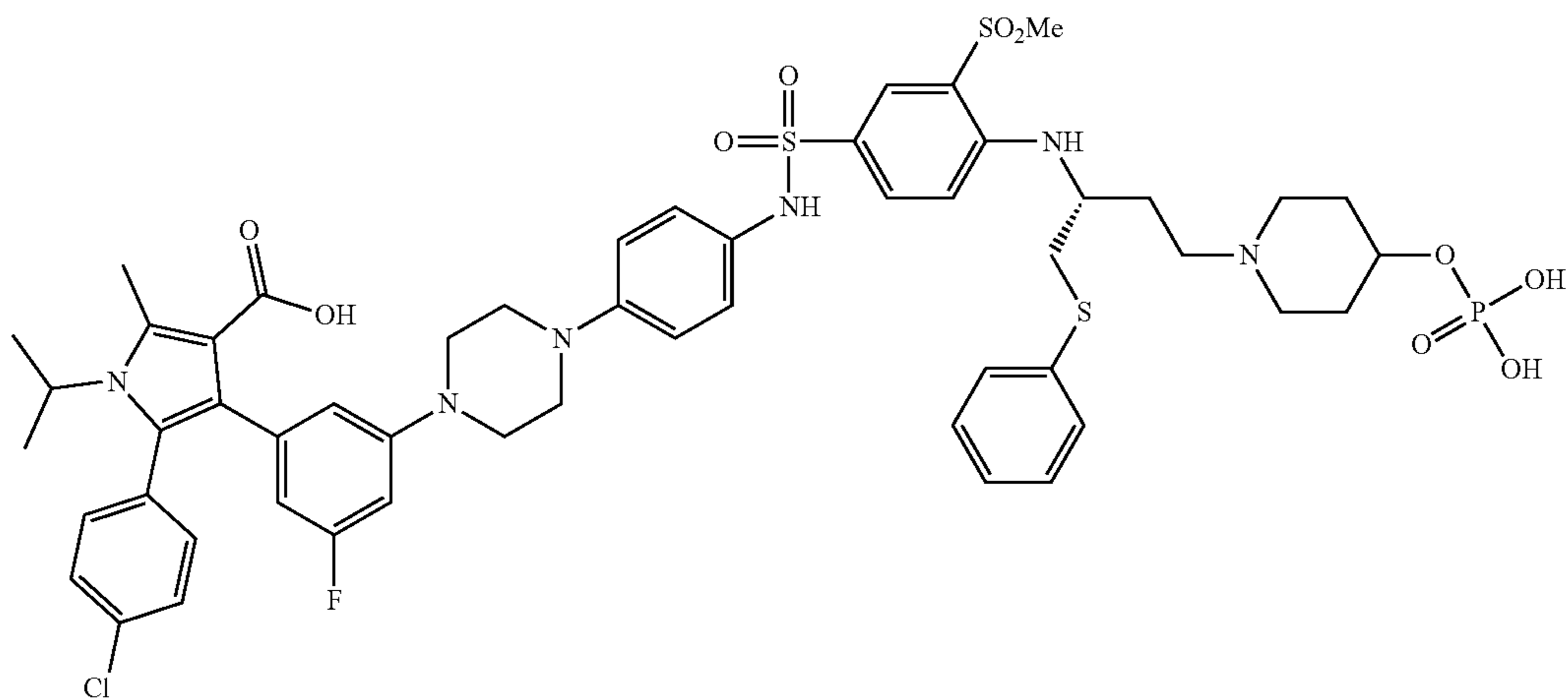
(R)-5-(4-chlorophenyl)-4-(3-fluoro-5-(4-(4-((3-(methylsulfonyl)-4-((1-(phenylthio)-4-(4-(phosphonoxy)piperidin-1-yl)butan-2-yl)amino)phenyl)sulfonamido)phenyl)piperazin-1-yl)phenyl)-1-isopropyl-2-methyl-1H-pyrrole-3-carboxylic acid
