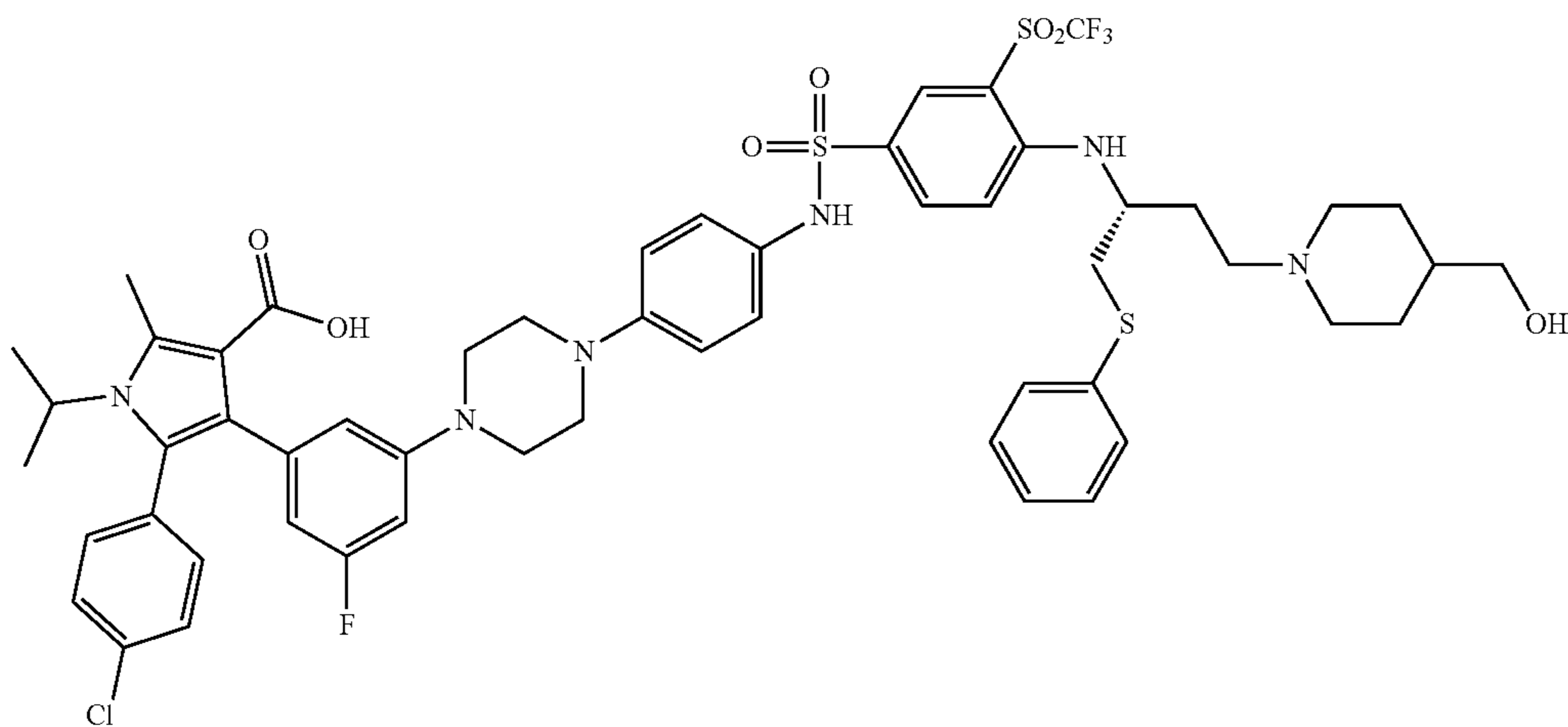
(R)-5-(4-chlorophenyl)-4-(3-fluoro-5-(4-(4-((4-(4-(hydroxymethyl)piperidin-1-yl)-1-(phenylthio)butan-2-yl)amino)-3-((trifluoromethyl)sulfonyl)phenyl)sulfonamido)phenyl)piperazin-1-yl)phenyl)-1-isopropyl-2-methyl-1H-pyrrole-3-carboxylic acid
