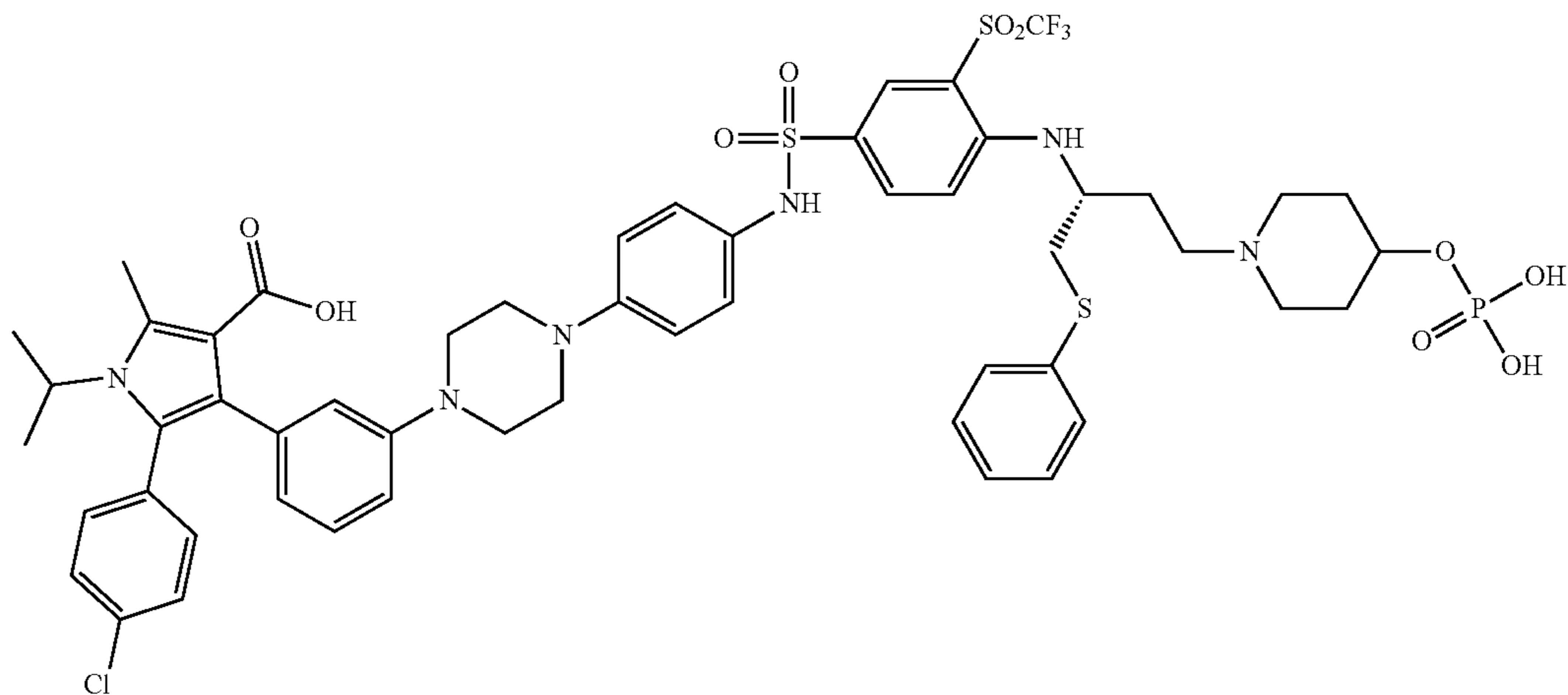
(R)-5-(4-chlorophenyl)-1-isopropyl-2-methyl-4-(3-(4-(4-((1-(phenylthio)-4-(4-phosphonoxy)piperidin-1-yl)butan-2-yl)amino)-3-((trifluoromethyl)sulfonyl)phenyl)sulfonamido)phenyl)piperazin-1-yl)phenyl)-1H-pyrrole-3-carboxylic acid
