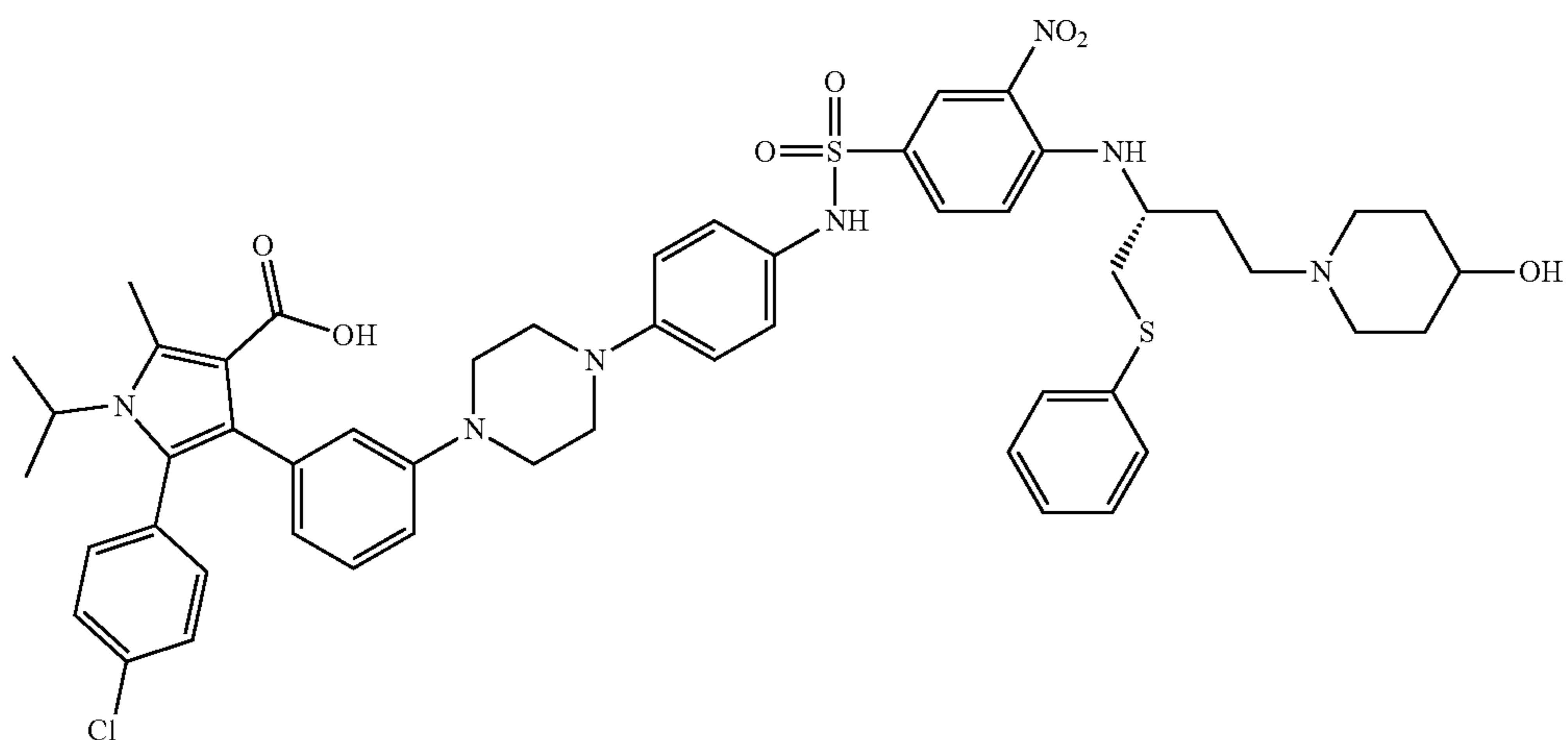
(R)-5-(4-chlorophenyl)-4-(3-(4-(4-((4-(4-hydroxypiperidin-1-yl)-1-(phenylthio)butan-2-yl)amino)-3-nitrophenyl)sulfonamido)phenyl)piperazin-1-yl)phenyl)-1-isopropyl-2-methyl-1H-pyrrole-3-carboxylic acid
