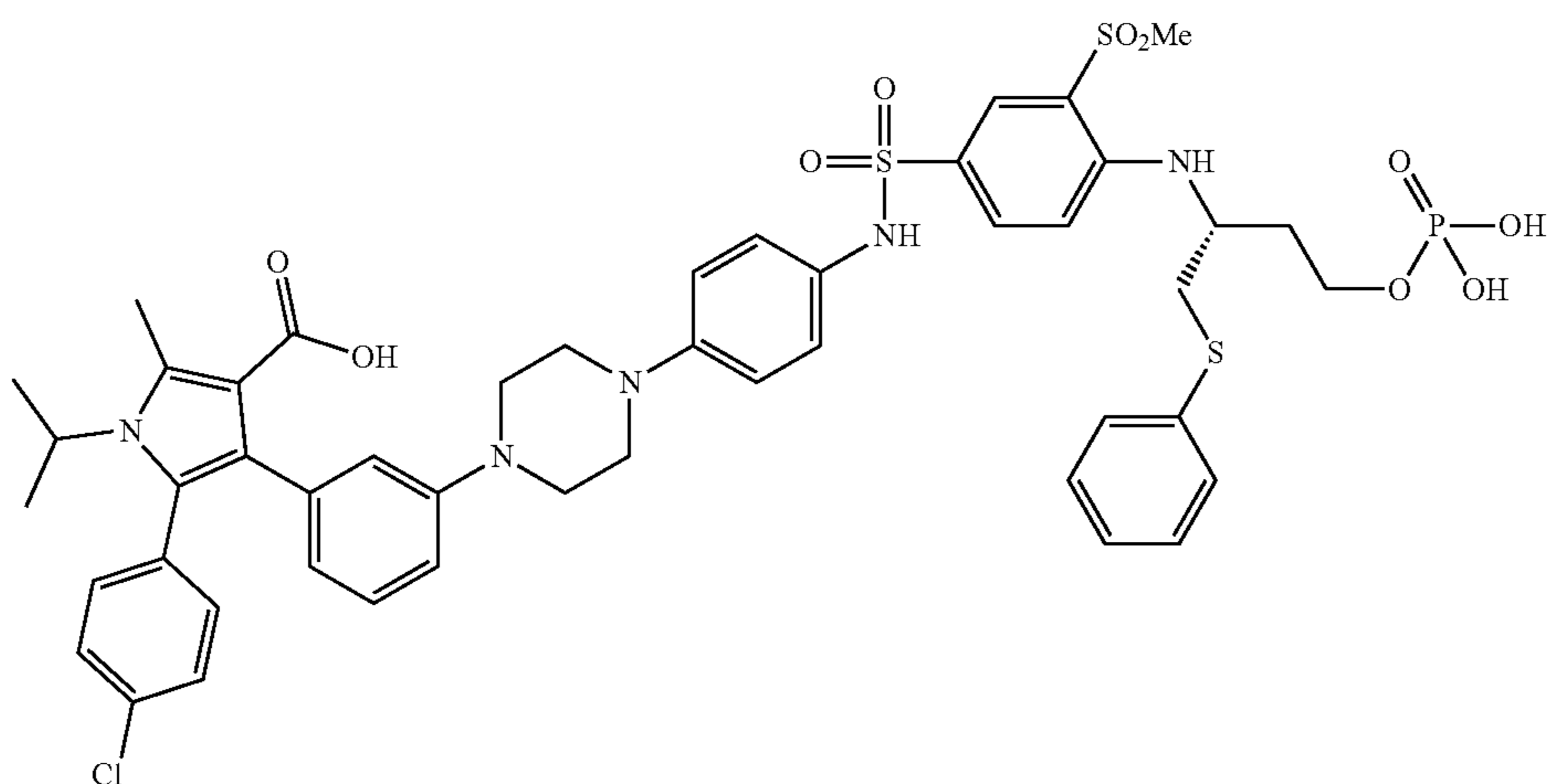
(R)-5-(4-chlorophenyl)-1-isopropyl-2-methyl-4-(3-(4-(4-((3-(methylsulfonyl)-4-((1-(phenylthio)-4-(phosphonooxy)butan-2-yl)amino)phenyl)sulfonamido)phenyl)piperazin-1-yl)phenyl)-1H-pyrrole-3-carboxylic acid
