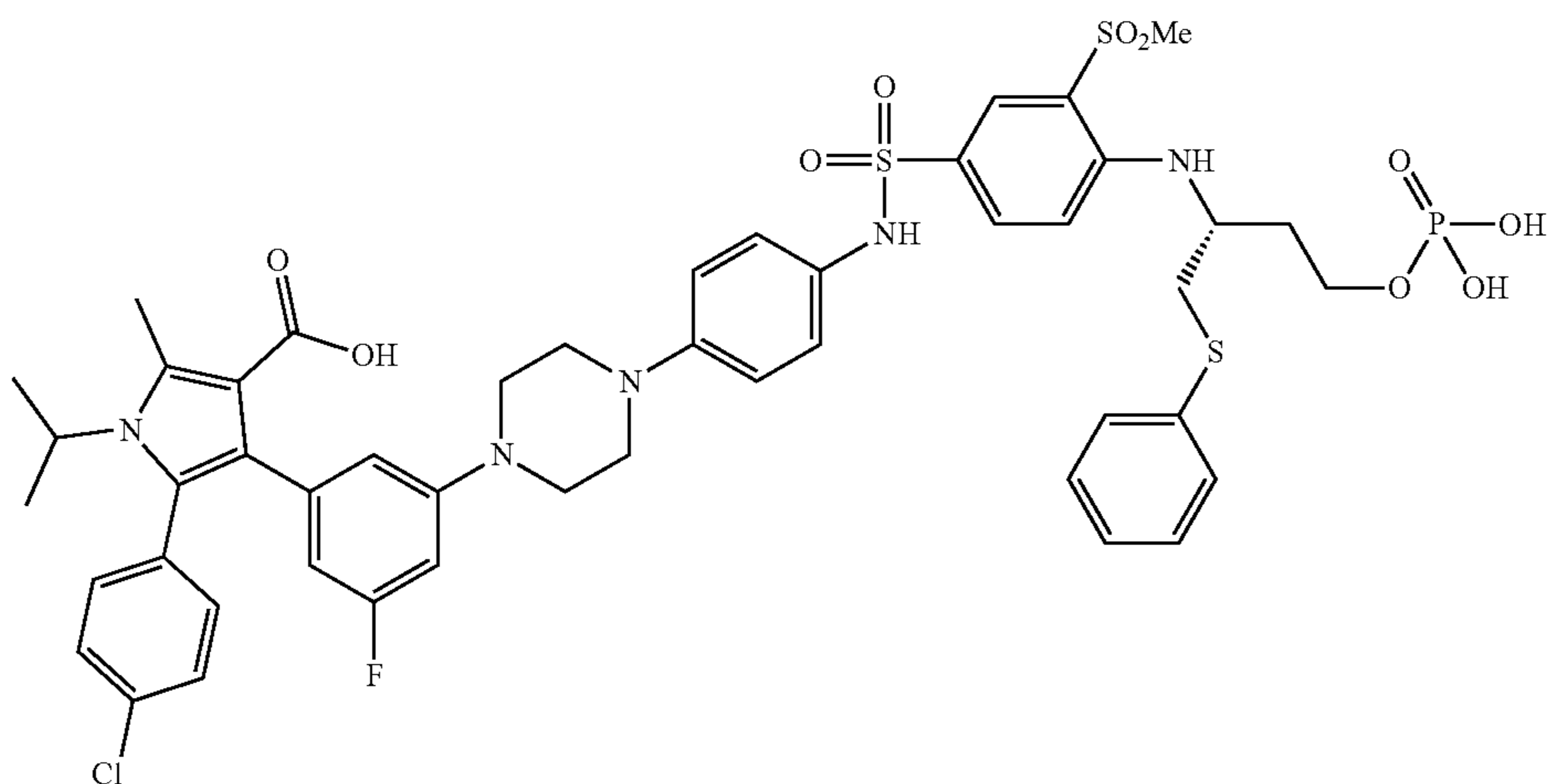
(R)-5-(4-chlorophenyl)-4-(3-fluoro-5-(4-(4-((3-(methylsulfonyl)-4-((1-(phenylthio)-4-(phosphonooxy)butan-2-yl)amino)phenyl)sulfonamido)phenyl)piperazin-1-yl)phenyl)-1-isopropyl-2-methyl-1H-pyrrole-3-carboxylic acid
