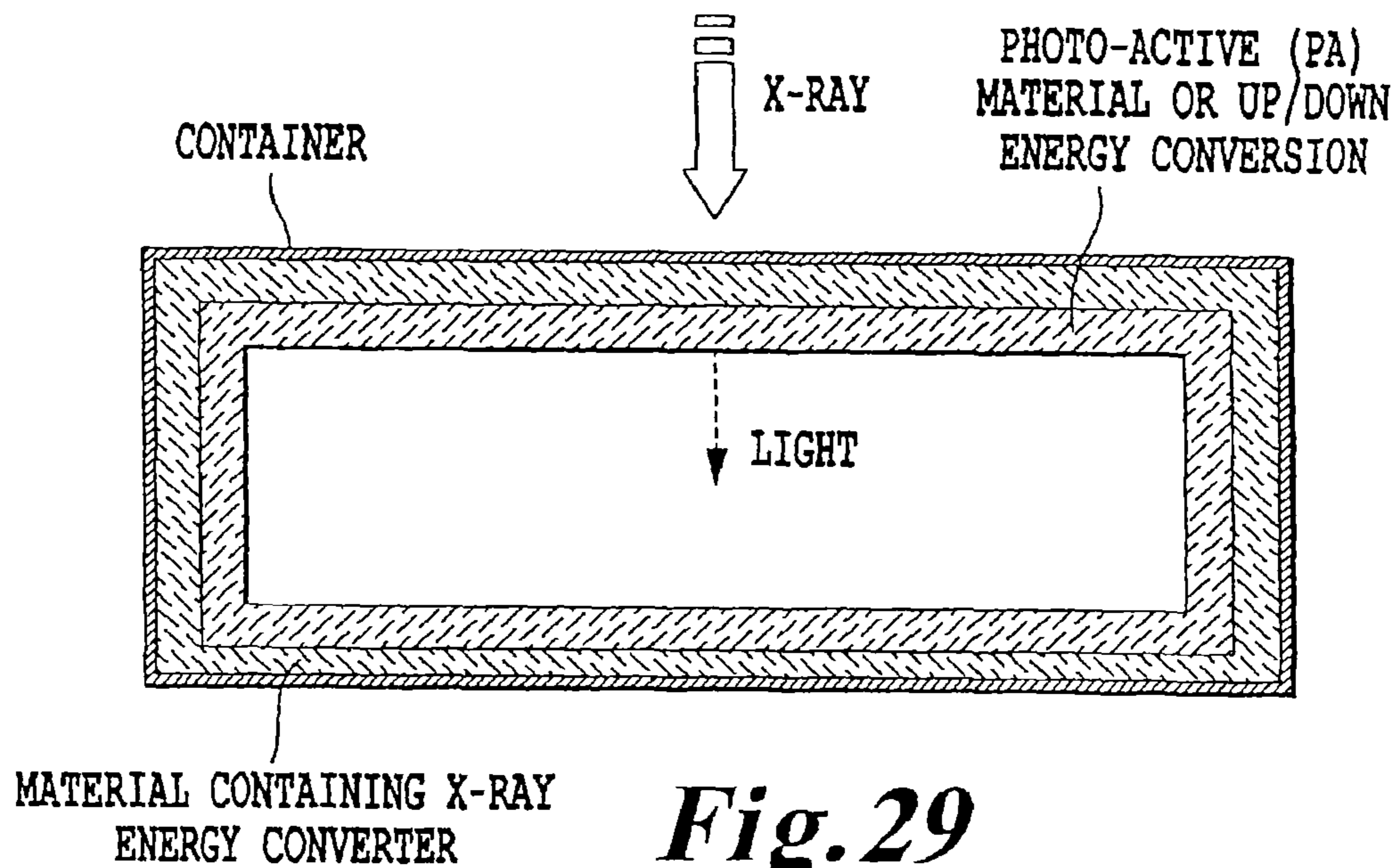
STERILIZATION SYSTEM 3
