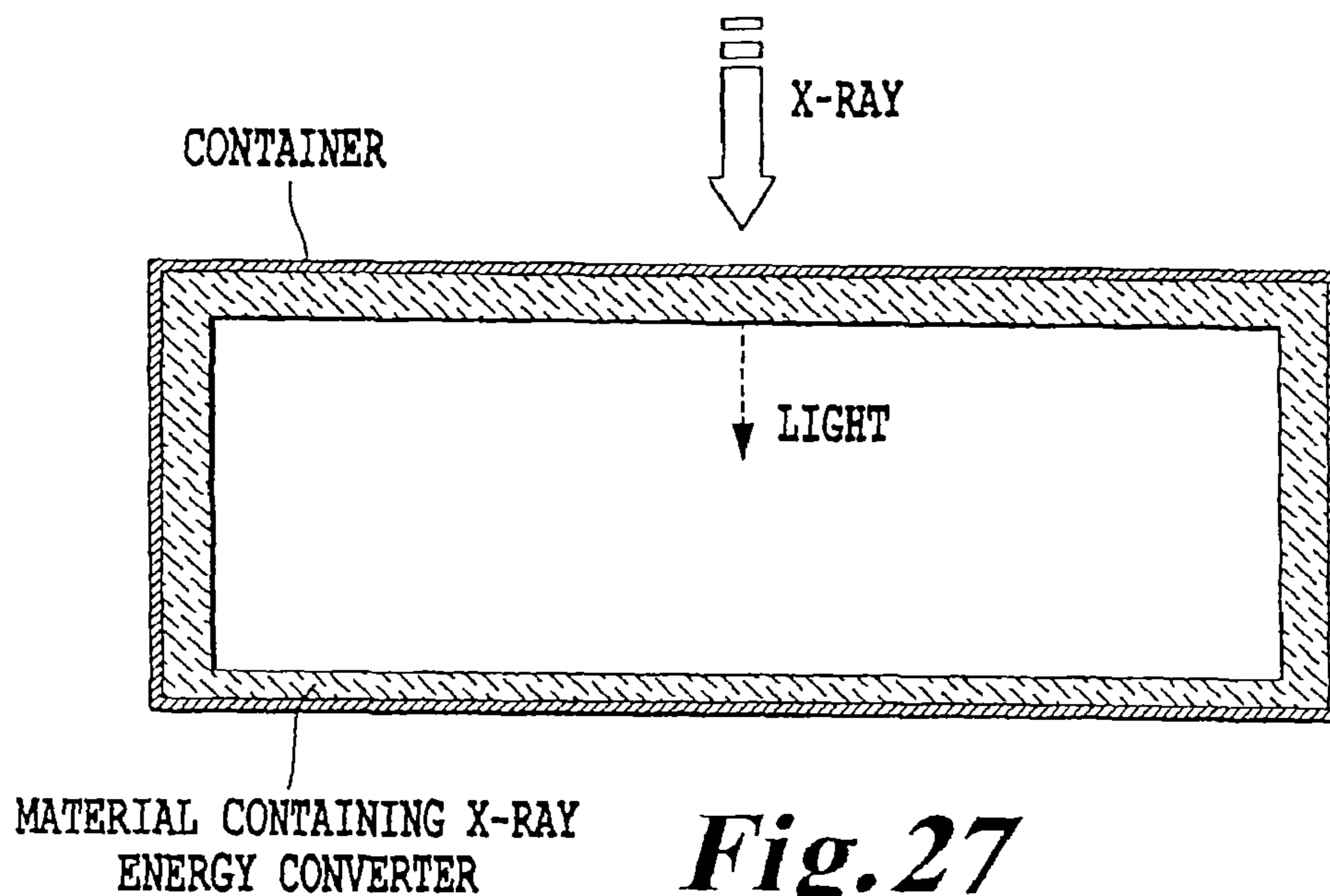
STERILIZATION SYSTEM 1
