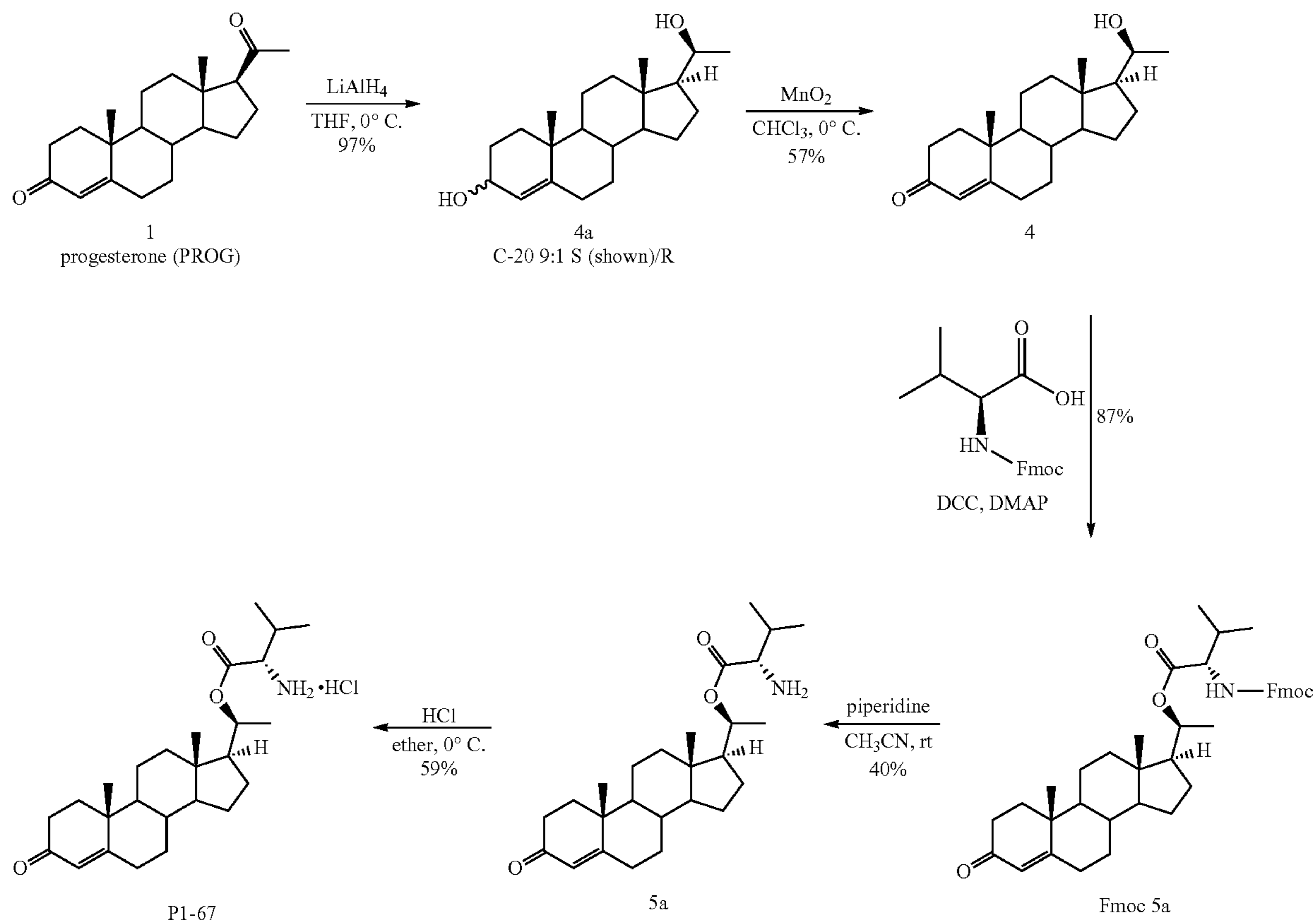
Scheme 15
