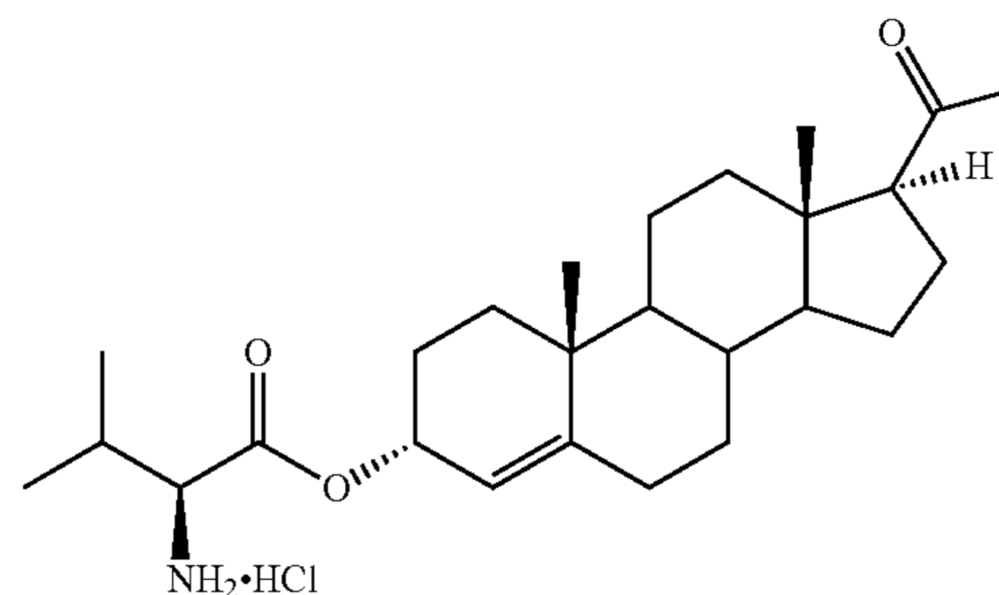
3a-L-Valine-progesterone-HCl (P1-163)
