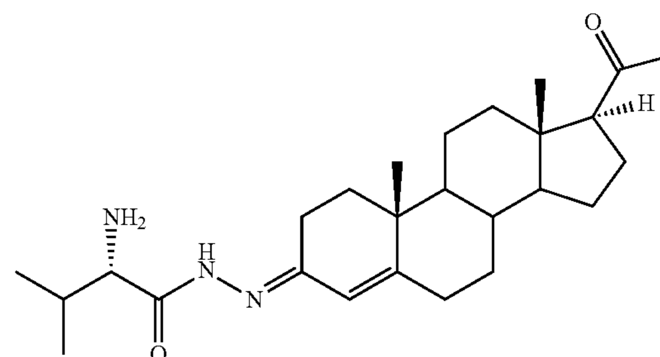
3-Valine-hydrazide-progesterone (35)
