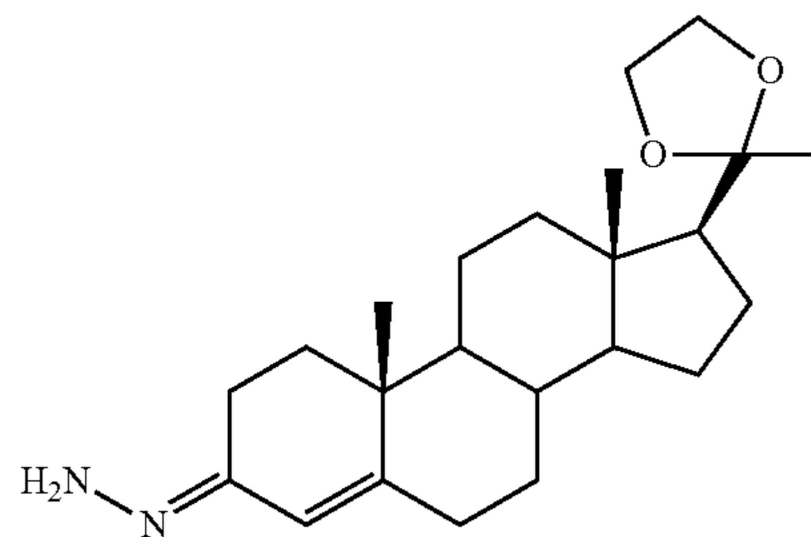
3-Hydrazine-20-ketal-progesterone (10)
