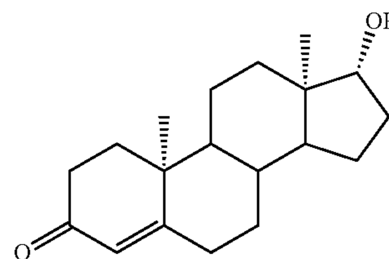
ent-Testosterone (53)
