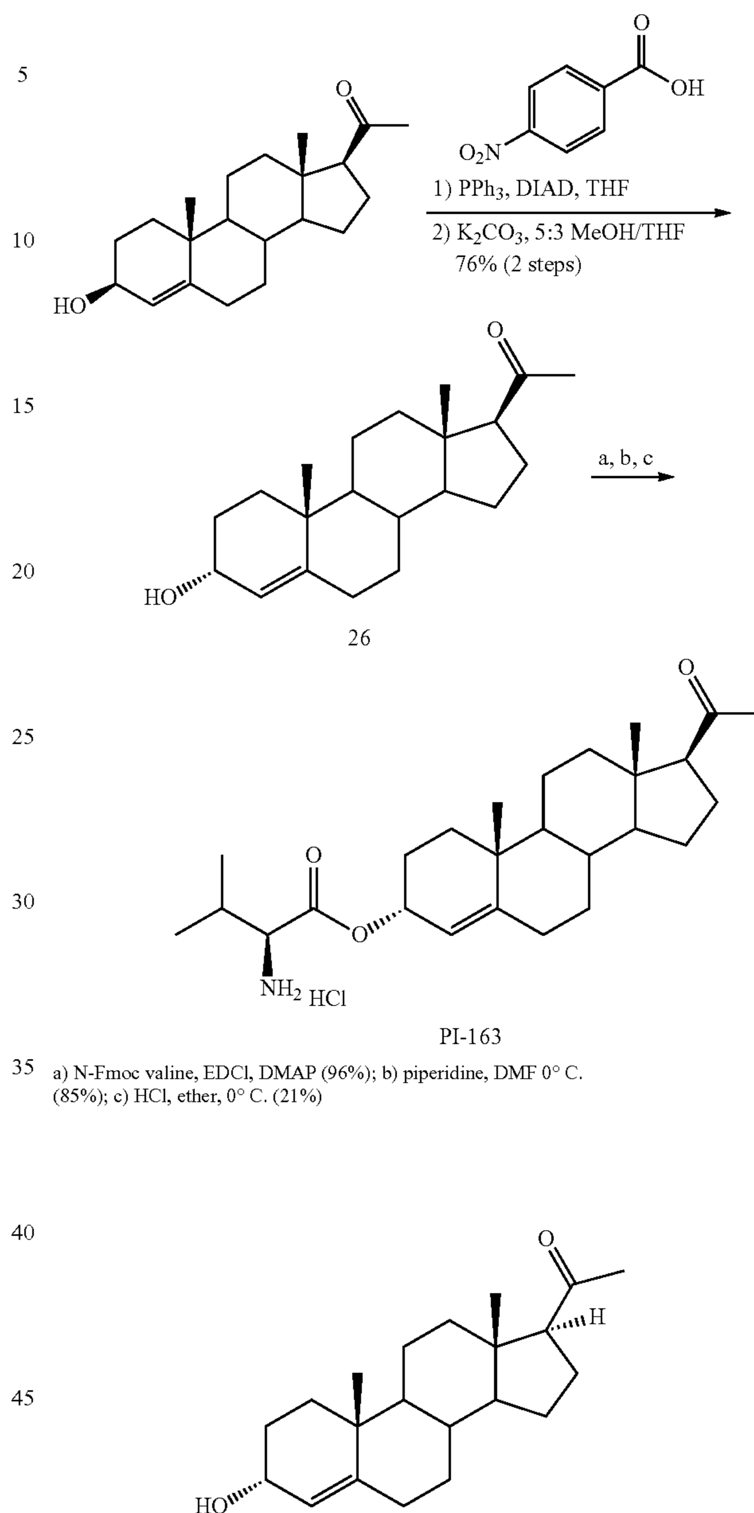
Scheme 14
