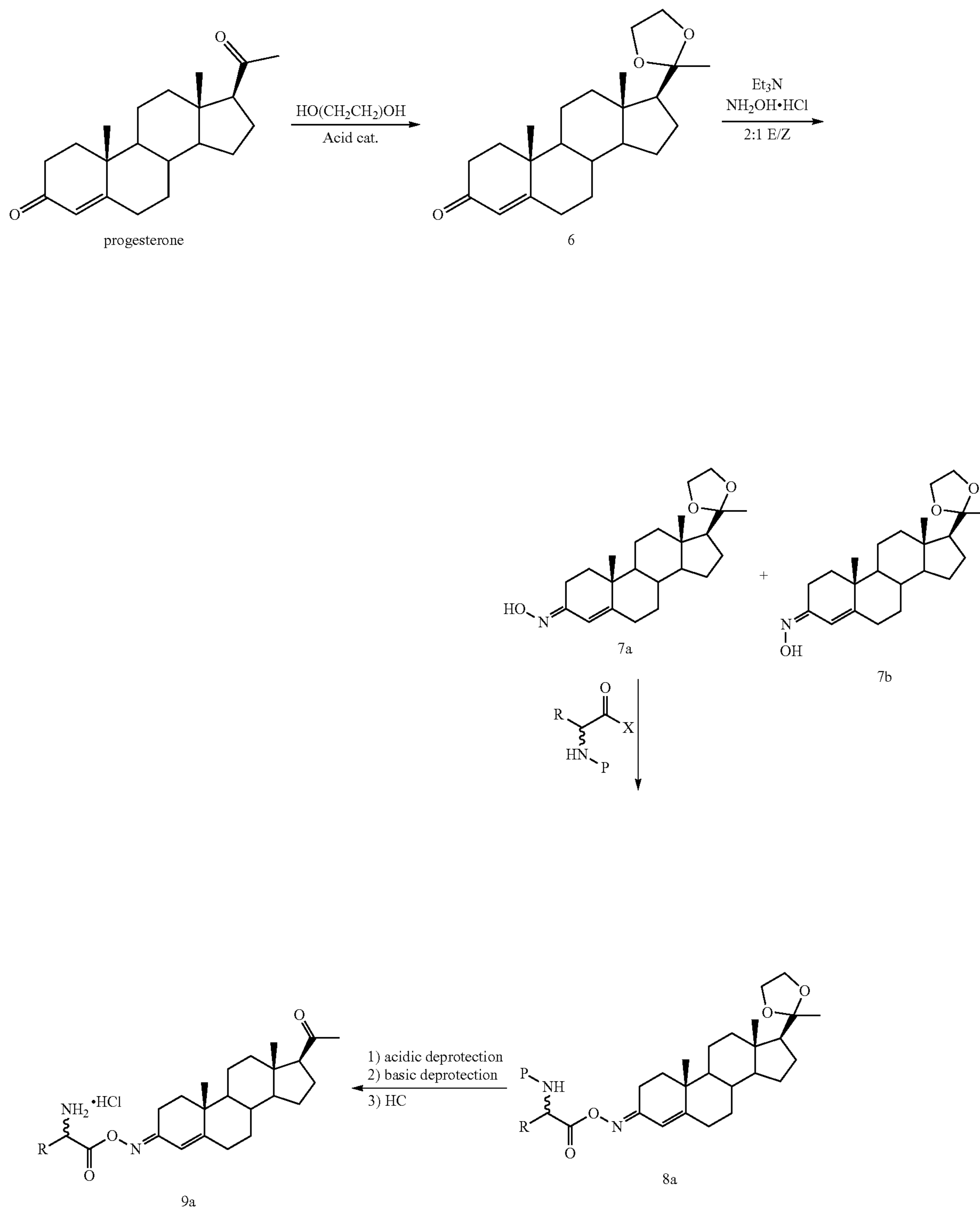
Scheme 3
