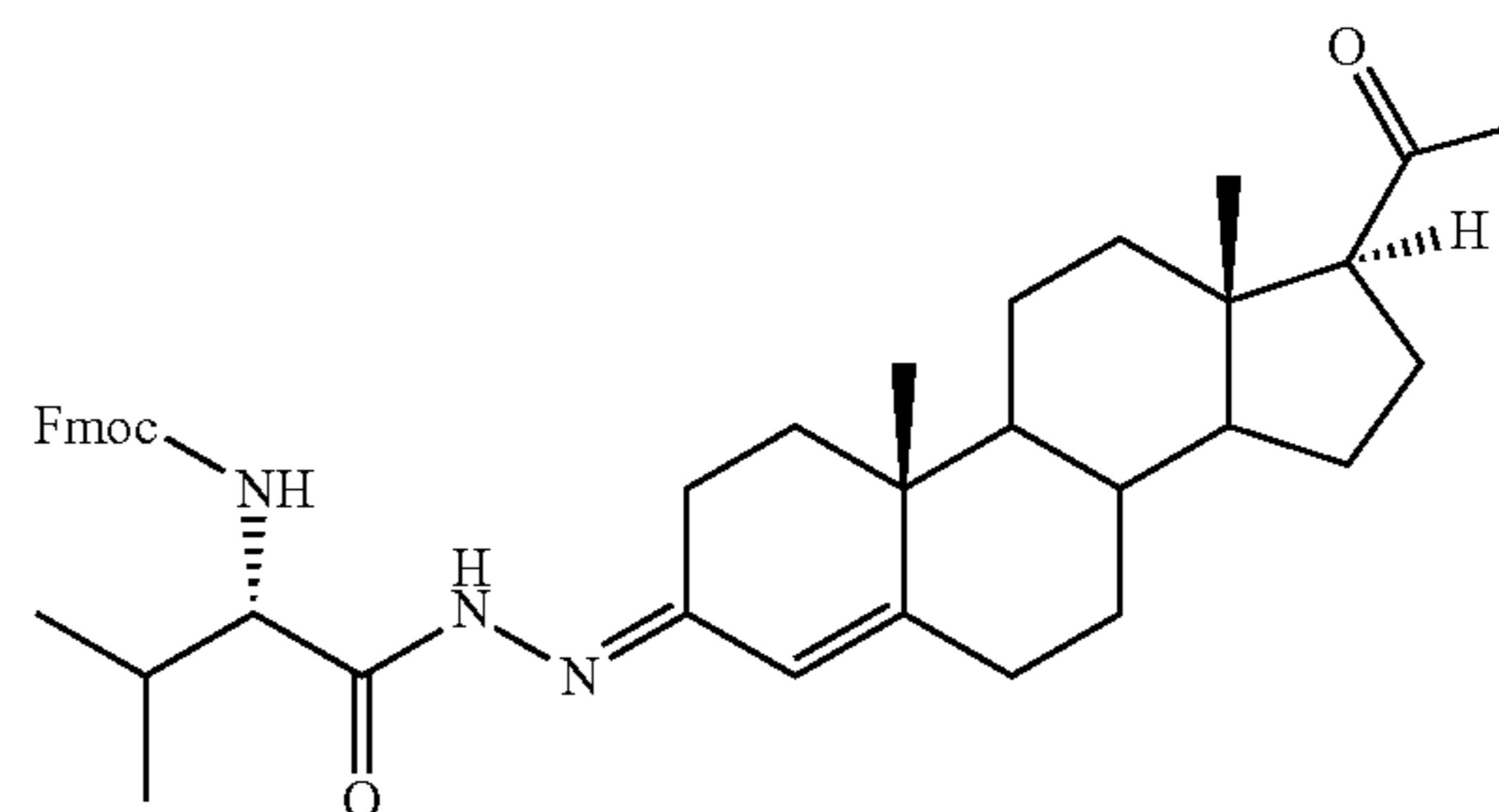
N-Fmoc-valine-3-hydrazide-progesterone (34)
