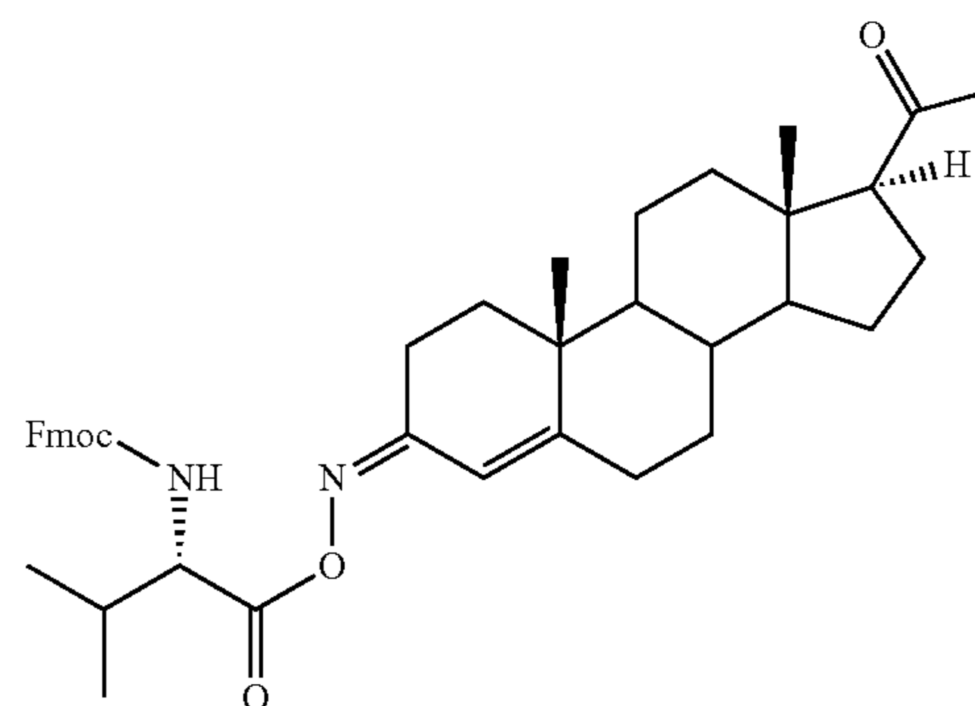
N-Fmoc-valine-3-Z-oxime-progesterone (32)
