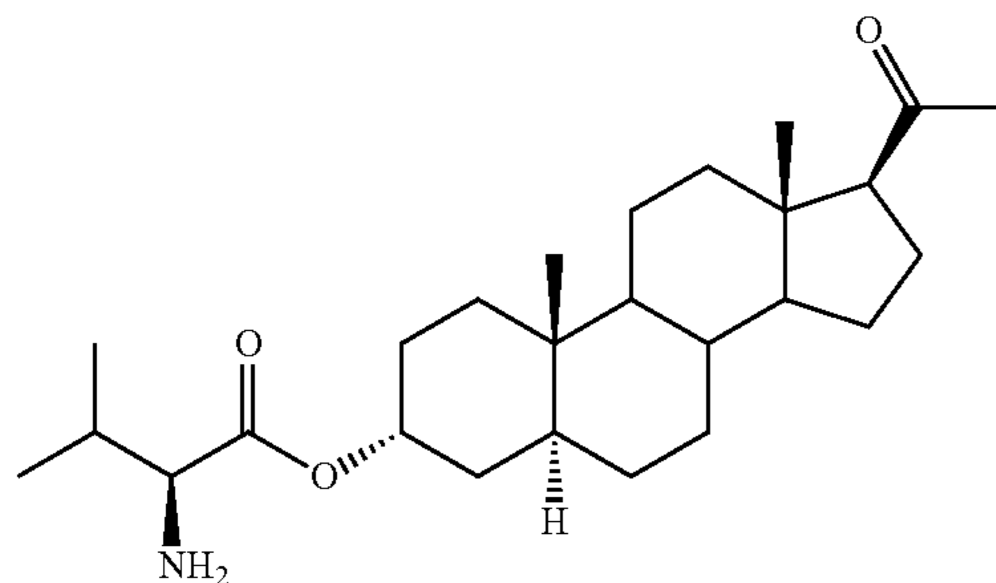
3α-L-Valine-5α-pregnan-20-one (15a)
