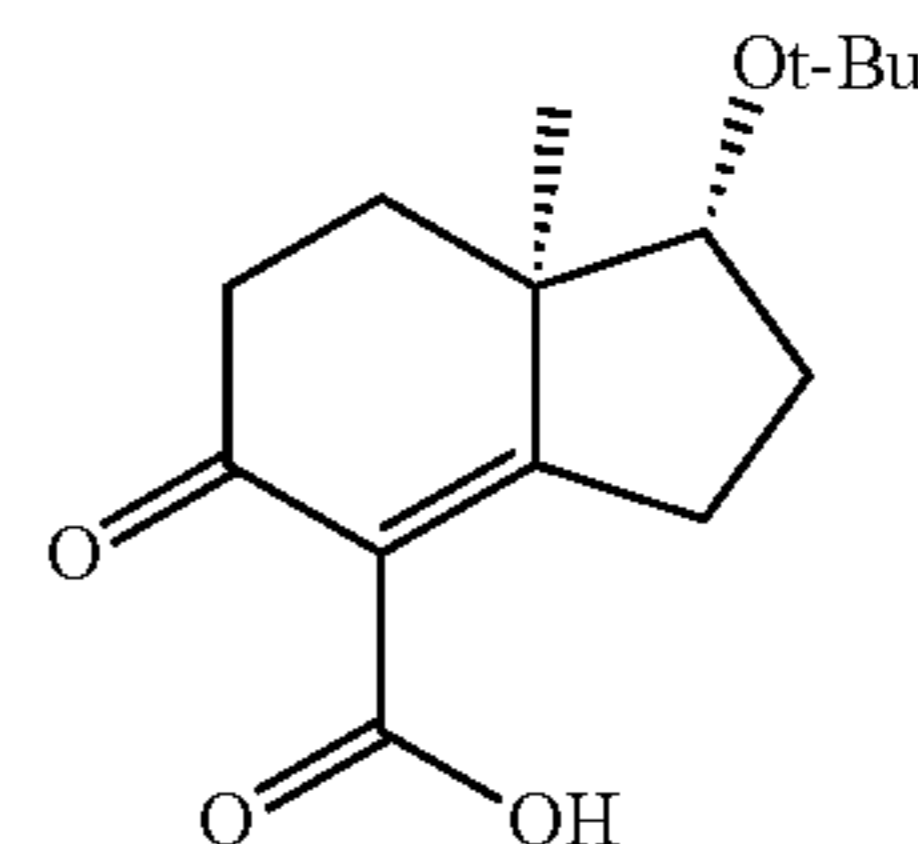
(-)-(1R,7aR)-5,6,7,7a-Tetrahydro-1-tert-butoxy-7a-methyl-5-oxo-4-indancarboxylic acid (43)
