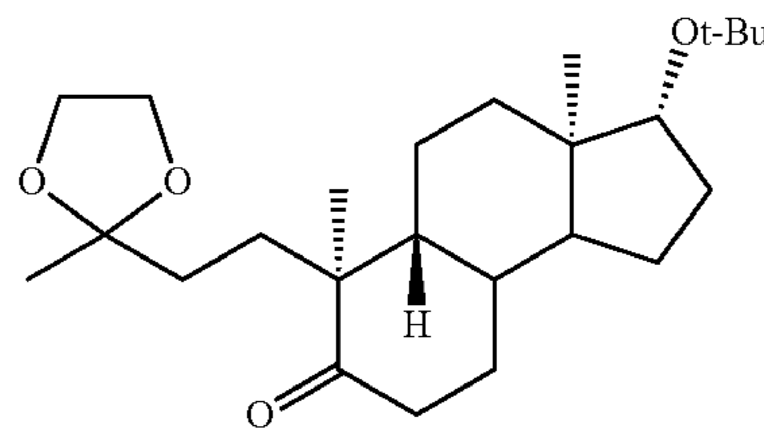
(-)-30-ter-Butoxy-3a,5a-dimethyl-1,2,3,3a,4,5,5a,6,8,9,9a,9a-dodecahydro-6-[2-(2-methyl-1,3-dioxolan-2-yl)ethyl]-7H-benz[c]inden-7-one (52)
