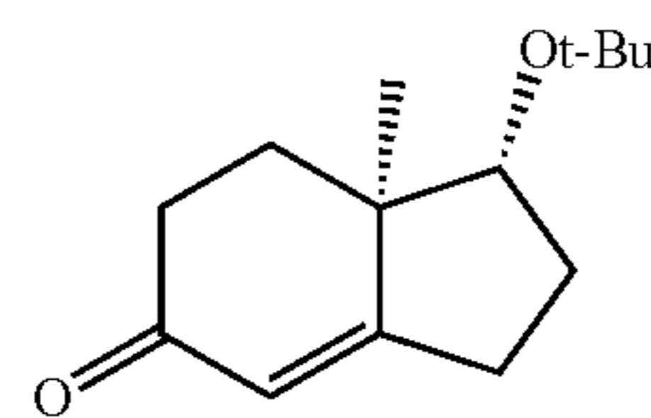
(1R,7aR)-1-tert-Butoxy-7a-methyl-1,2,3,6,7,7a-hexahydro-inden-5-one (41)
