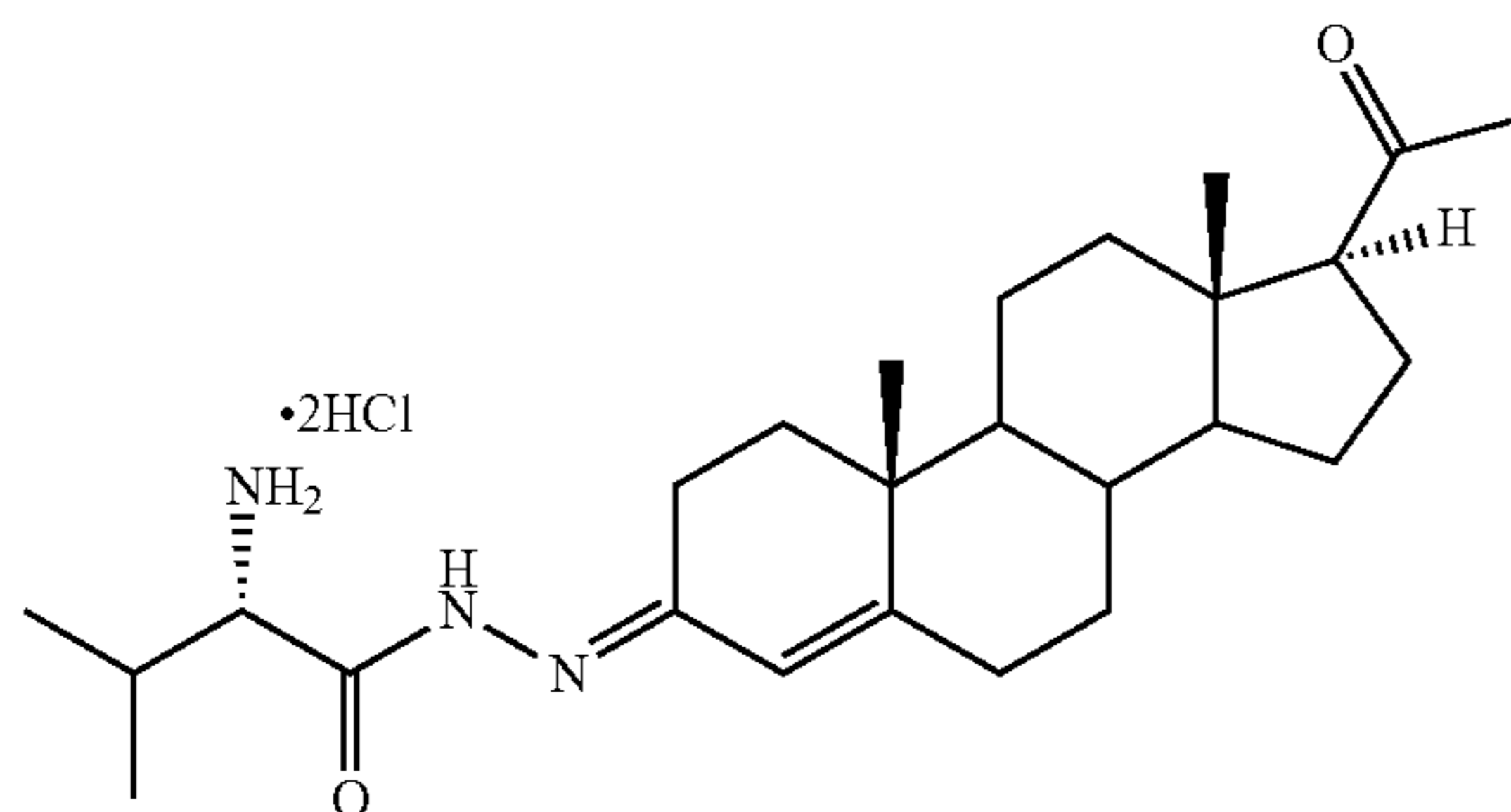
3-Valine-hydrazide-progesterone (P2-29)
