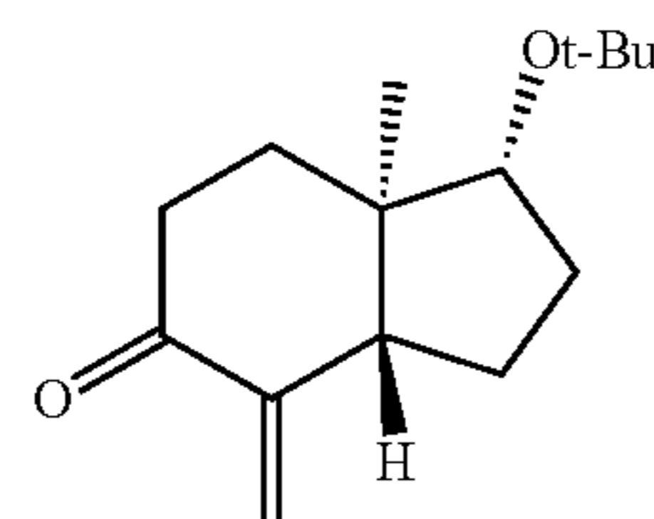
(-)-(1R,3aS,7aR)-1-tert-Butoxy-7a-methyl-3a,6,7,7a-tetrahydro-4-methyleneindan-5(4H)-one (45)
