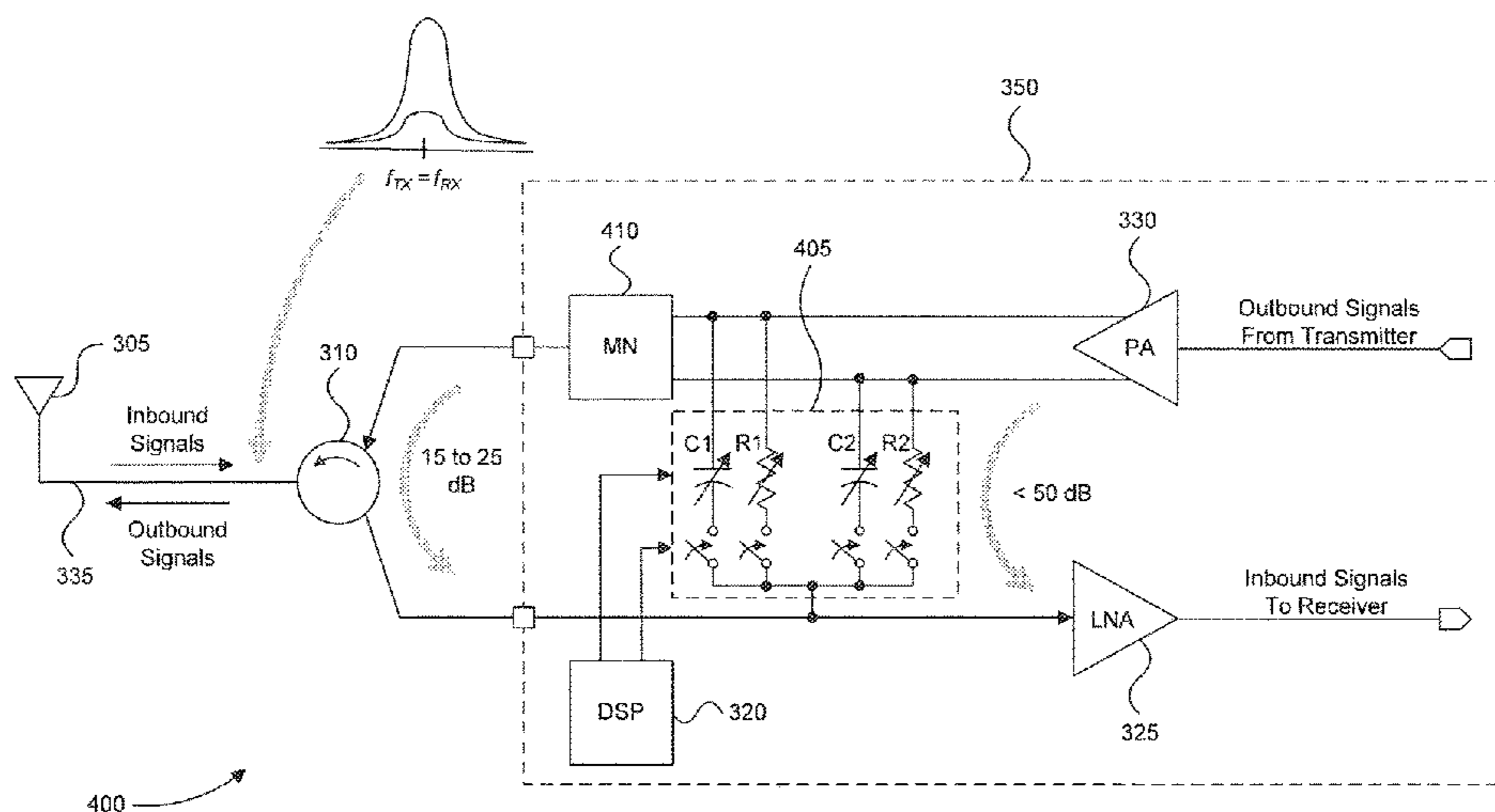
(Self-Interference Cancellation)
