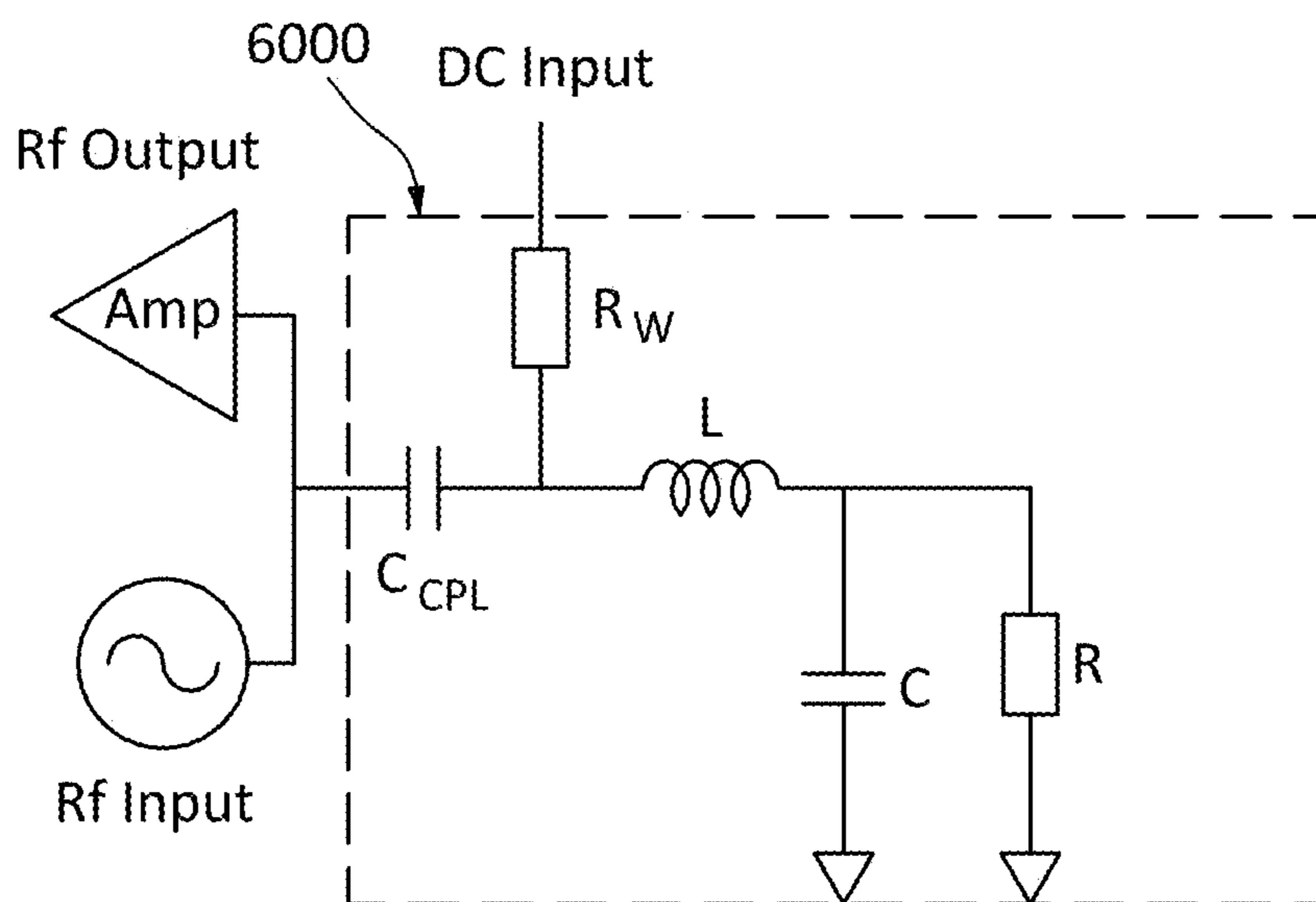
"Bias tee" setup
