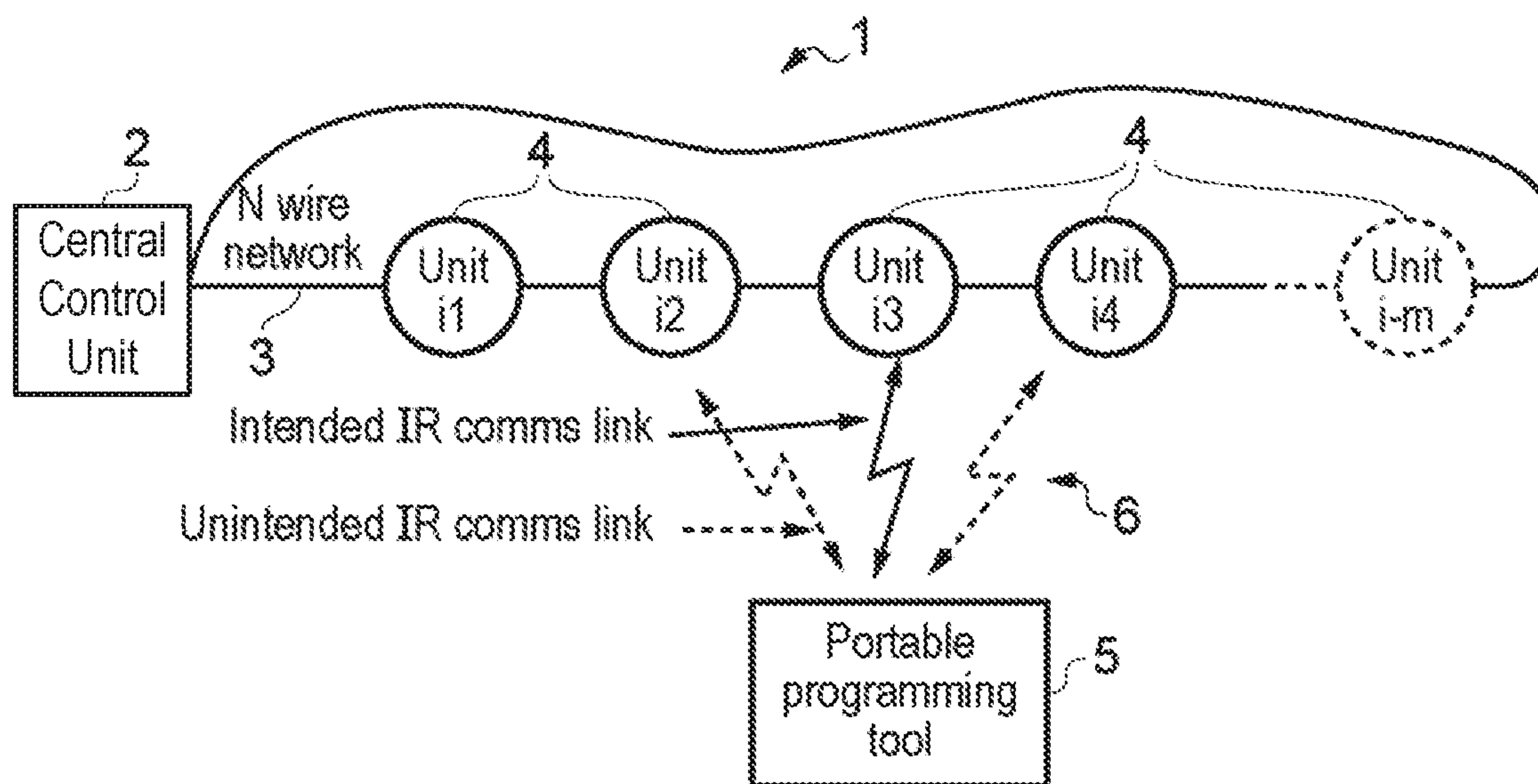
System level overview block diagram
