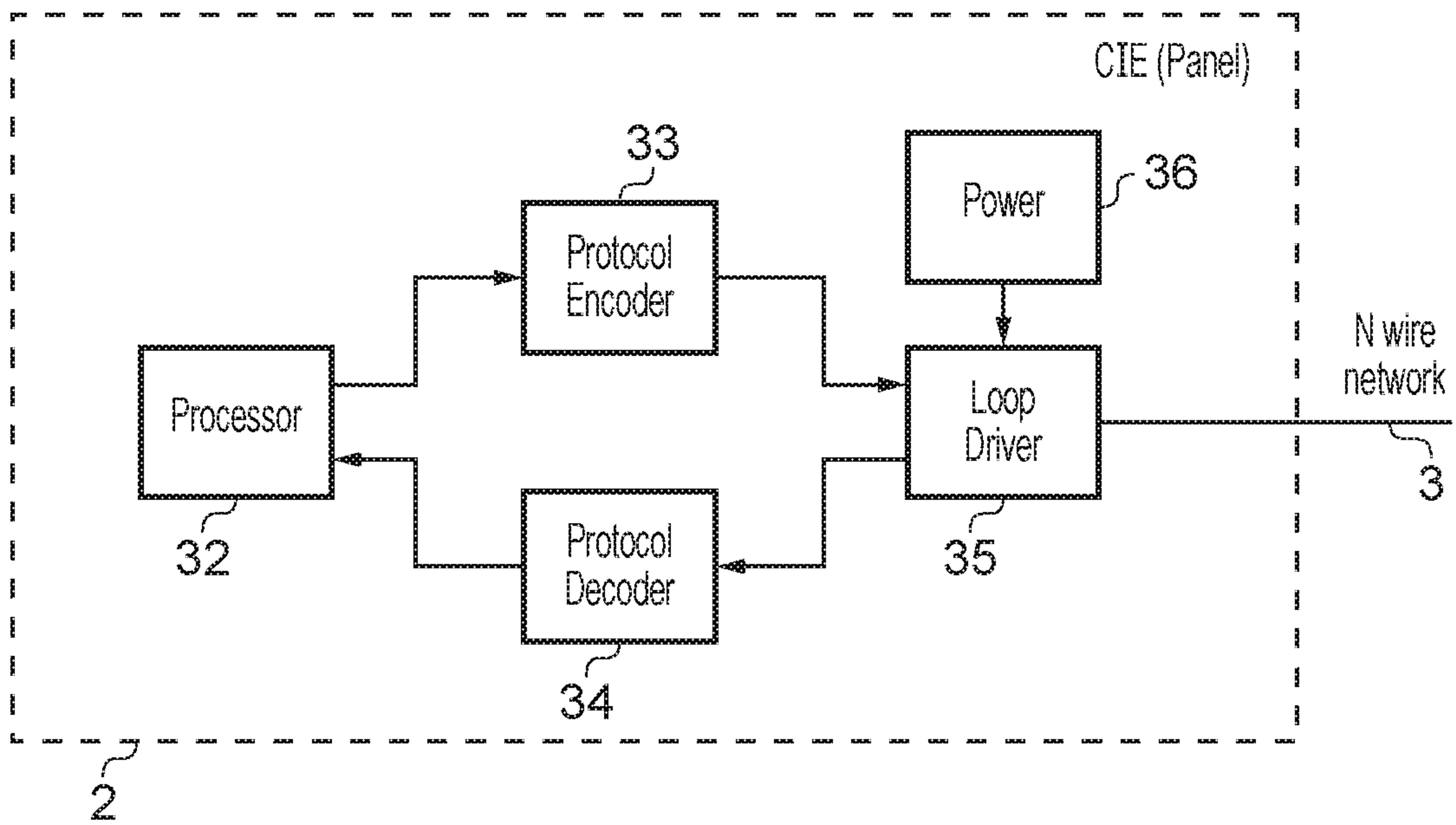
Block diagram of Control and Indicating Equipment
