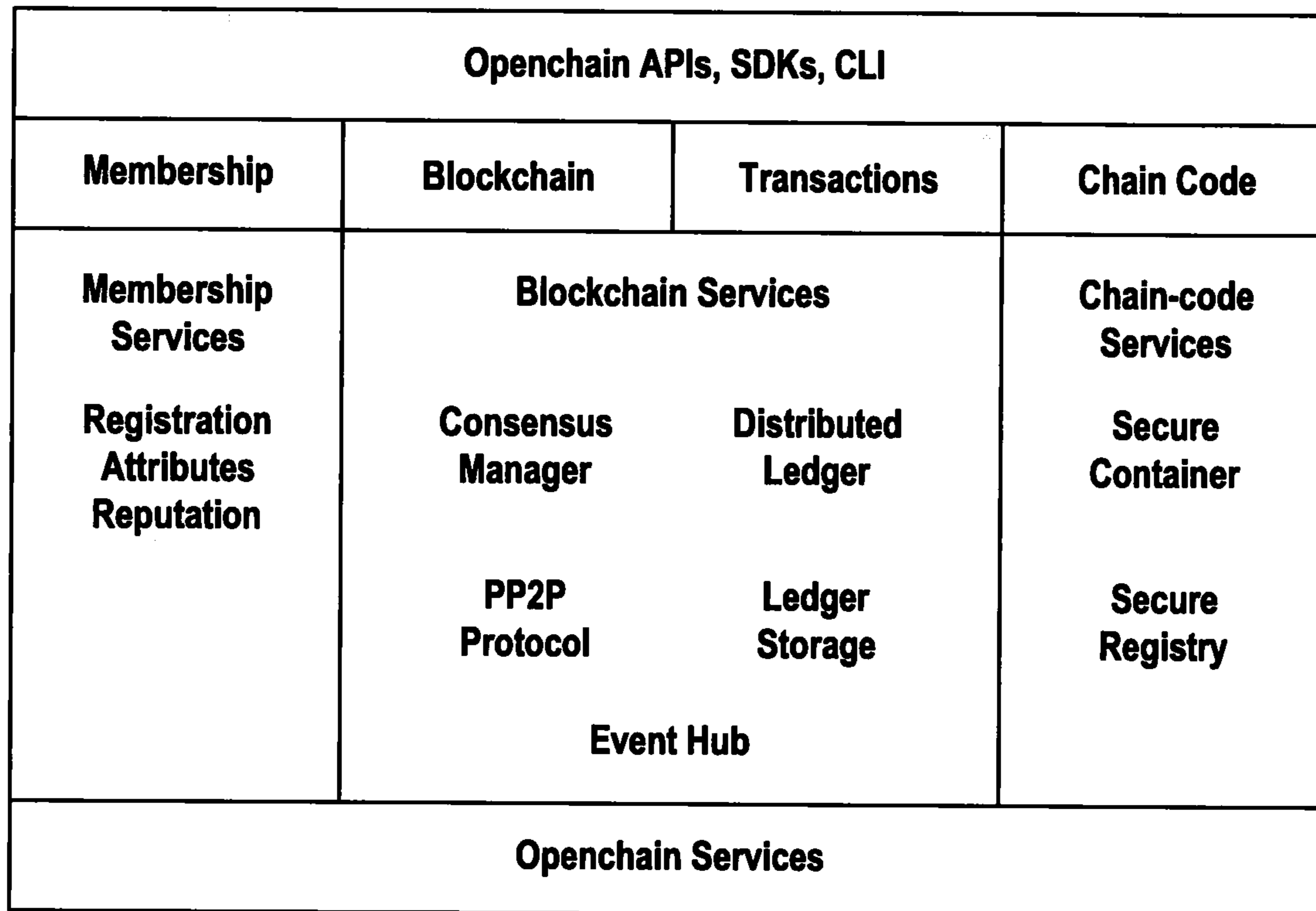
Platform
