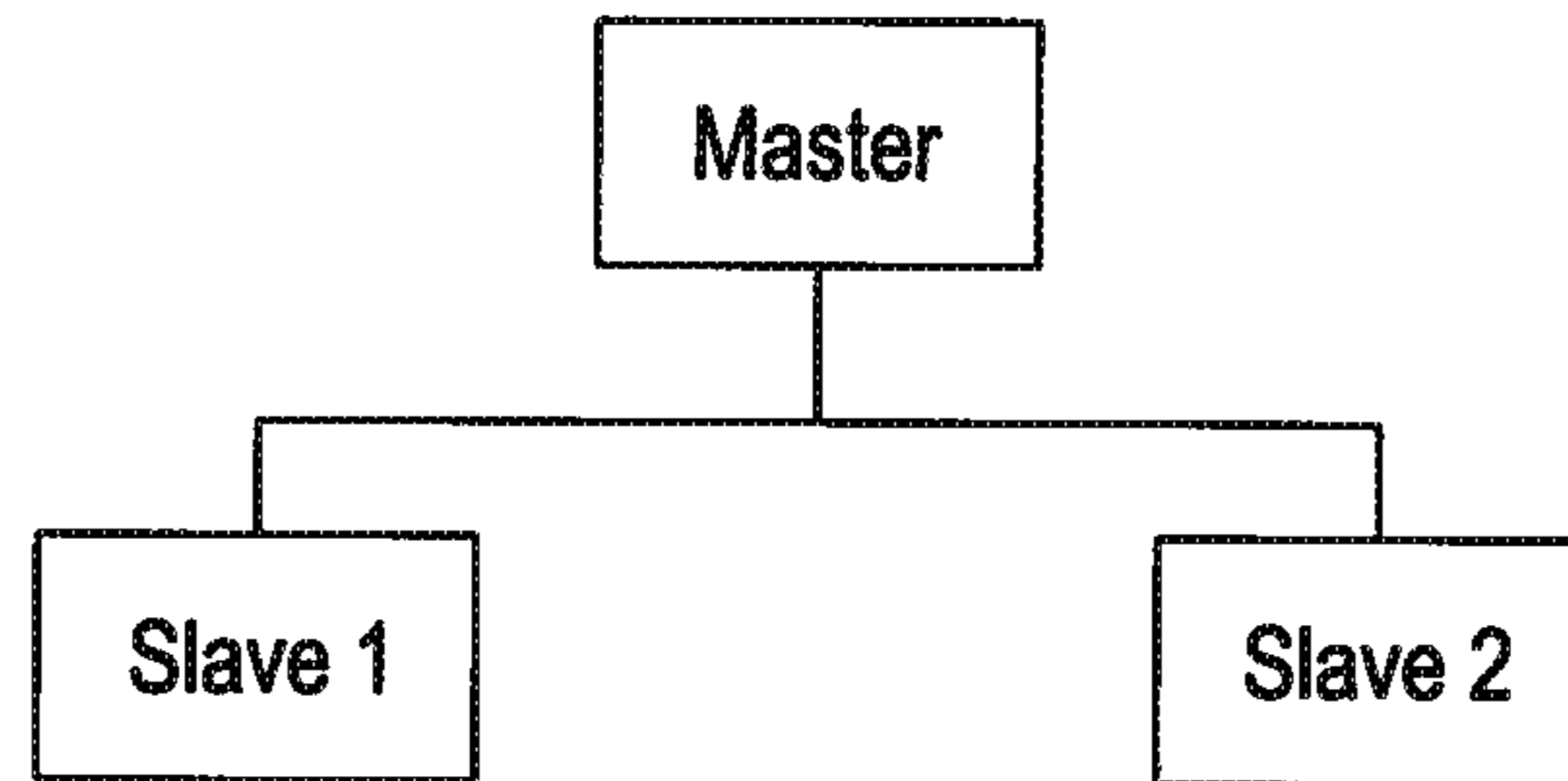
Hierarchical Systems
