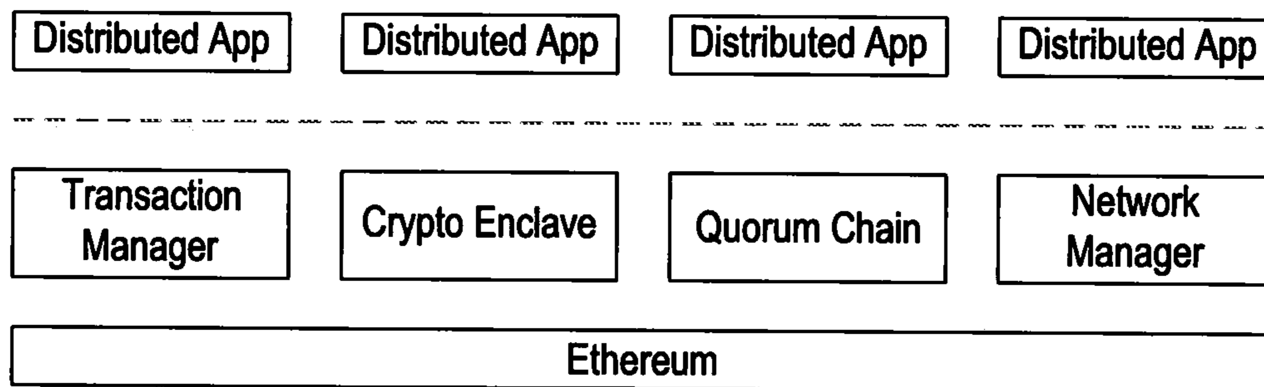
Architecture
