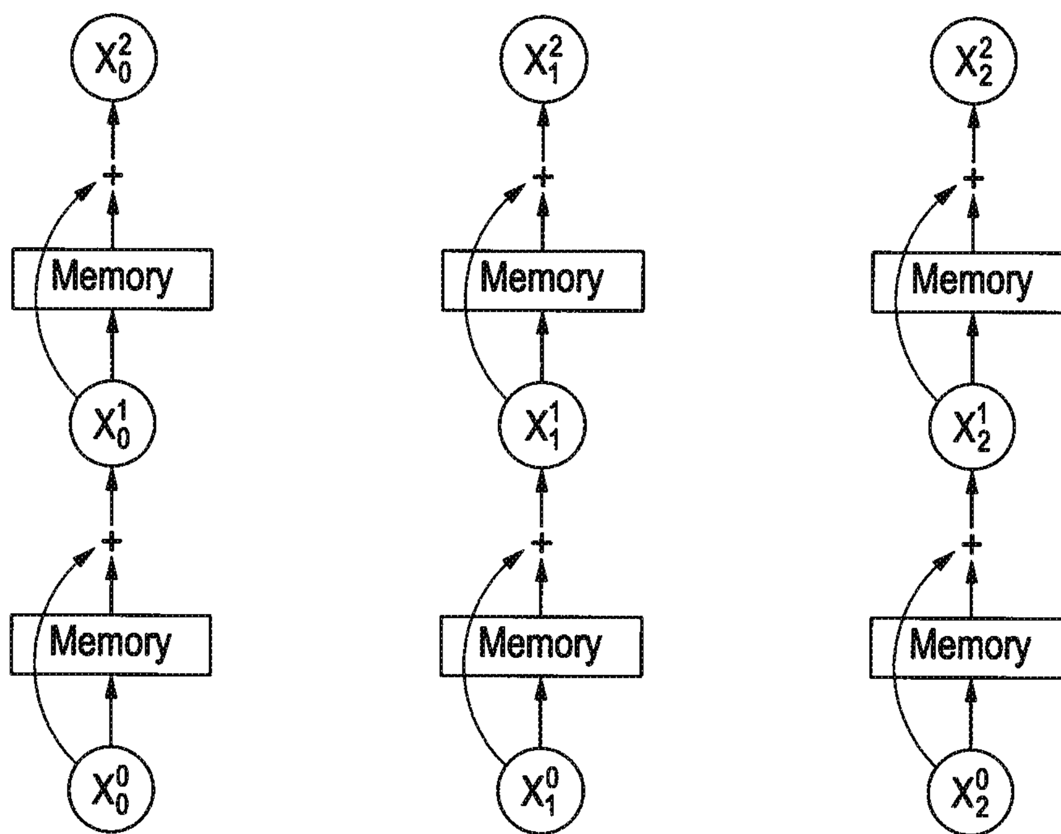
Neural Network
