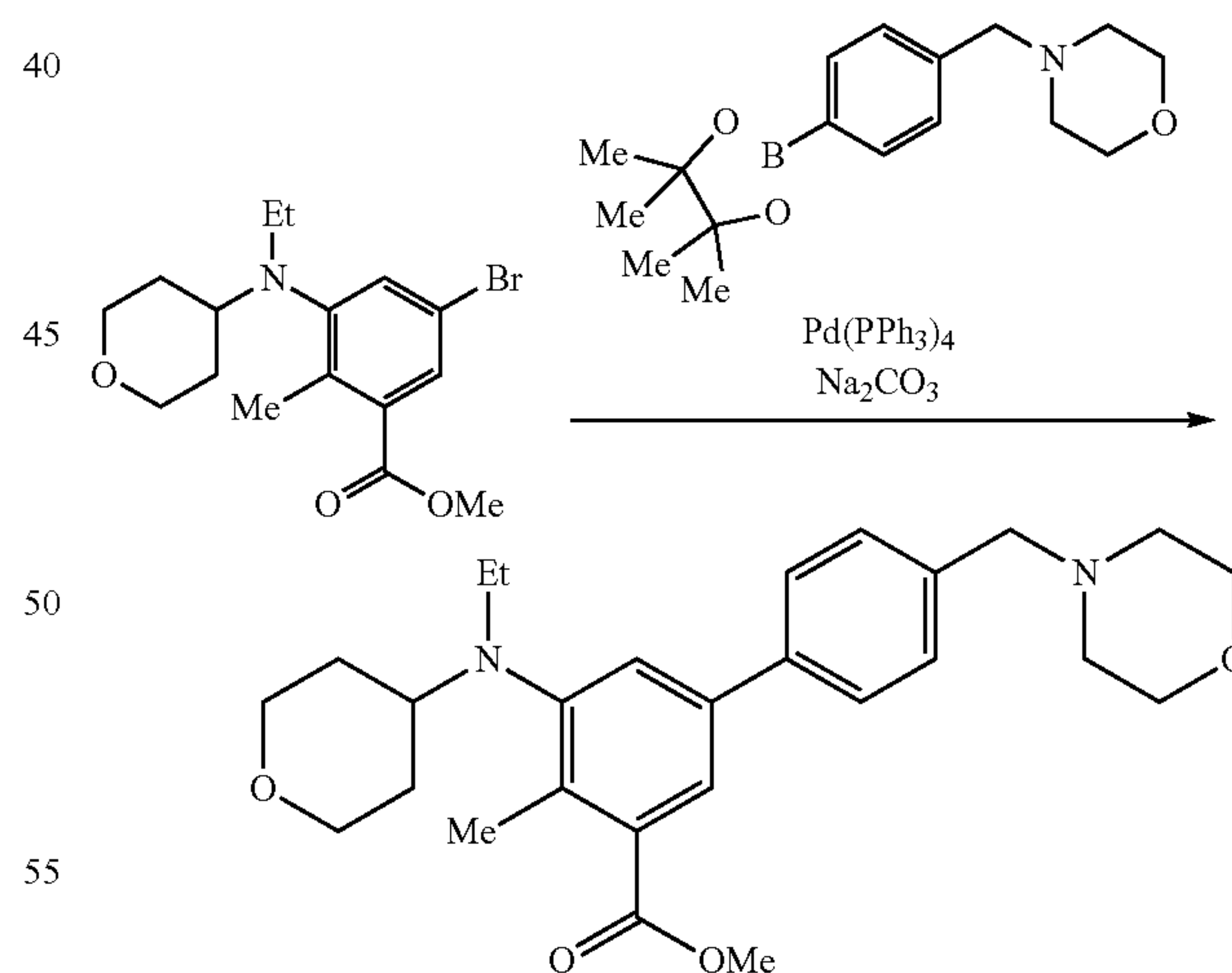
Methyl 5-(ethyl(tetrahydro-2H-pyran-4-yl)amino)-4-methyl-4'-(morpholinomethyl)-[1,1'-biphenyl]-3-carboxylate
