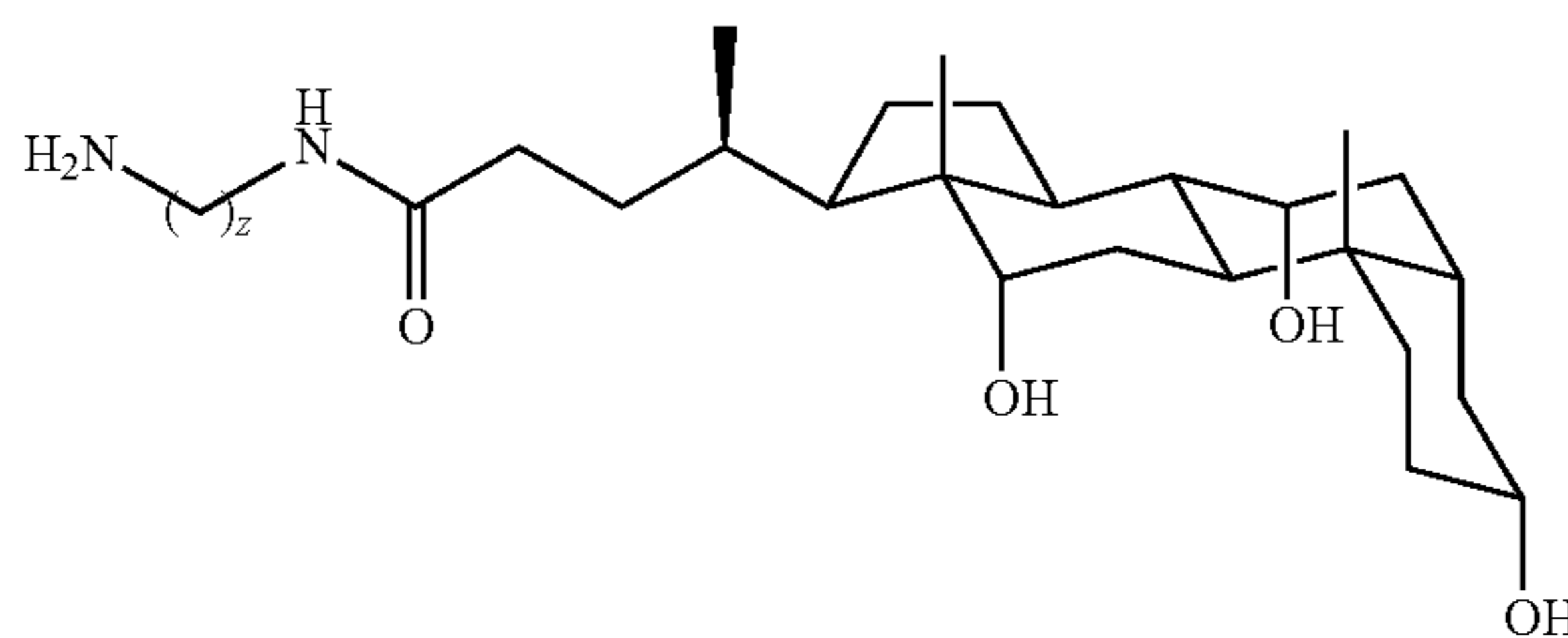
cholic acid derivative
