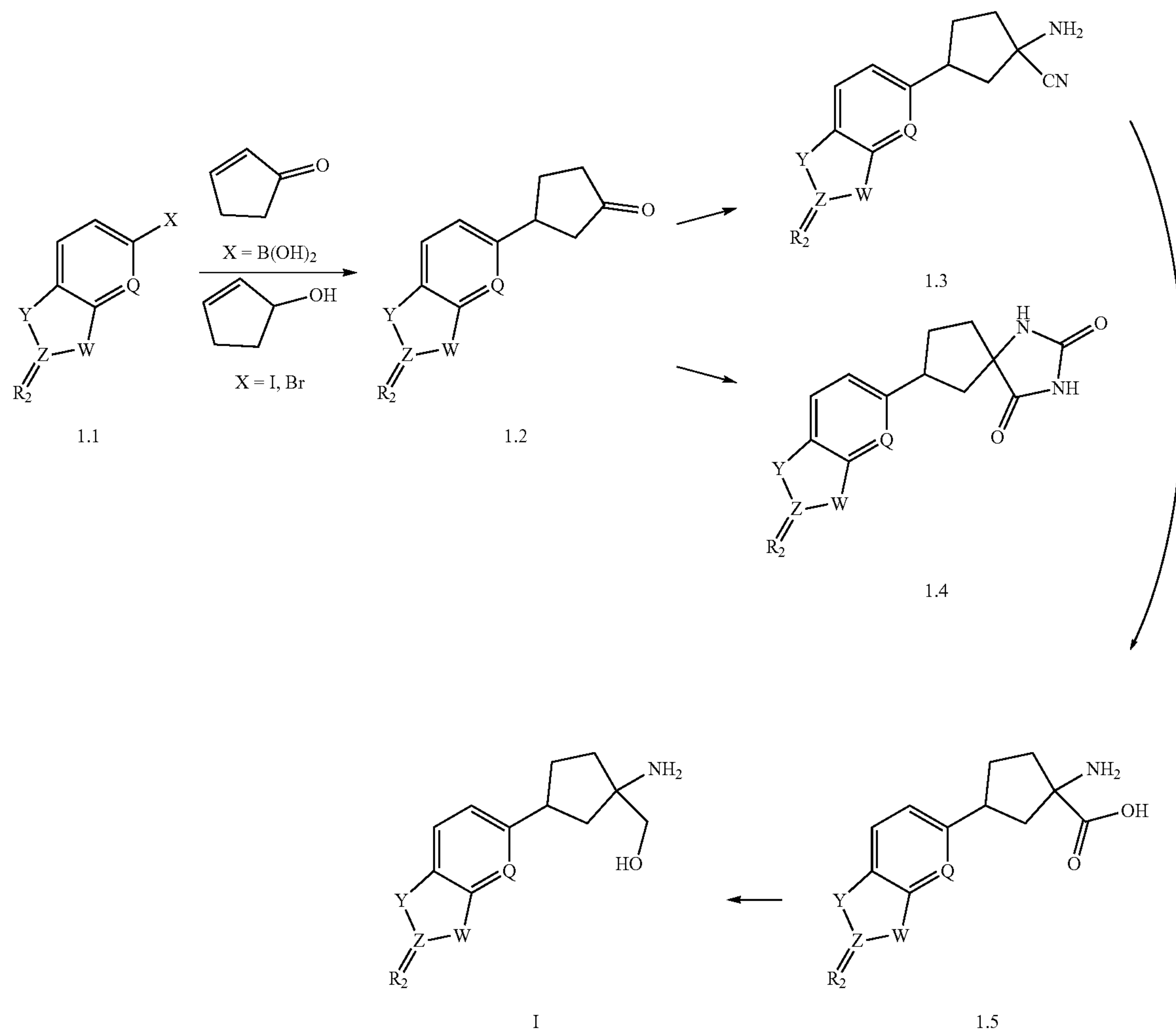
SCHEME 1
