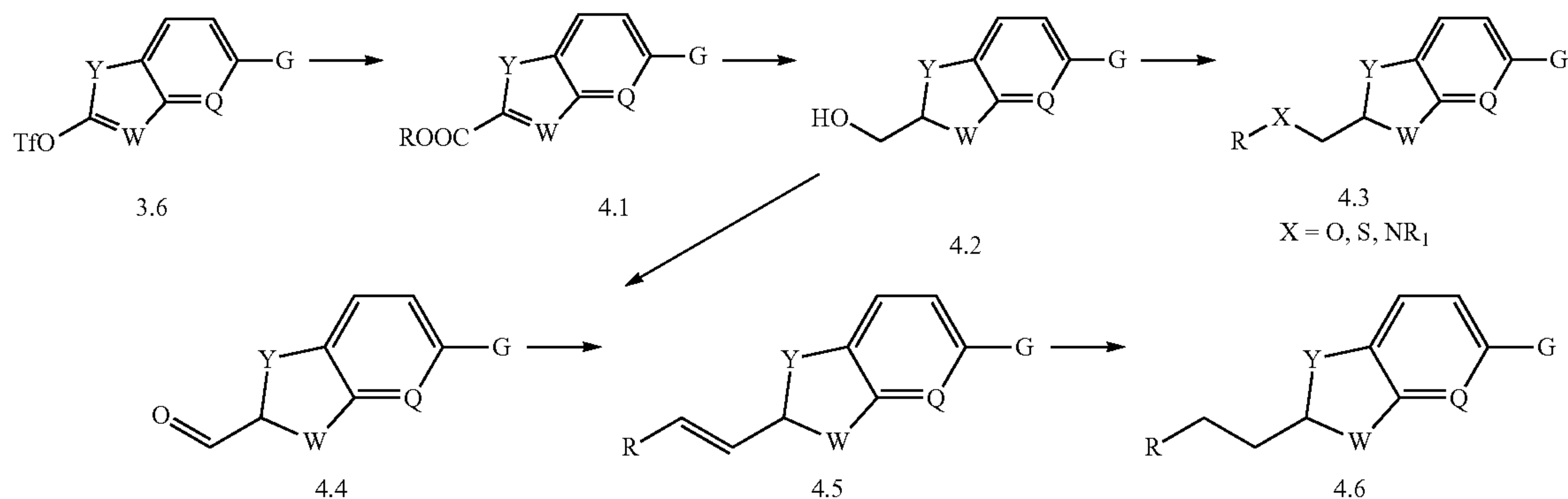
SCHEME 4
