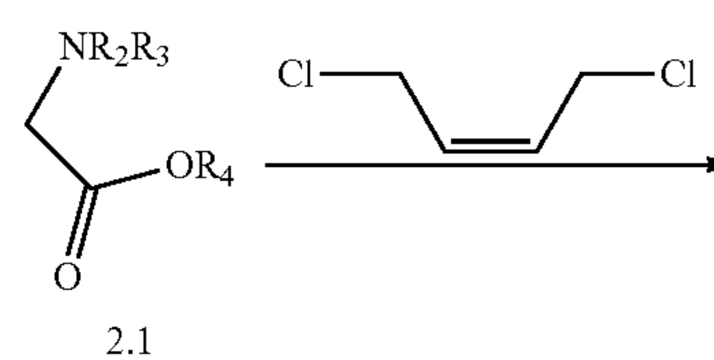
SCHEME 2
