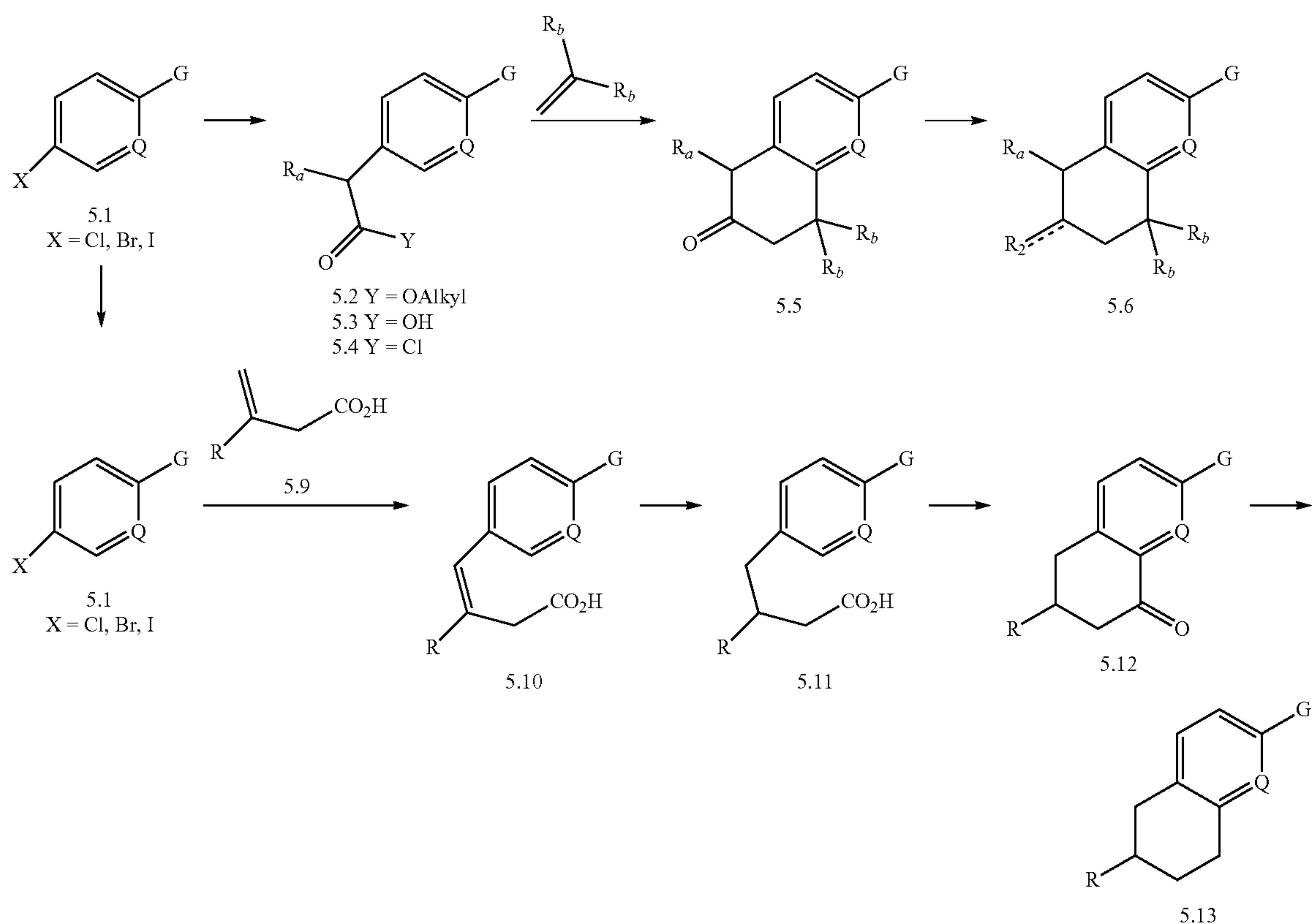
SCHEME 5
