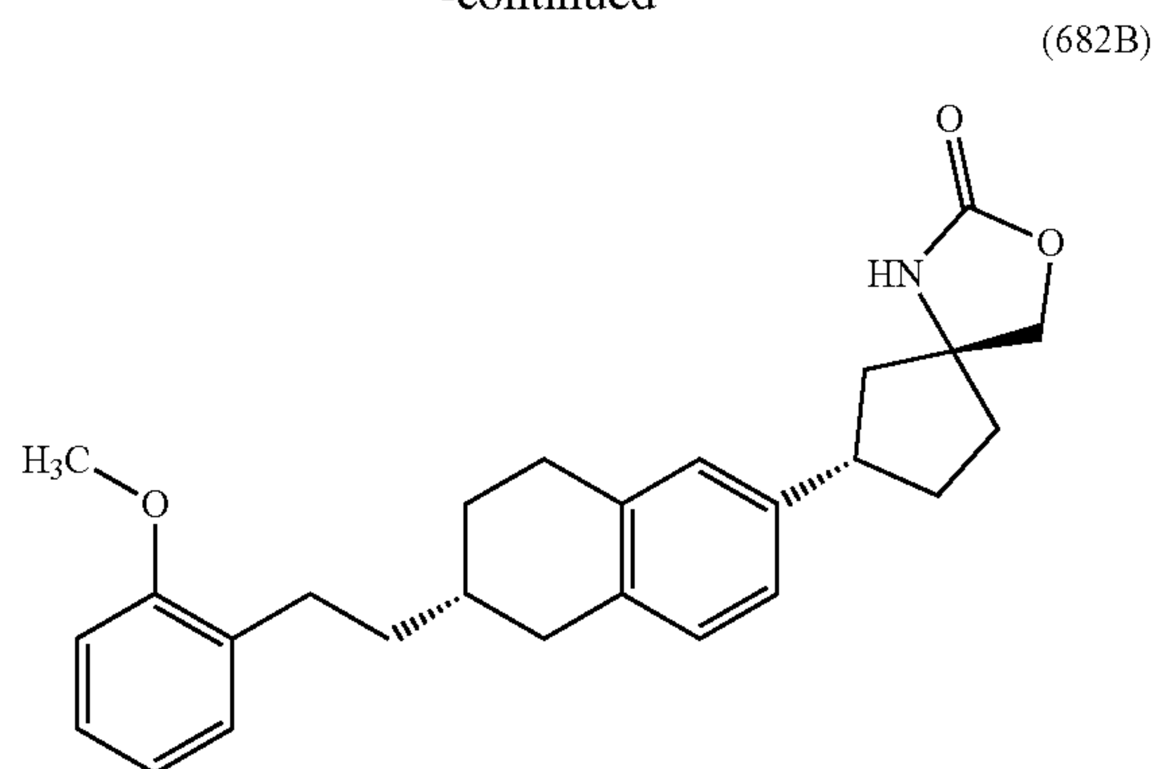
Isomer 2
