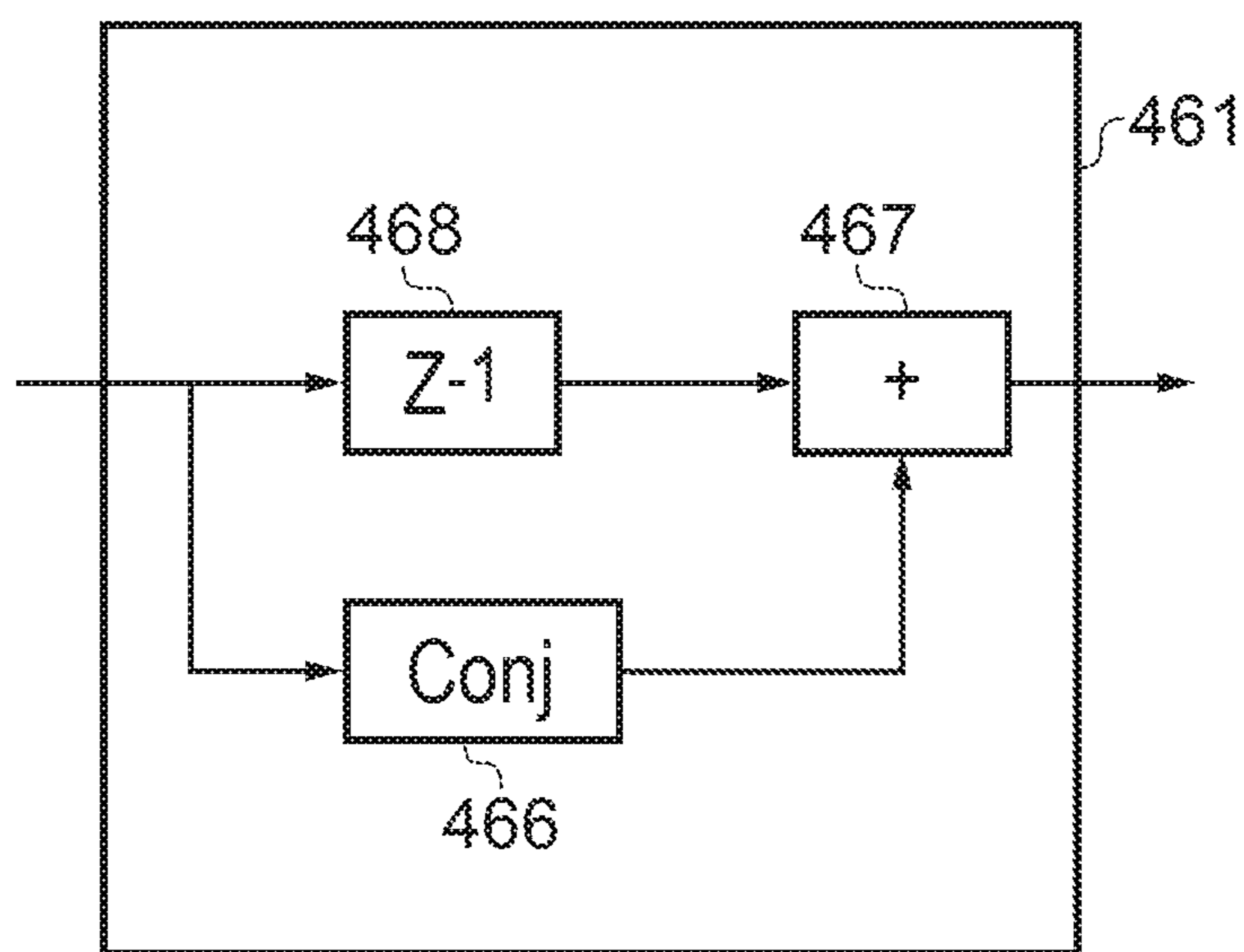
Differential Encoder
