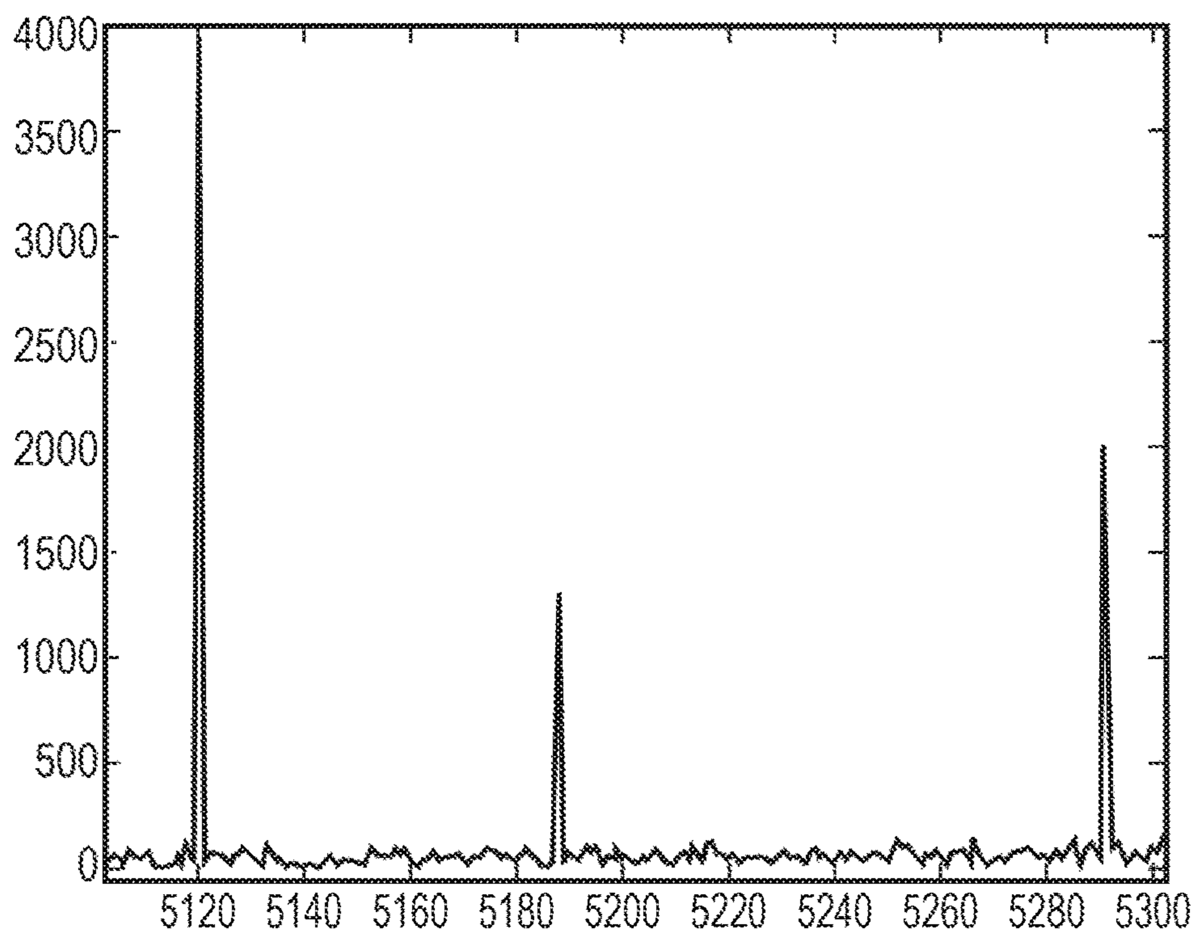
Matched filter output for multipath channel
