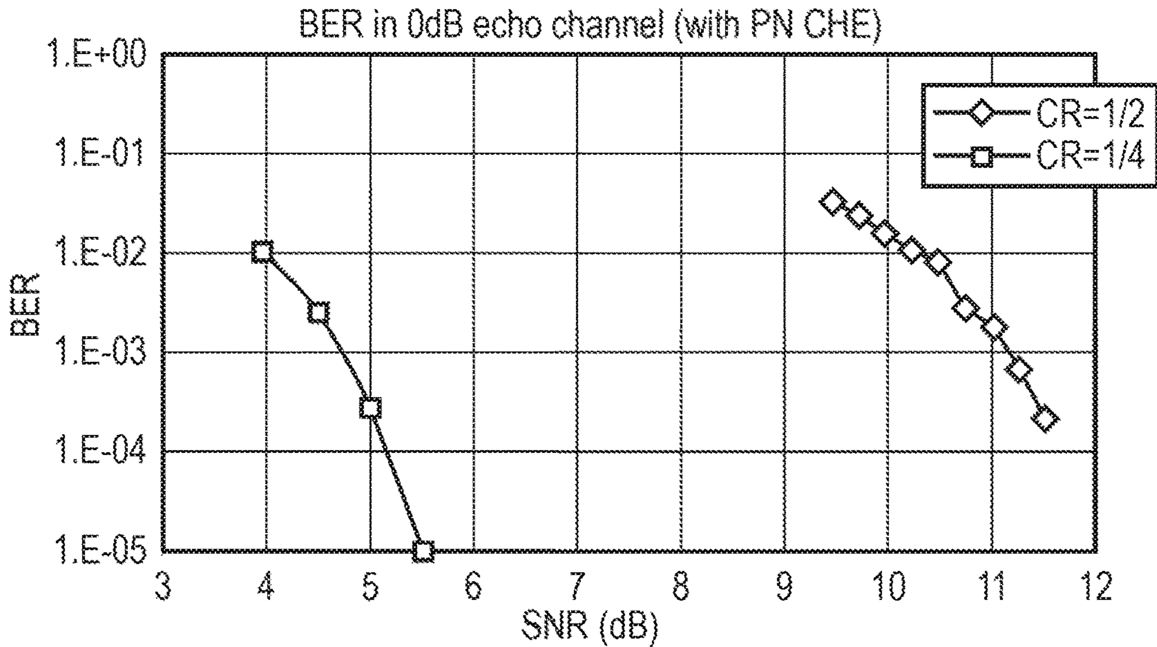
Multipath (2 paths) performance (real channel estimation)
