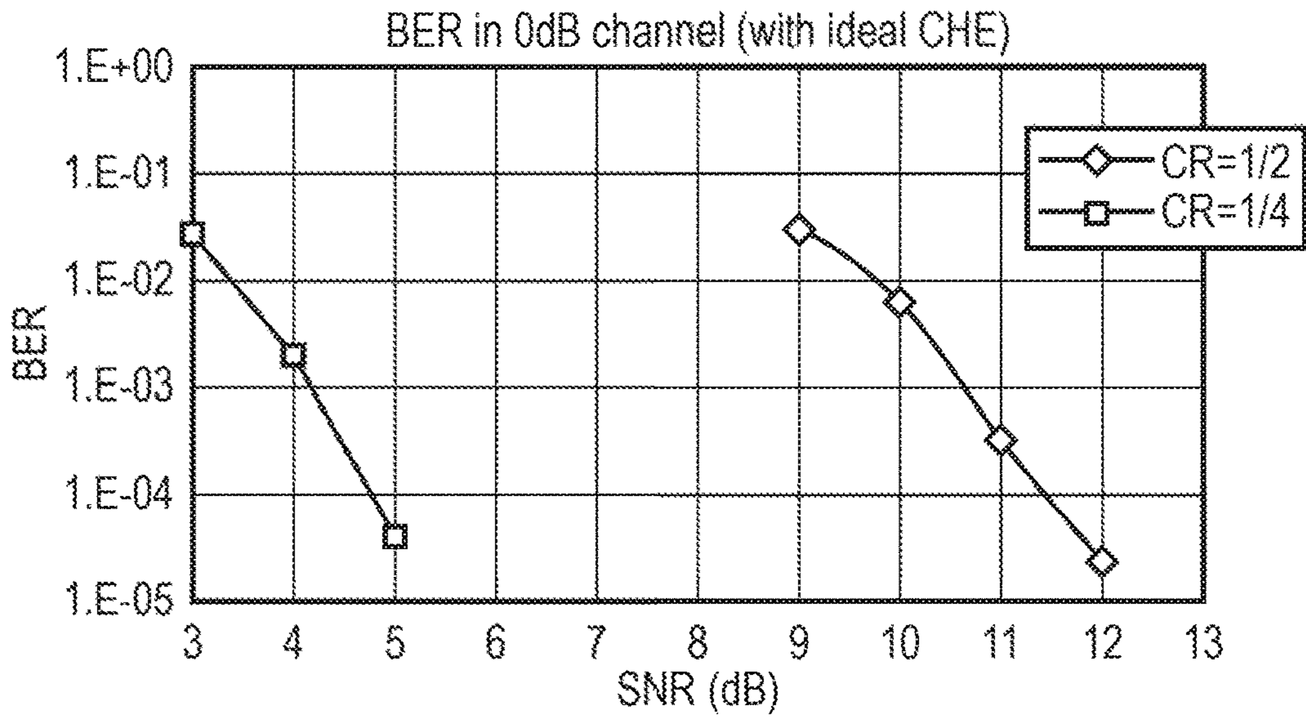
Multipath (2 paths) performance (ideal channel estimation)
