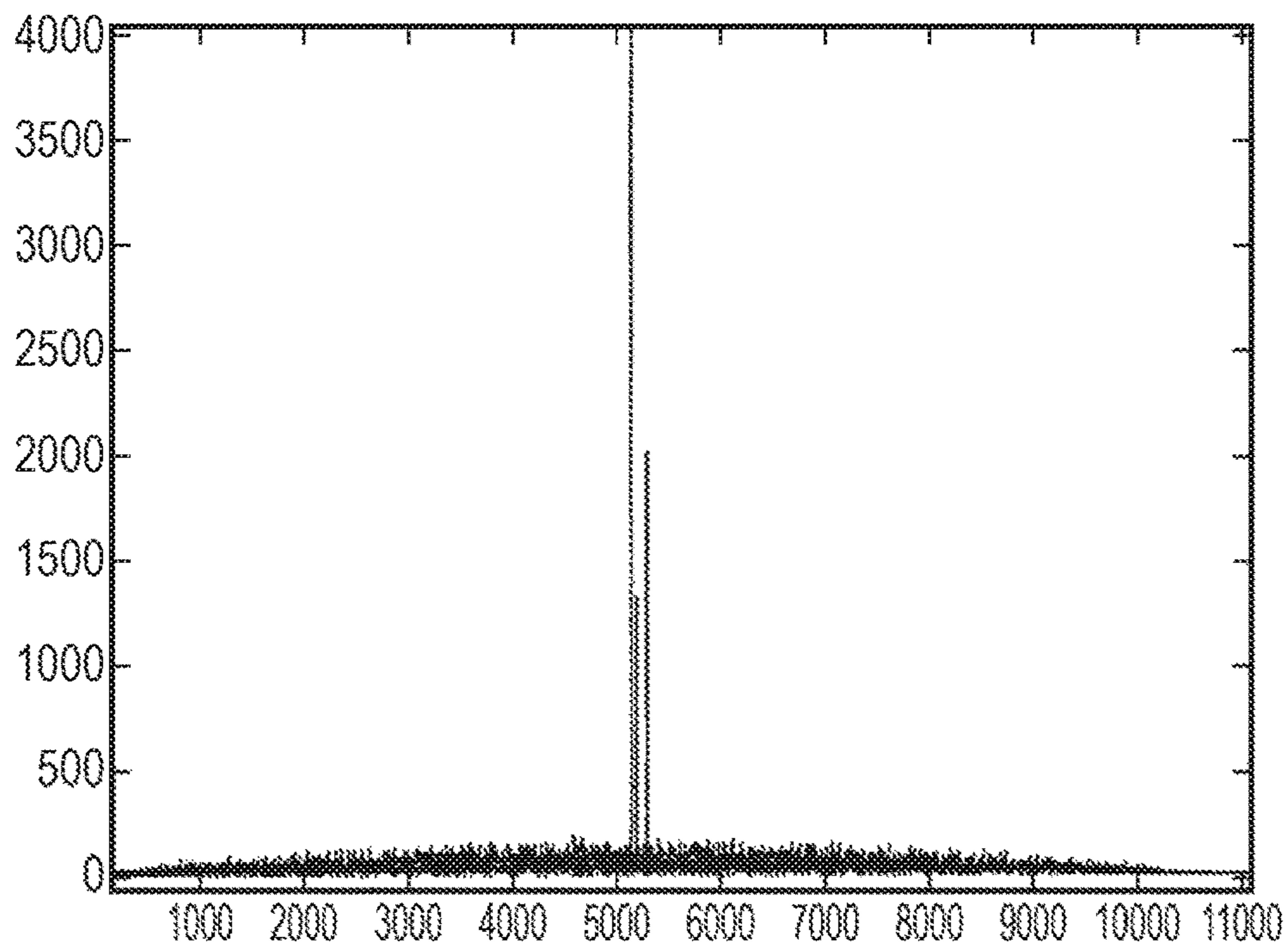
Matched filter output for multipath channel
