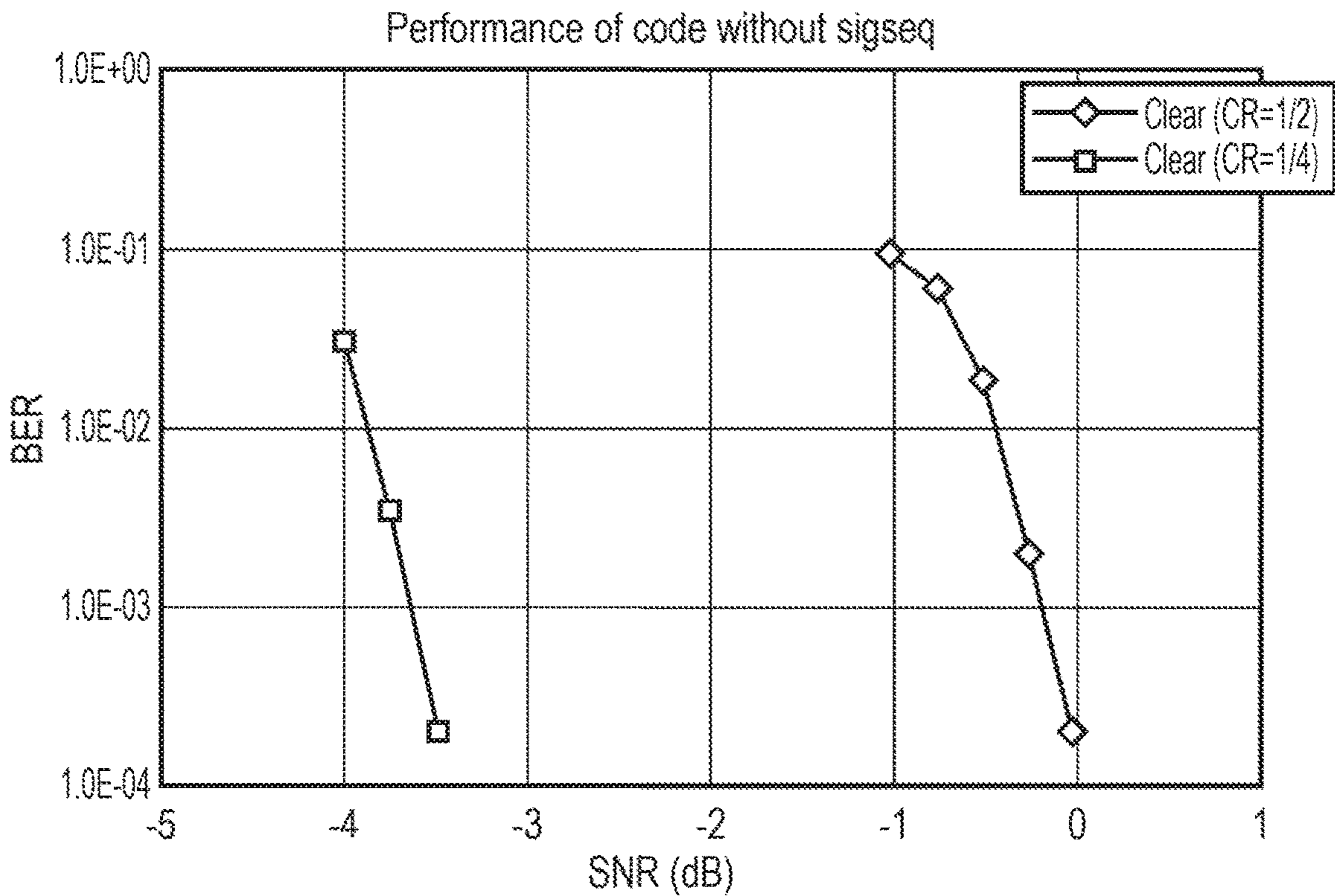
AWGN performance of preamble protection codes
