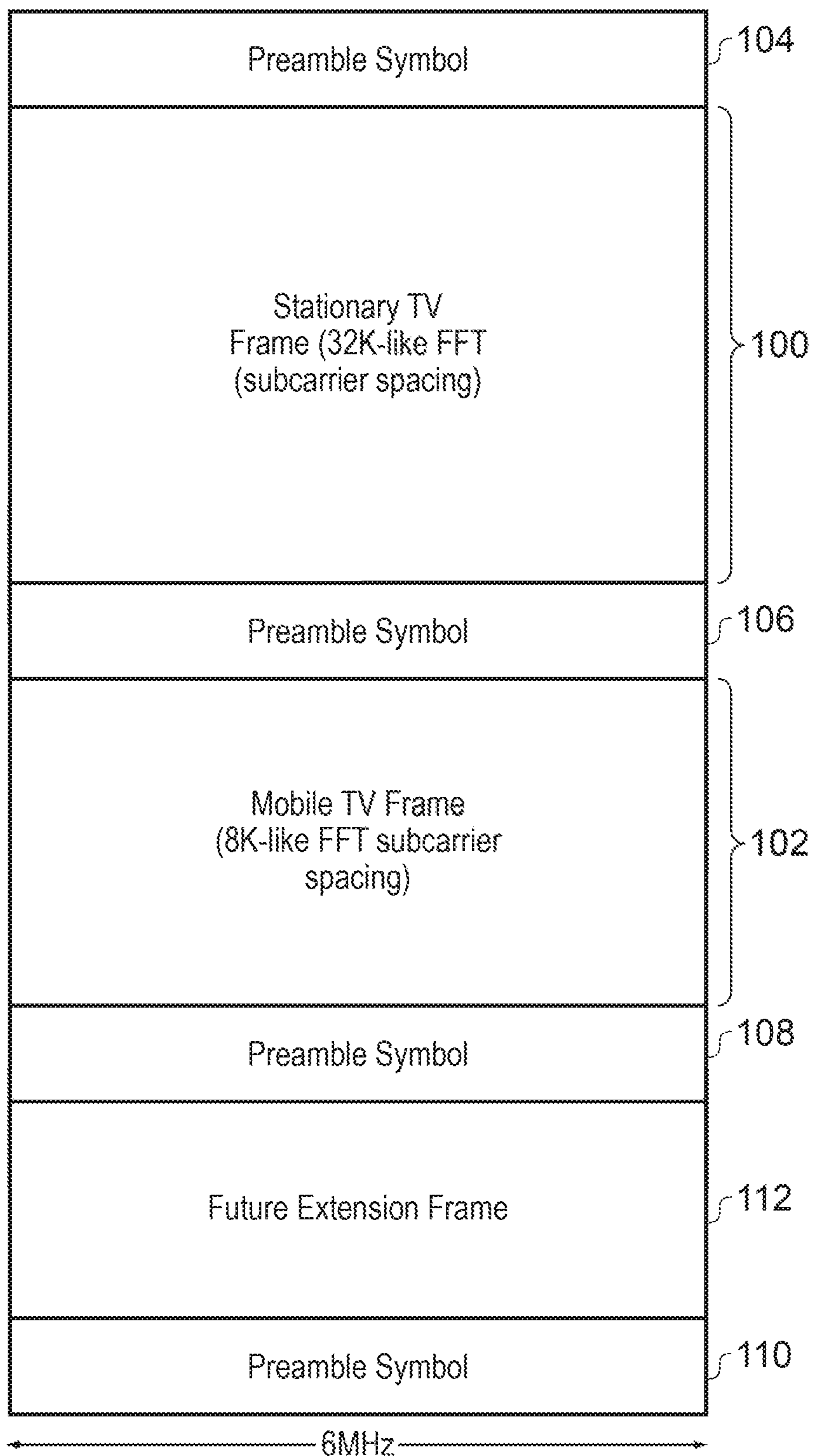
Framing concept for ATSC3-0
