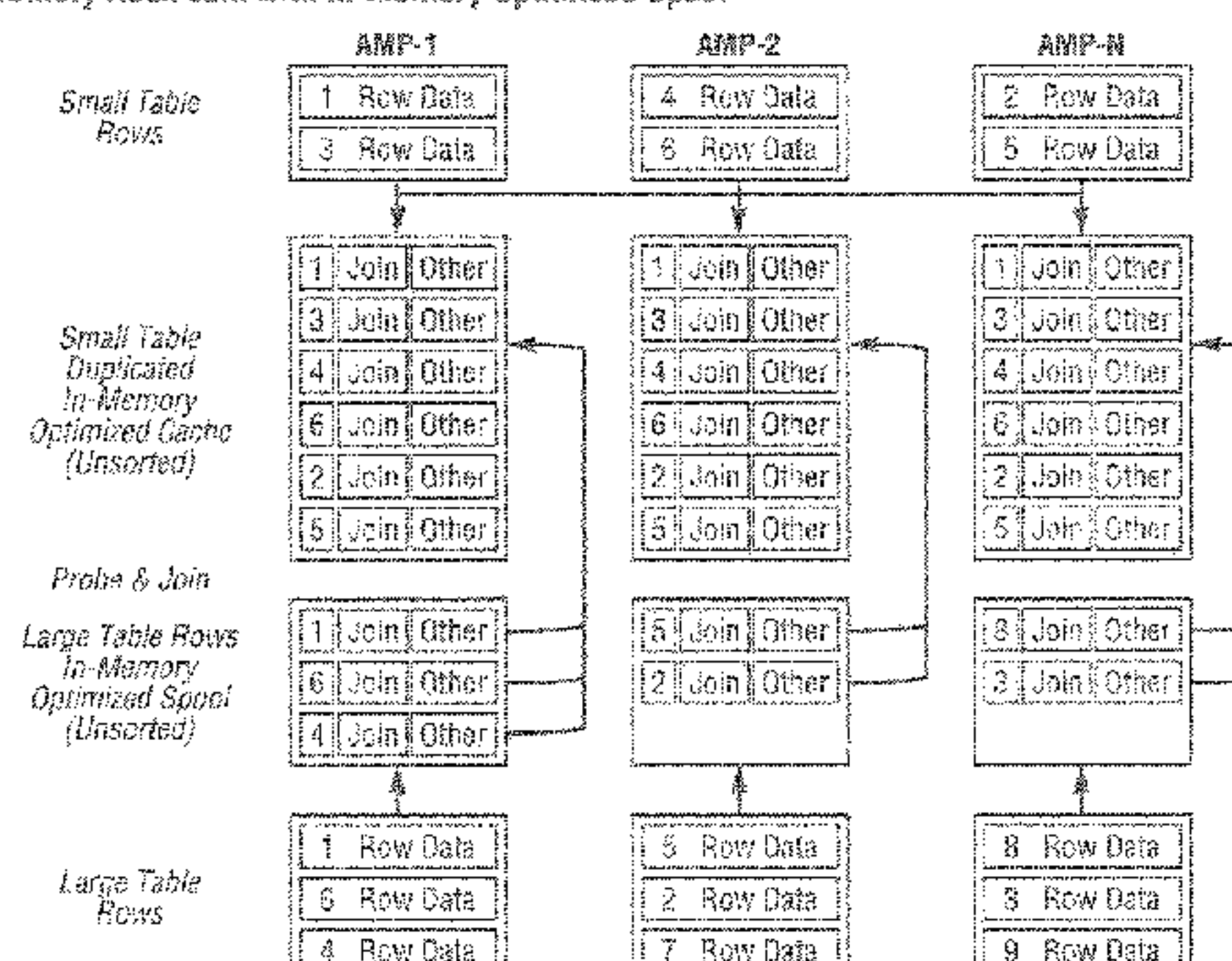
In-Memory Hash Join with In-Memory Optimized Spool
