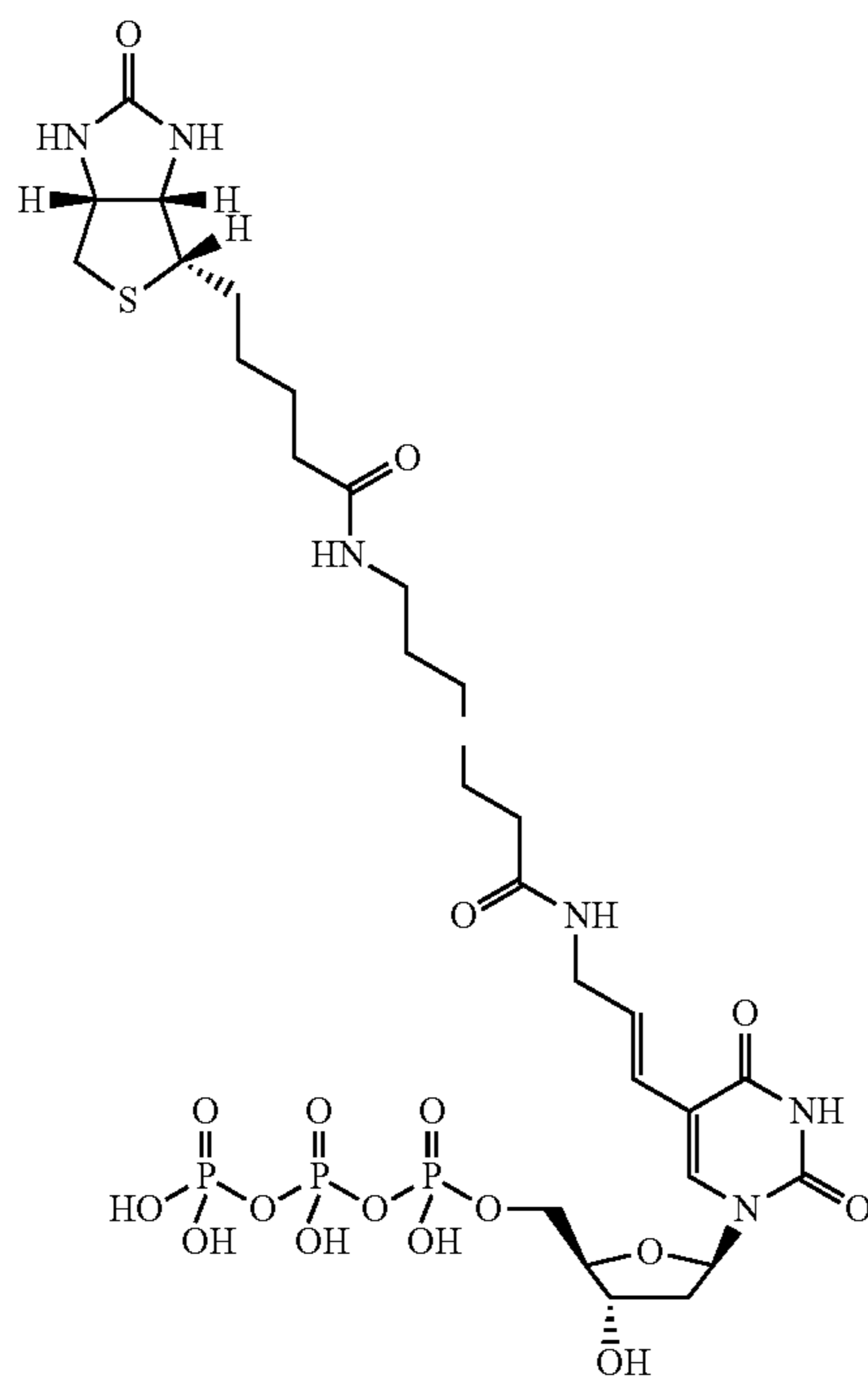
Biotin-11-dUTP
