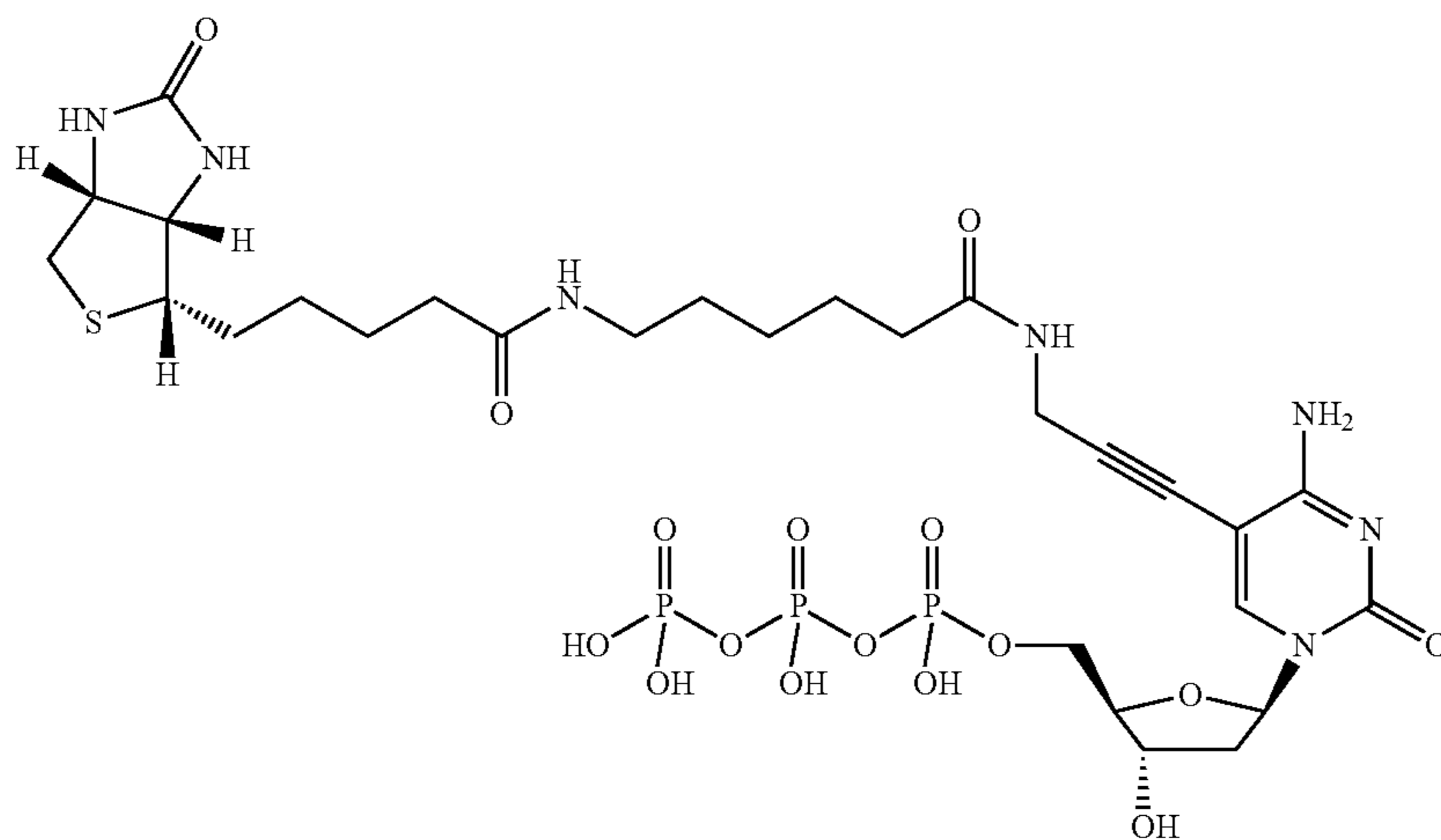
Biotin-11-dCTP
