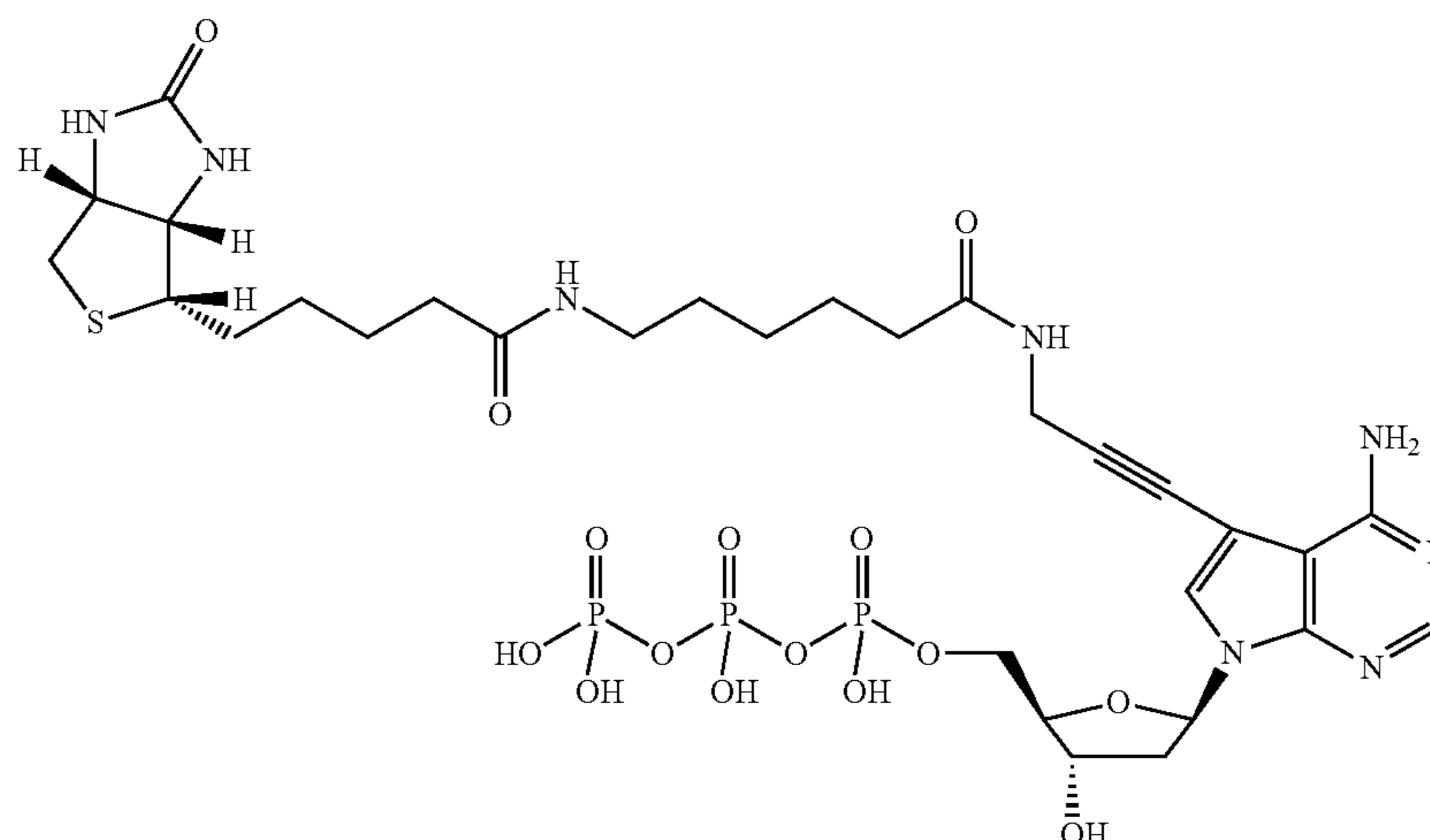
Biotin-11-dATP
