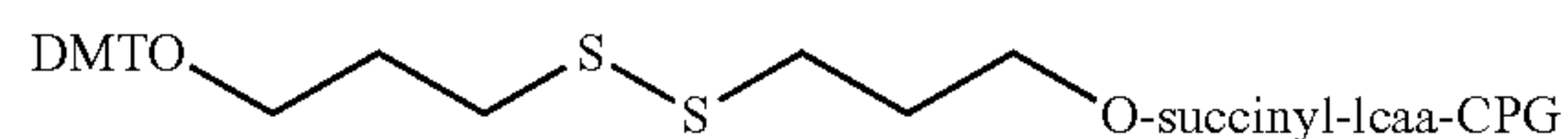
3'-Thiol-Modifier C3 S—S CPG
