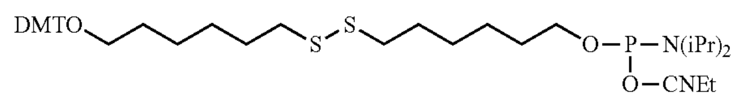
Thiol-Modifier C6 S—S
