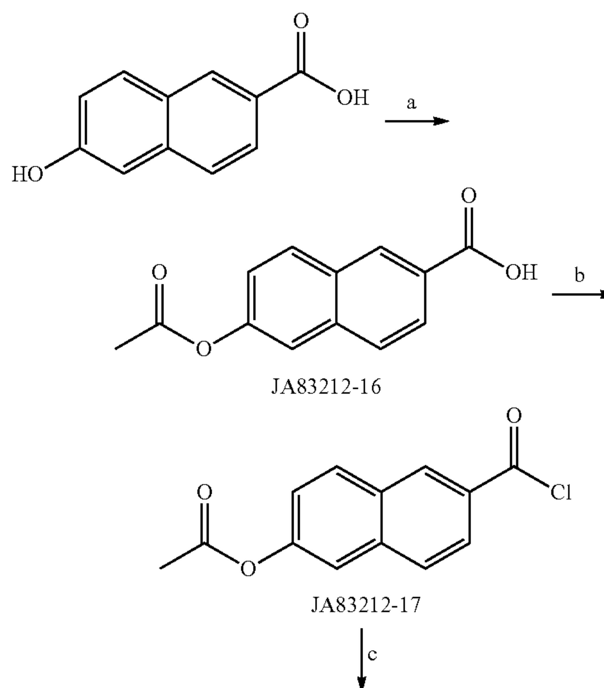
Scheme 5. Synthesis of 6-HNA containing monomer 2.
