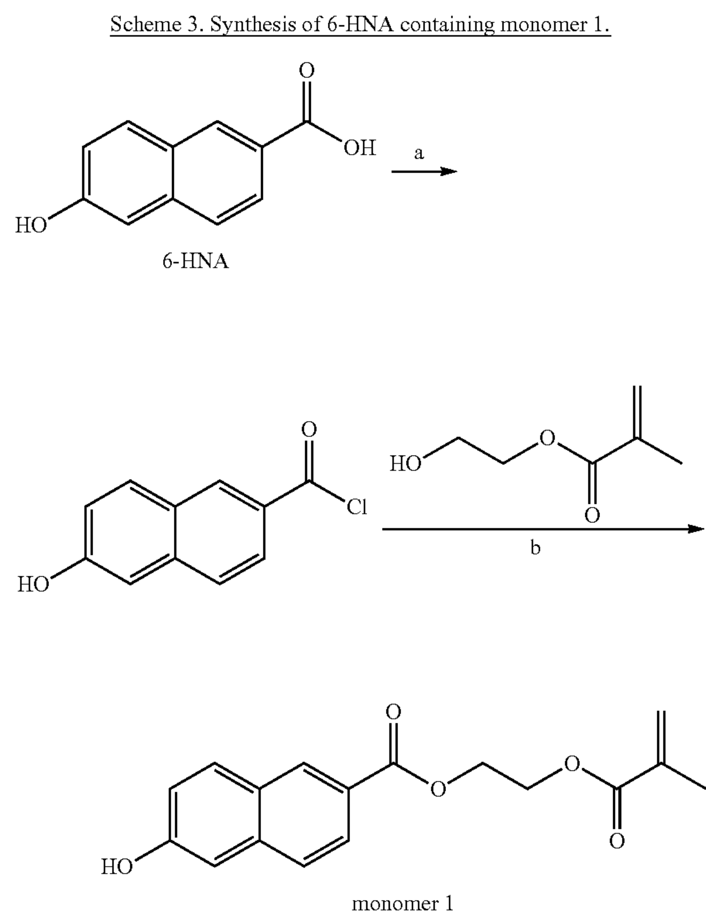
Scheme 3. Synthesis of 6-HNA containing monomer 1. (a) thionyl chloride, THF, RT, 1 hr. (b) 2-hydroxyethylmethacrylate, triethylamine, THF, 0° C. to RT, 18 hrs.
