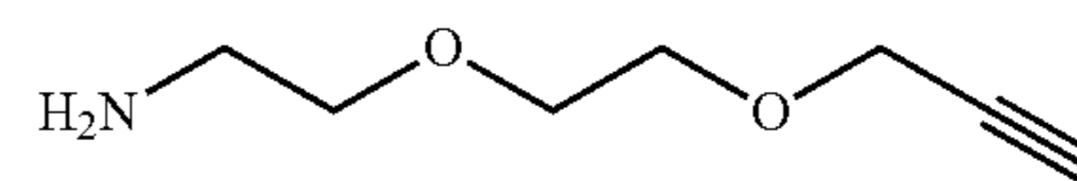
2-(2-(prop-2-ynoxy)ethoxy)ethanamine (s-5)
