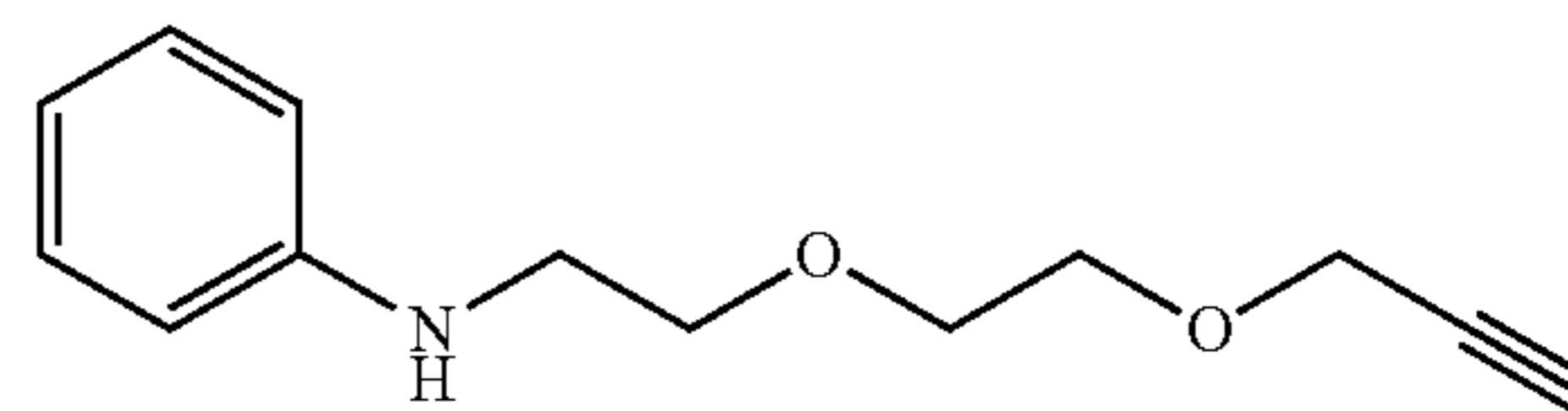
N-(2-(2-(prop-2-ynyloxy)ethoxy)ethyl)aniline (s-9)
