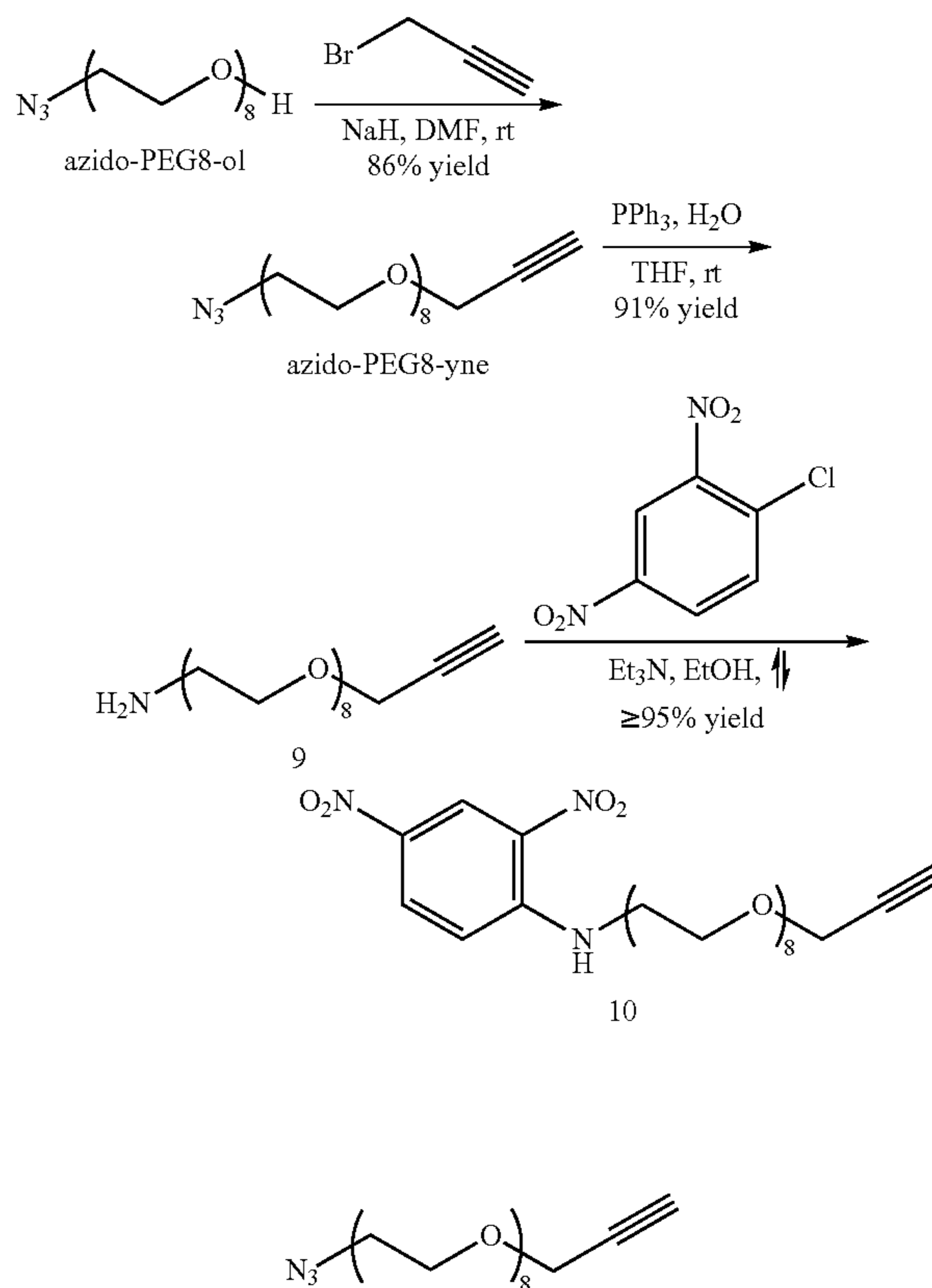
1-azido-3,6,9,12,15,18,21,24-octaoxaheptacos-26-yne (azido-PEG8-yne)
