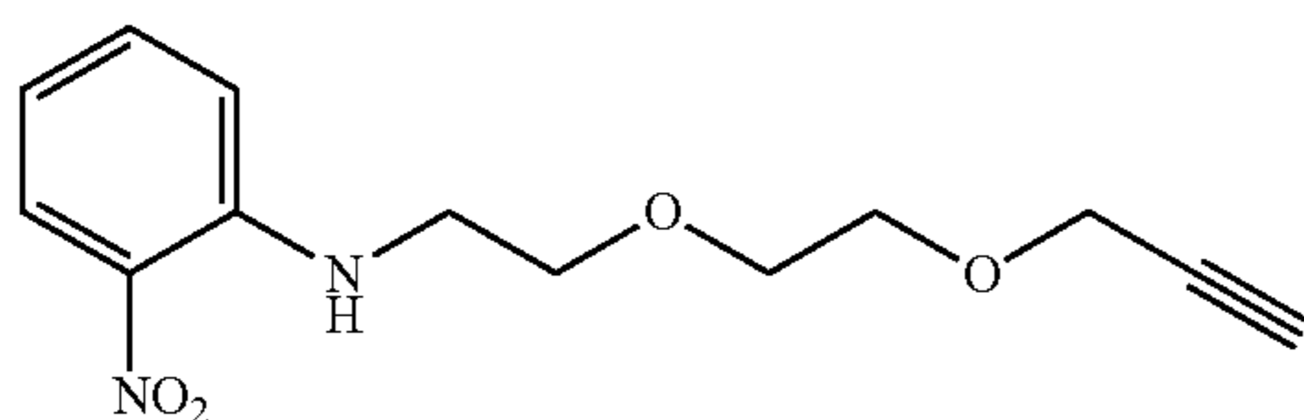
2-nitro-N-(2-(2-(prop-2-ynyloxy)ethoxy)ethyl)aniline (s-6)
