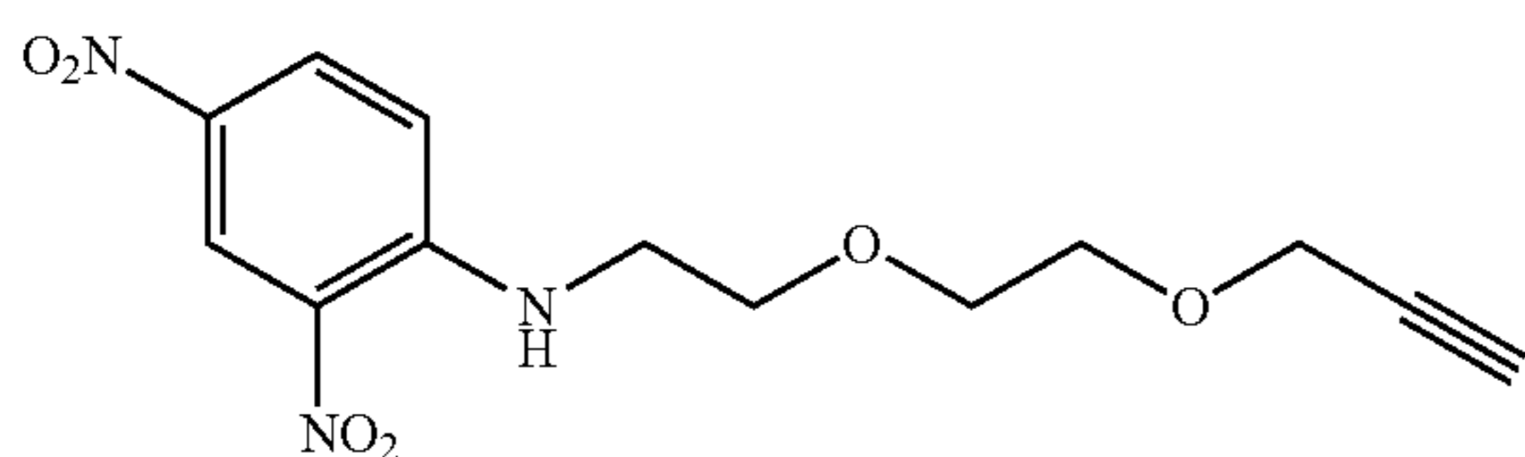
2,4-dinitro-N-(2-(2-(prop-2-ynoxy)ethoxy)ethyl)aniline (s-2b)
