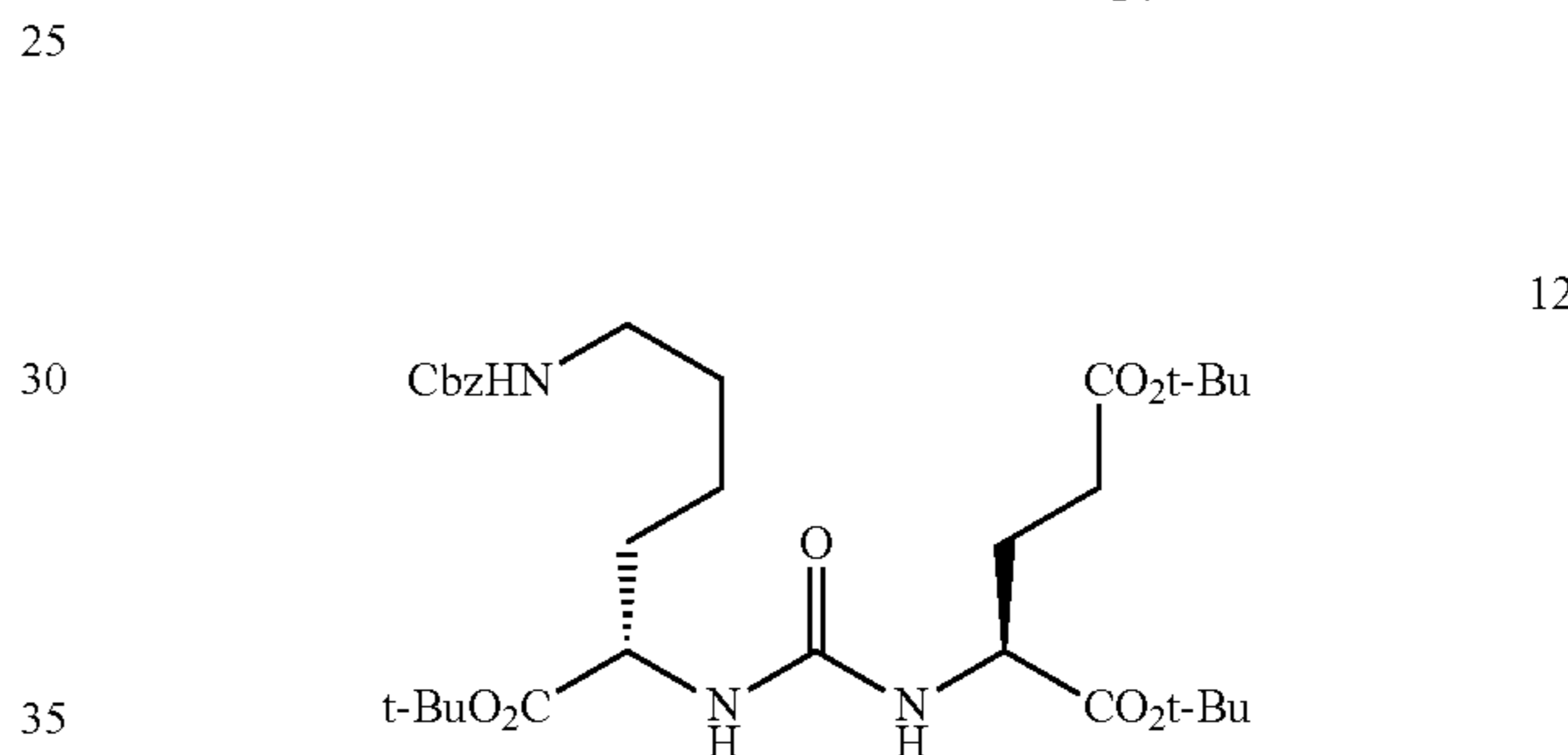
(9S,13S)-tri-tert-butyl 3,11-dioxo-1-phenyl-2-oxa-4,10,12-triazapentadecane-9,13,15-tricarboxylate (12)
