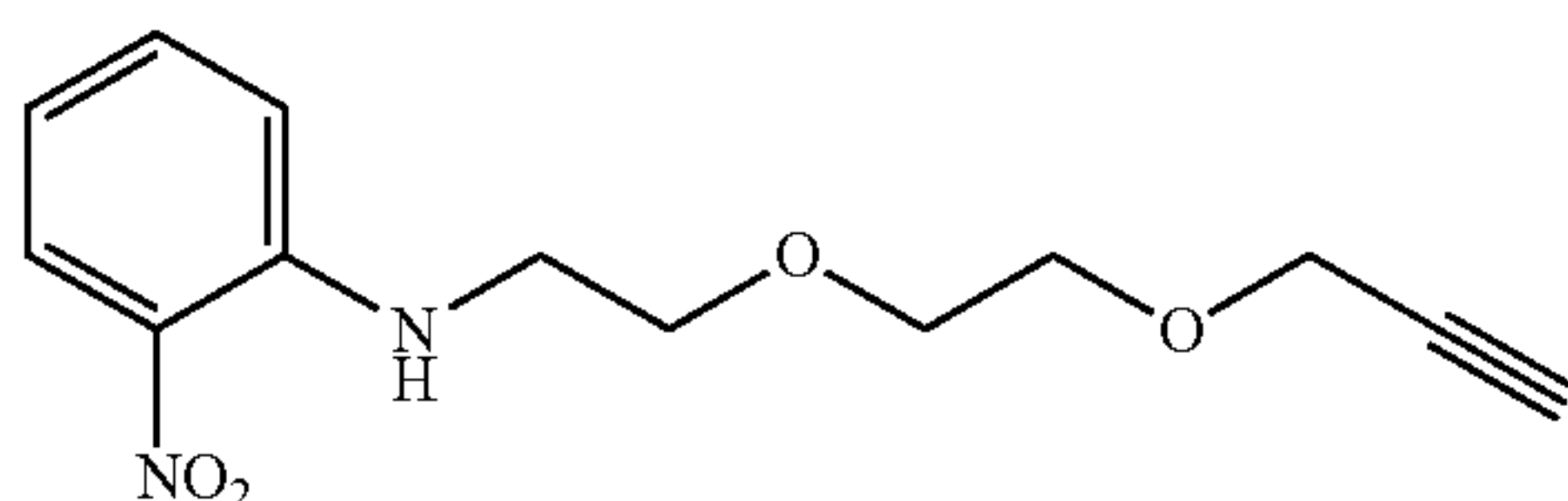
2-nitro-N-(2-(2-(prop-2-ynyloxy)ethoxy)ethyl)aniline (s-6)
