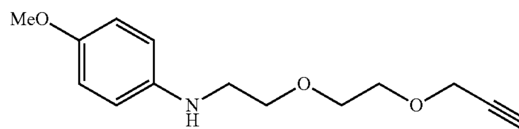
4-methoxy-N-(2-(2-(prop-2-ynyloxy)ethoxy)ethyl)aniline (s-10)
