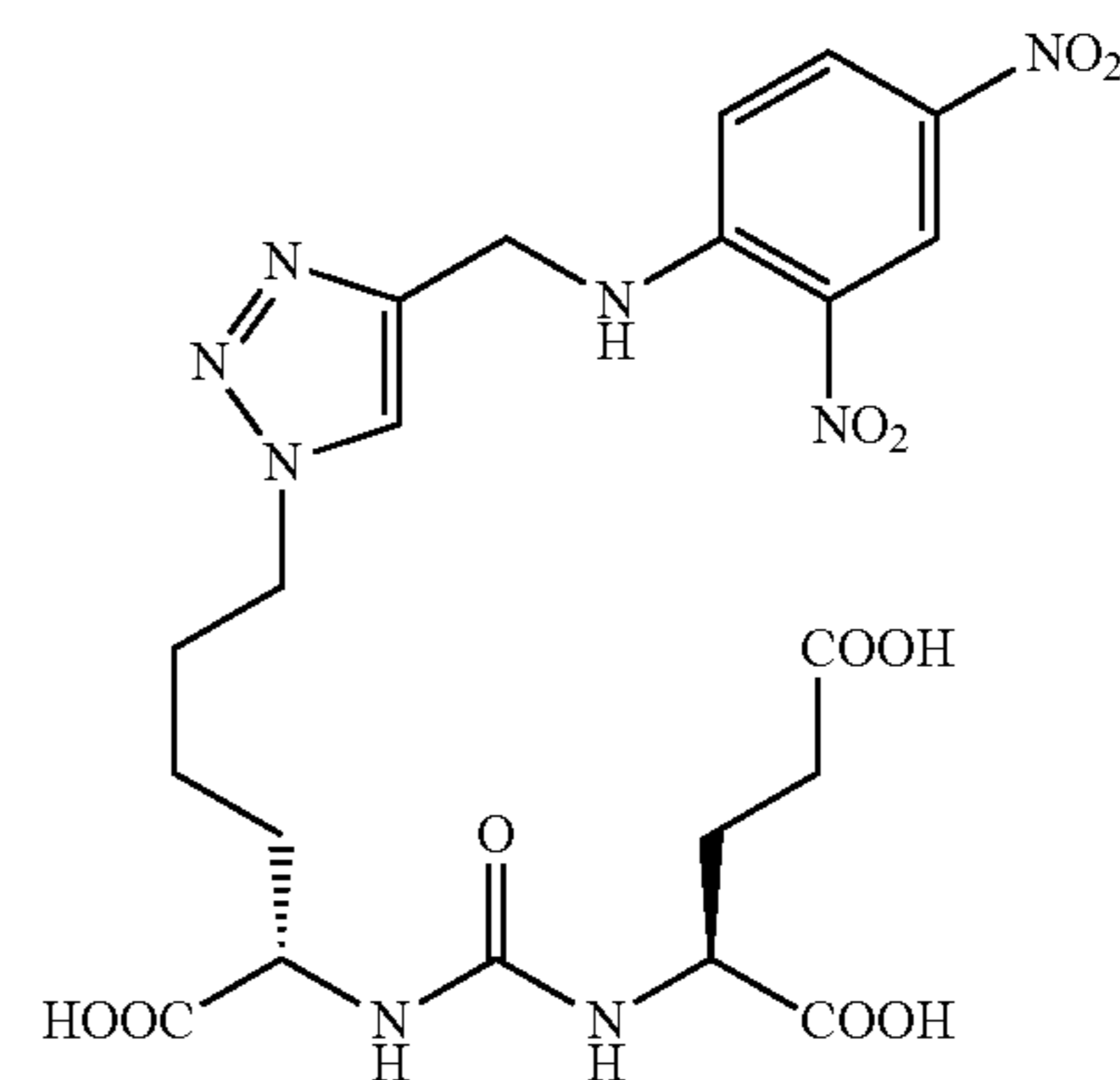
(S)-2-(3-((S)-1-carboxy-5-(4-((2,4-dinitrophenylamino)methyl)-1H-1,2,3-triazol-1-yl)pentyl)ureido)pentanedioic acid (1)
