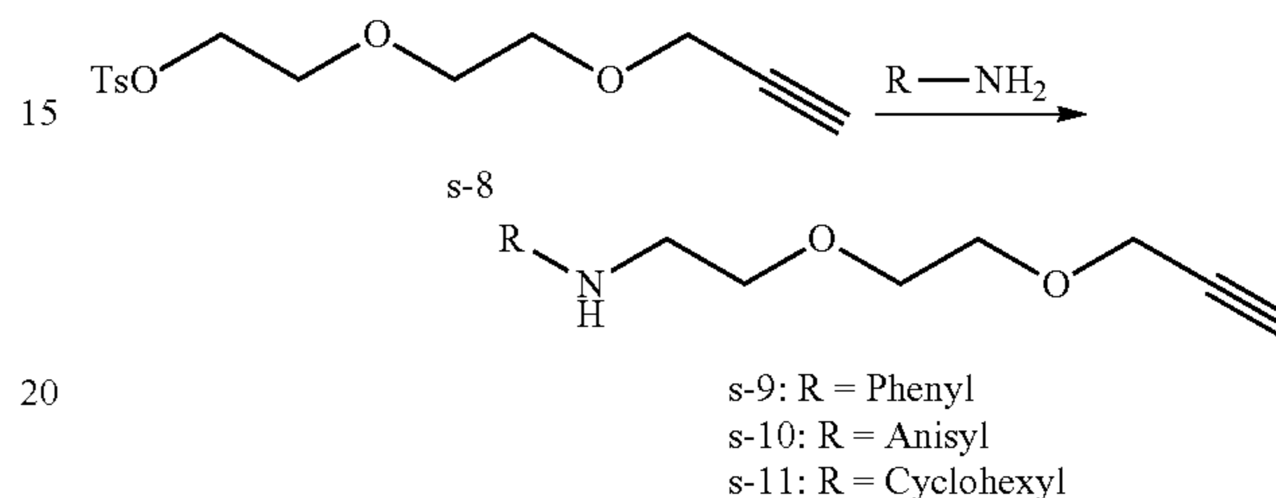
Scheme S-3: General synthesis of (PEG) 2 -alkynes.
