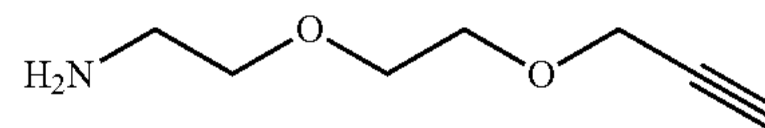
2-(2-(prop-2-ynyloxy)ethoxy)ethanamine (s-5)
