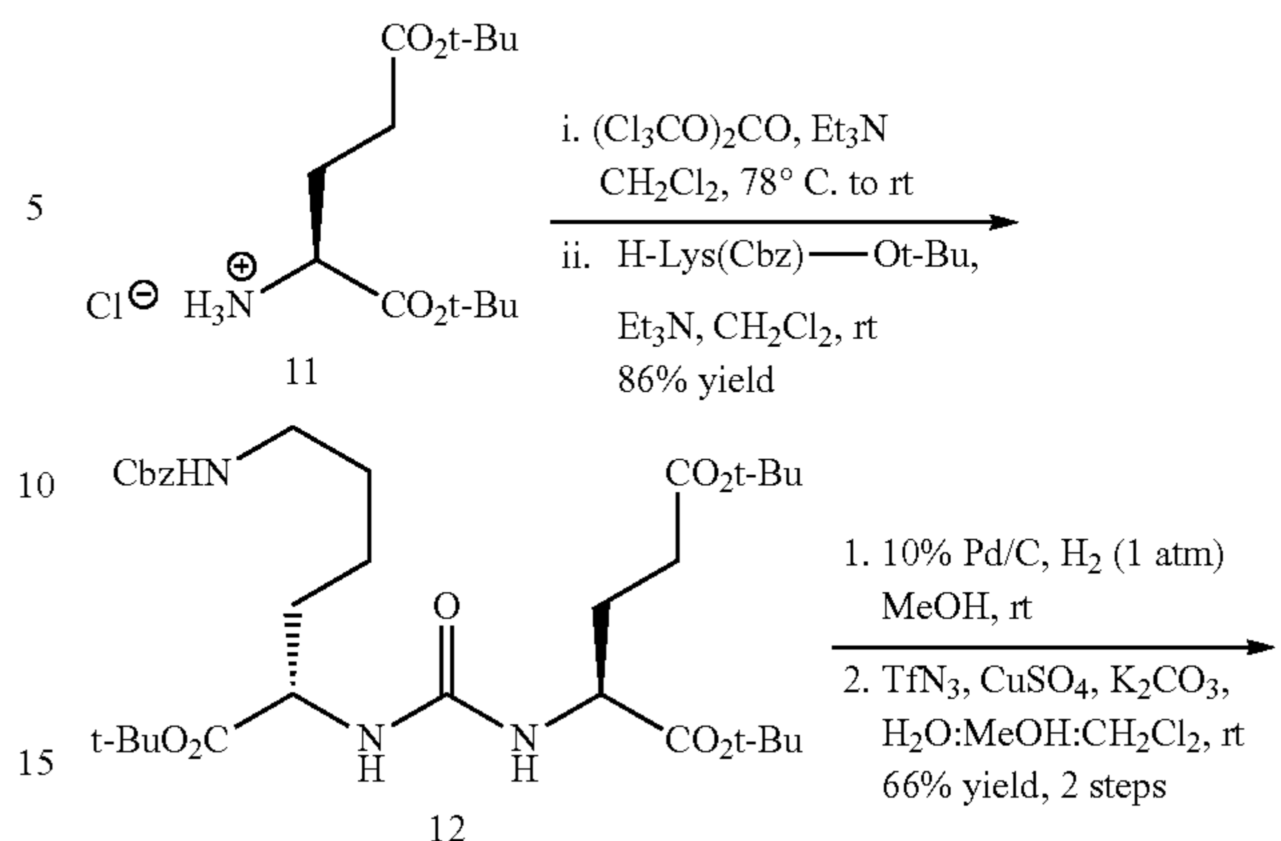
3,6,9,12,15,18,21,24-octaoxaheptacos-26-yn-1-amine (9)
