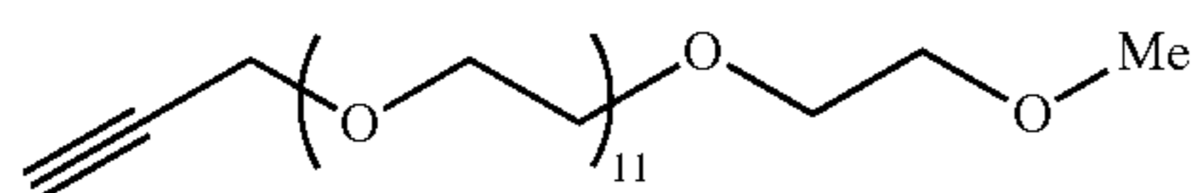
2,5,8,11,14,17,20,23,26,29,32,35,38-tridecaoxahentetracont-40-yne (s-13e)
