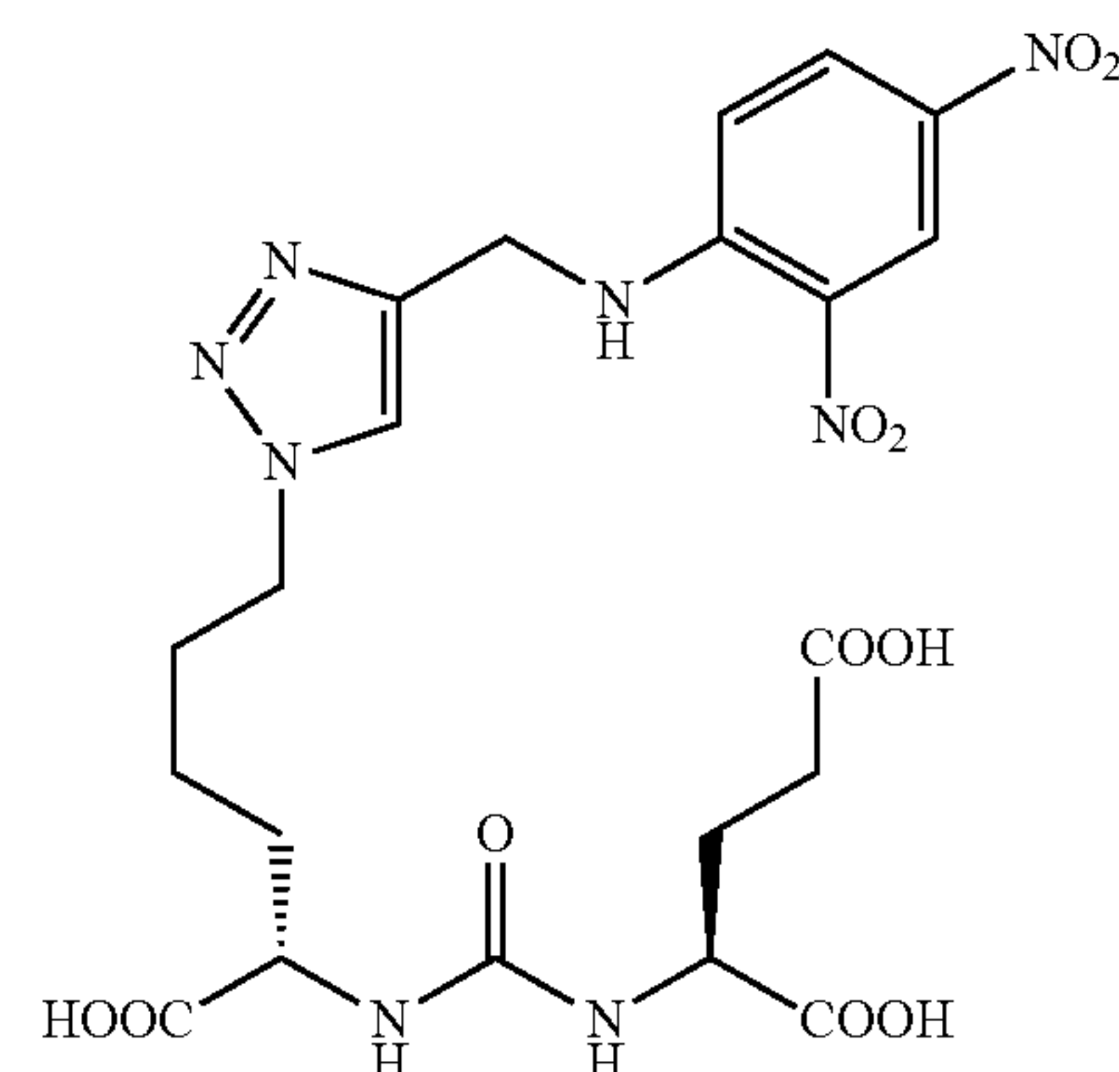
(S)-2-(3-((S)-1-carboxy-5-(4-((2,4-dinitrophenylamino)methyl)-1H-1,2,3-triazol-1-yl)pentyl)ureido)pentanedioic acid (1)
