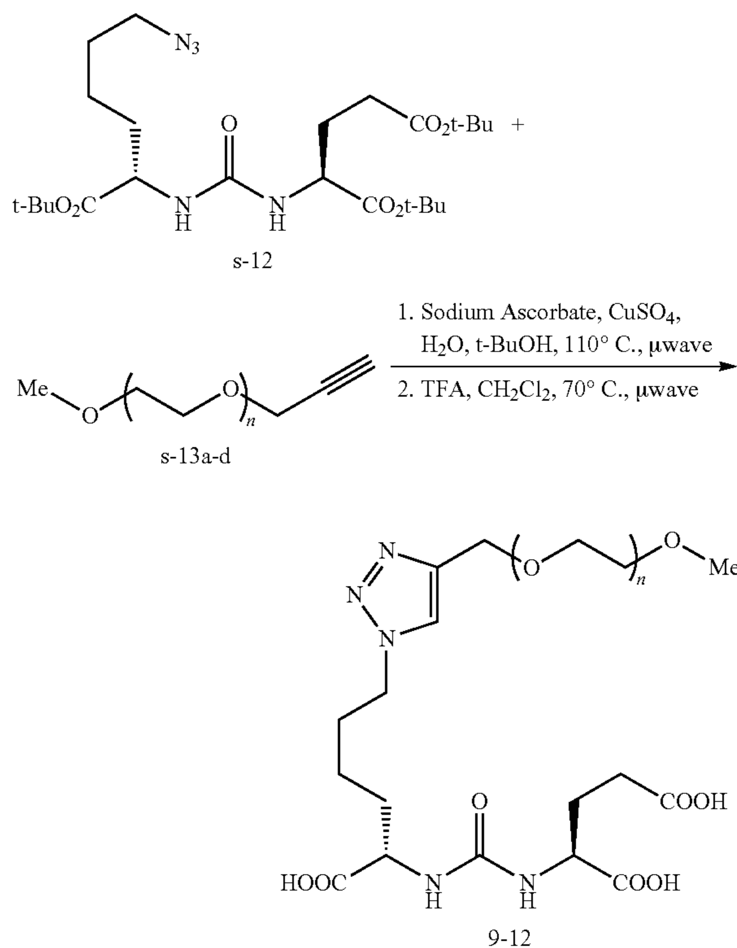
Scheme S-5: General synthesis of 8-12 (8, n = 0; 9, n = 2; 10, n = 4; 11, n = 8; 12, n = 12) from s-13a-e (a, n = 0; b, n = 2; c, n = 4; d, n = 8; e, n = 12).
