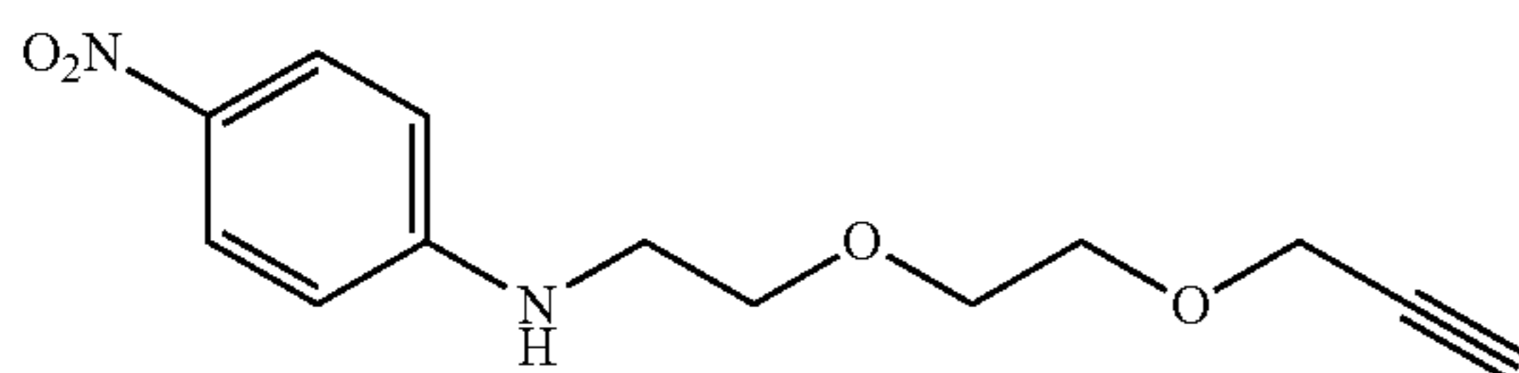
4-nitro-N-(2-(2-(prop-2-ynyloxy)ethoxy)ethyl)aniline (s-7)
