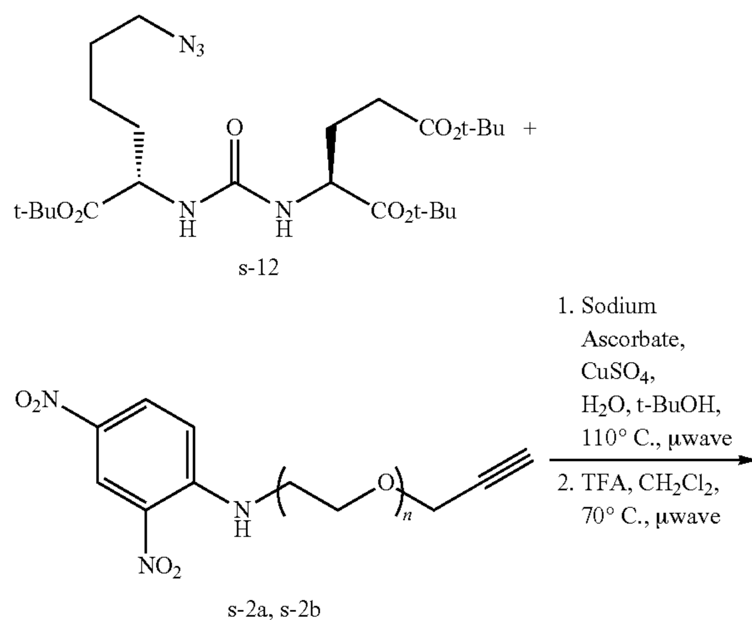
Scheme S-4: General synthesis of 2 and 3. (2, n = 1; 3, n = 2).
