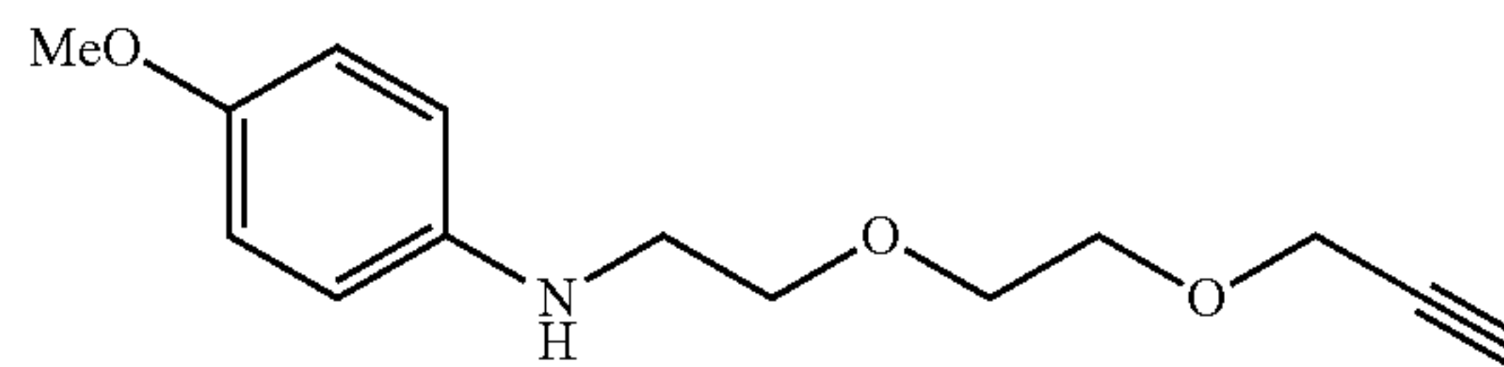
4-methoxy-N-(2-(2-(prop-2-ynyloxy)ethoxy)ethyl)aniline (s-10)
