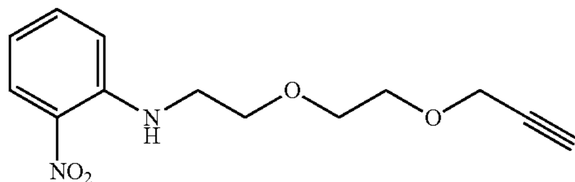
2-nitro-N-(2-(2-(prop-2-ynyloxy)ethoxy)ethyl)aniline (s-6)
