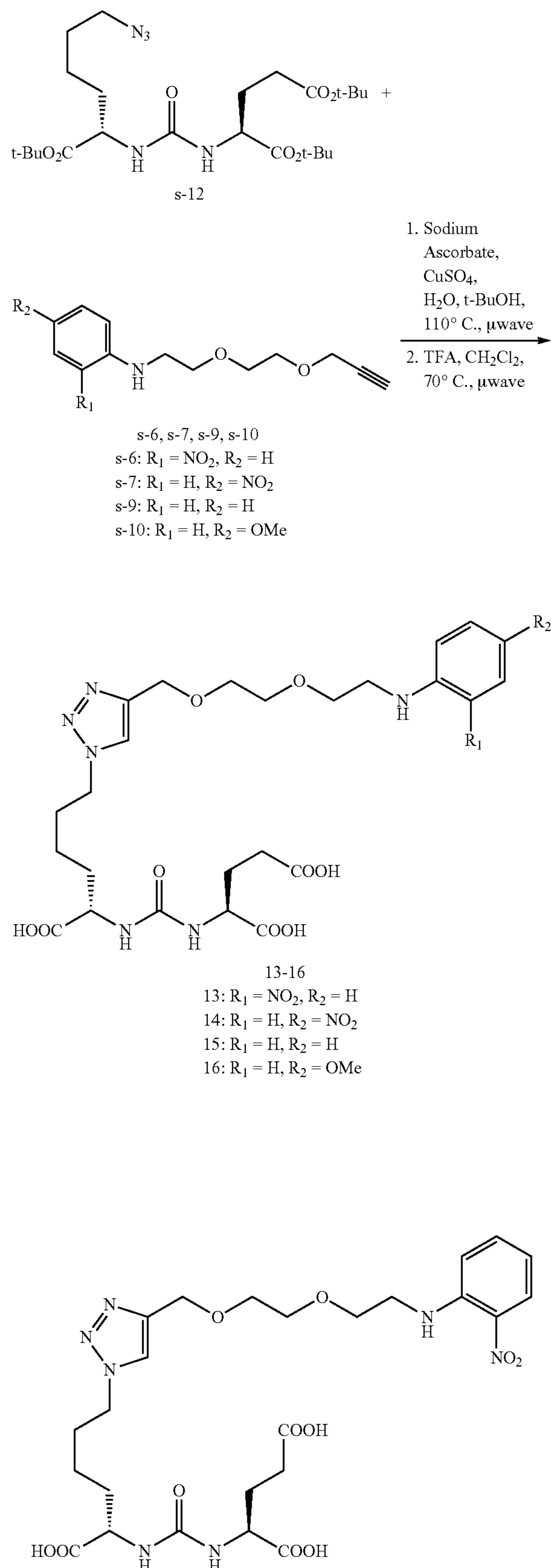
Scheme S-6: General synthesis of 13-16.
