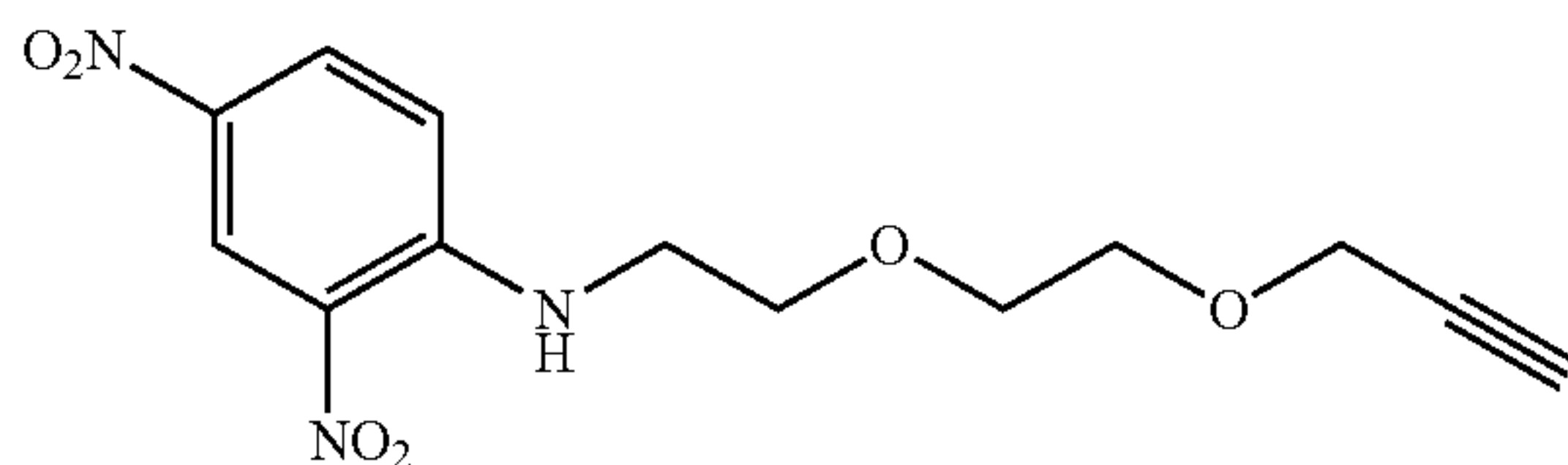
2,4-dinitro-N-(2-(2-(prop-2-ynyloxy)ethoxy)ethyl)aniline (s-2b)
