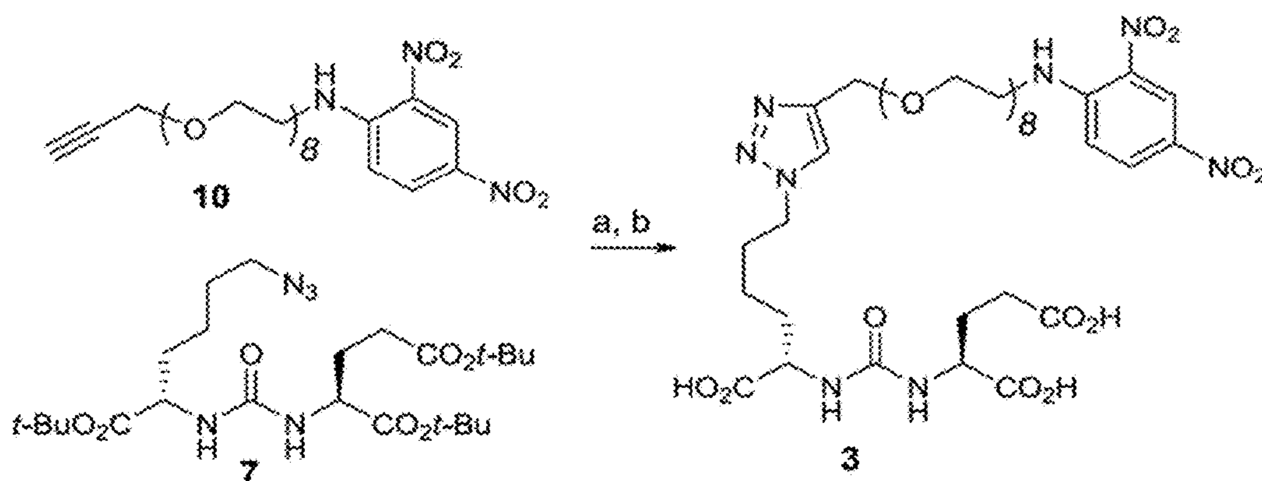
Scheme 3
