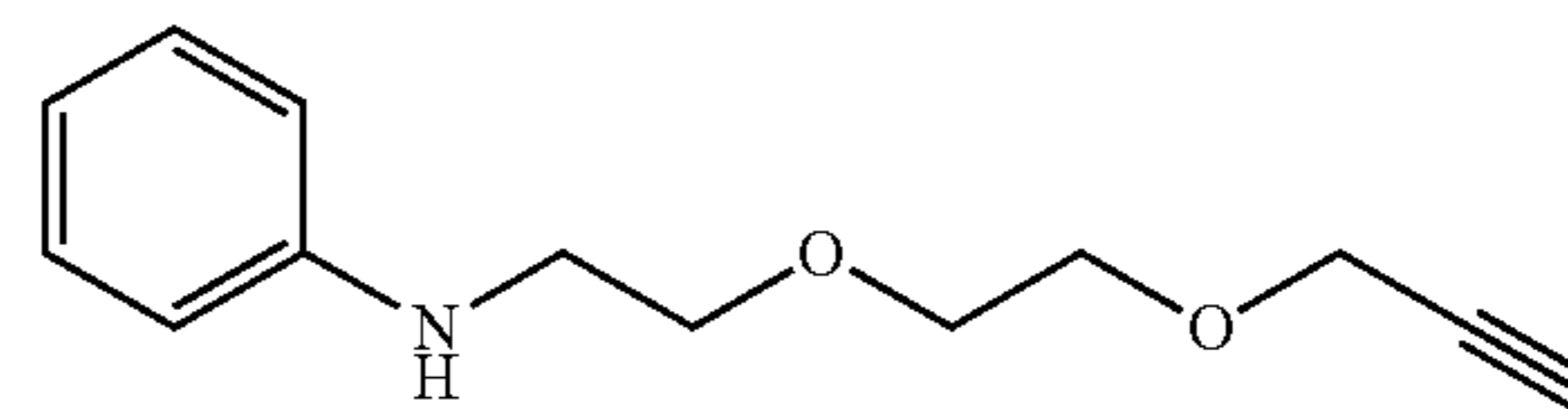
N-(2-(2-(prop-2-ynyloxy)ethoxy)ethyl)aniline (s-9)
