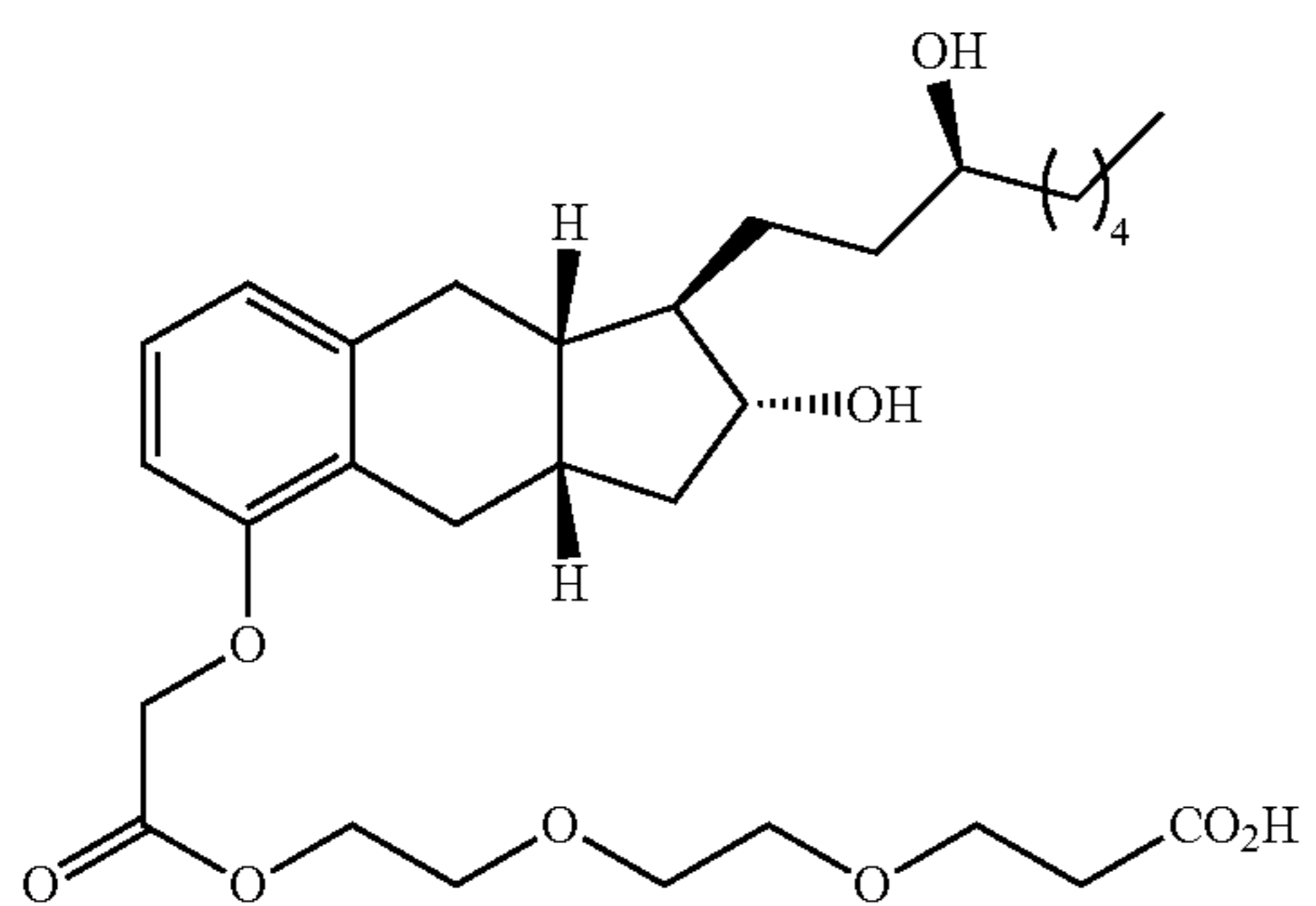
Compound II-19
