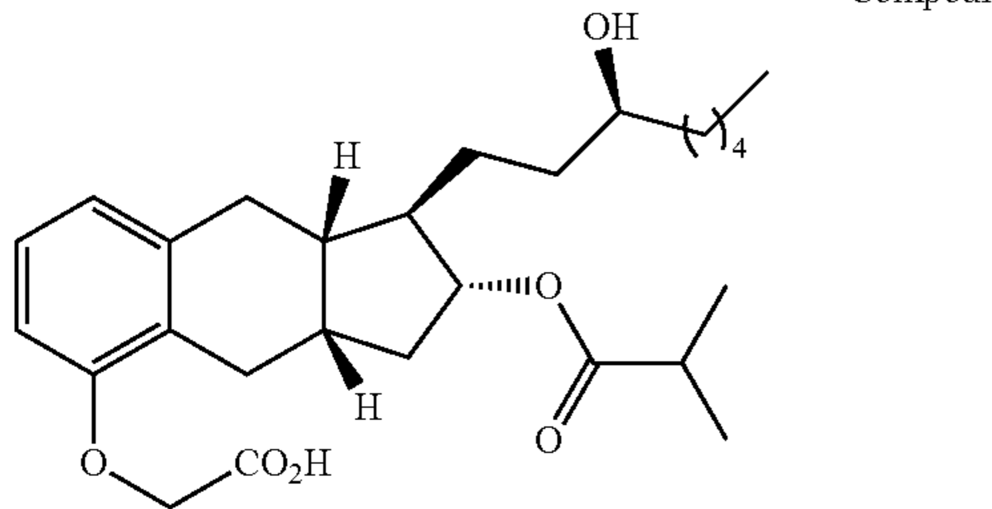
Compound Ia-23
