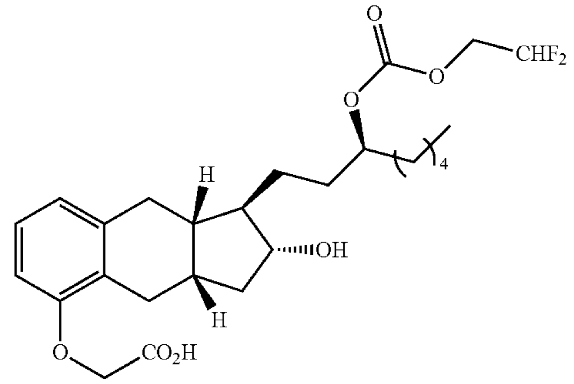
Compound Ib-13
