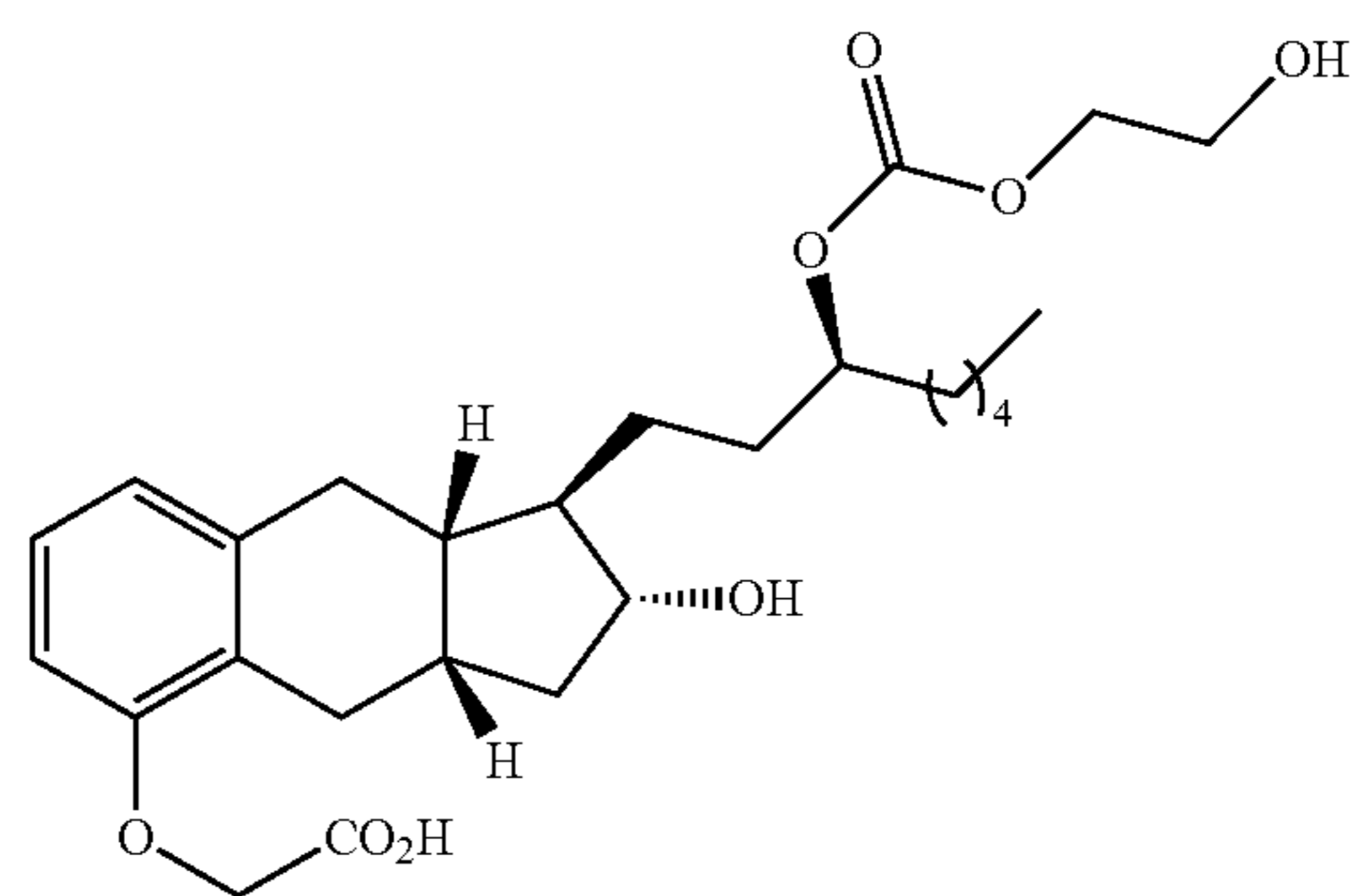
Compound Ib-14
