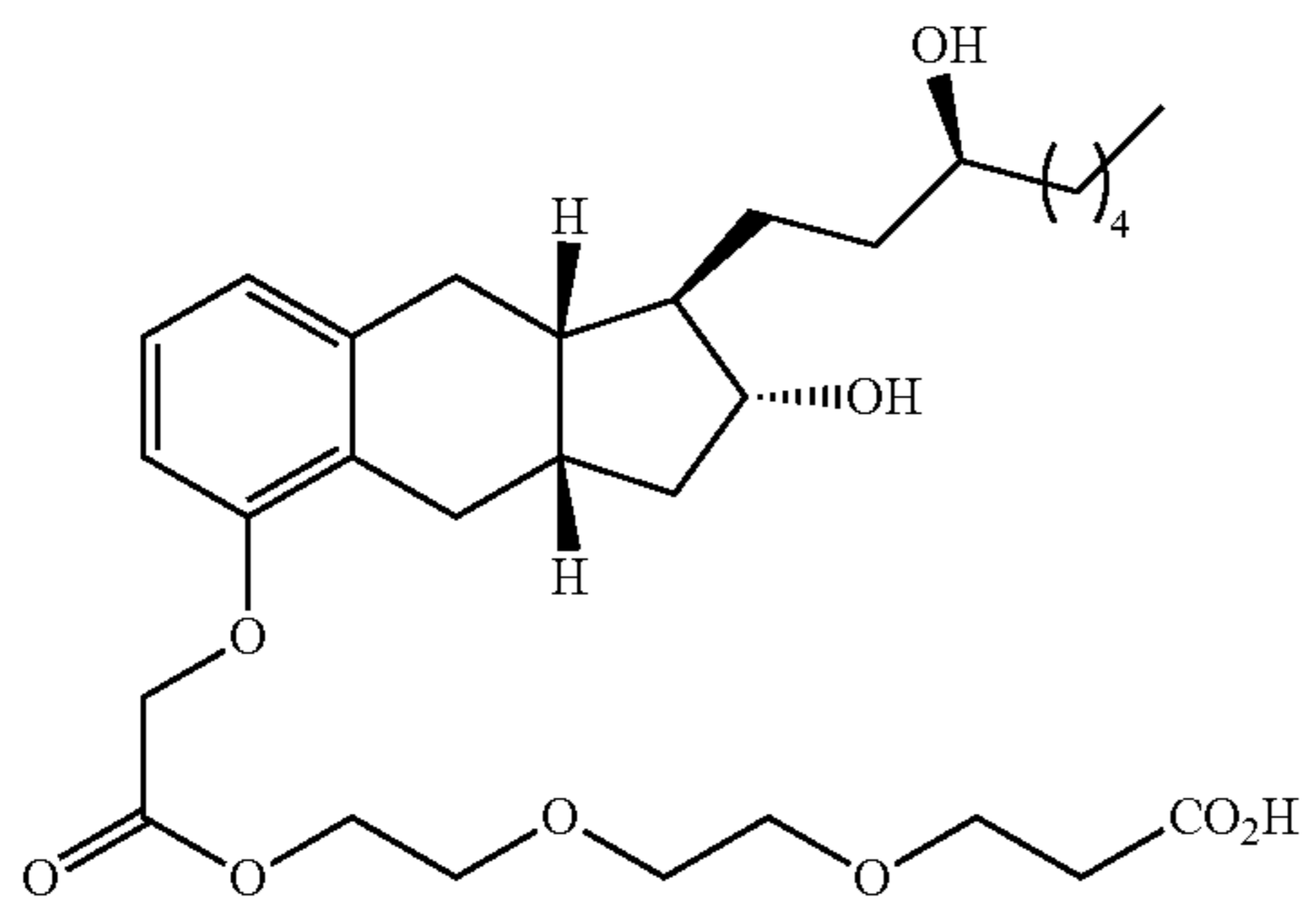
Compound II-19
