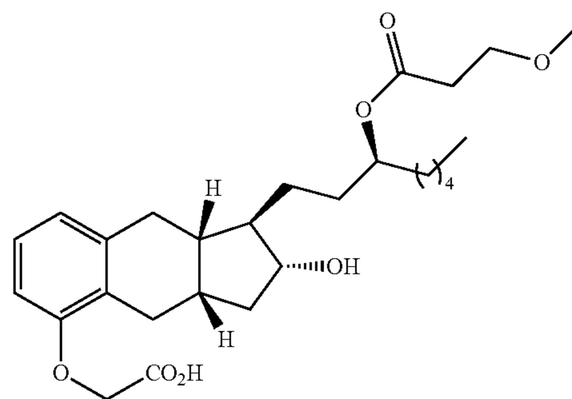
Compound Ib-6
