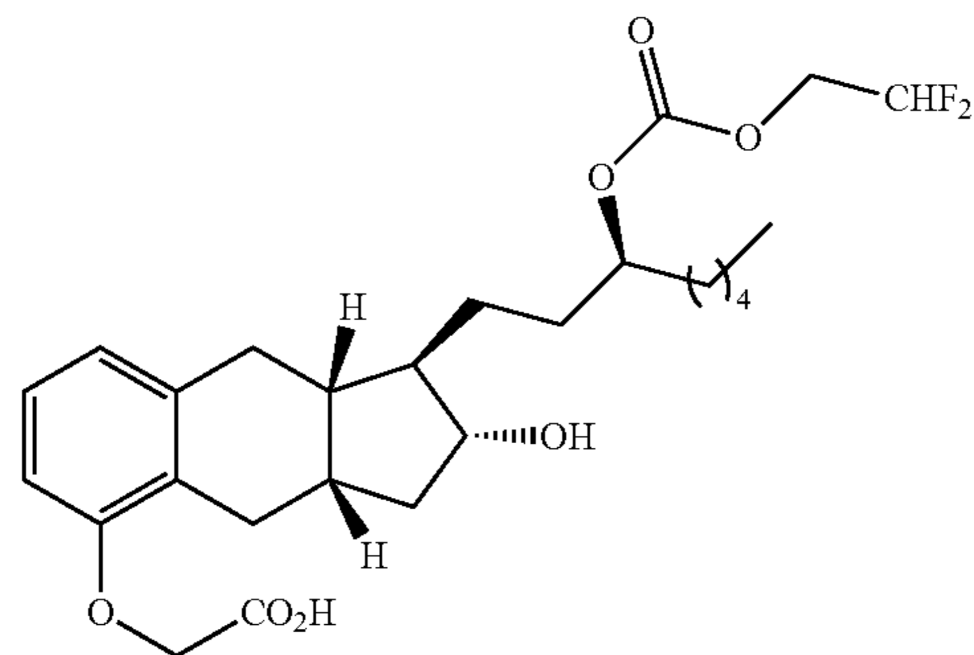
Compound Ib-13
