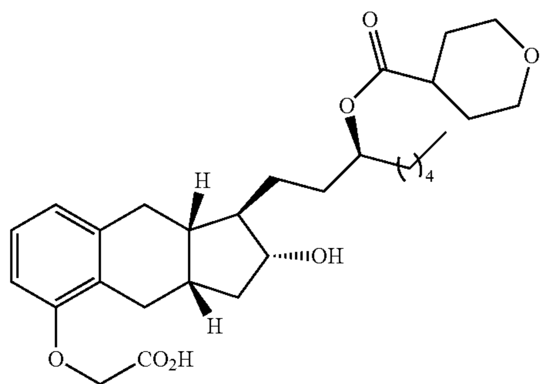
Compound Ib-34
