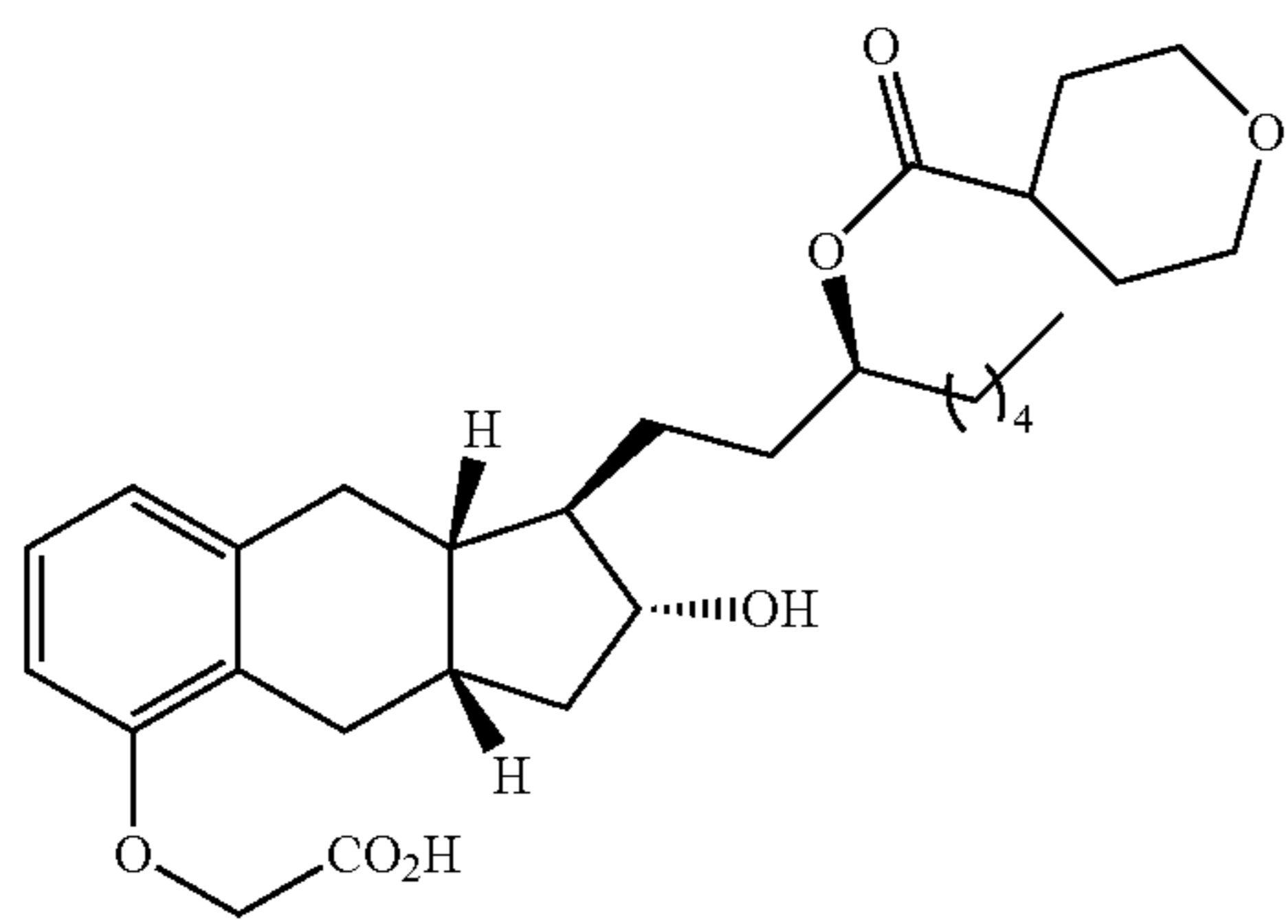
Compound Ib-34
