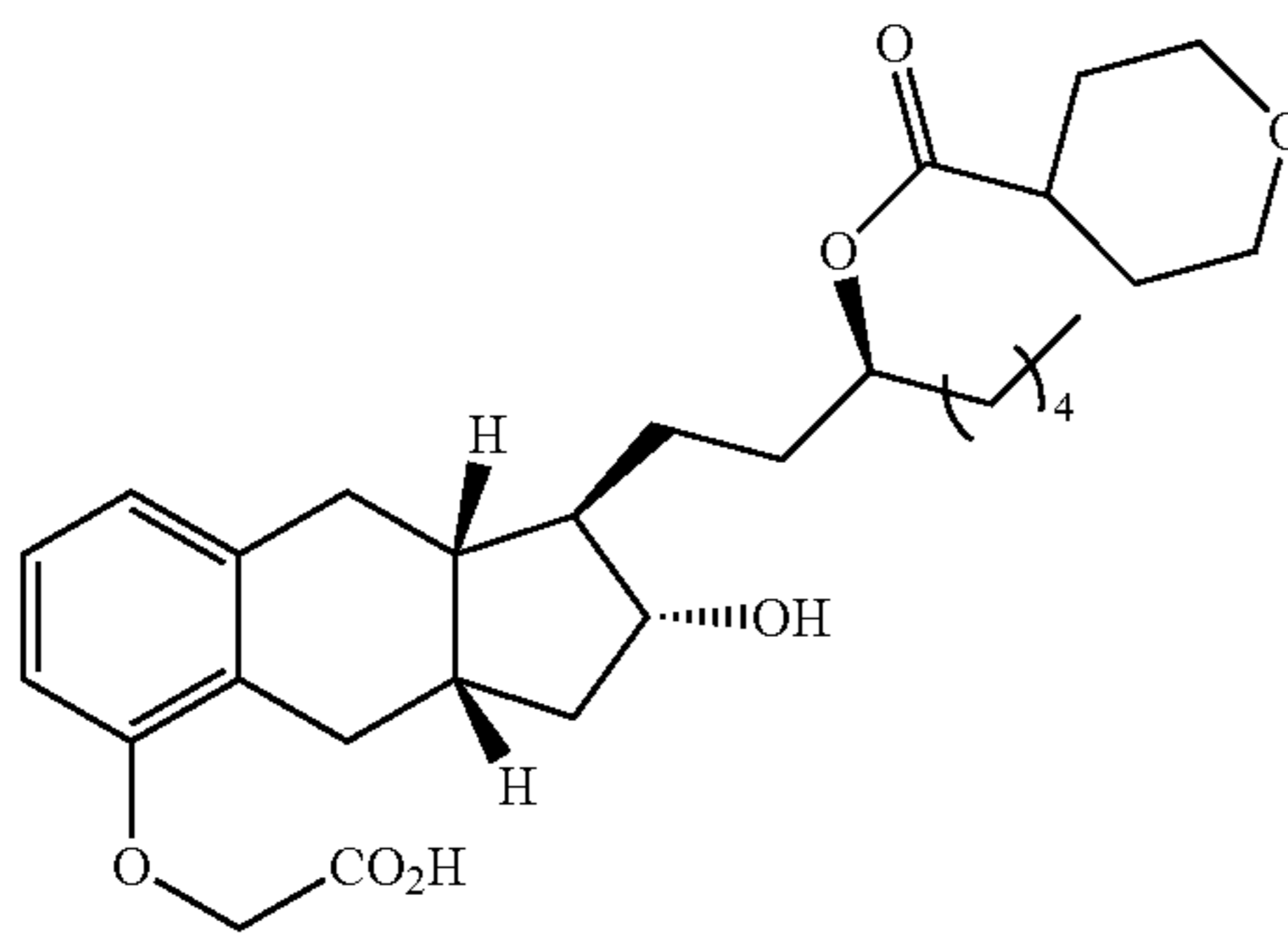
Compound Ib-34
