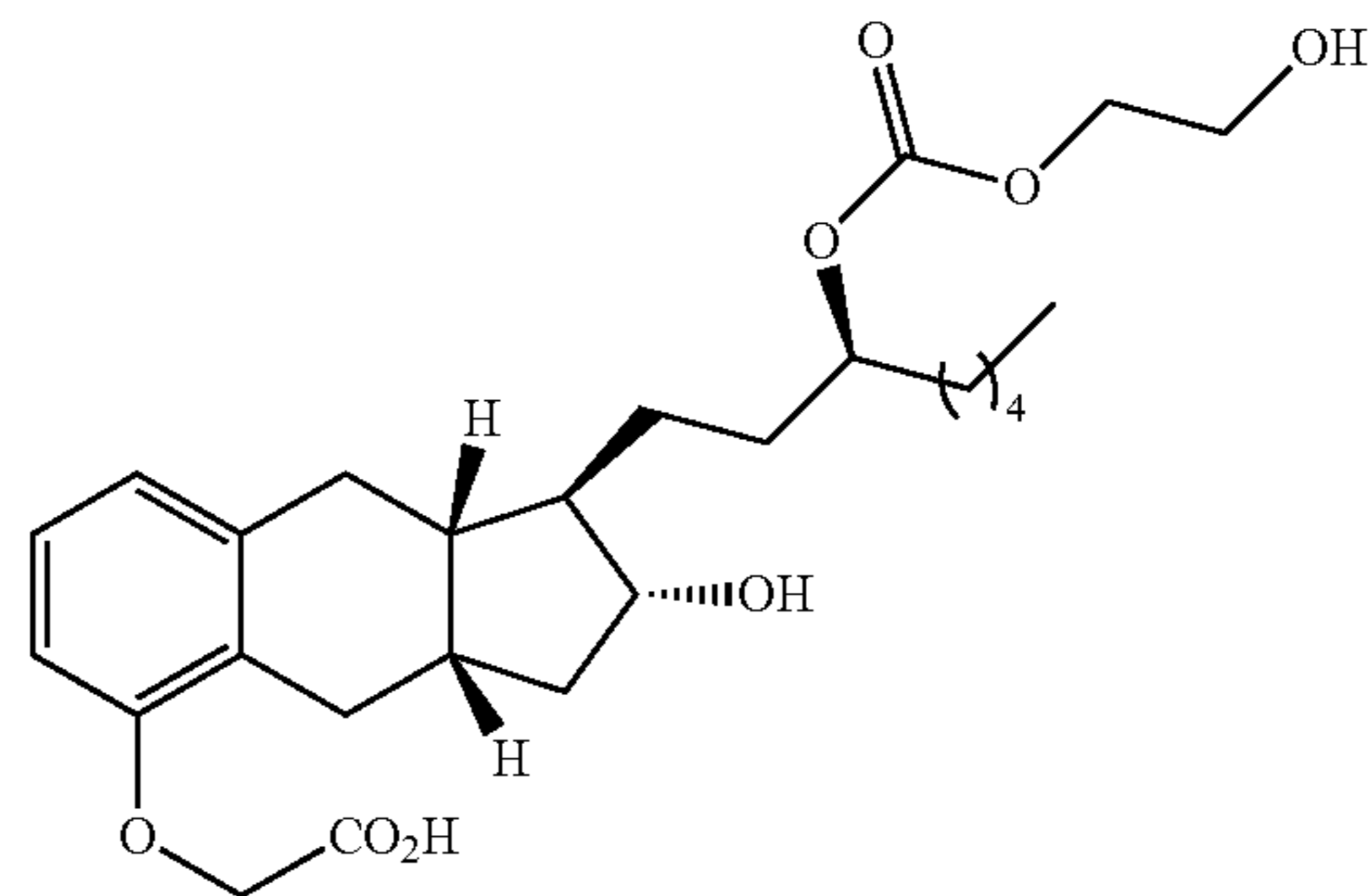
Compound Ib-14
