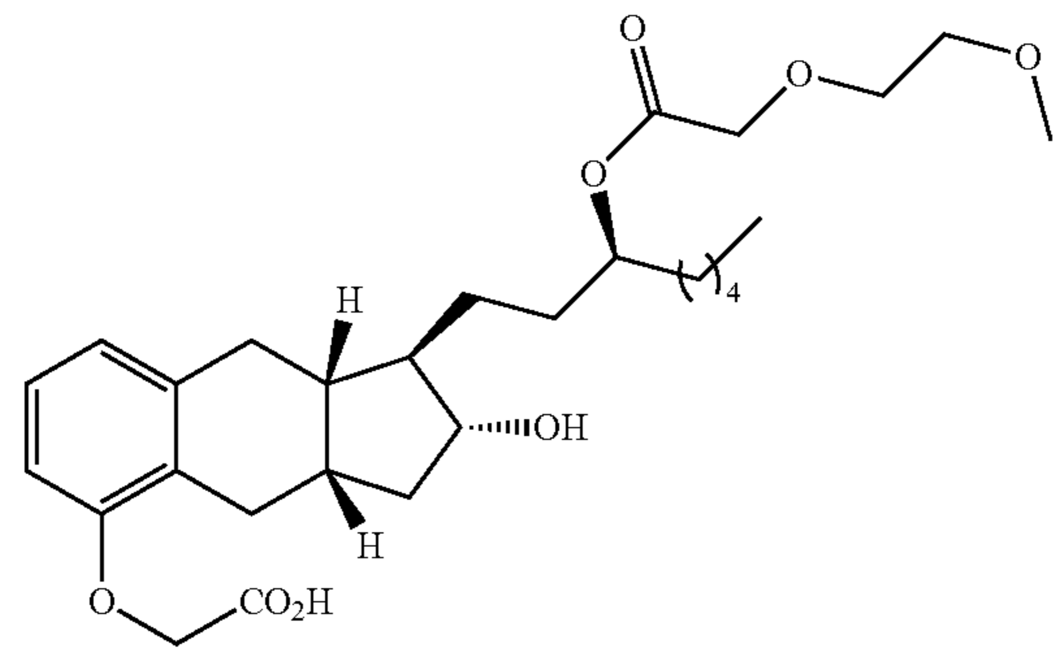
Compound Ib-21
