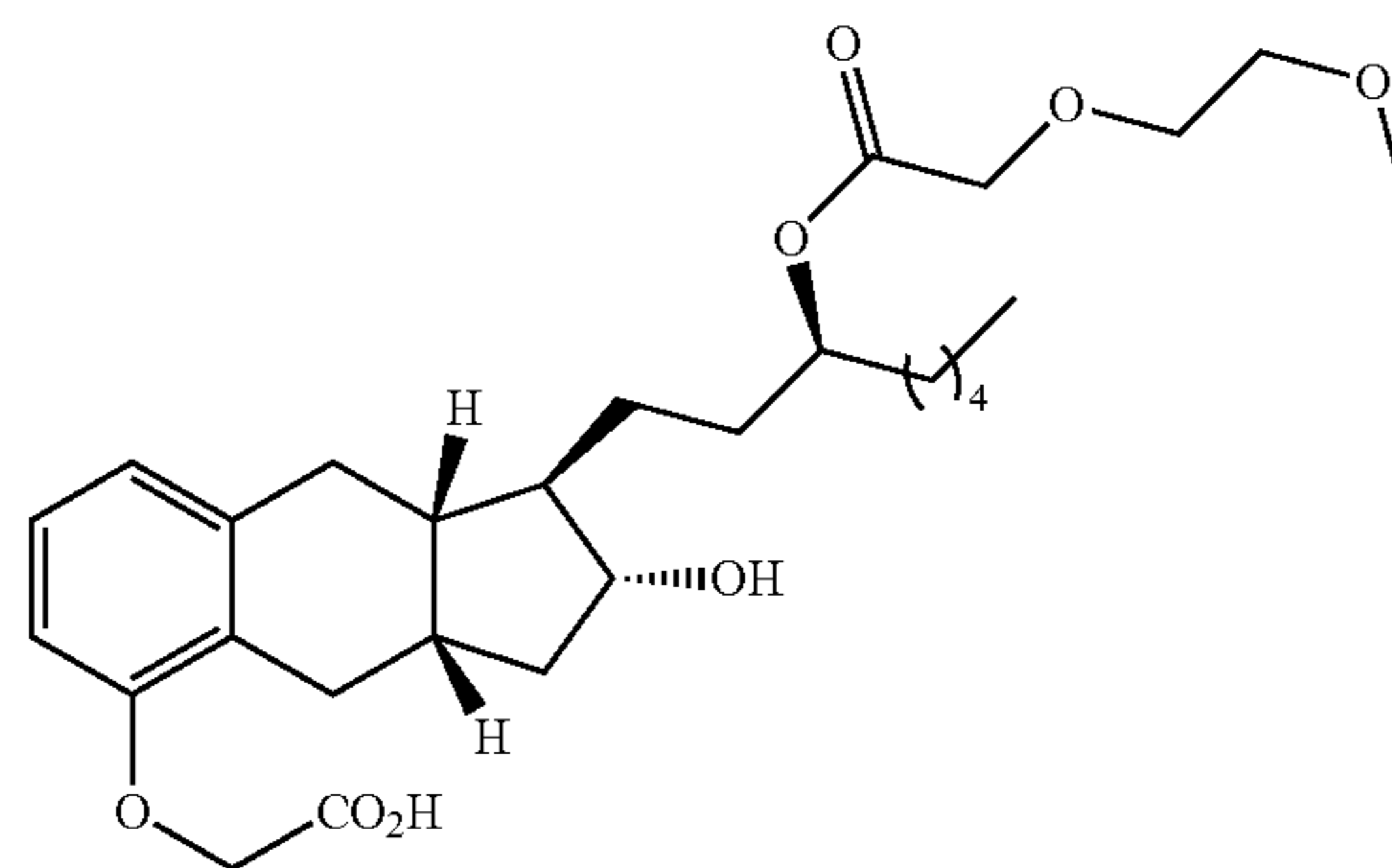
Compound Ib-21
