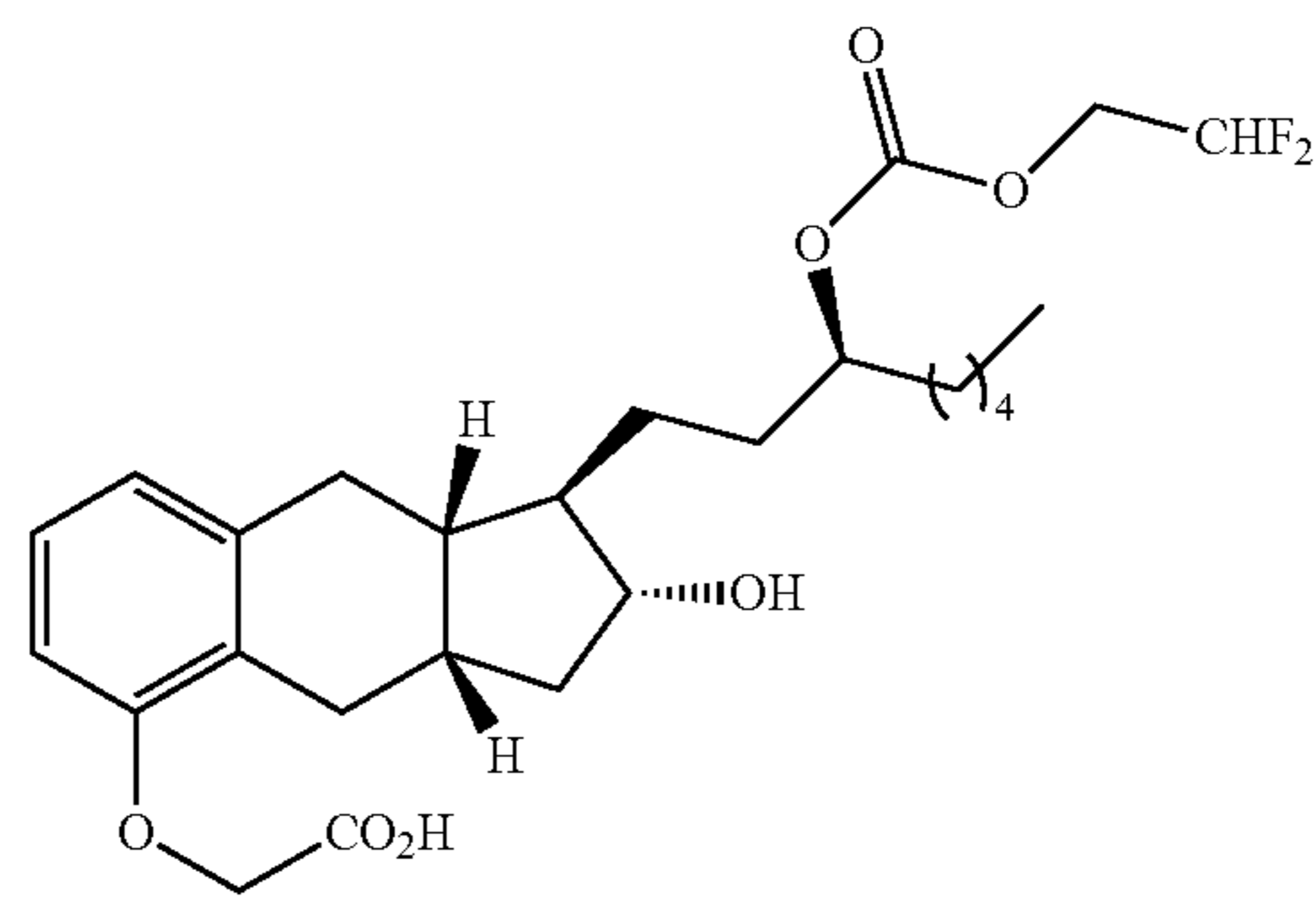
Compound Ib-13
