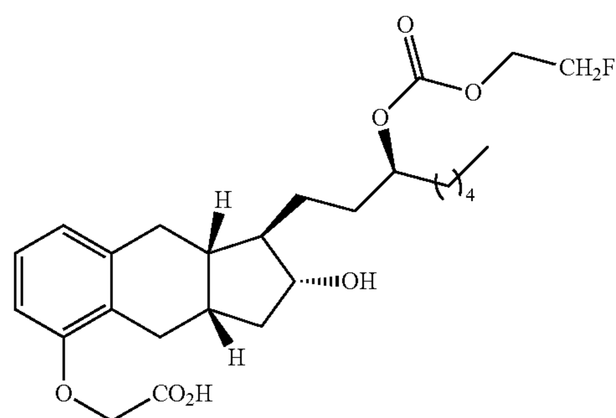
Compound Ib-12
