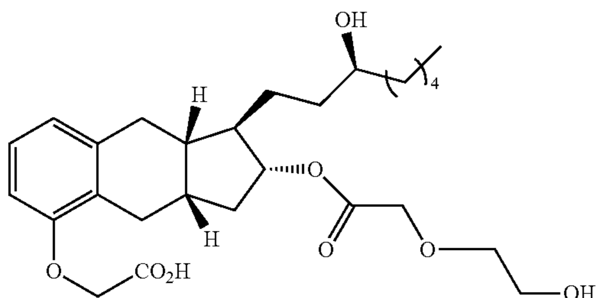
Compound Ia-21
