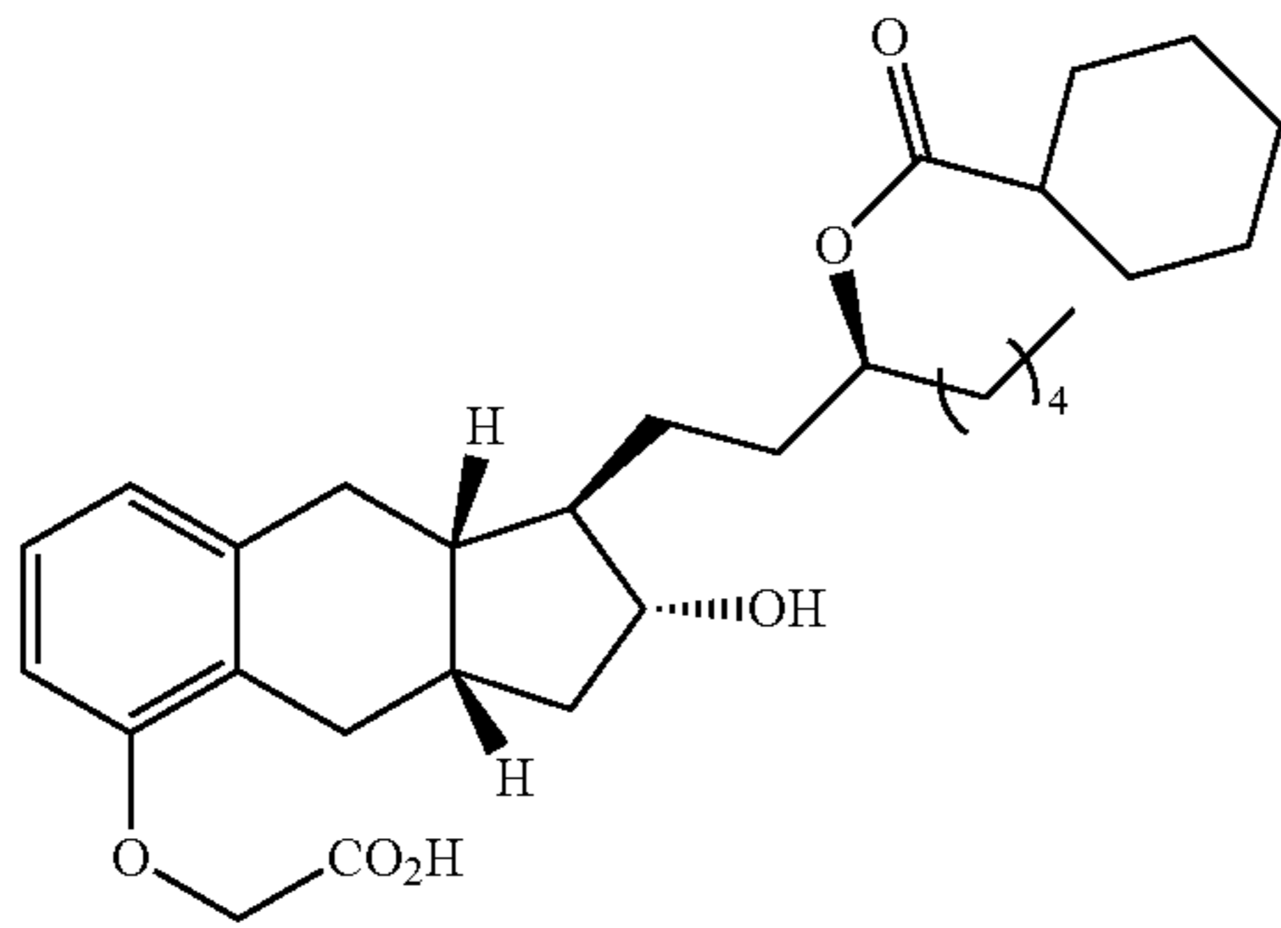
Compound Ib-31
