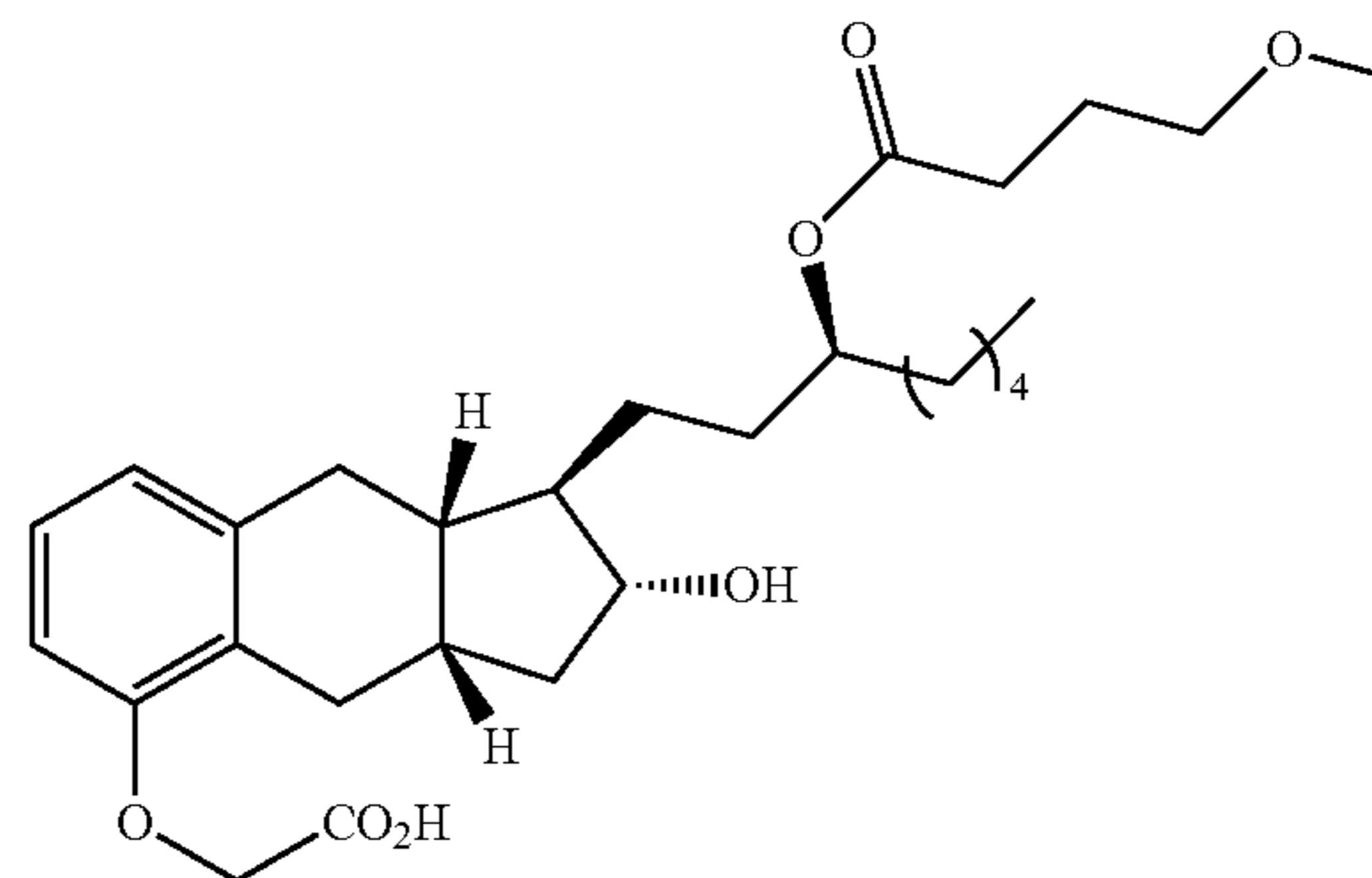
Compound Ib-19
