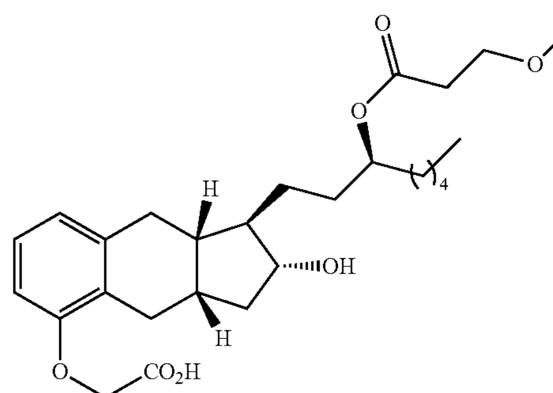
Compound Ib-6
