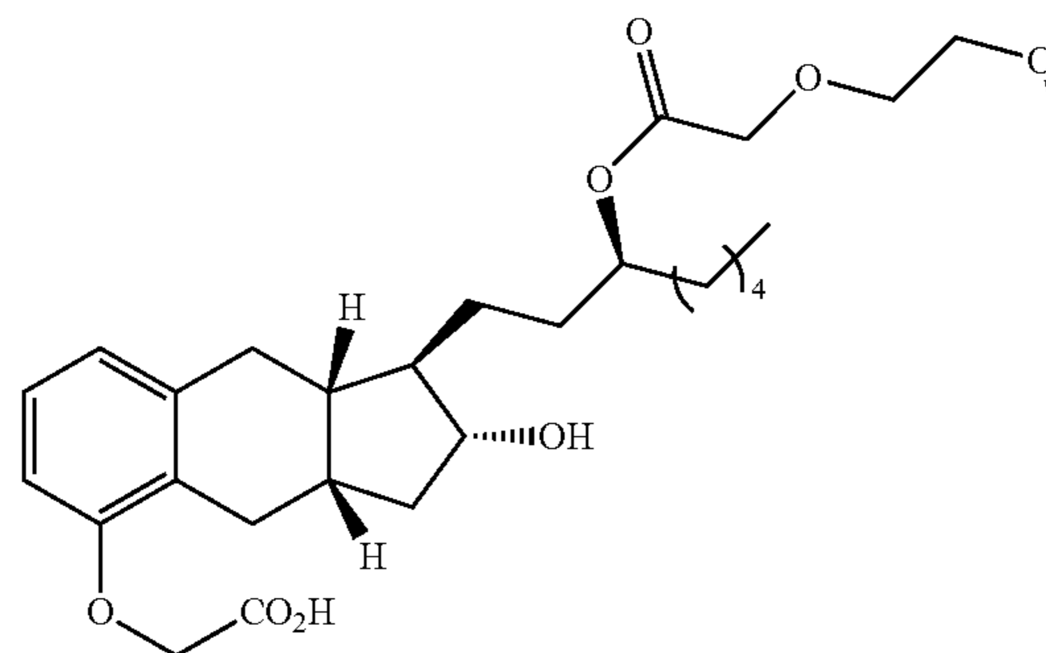
Compound Ib-21
