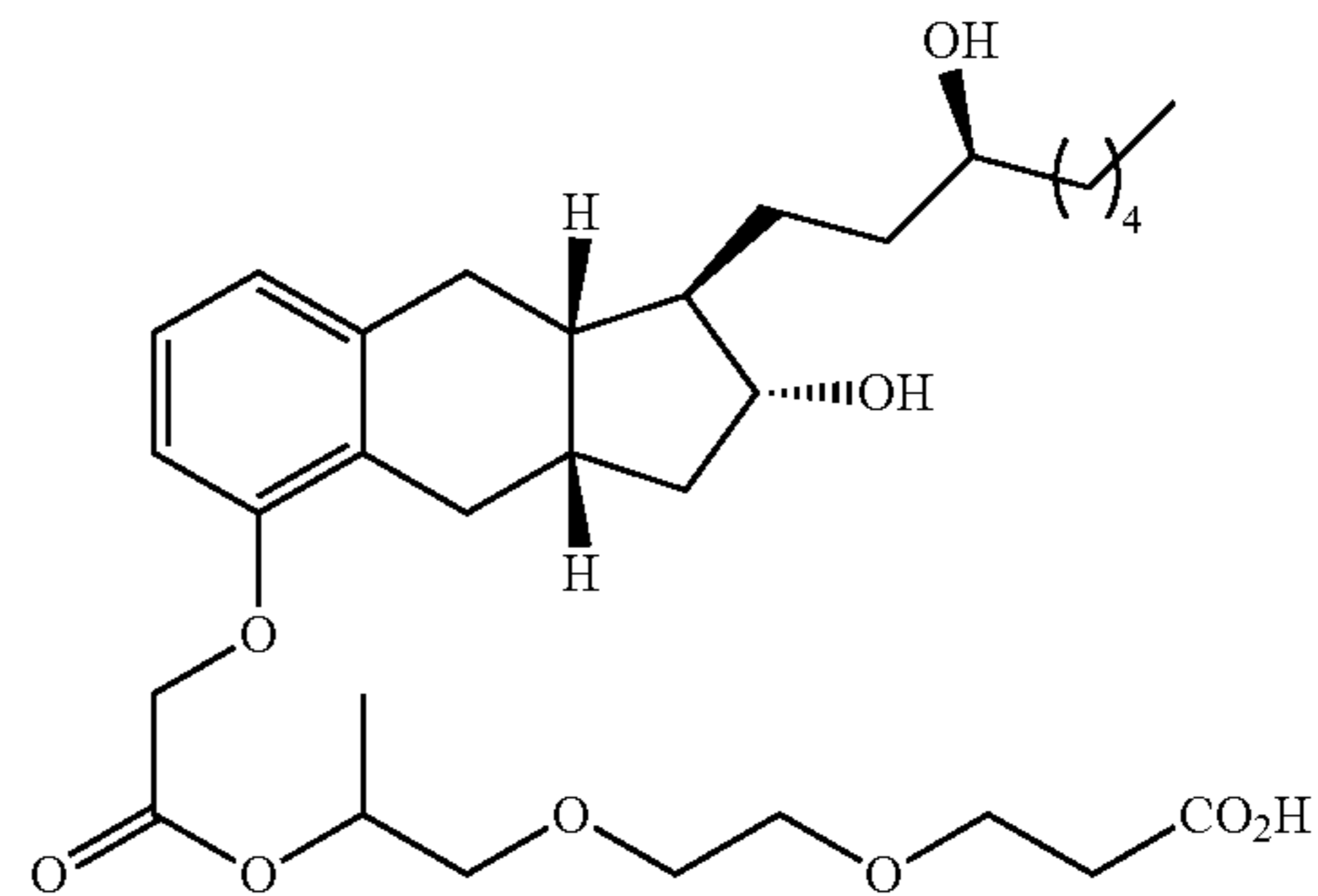
Compound II-21
