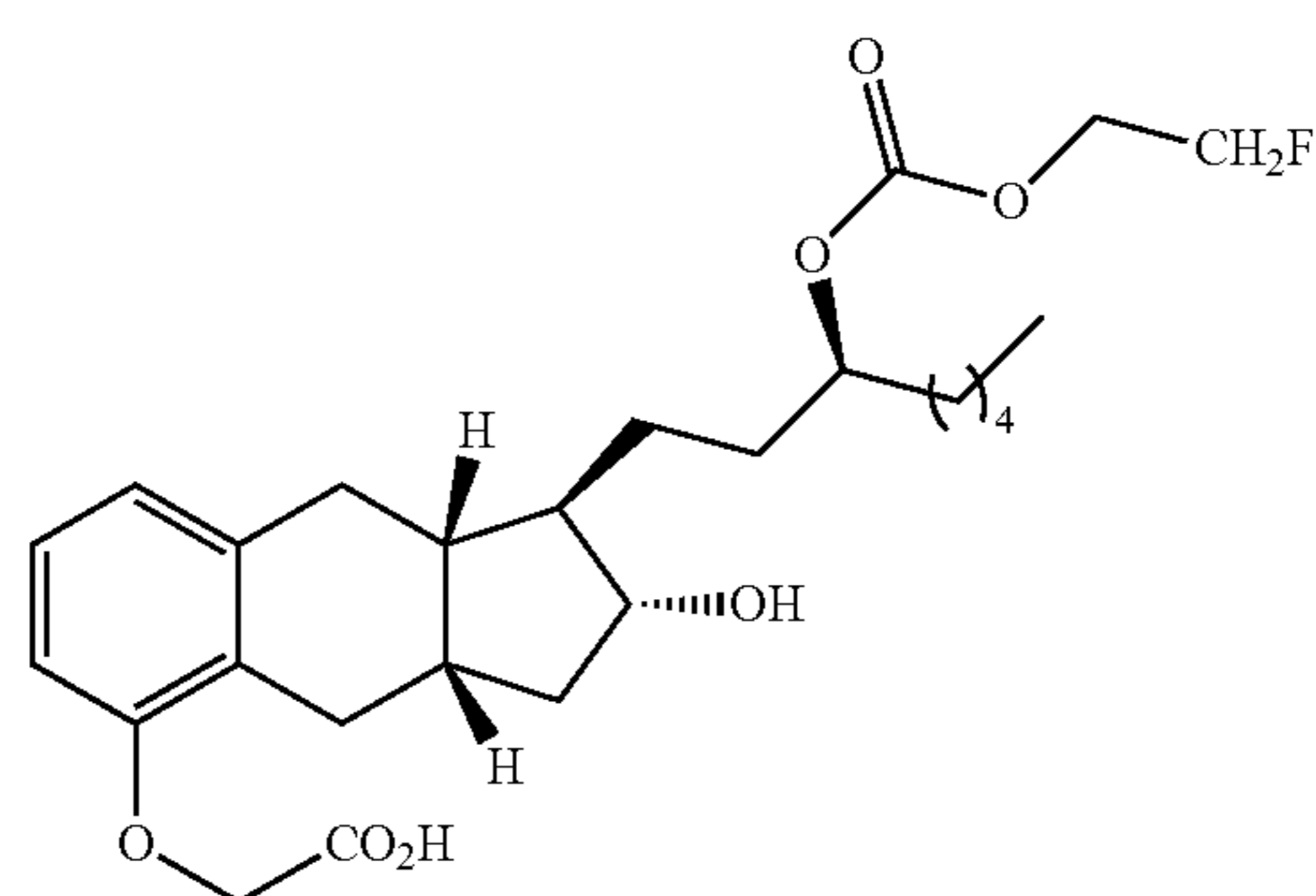
Compound Ib-12
