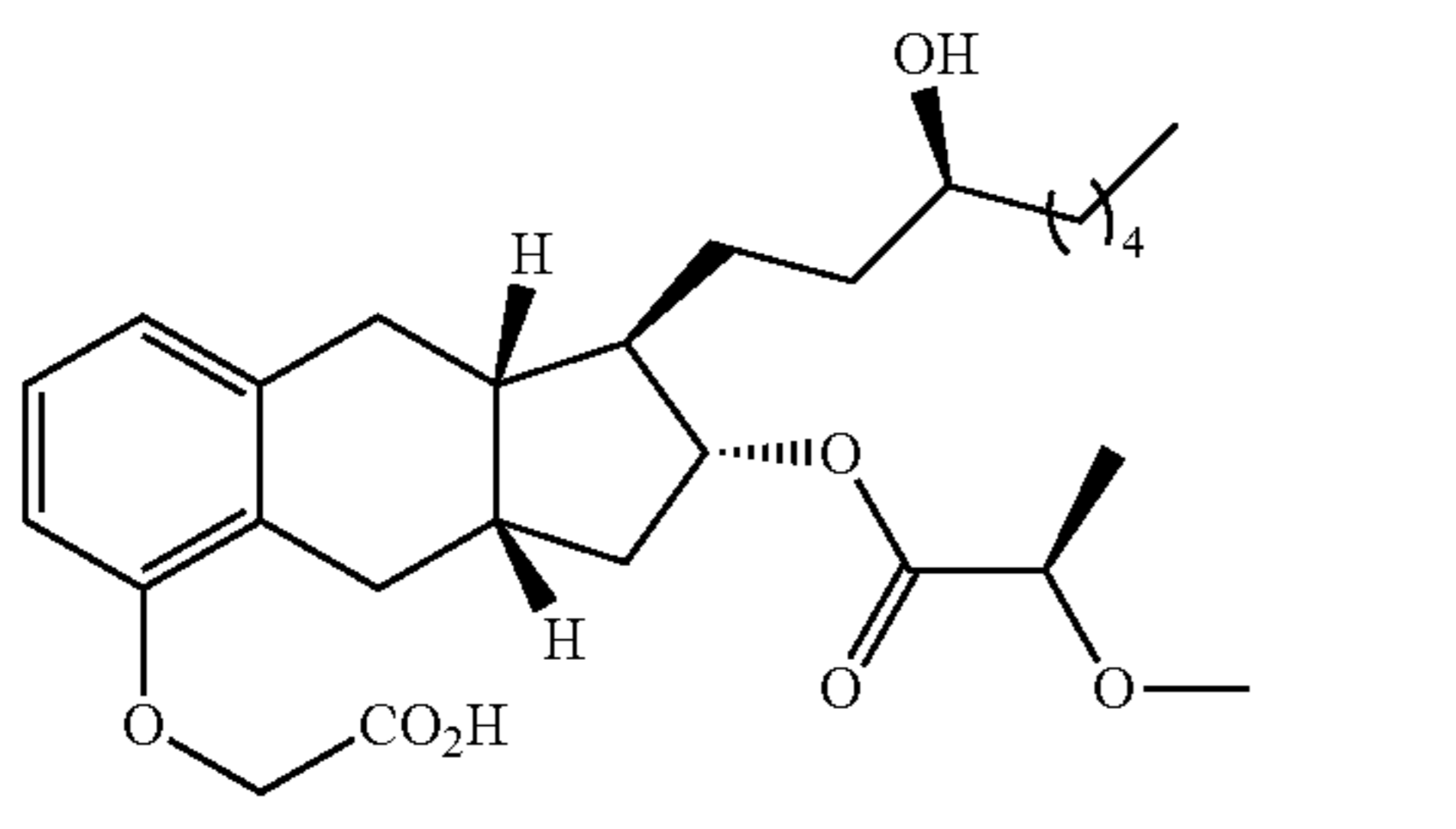
Compound Ia-24
