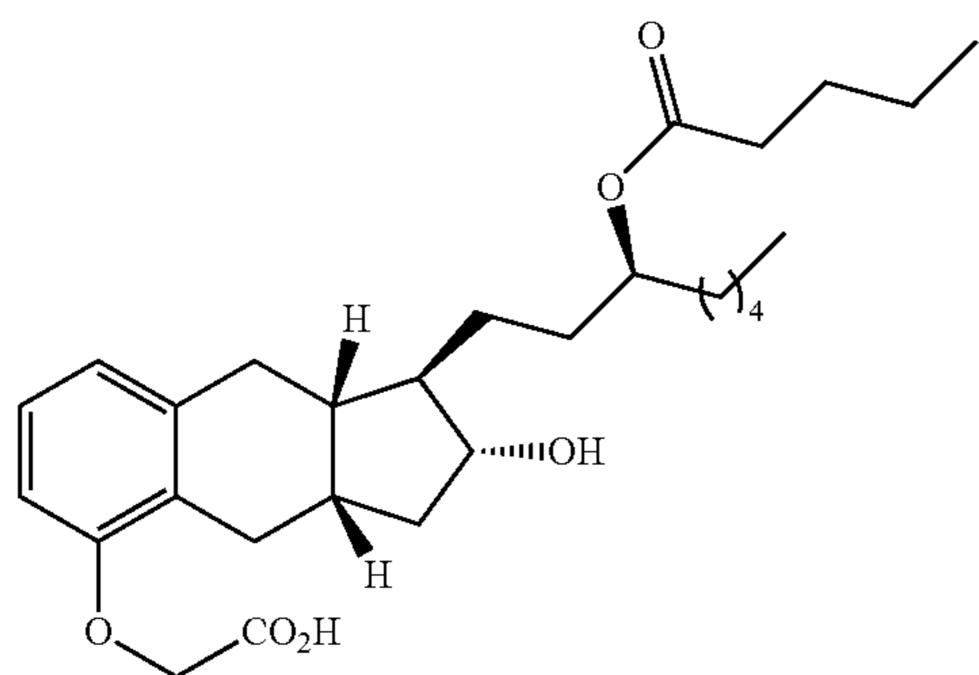
Compound Ib-3
