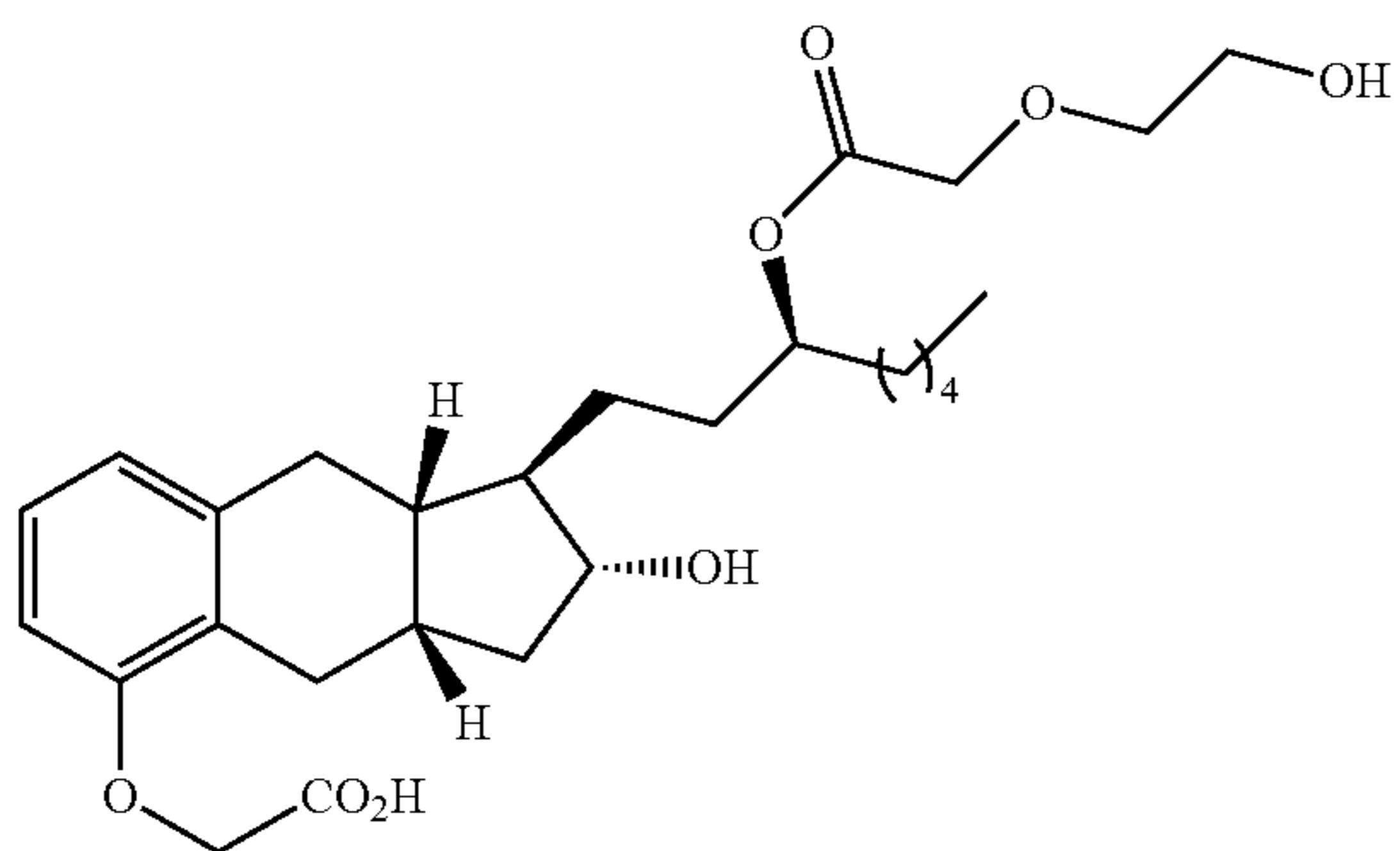
Compound Ib-20
