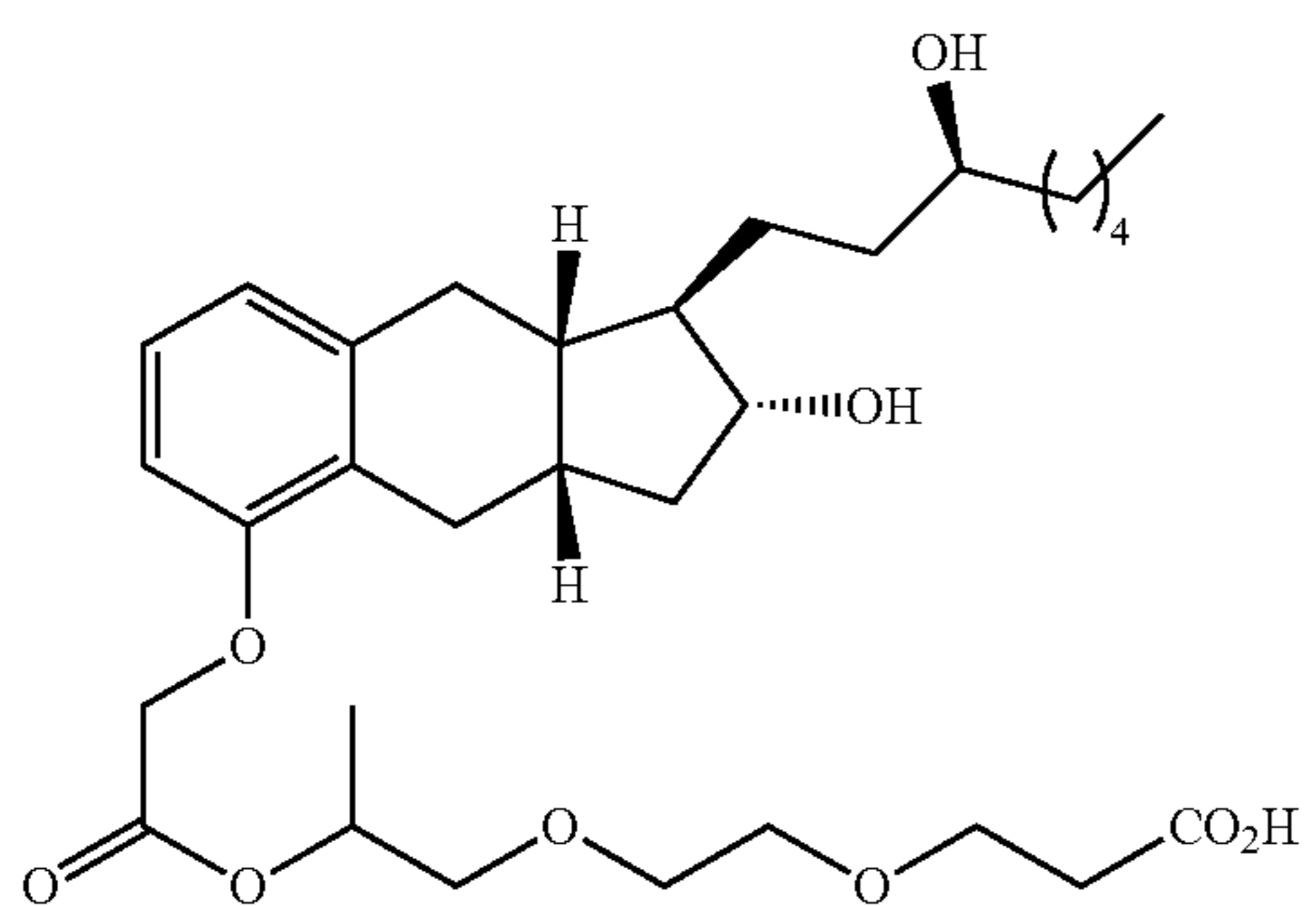
Compound II-20
