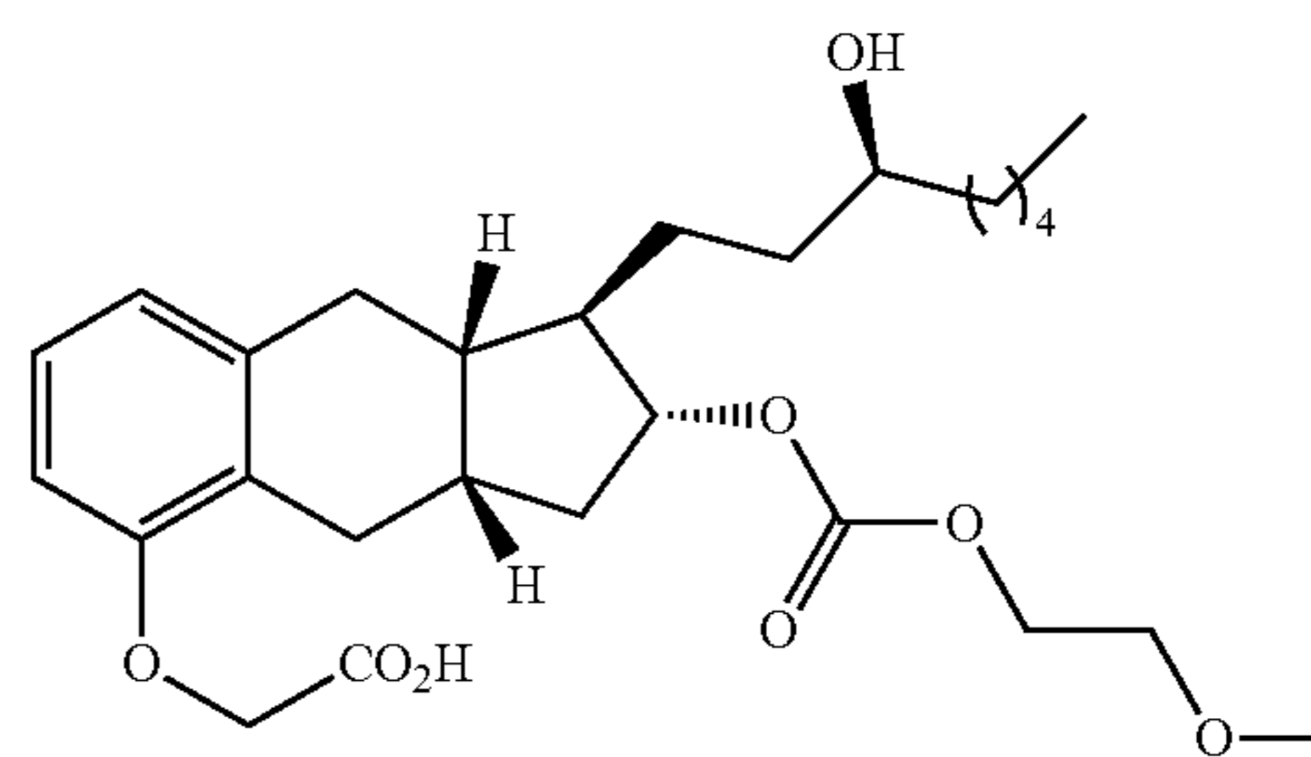
Compound Ia-15
