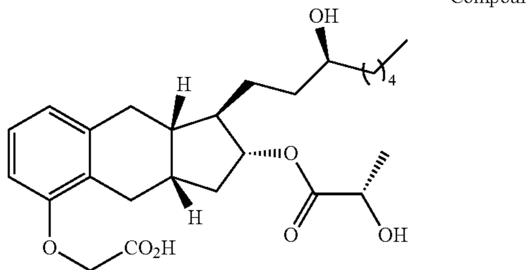
Compound Ia-25
