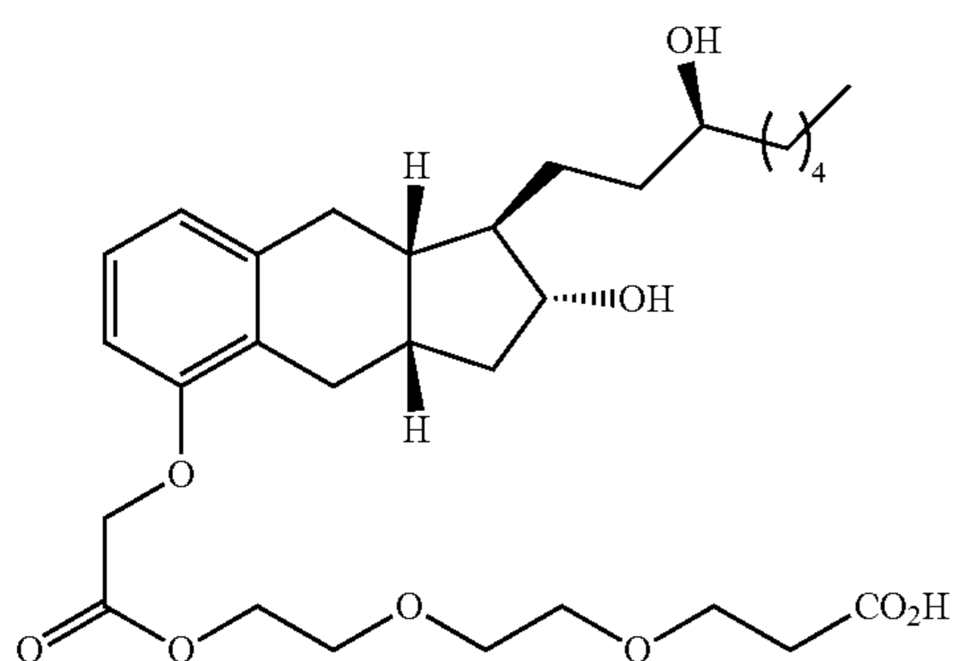
Compound II-19
