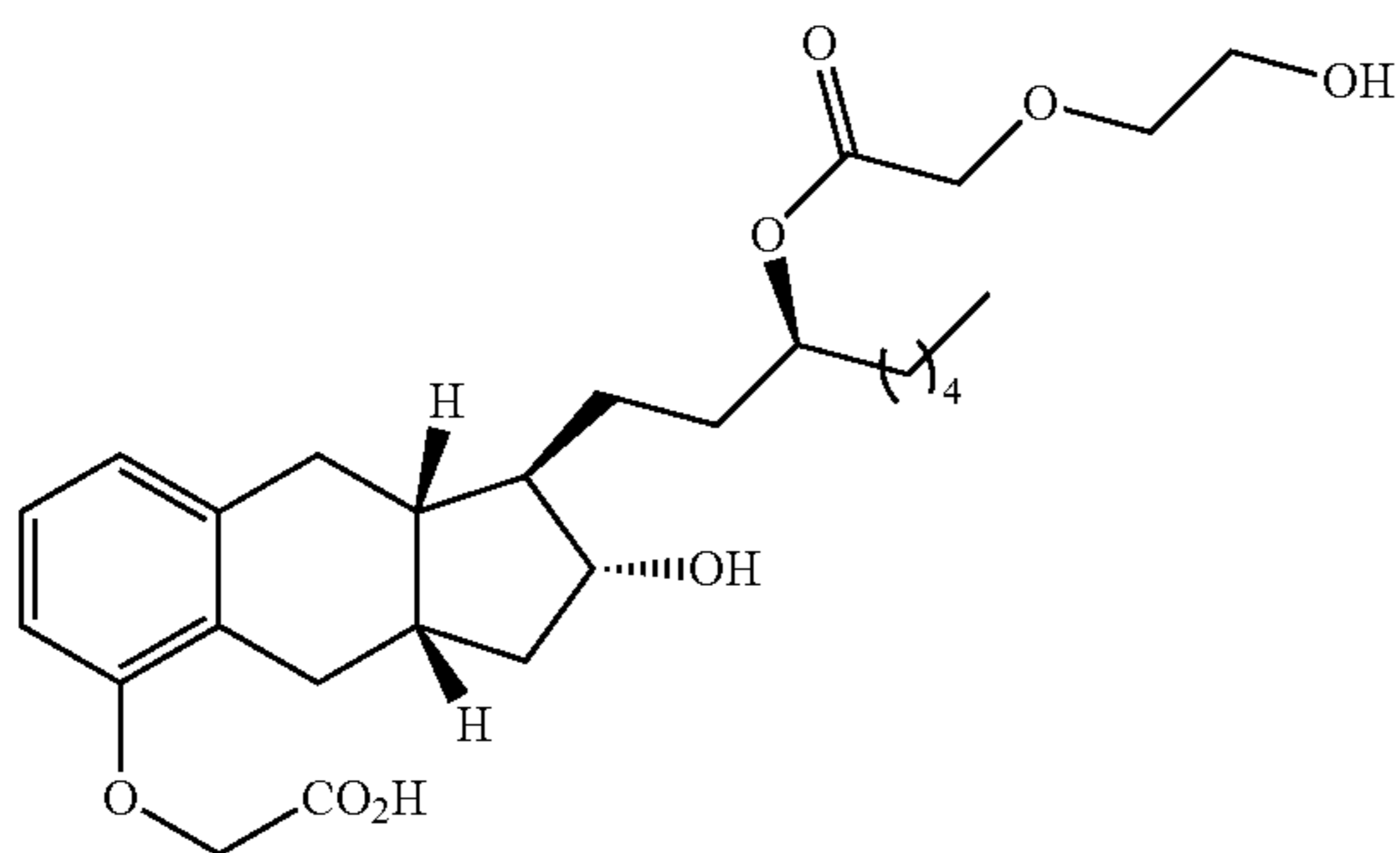
Compound Ib-20
