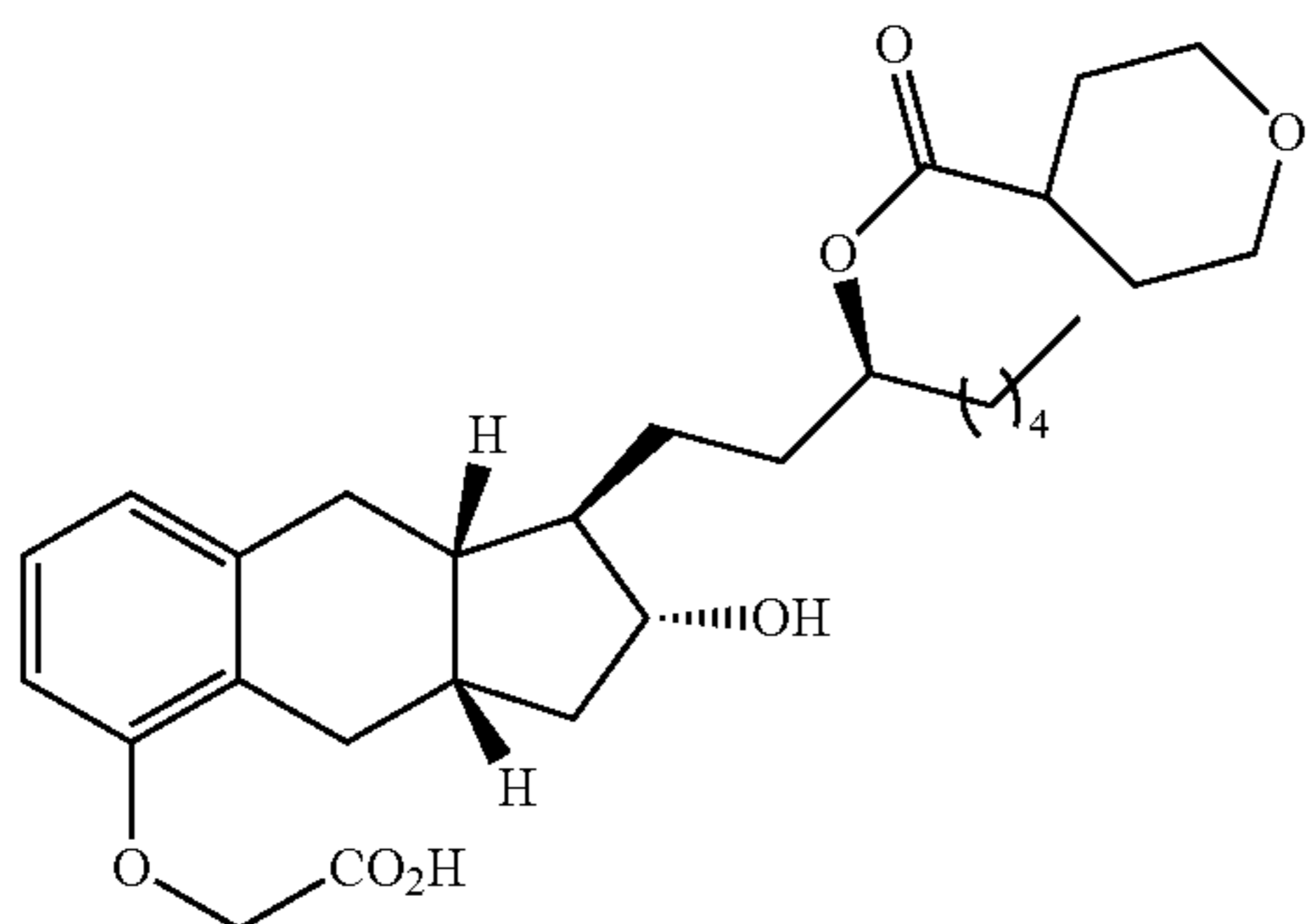
Compound Ib-34
