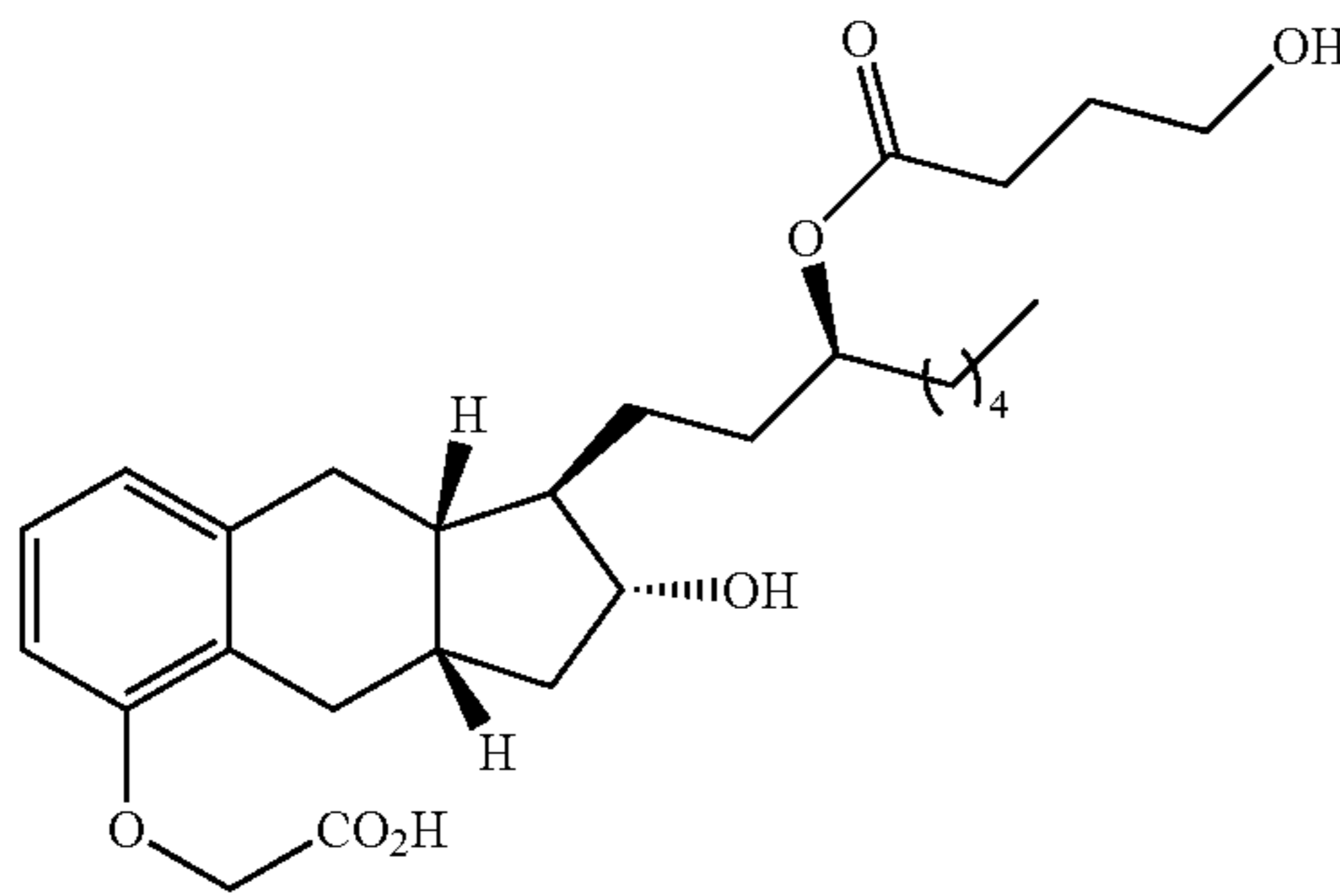
Compound Ib-18
