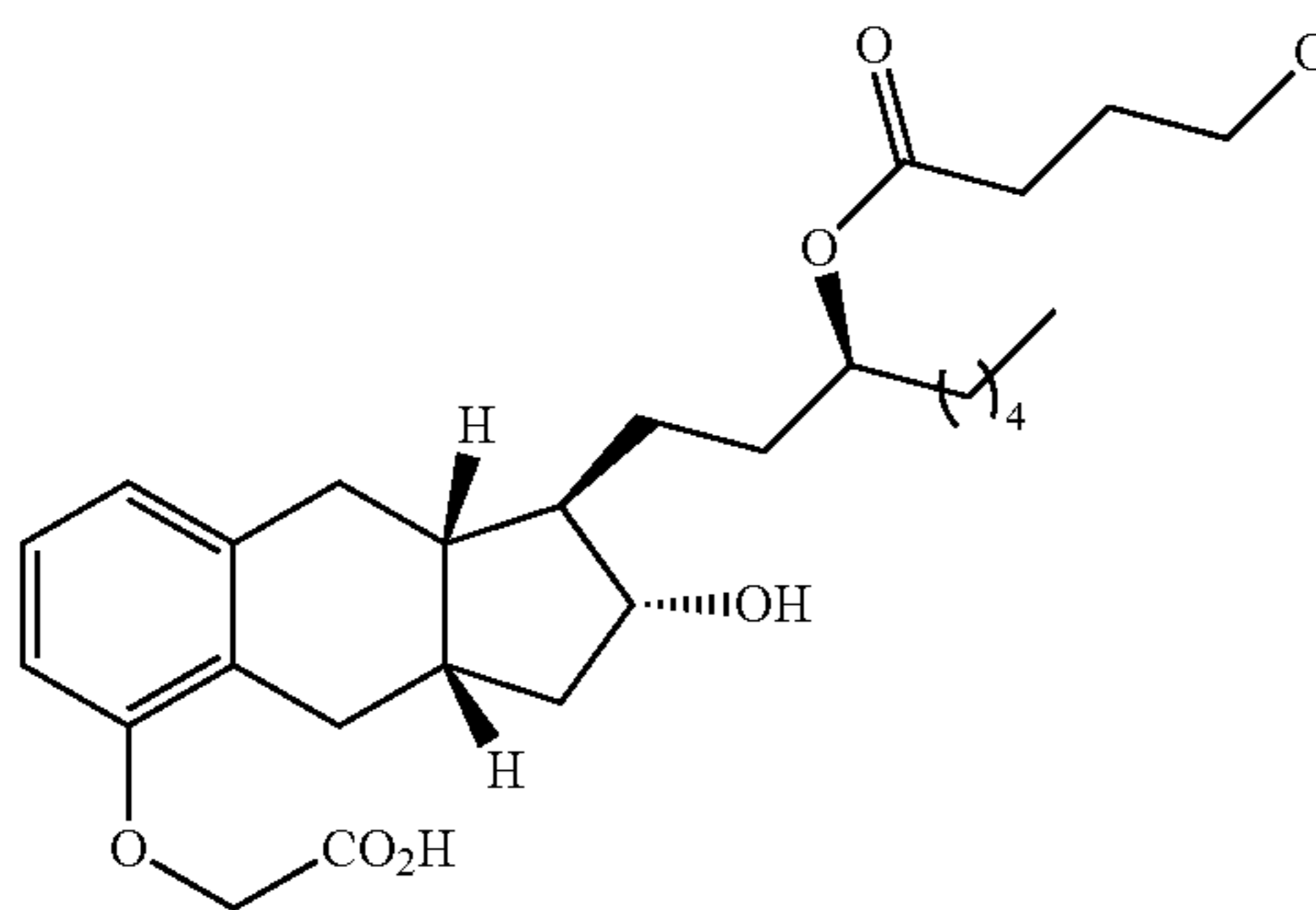
Compound Ib-18
