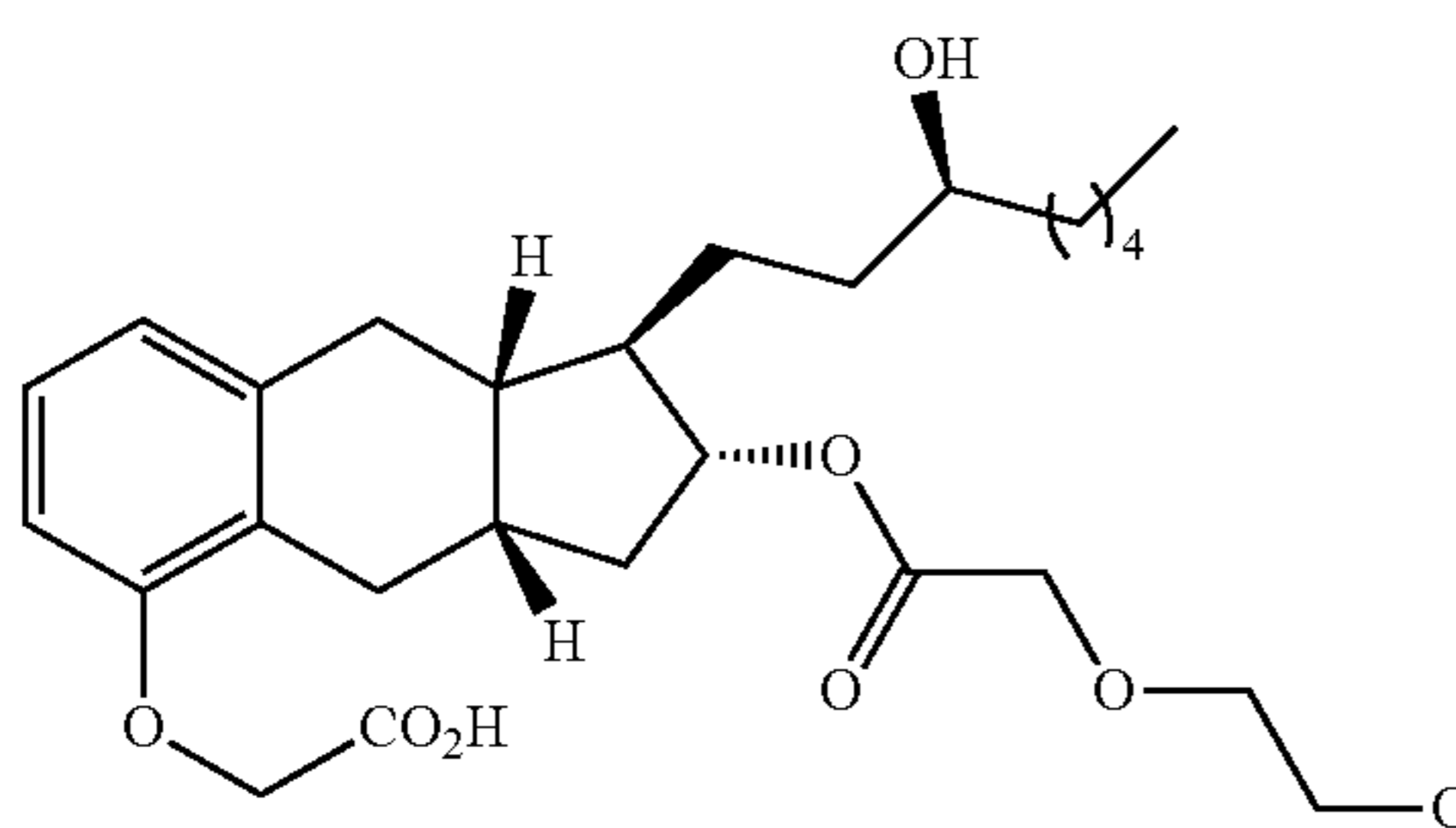
Compound Ia-22
