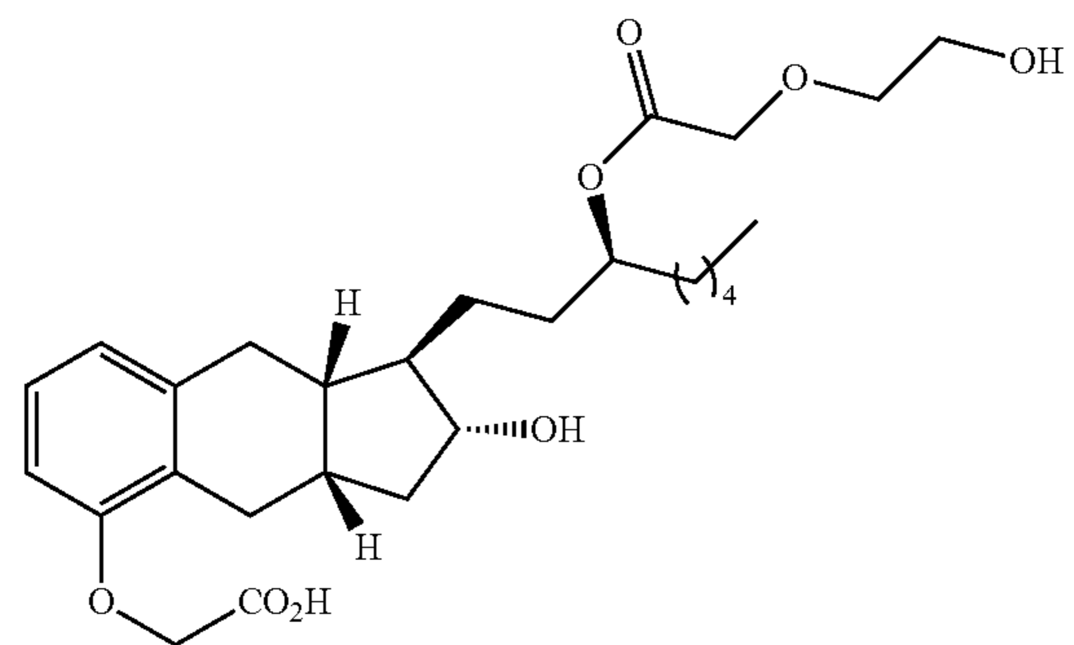
Compound Ib-20
