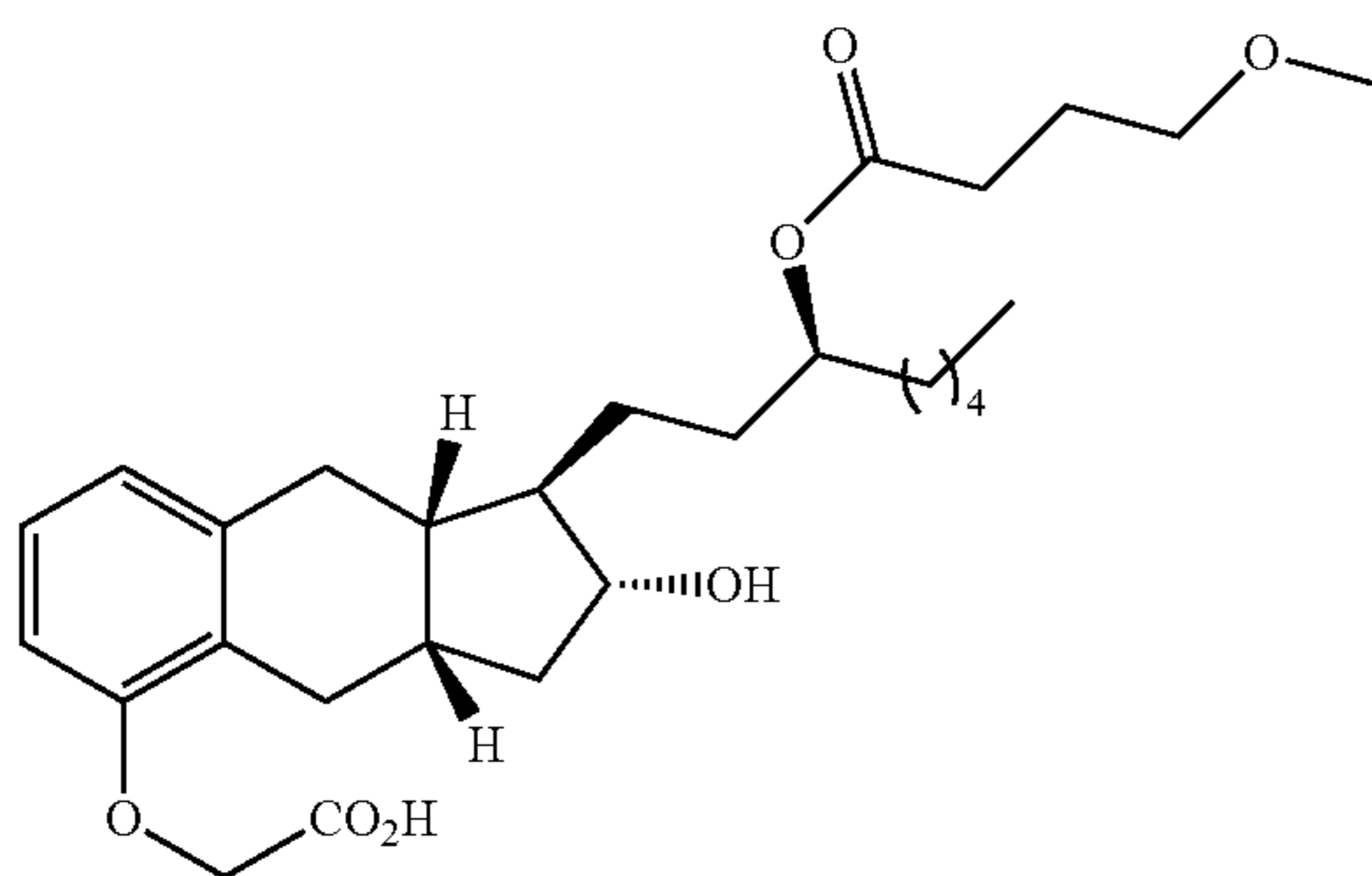
Compound Ib-19
