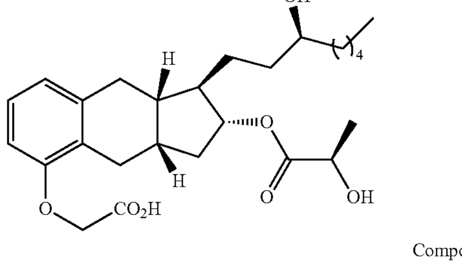
Compound Ia-23
