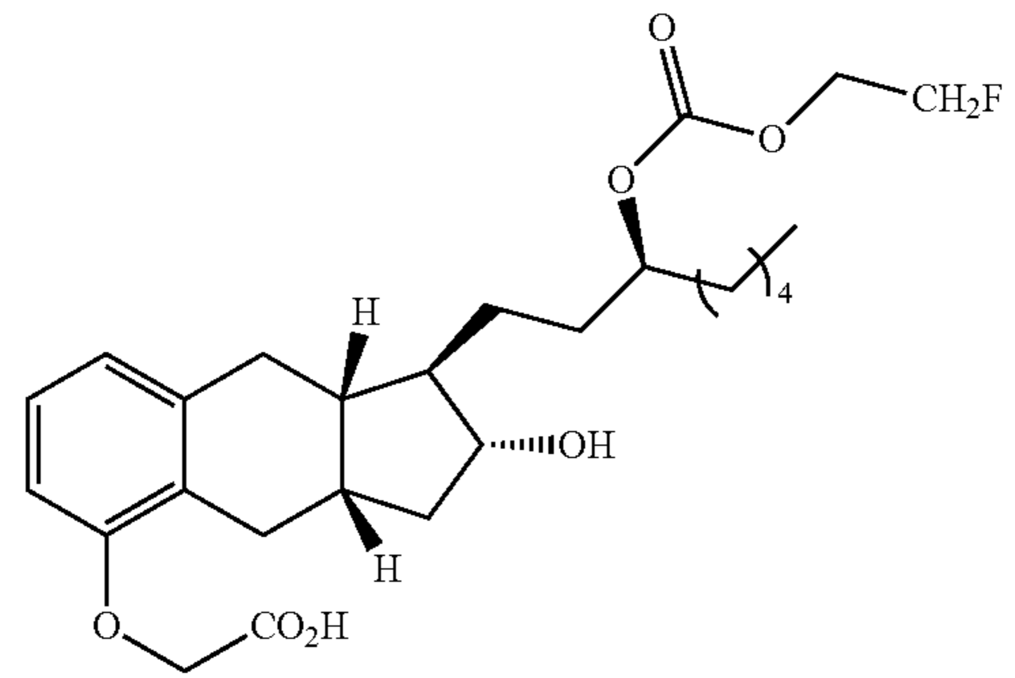
Compound Ib-12
