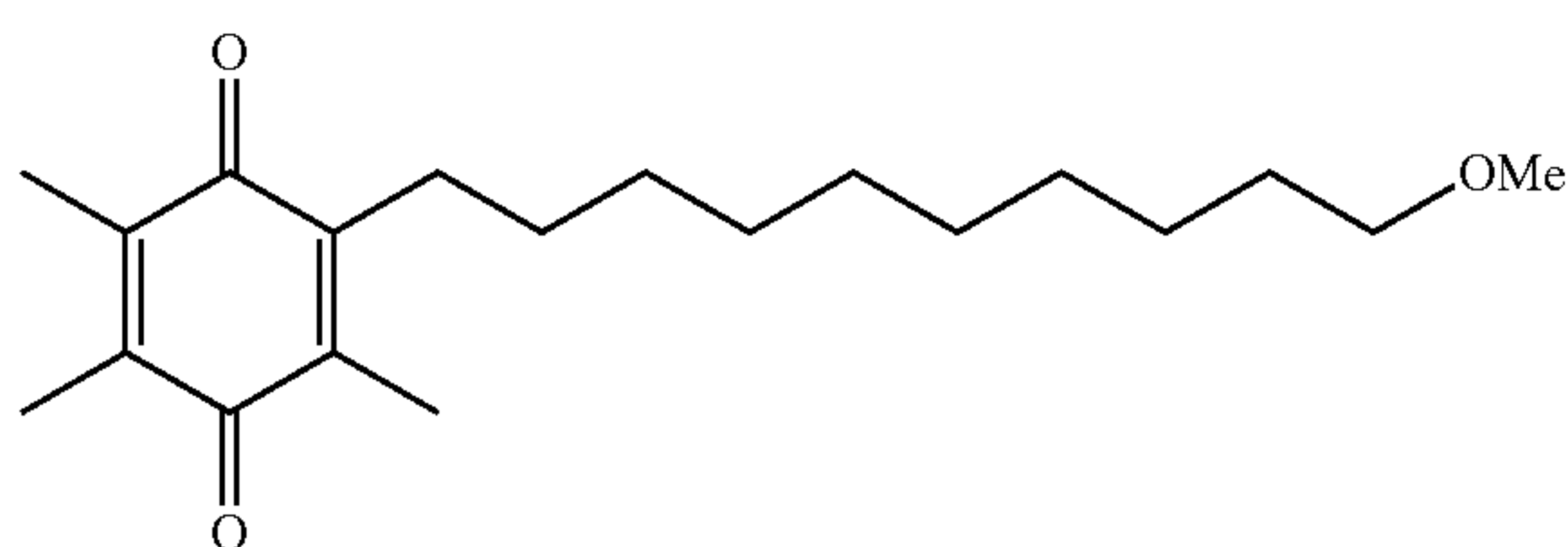
Step 1. 11-methoxyundecanoic acid (23)
