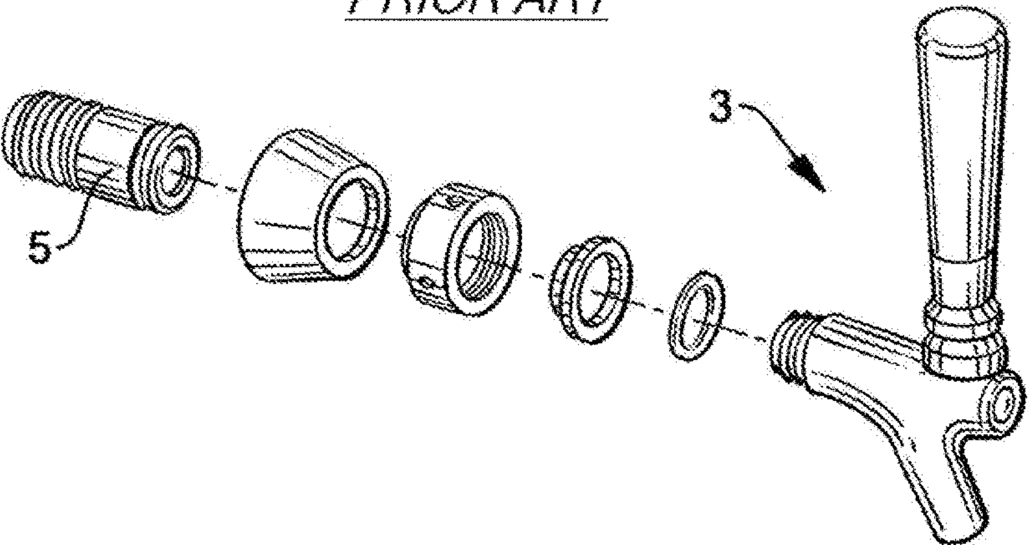
FIG. 2 PRIOR ART
