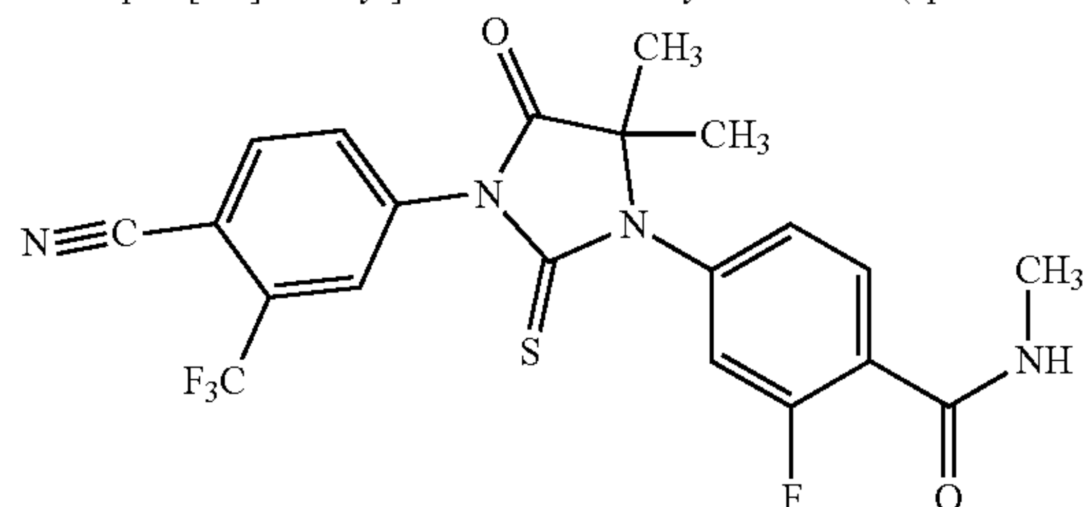
4-(3-(4-cyano-3-(trifluoromethyl)phenyl)-5,5-dimethyl-4-oxo-2-thioxoimidazolidin-1-yl)-2-fluoro-N-methylbenzamide (enzalutamide)
