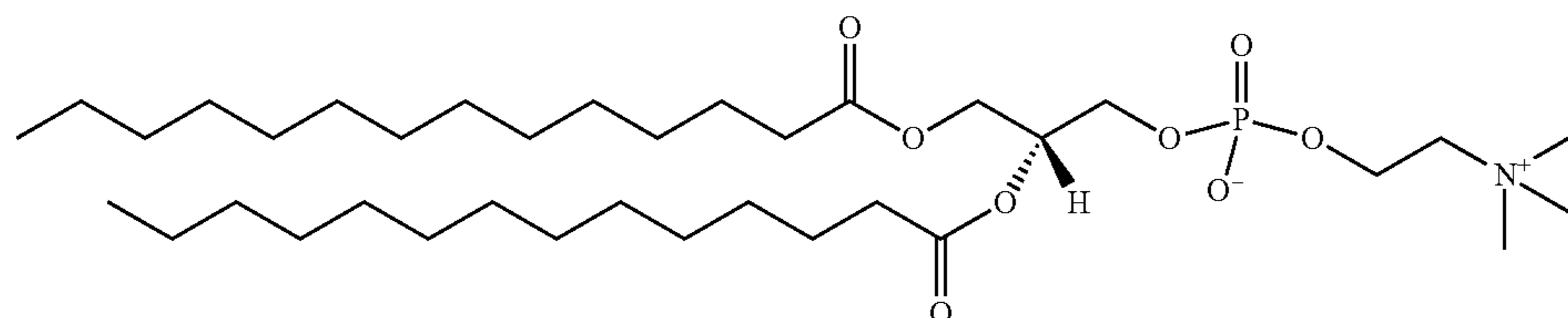
1,2-dimyristoyl-sn-glycero-3-phosphocholine (DMPC)
