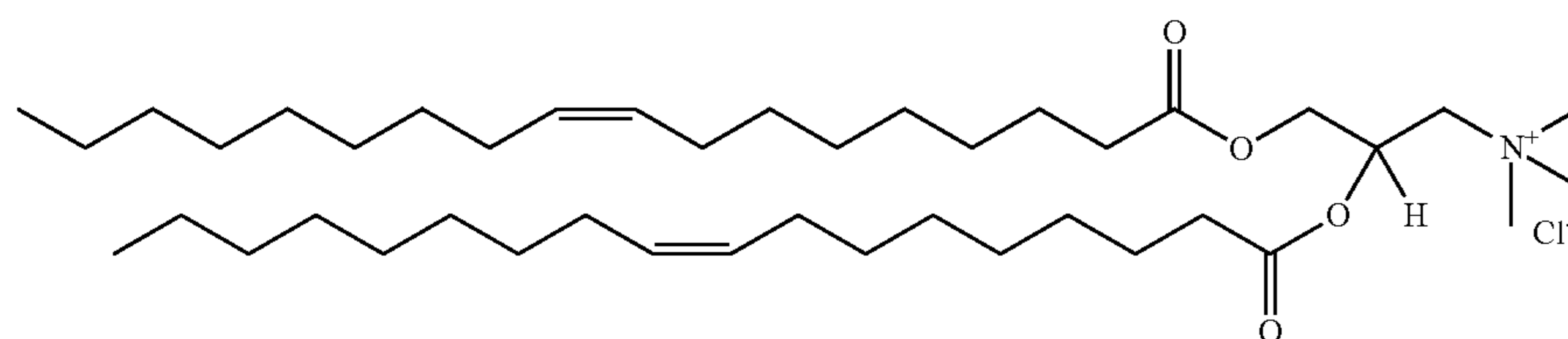
1,2-dioleoyl-3-trimethylammonium-propane (DOTAP)
