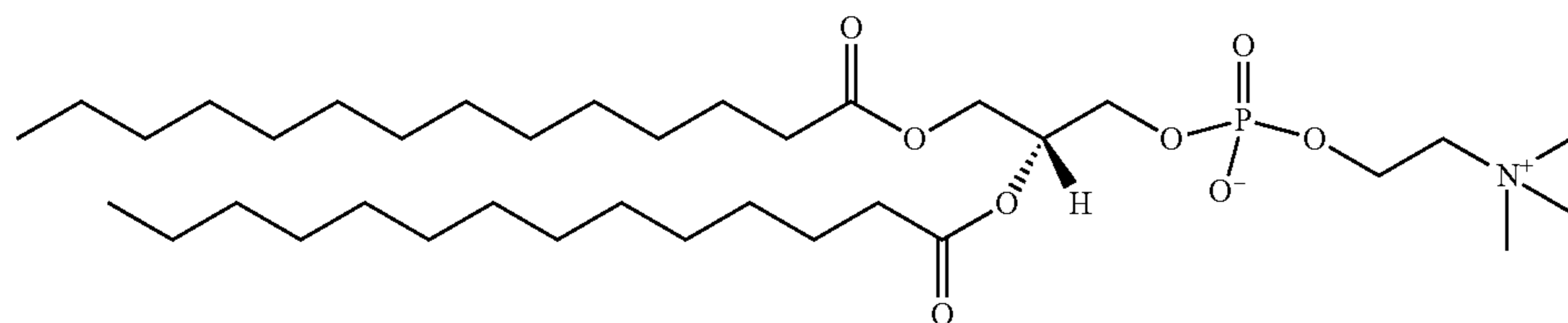
1,2-dimyristoyl-sn-glycero-3-phosphocholine (DMPC)
