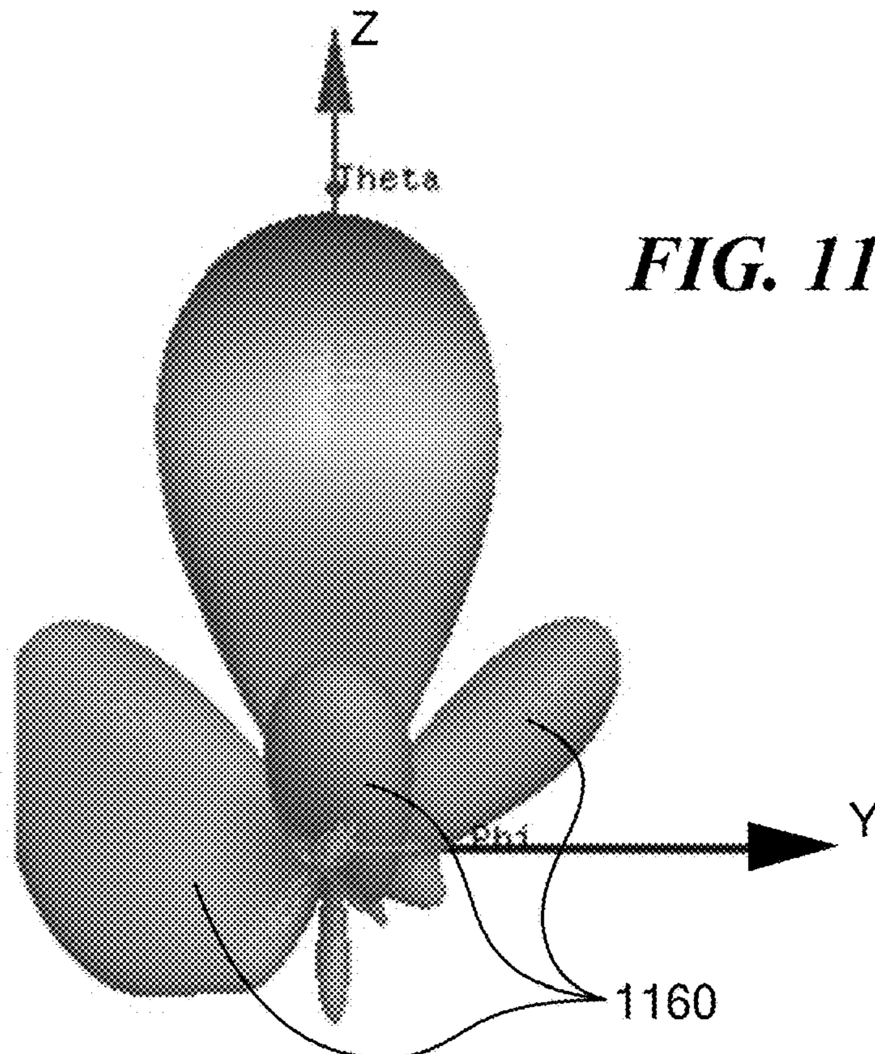
dB (RealizedGain)
