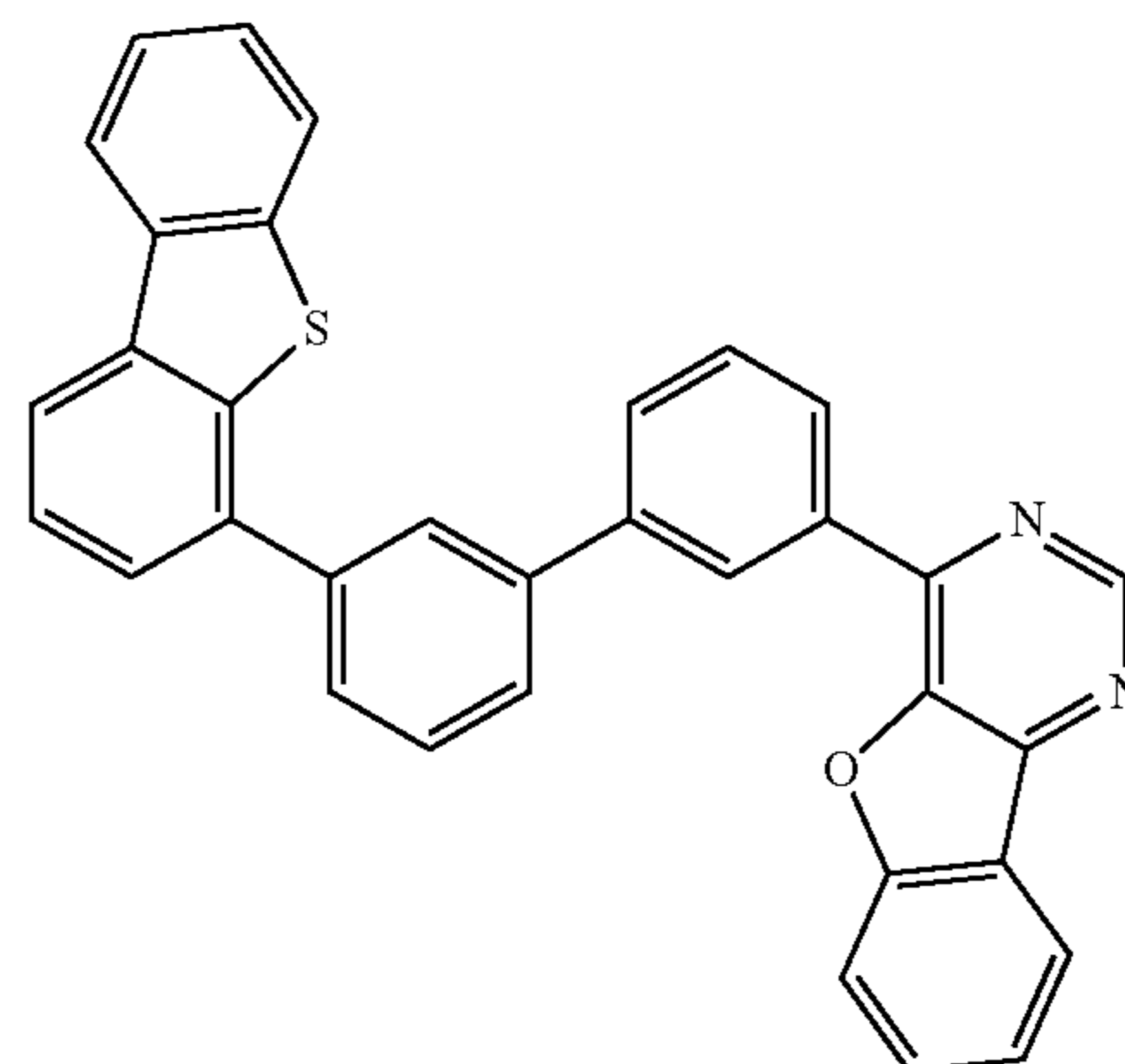
4mDBTBPBfpm-II
