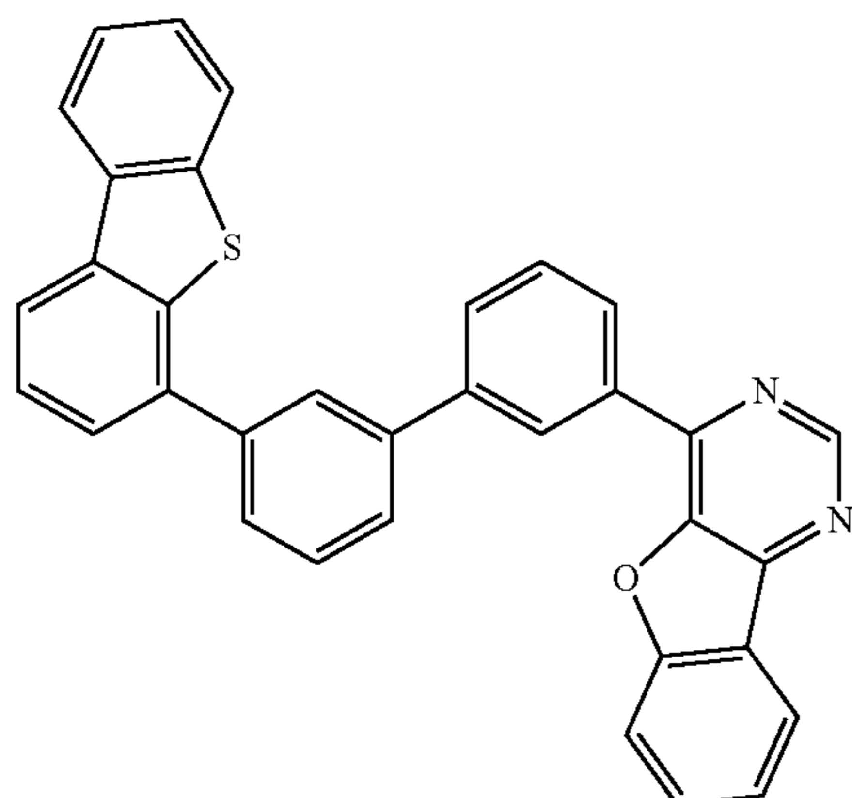
4mDBTBPBfpm-II
