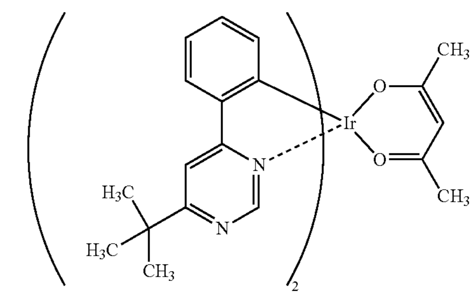
Ir(tBuppm) 2 (acac)
