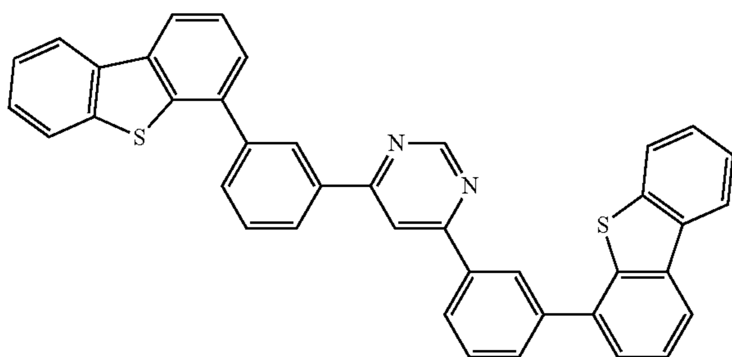
4,6DBTP2Pm-II
