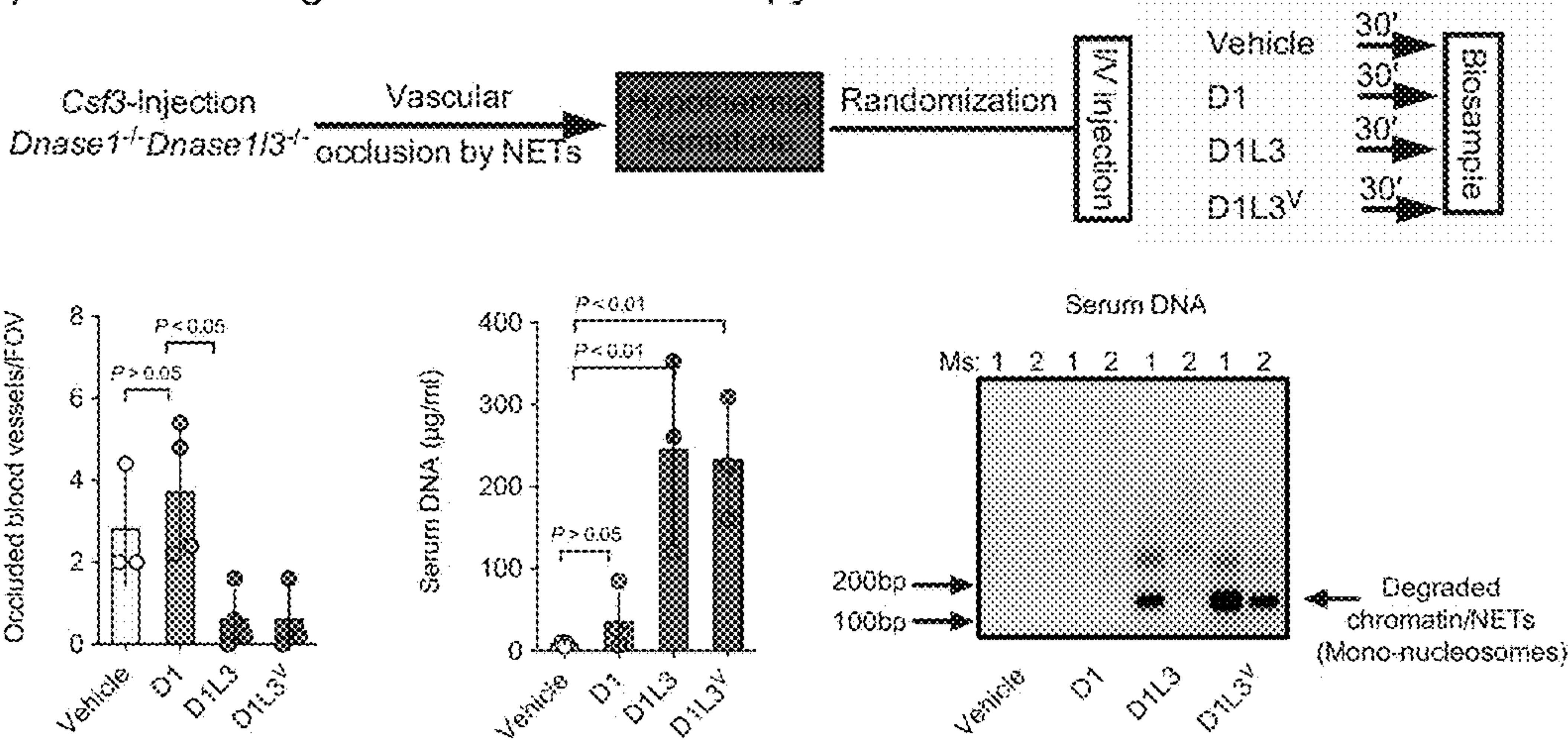
Fig. 36C Experimental design: Acute anti-NET therapy
