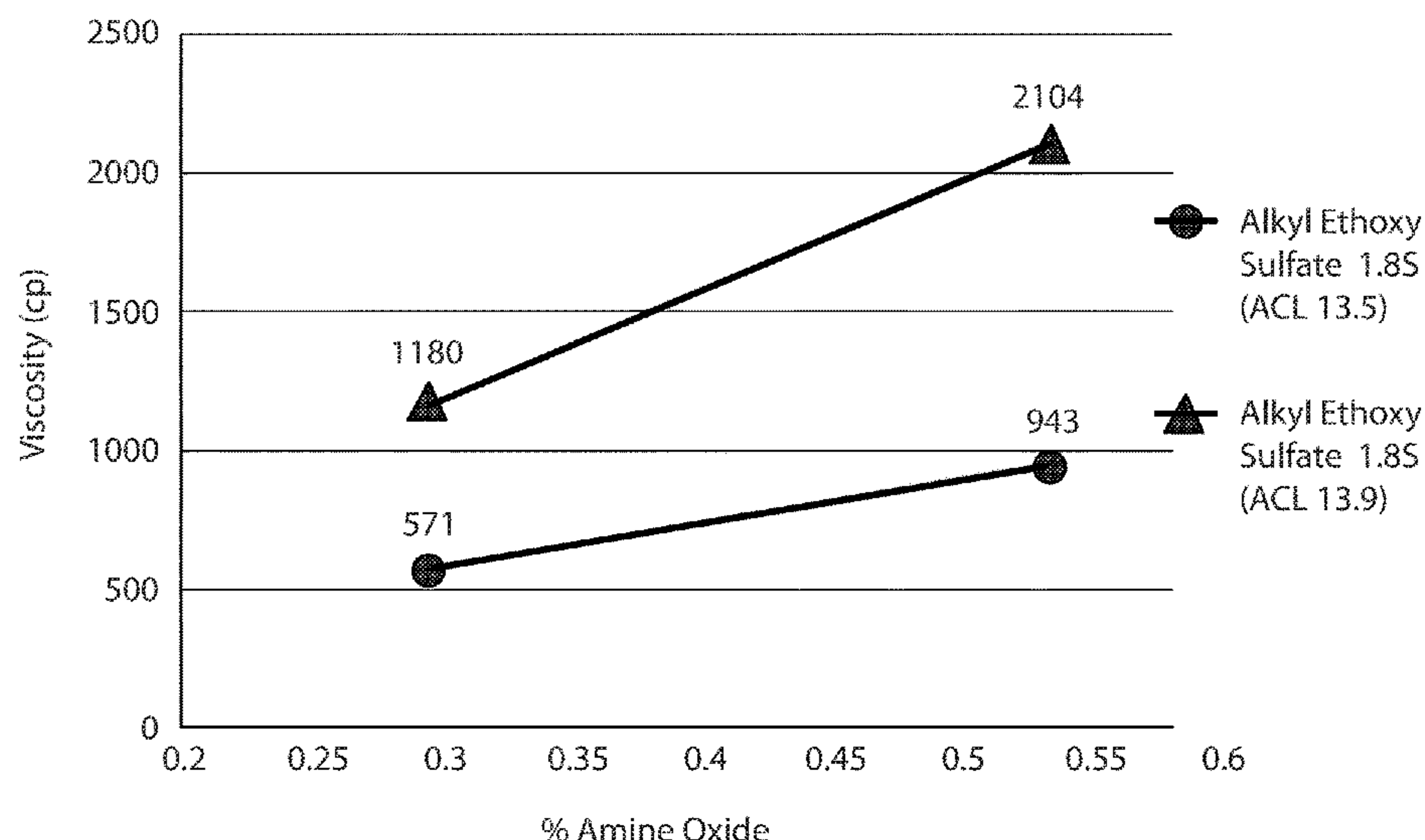
Example 4: Viscosity vs. Amine Oxide Level
