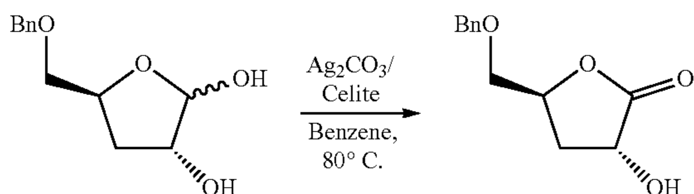
(3R,5S)-5-(benzyloxymethyl)-3-hydroxy-dihydrofuran-2(3H)-one
