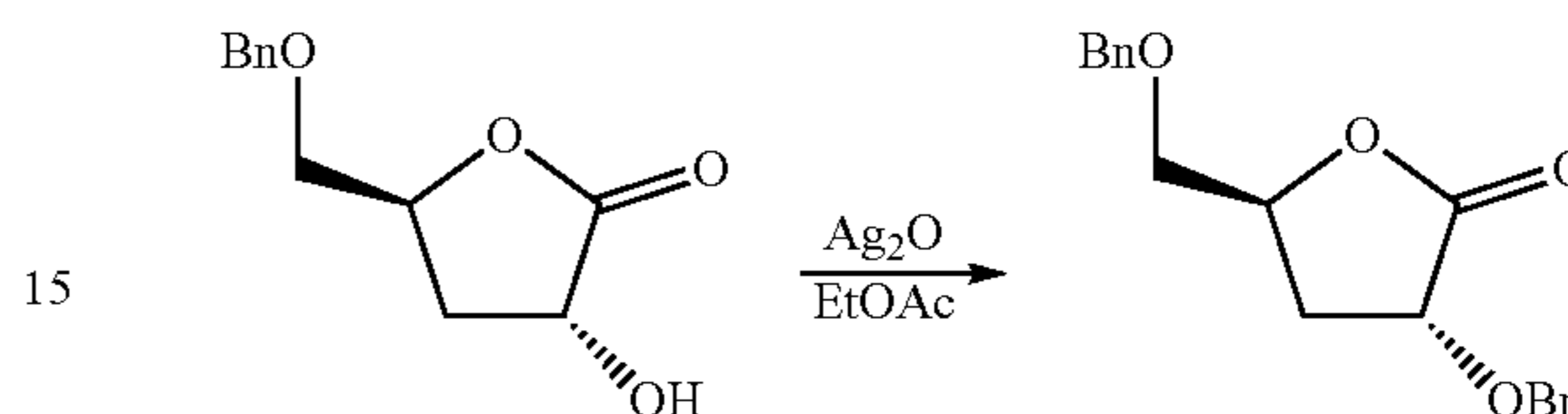
(3R, 5S)-3-(benzyloxy)-5-(benzyloxymethyl)-dihydrofuran-2(3H)-one
