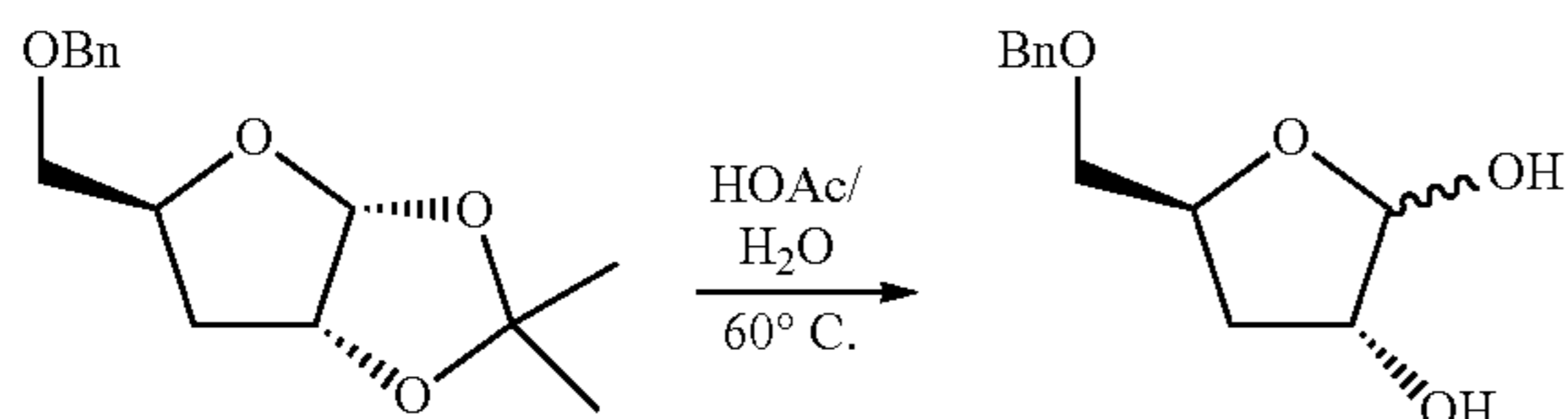
(3R,5S)-5-(benzyloxymethyl)-tetrahydrofuran-2,3-diol
