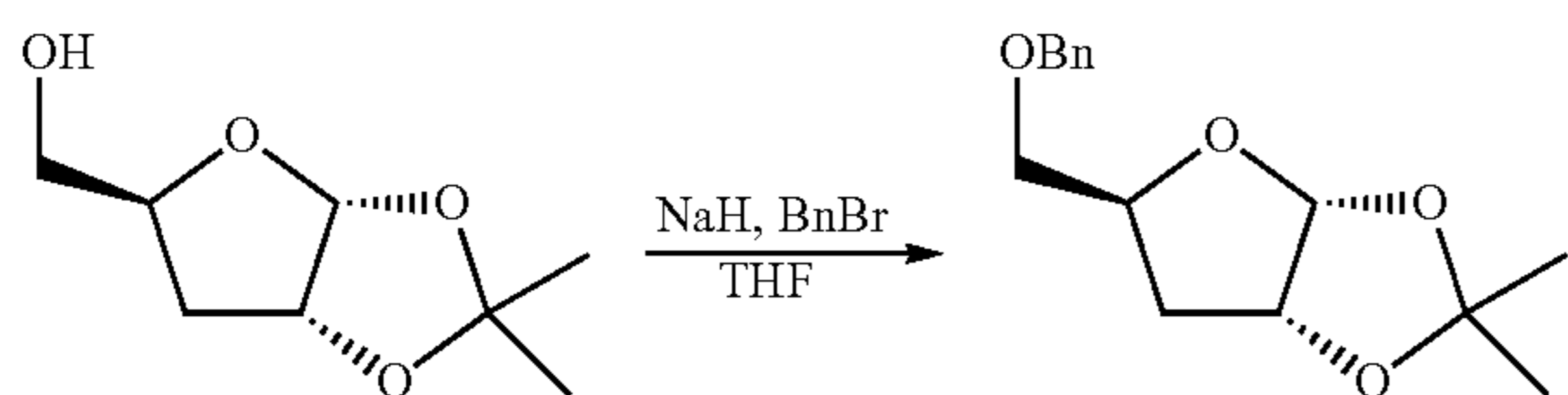
(3 \alpha R,5S,6 \alpha R)-5-(benzyloxymethyl)-2,2-dimethyl-tetrahydrofuro[2,3-d][1,3]dioxole
