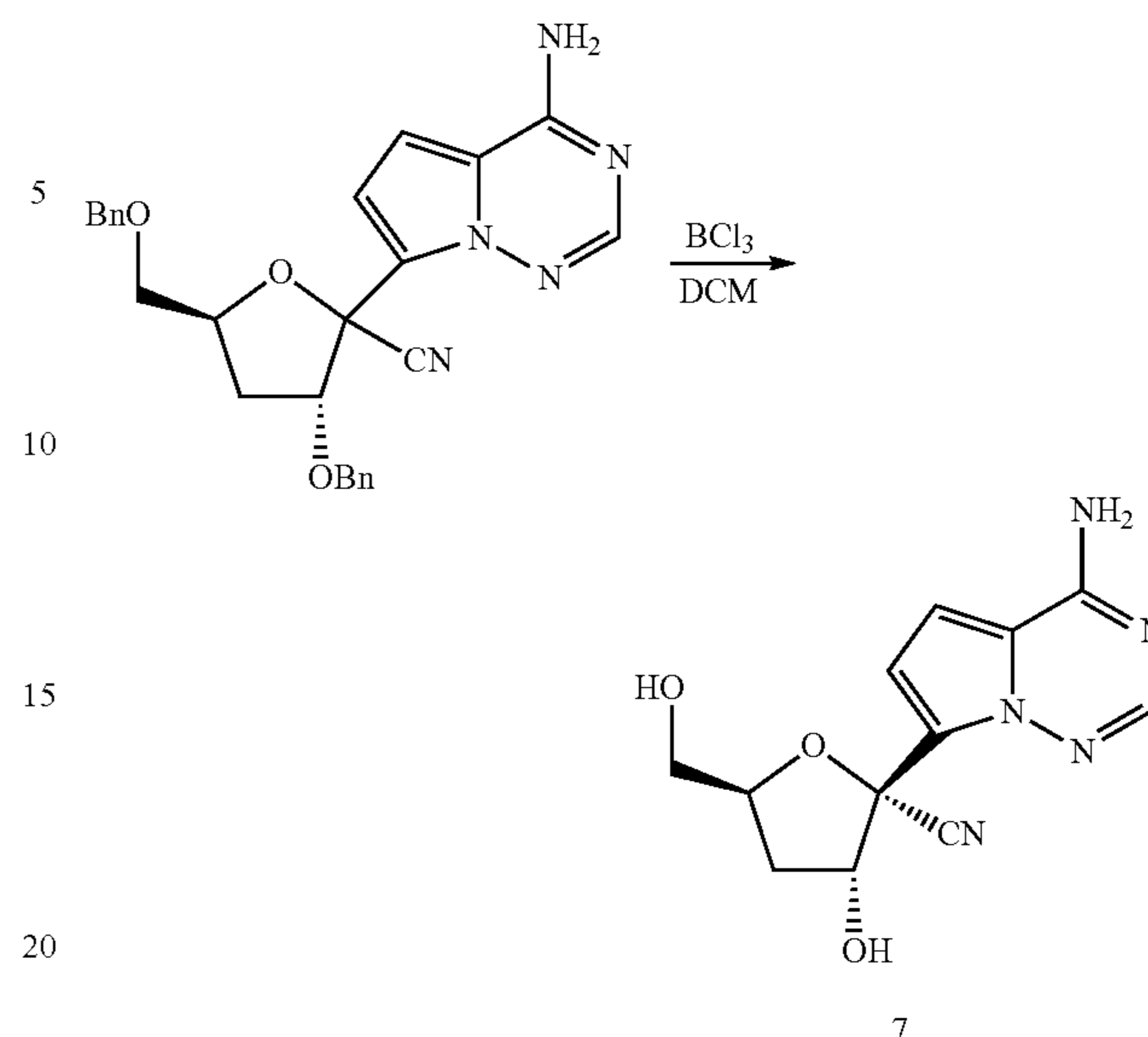
(2R,3R,5S)-2-(4-aminopyrrolo[1,2-f][1,2,4]triazin-7-yl)-3-hydroxy-5-(hydroxymethyl)-tetrahydrofuran-2-carbonitrile (7)
