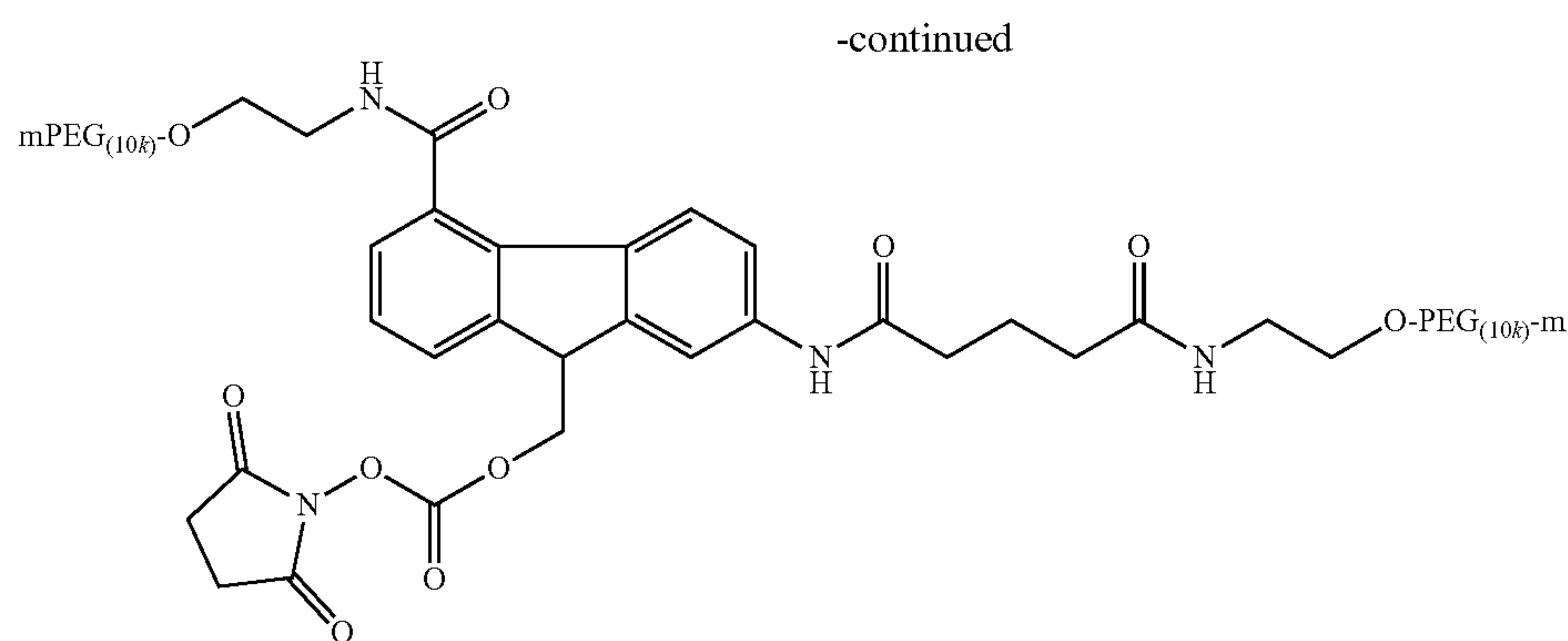
9-hydroxymethyl-4- (mPEG(10,000)-carboxyamide)-7-(mPEG(10,000)-amidoglutamic acid)fluorene-N-hydroxysuccinimide
