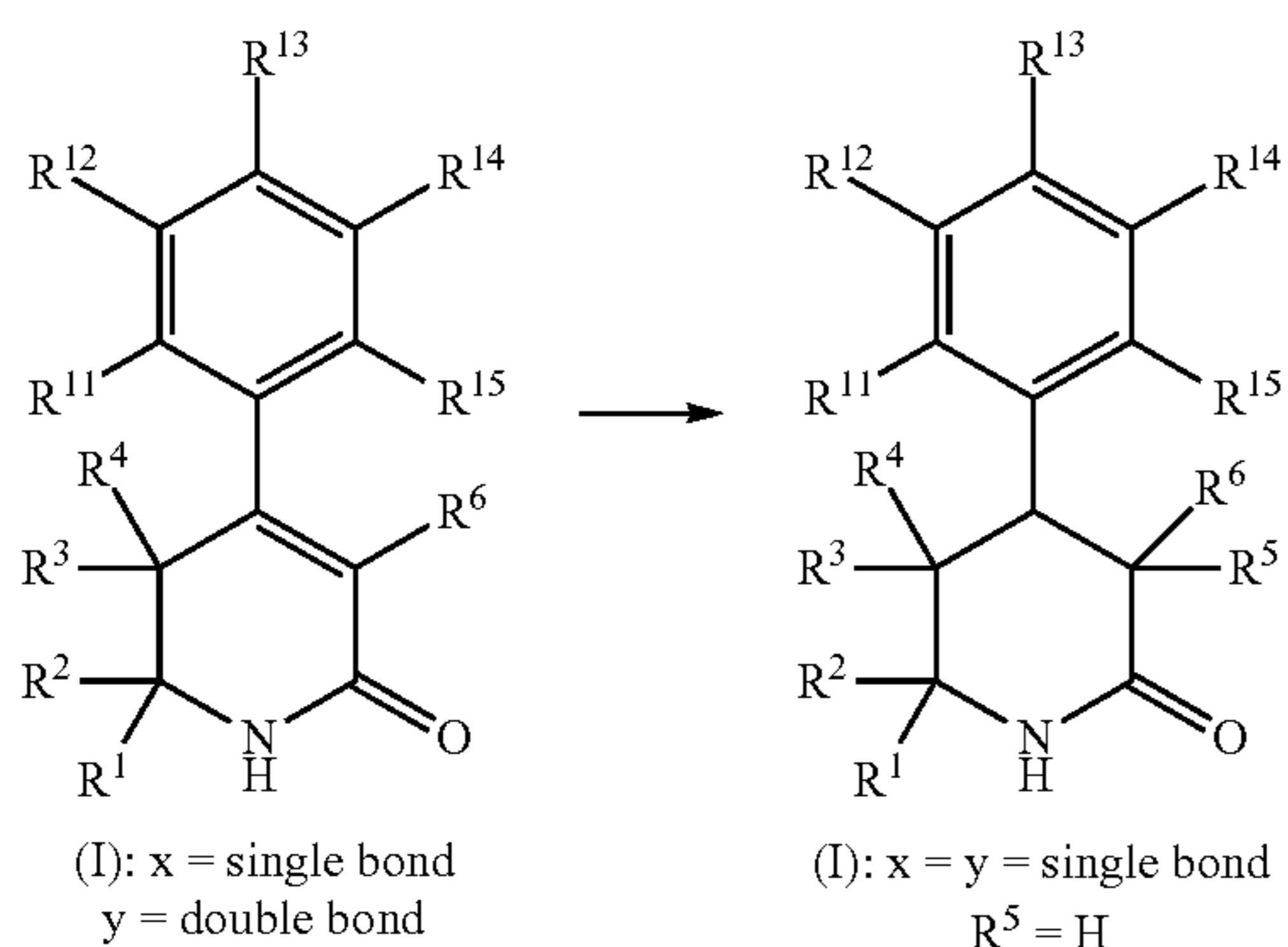
Scheme 11
