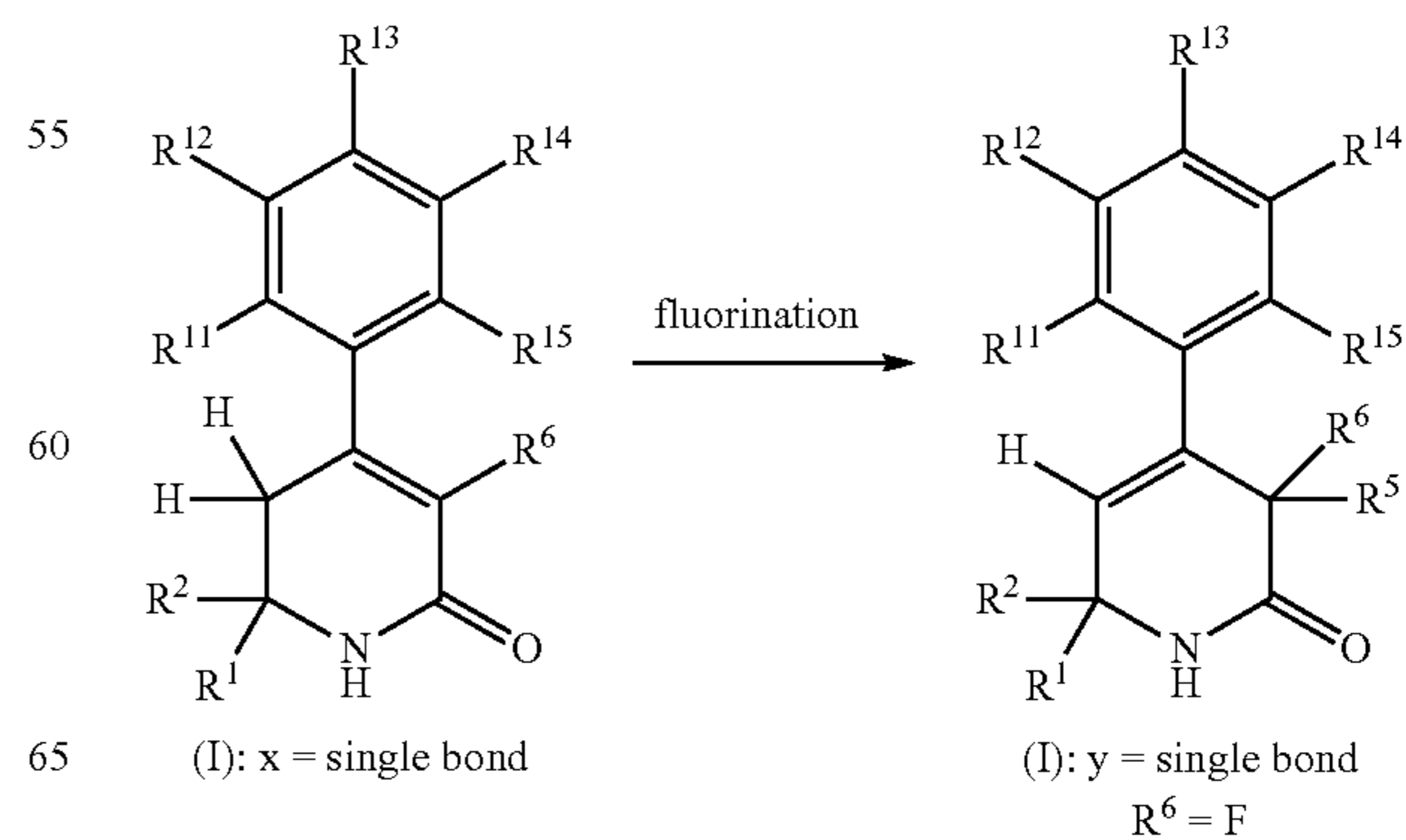
Scheme 10
