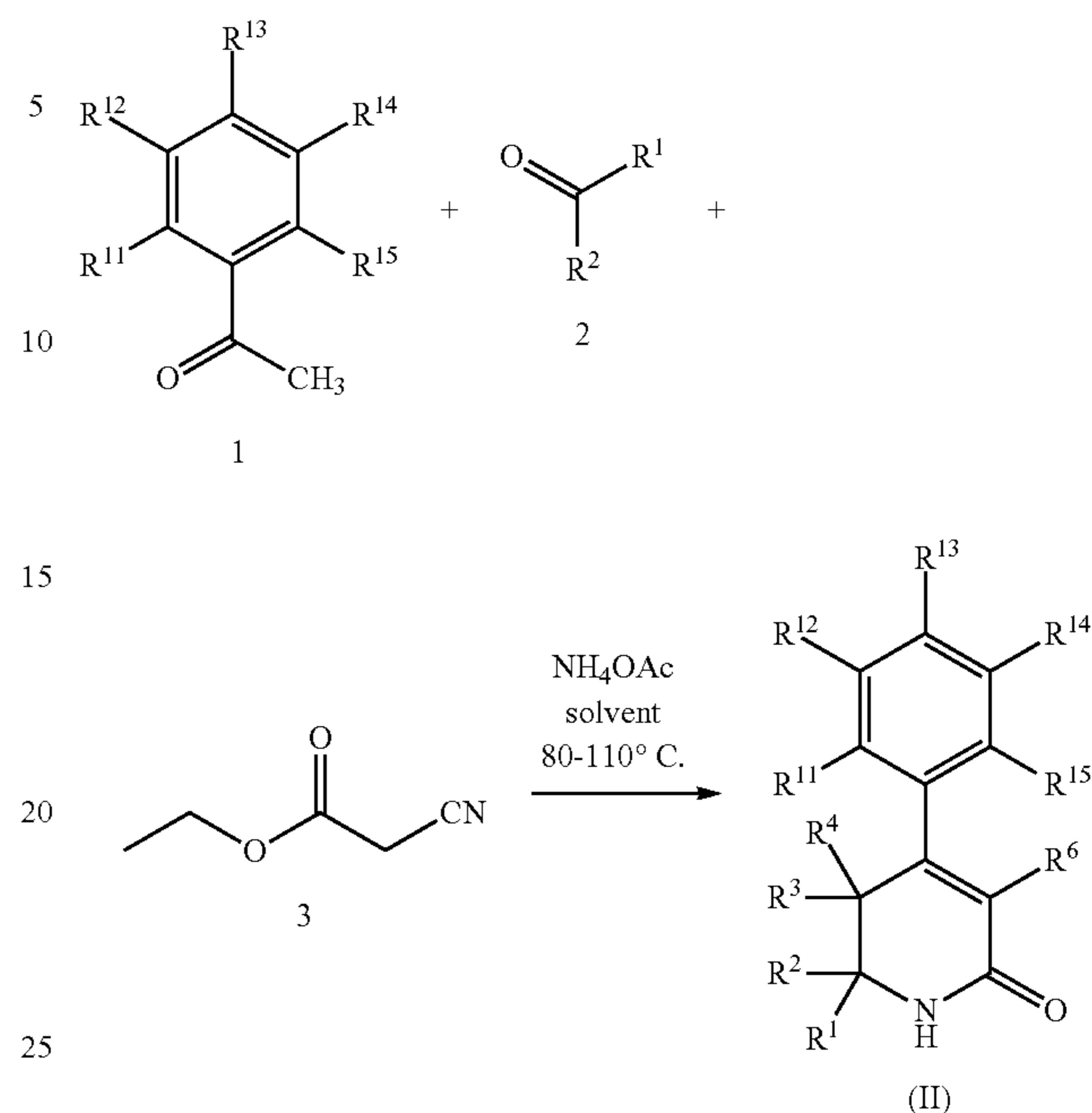
Scheme 1
