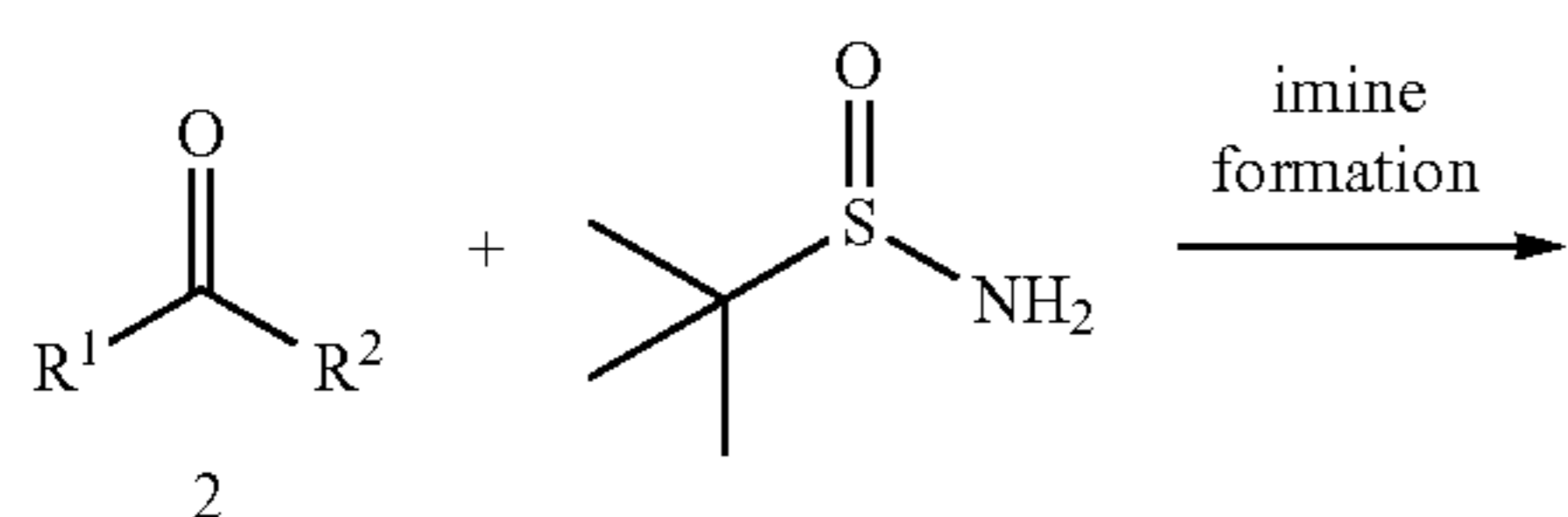
Scheme 12
