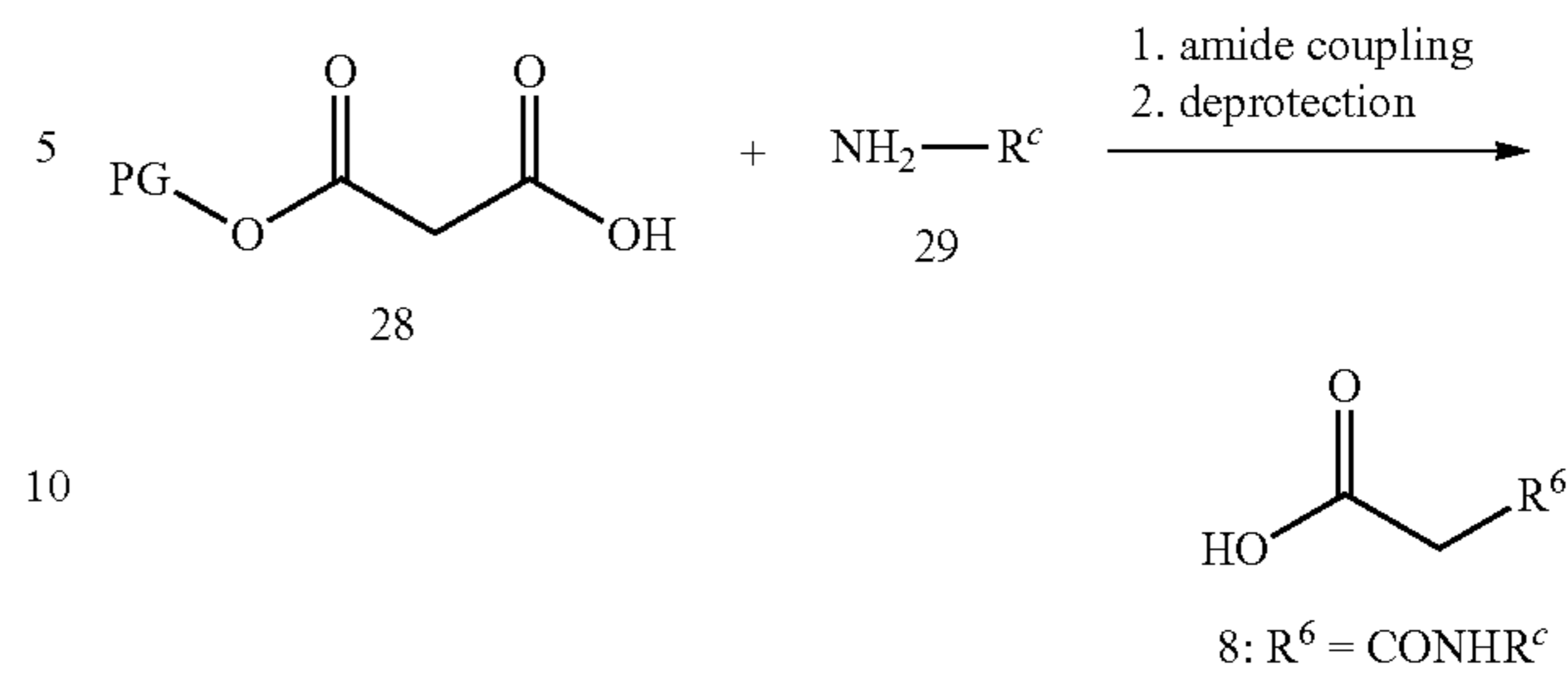
Scheme 8
