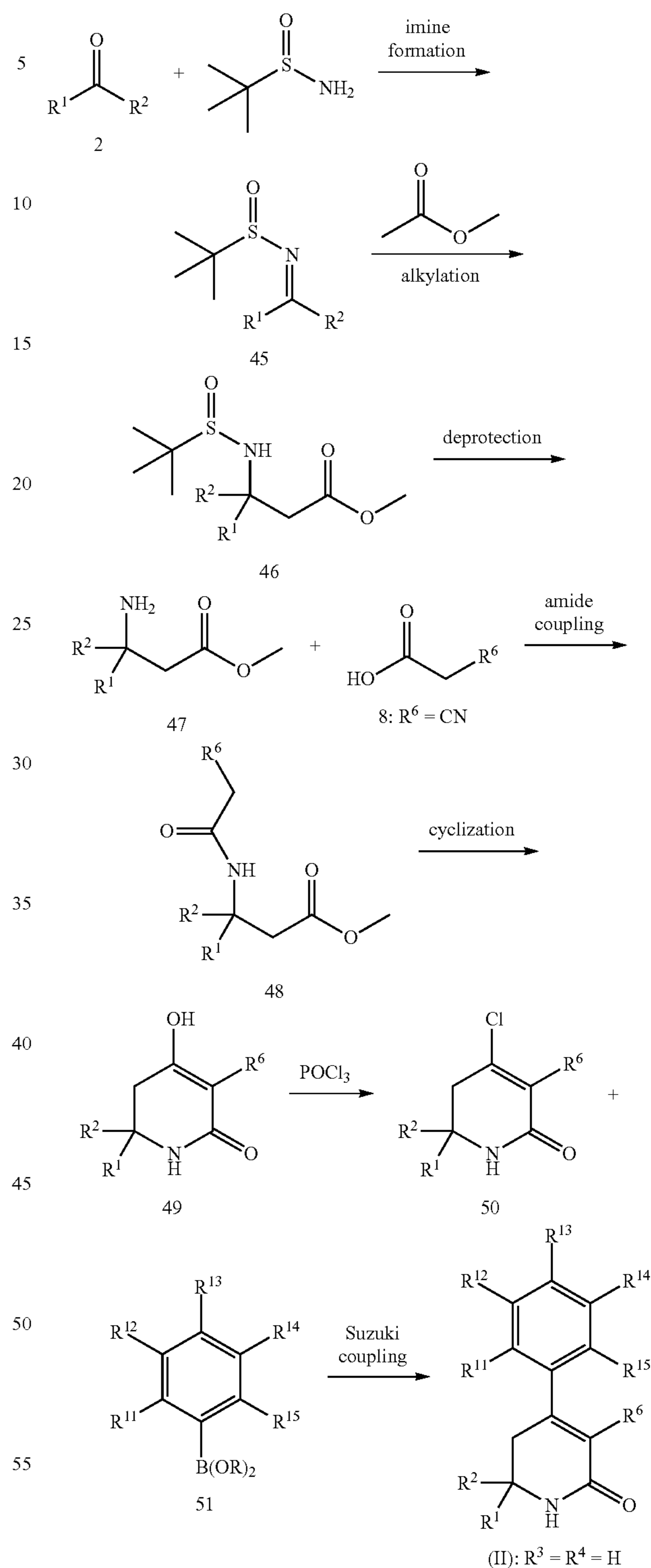
Scheme 13
