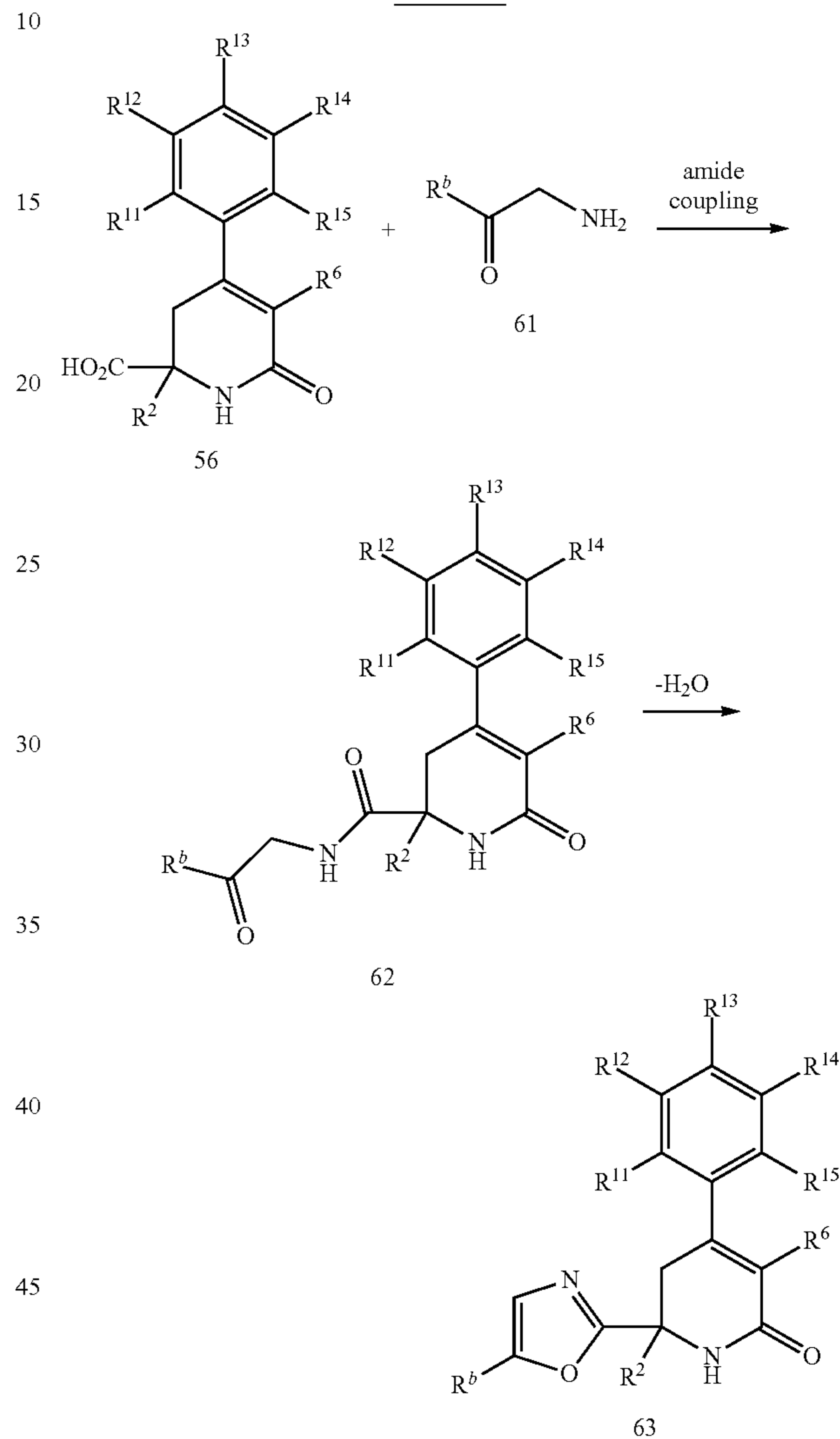
Scheme 16
