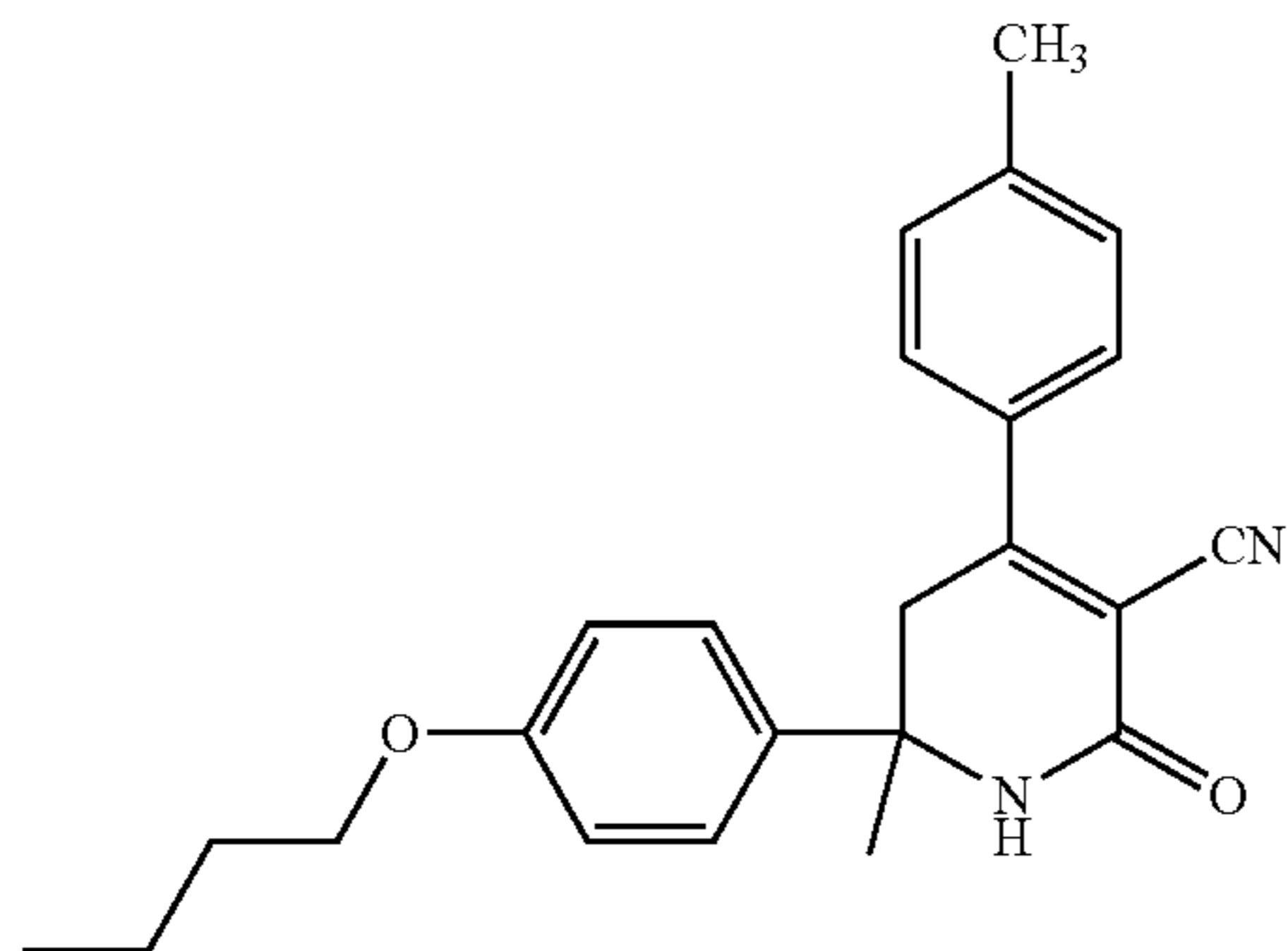
Intermediate 107A. (Z)-N-(1-(4-Butoxyphenyl)ethylidene)-2-methylpropane-2-sulfinamide
