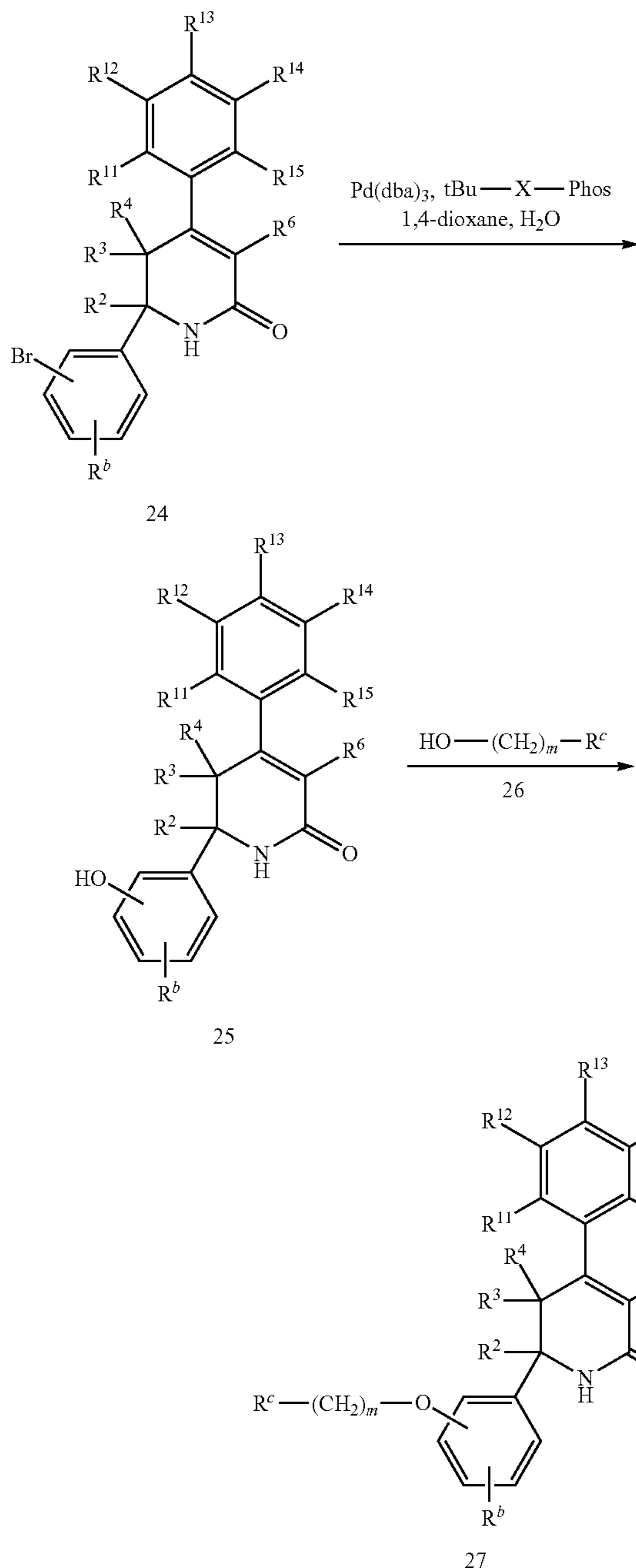
Scheme 7
