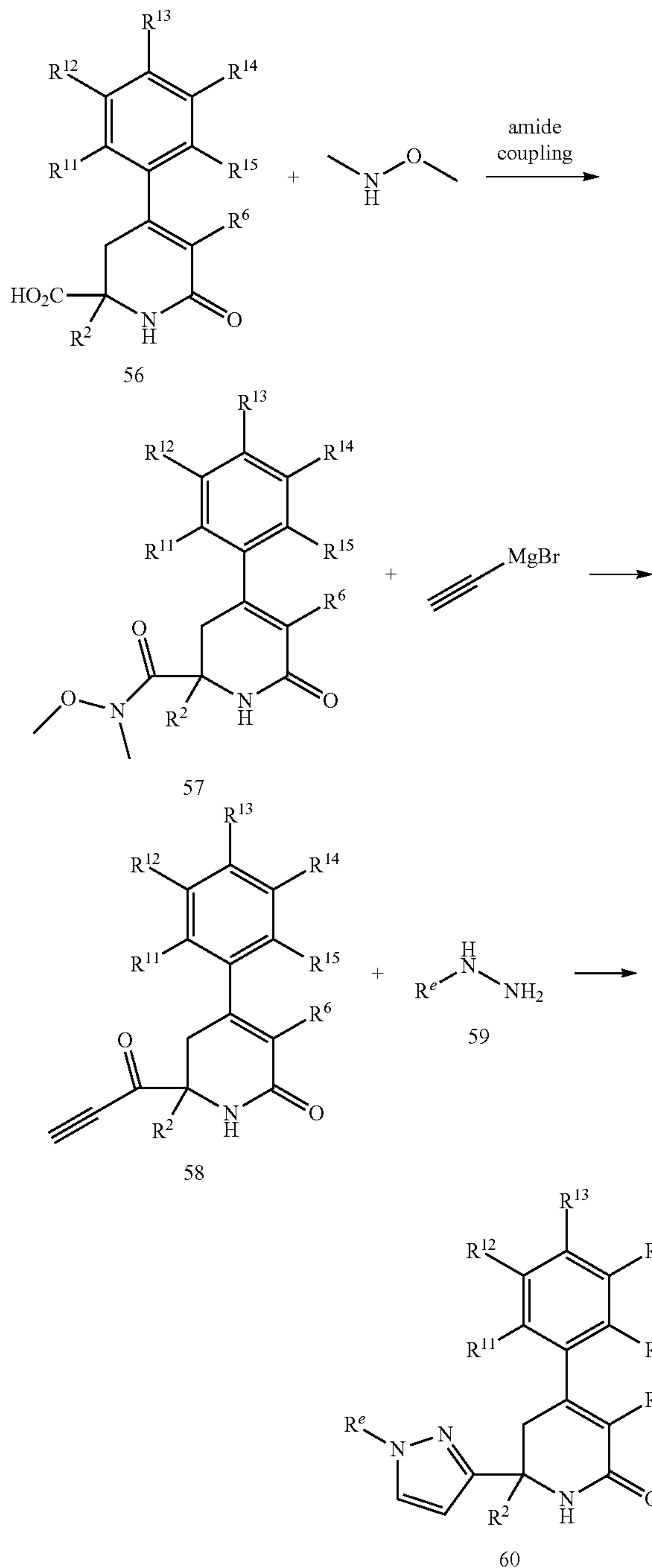
Scheme 15
