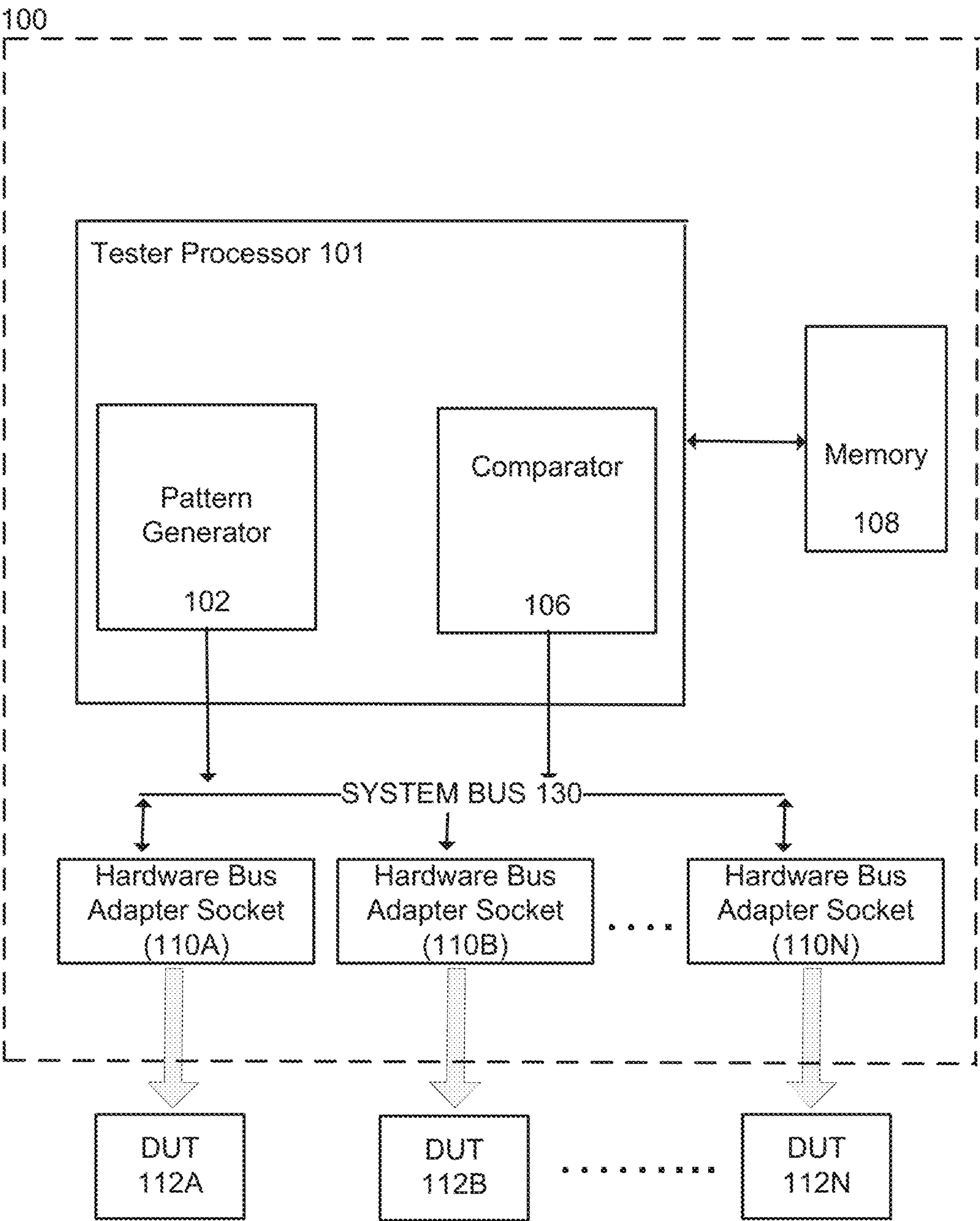
Figure 1 (PRIOR ART)
