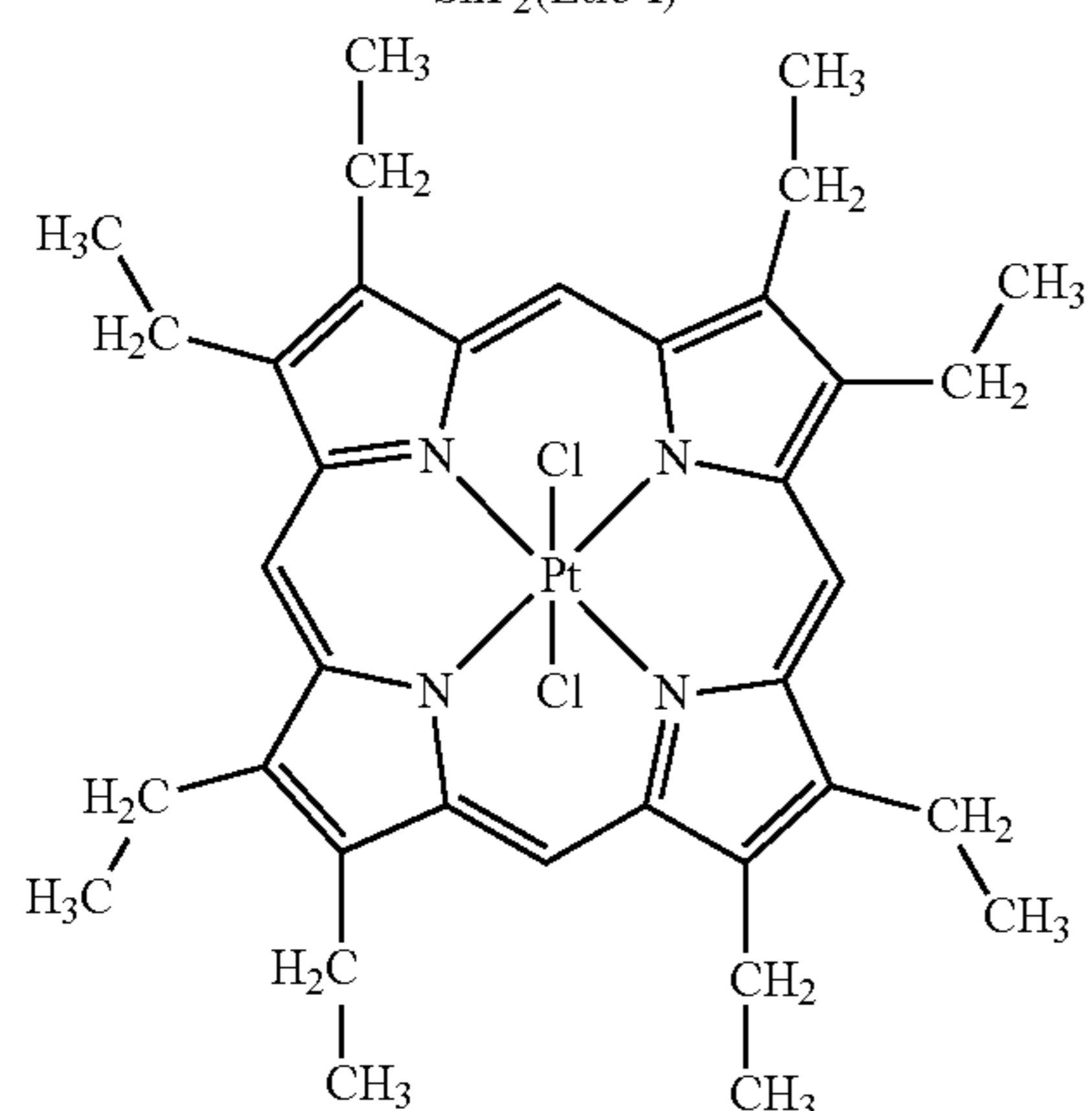
PtCl 2 OEP
