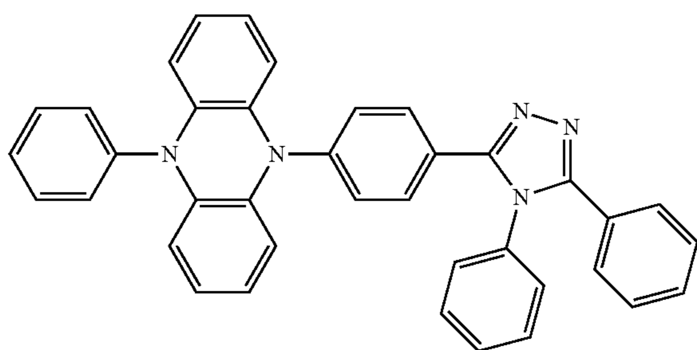
PPZ-3TPT
