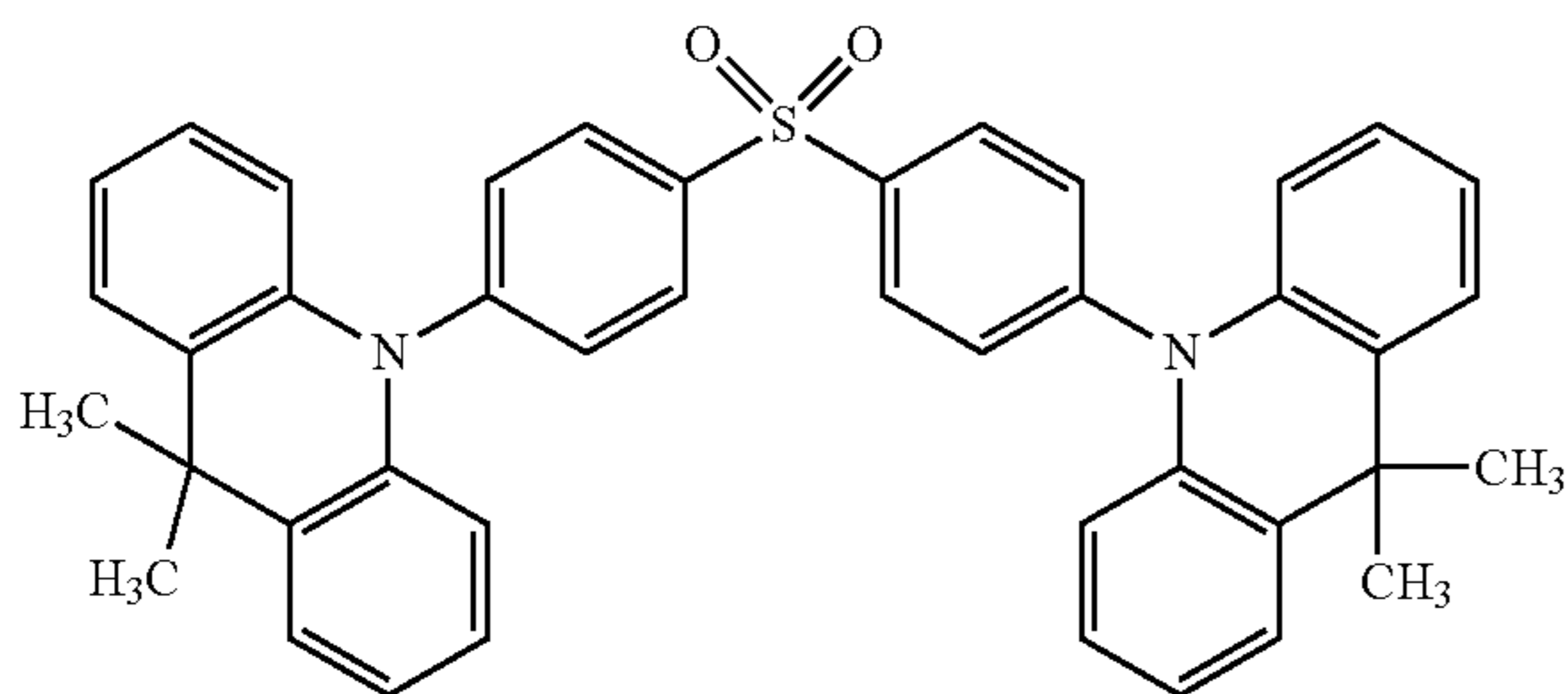
DMAC-DPS
