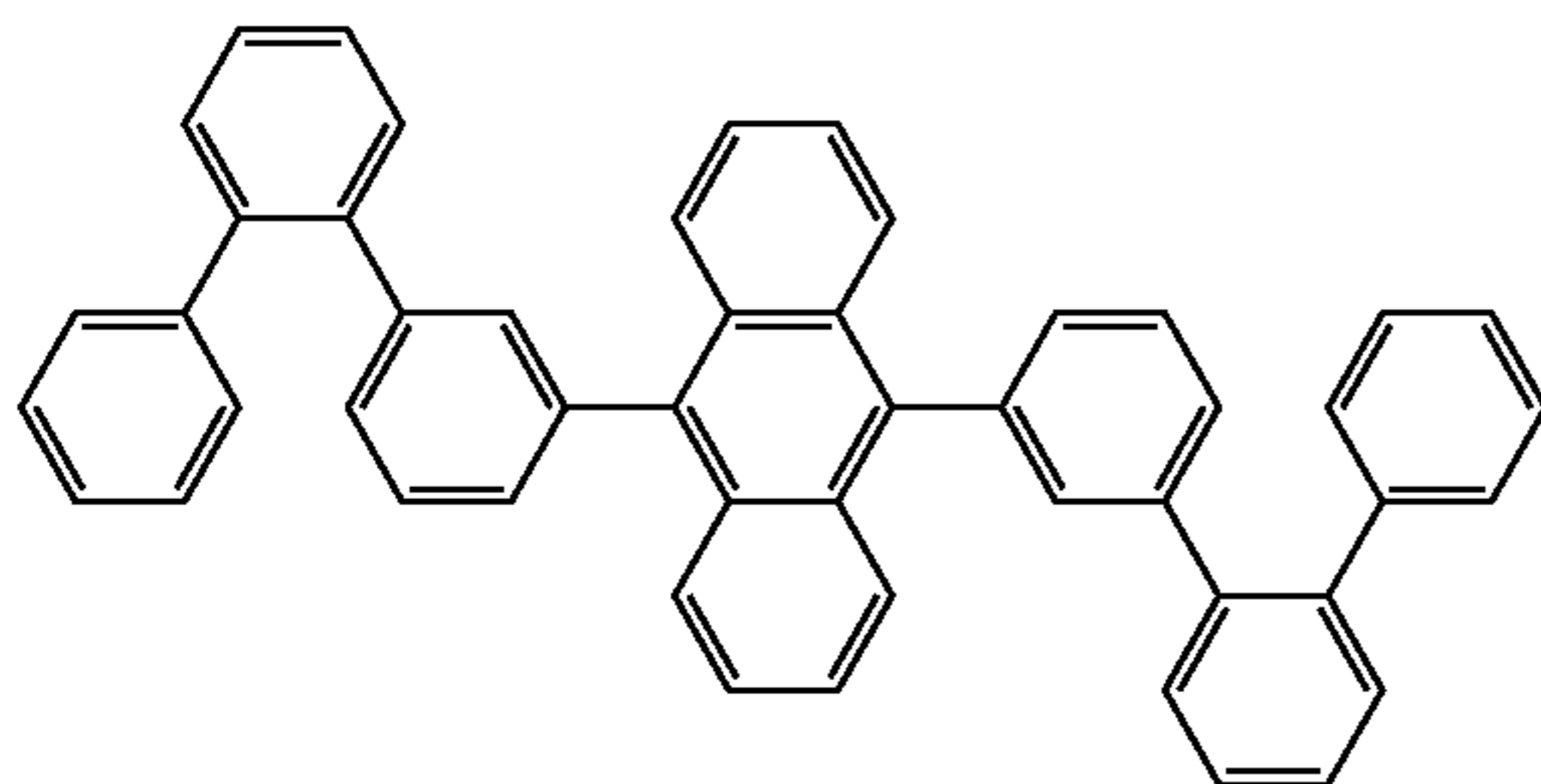
[Chemical Formula 128]
