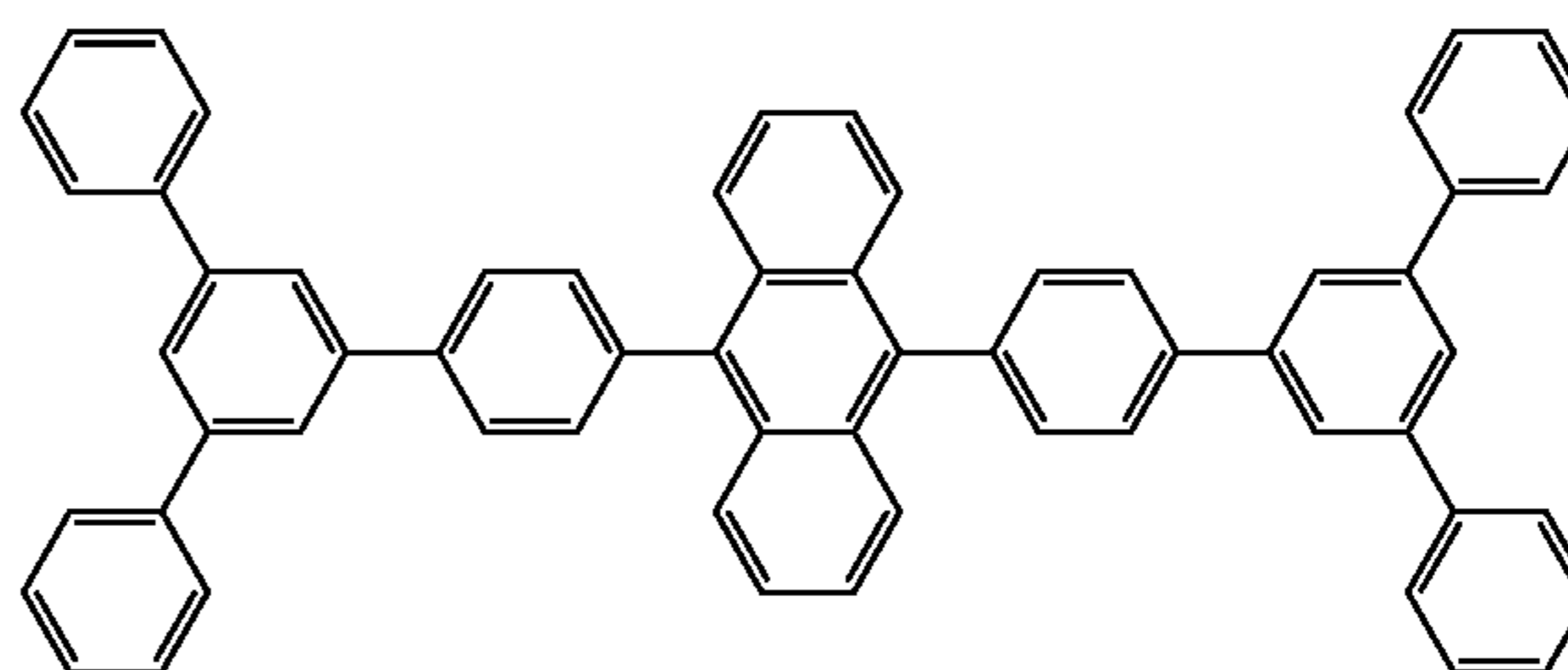
[Chemical Formula 117]
