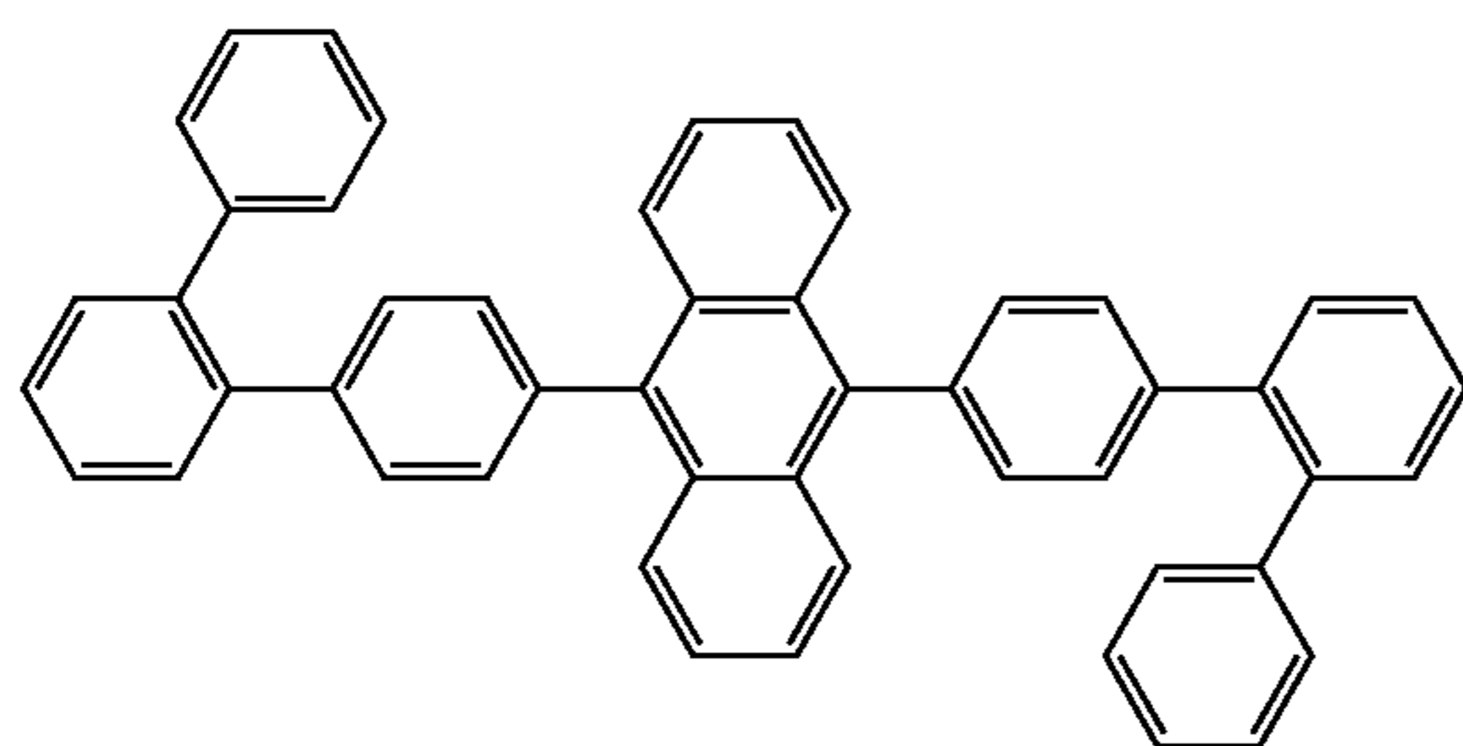
[Chemical Formula 101]
