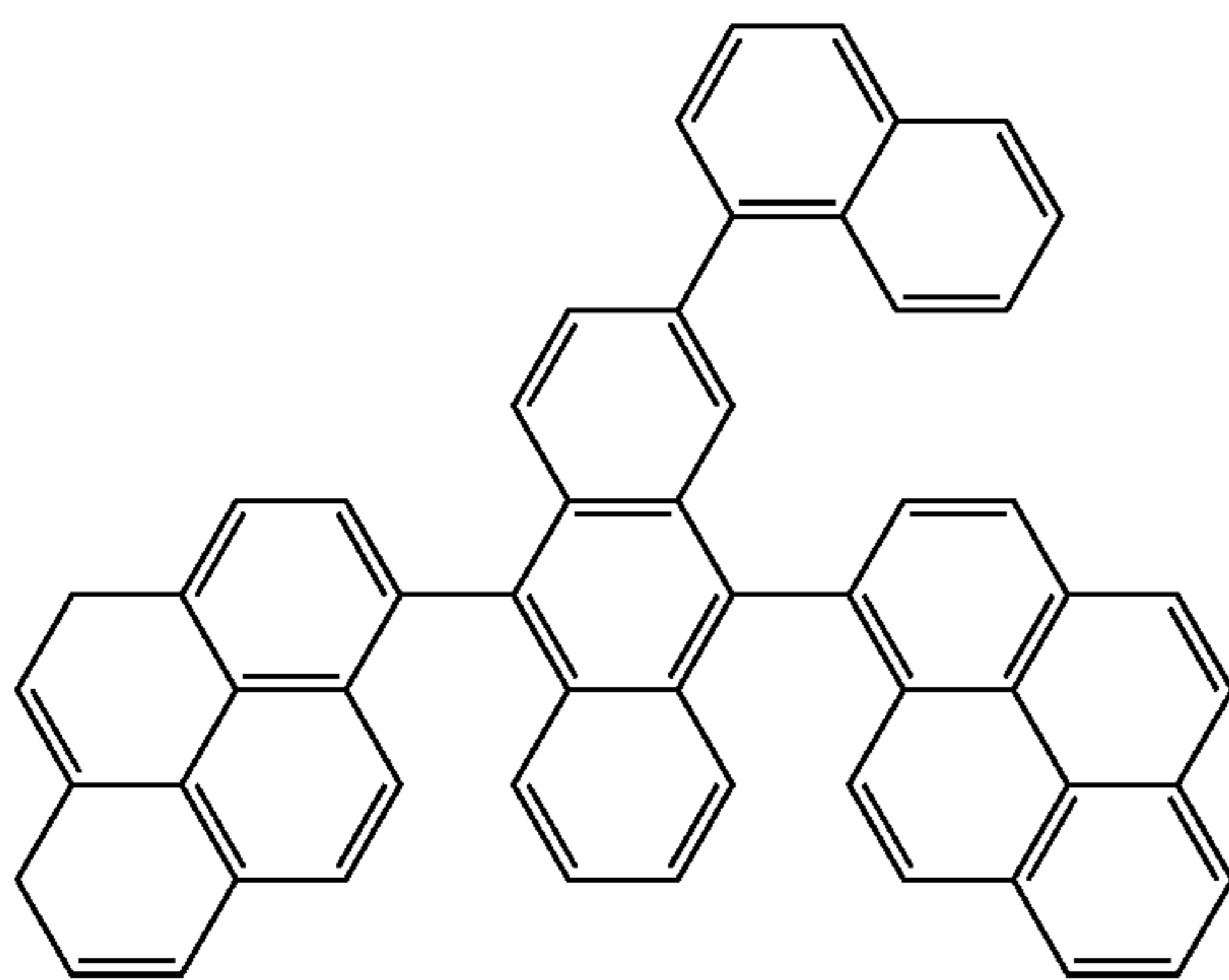
[Chemical Formula 278]
