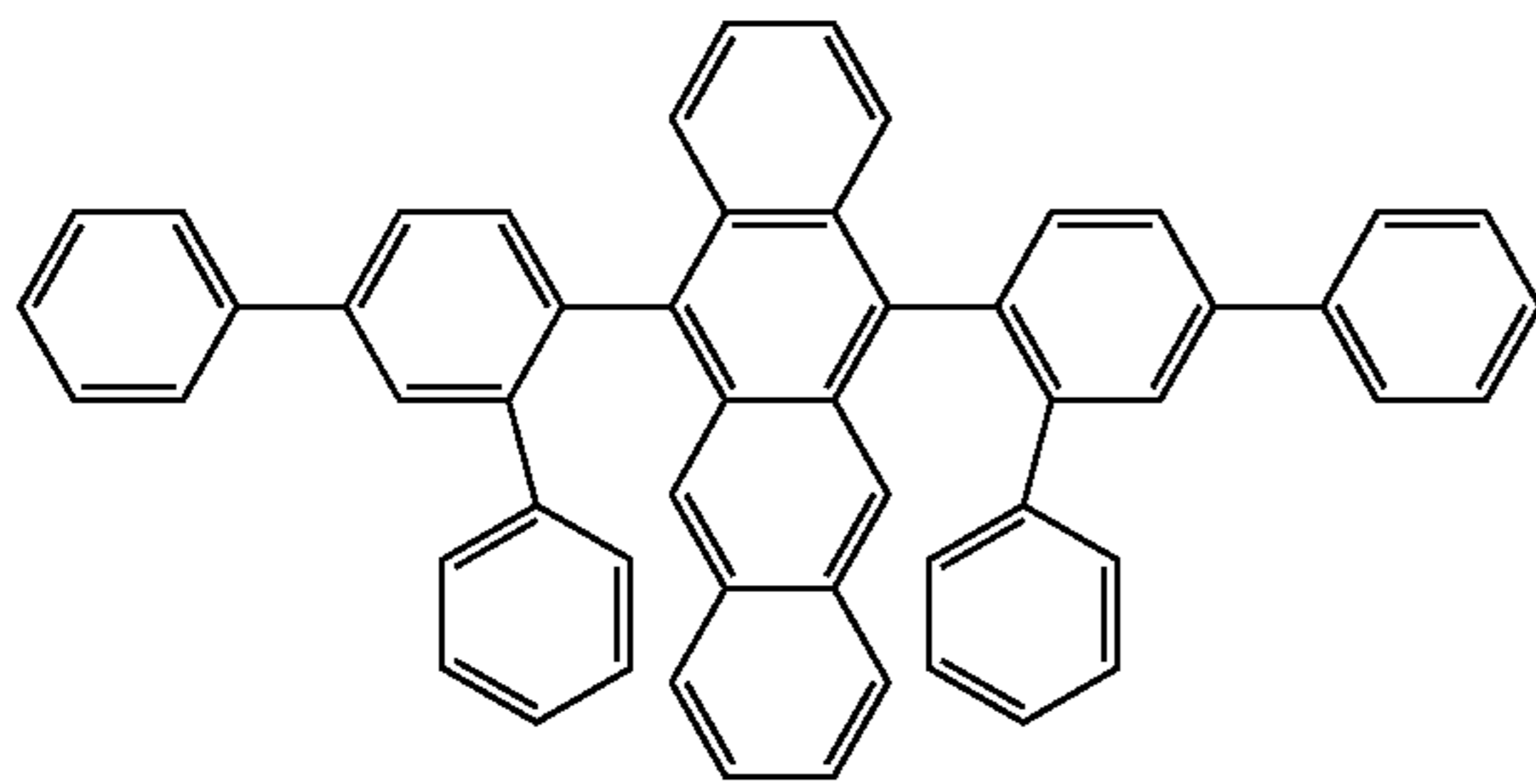
[Chemical Formula 126]
