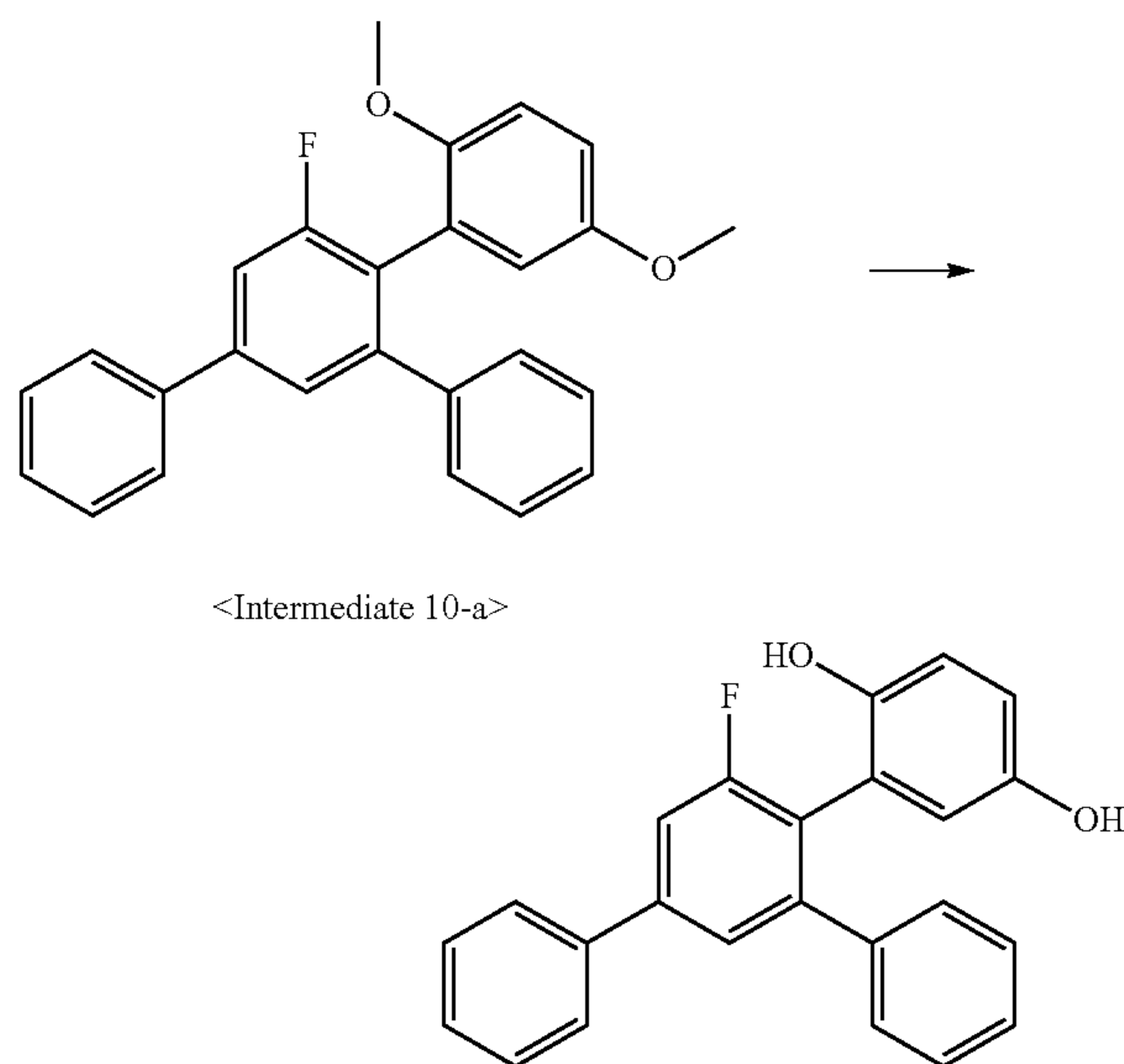
&lt;Reaction Scheme 58&gt;
