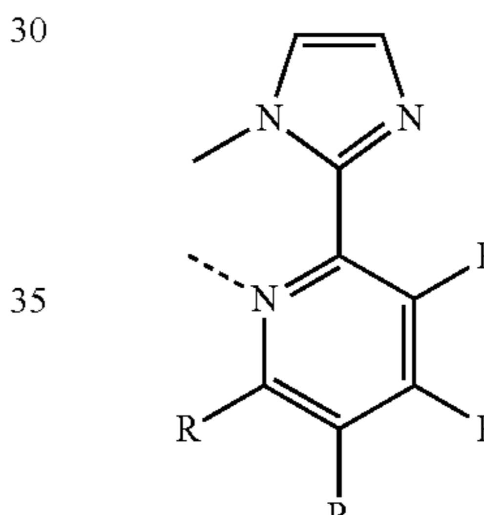
[Structural Formula C19]
