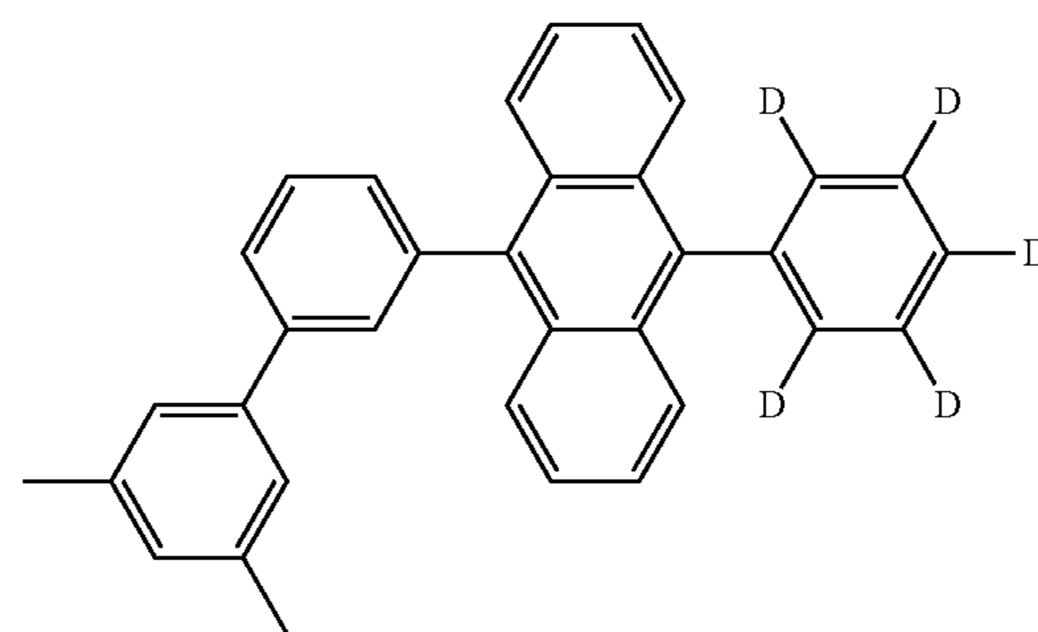
[Chemical Formula 191]
