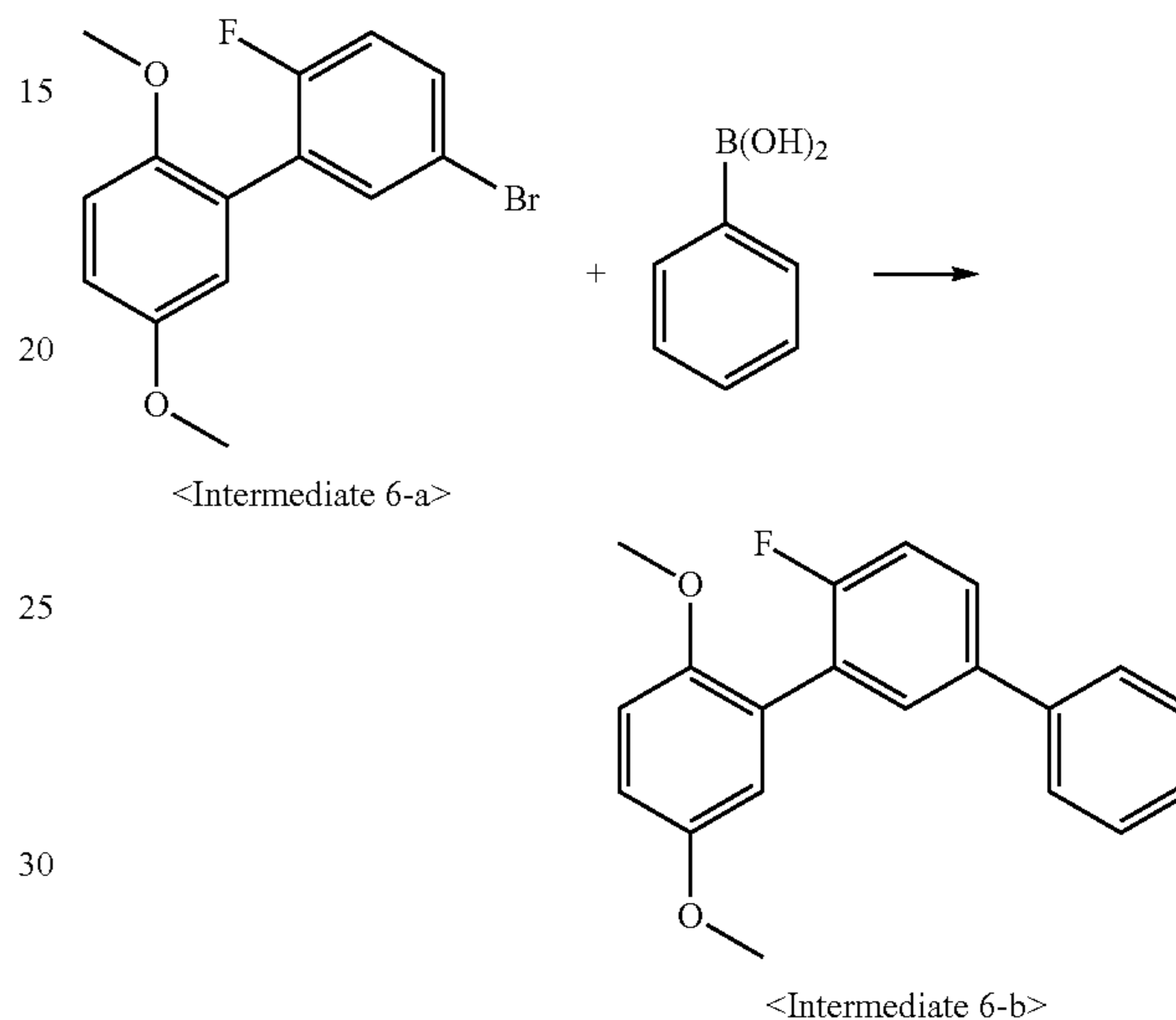
&lt;Reaction Scheme 31&gt;
