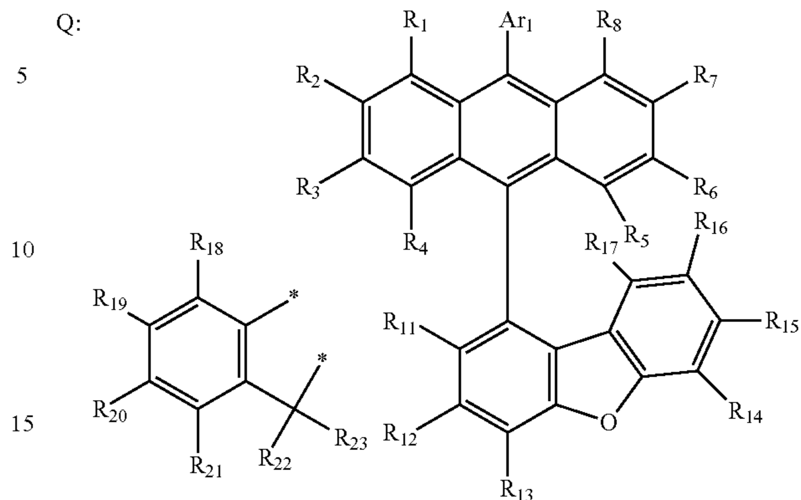
[Chemical Formula B-2]
