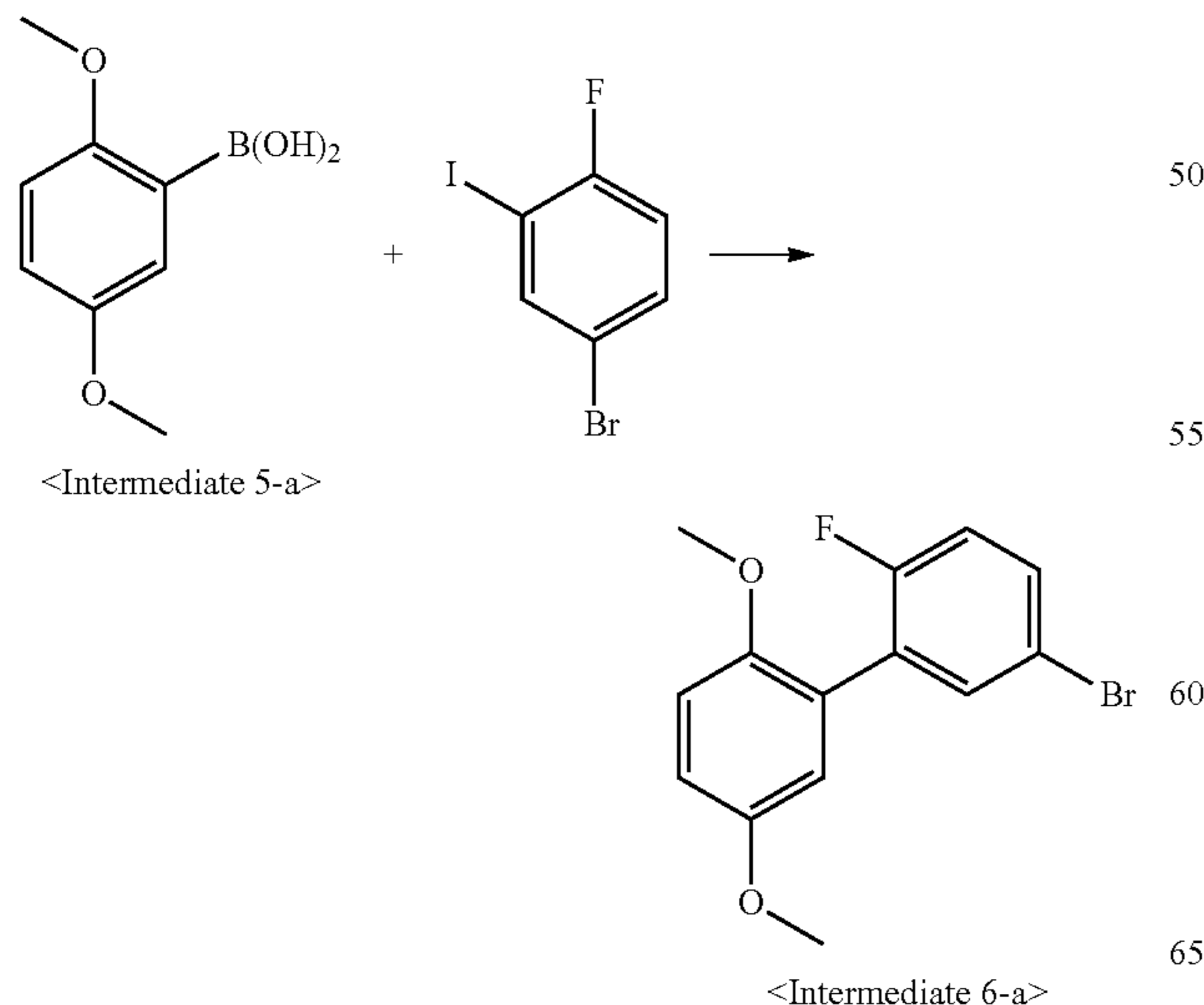
&lt;Reaction Scheme 30&gt;
