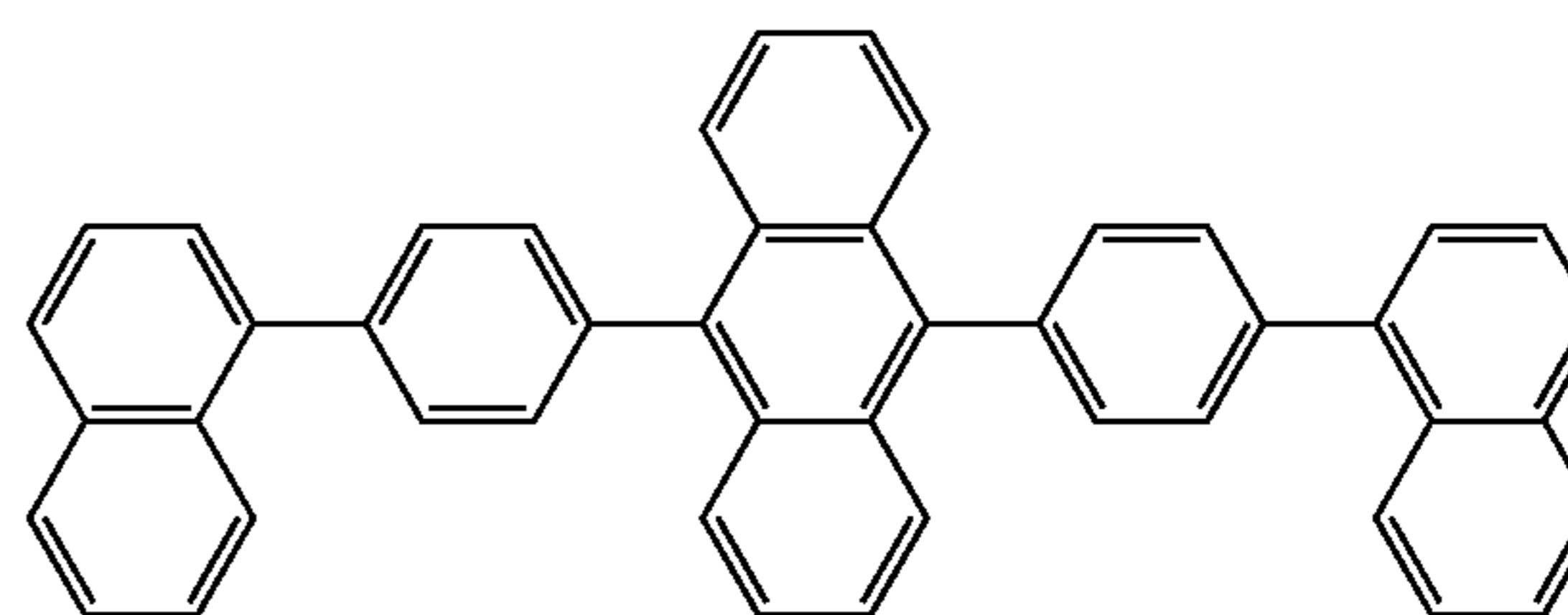
[Chemical Formula 102]
