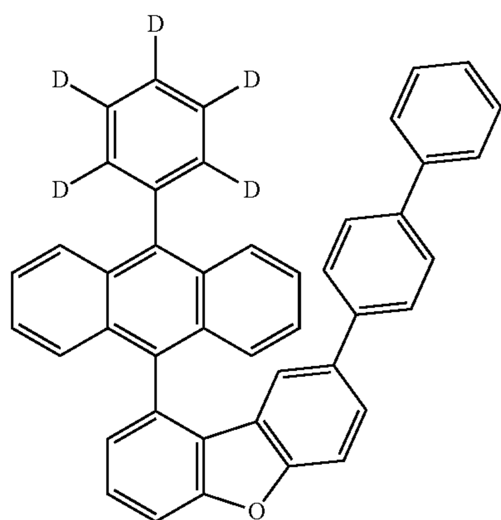
<Reaction Scheme 51>
