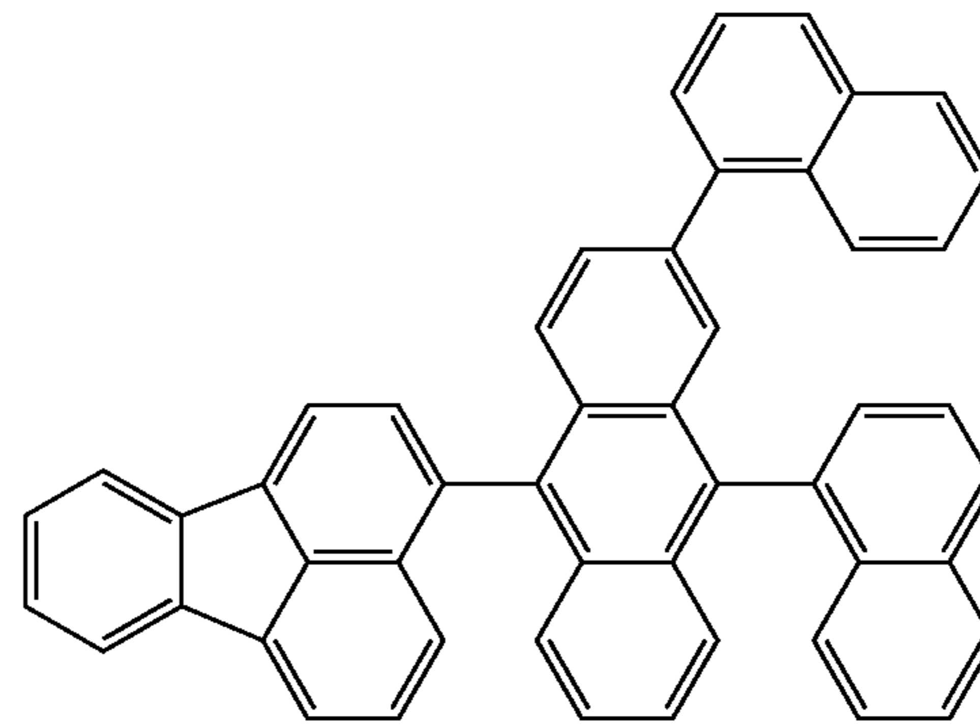
[Chemical Formula 275]
