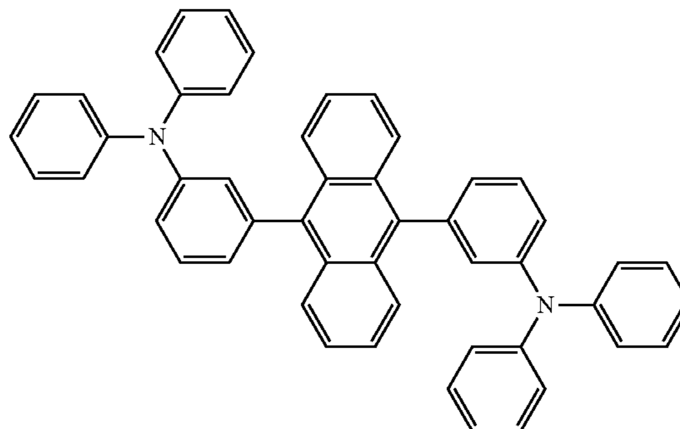
[Chemical Formula 117]
