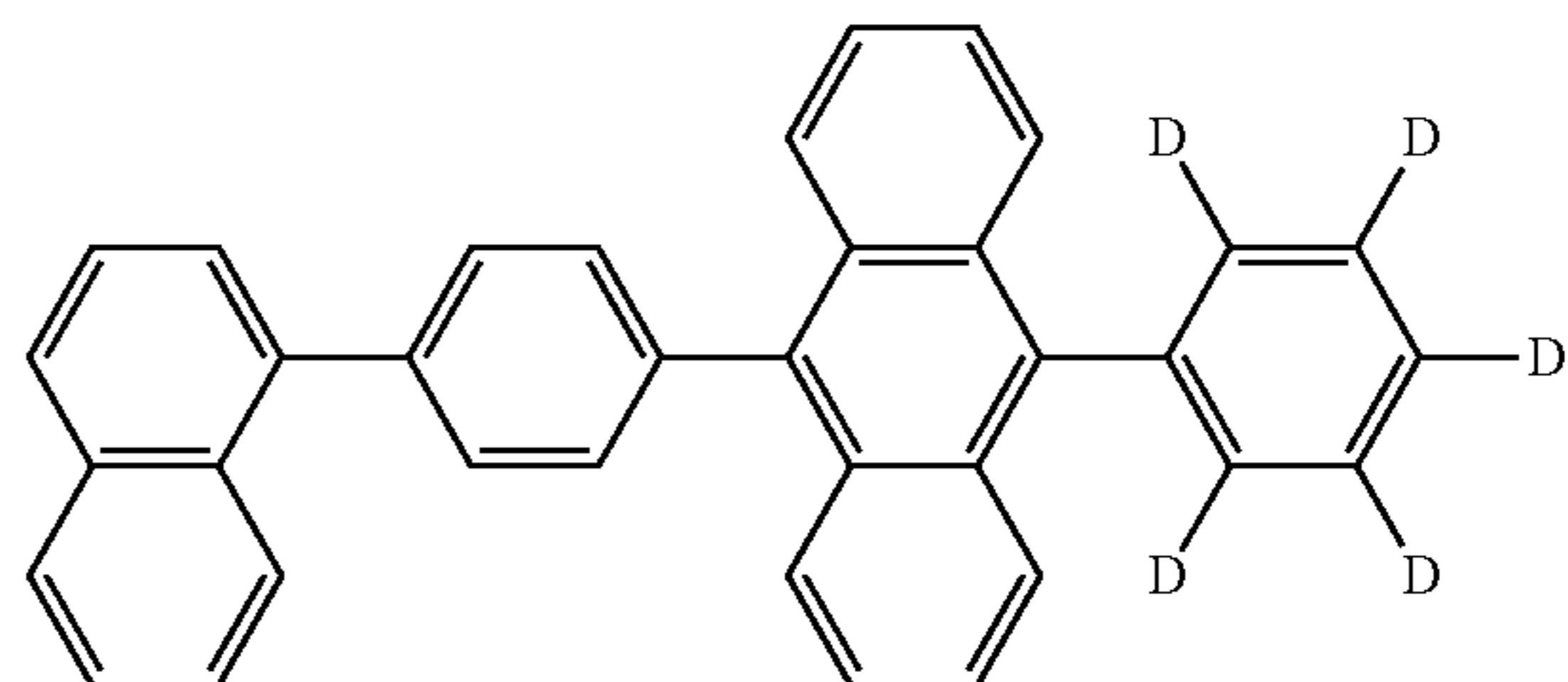
[Chemical Formula 129]
