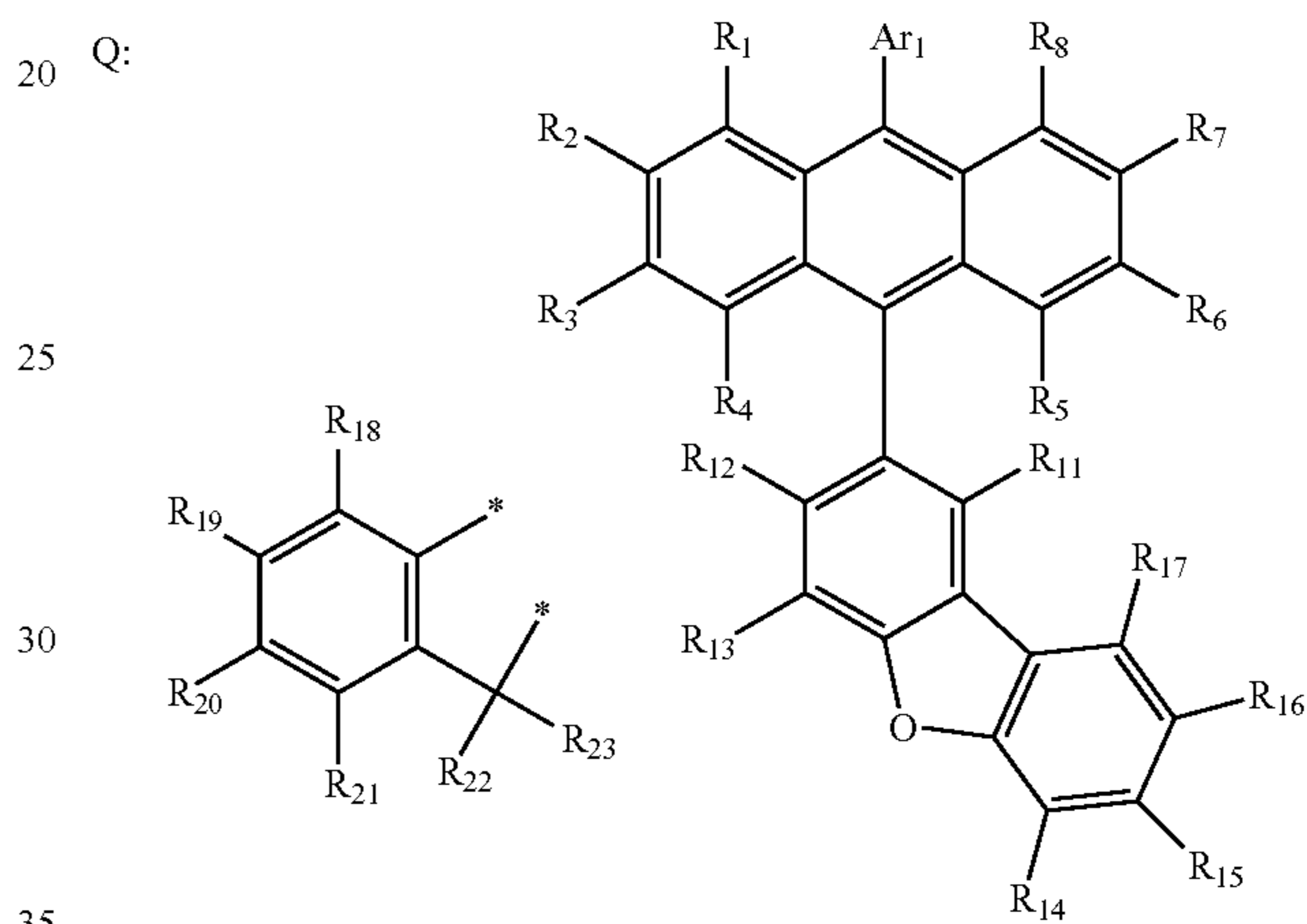
[Chemical Formula B-2]
