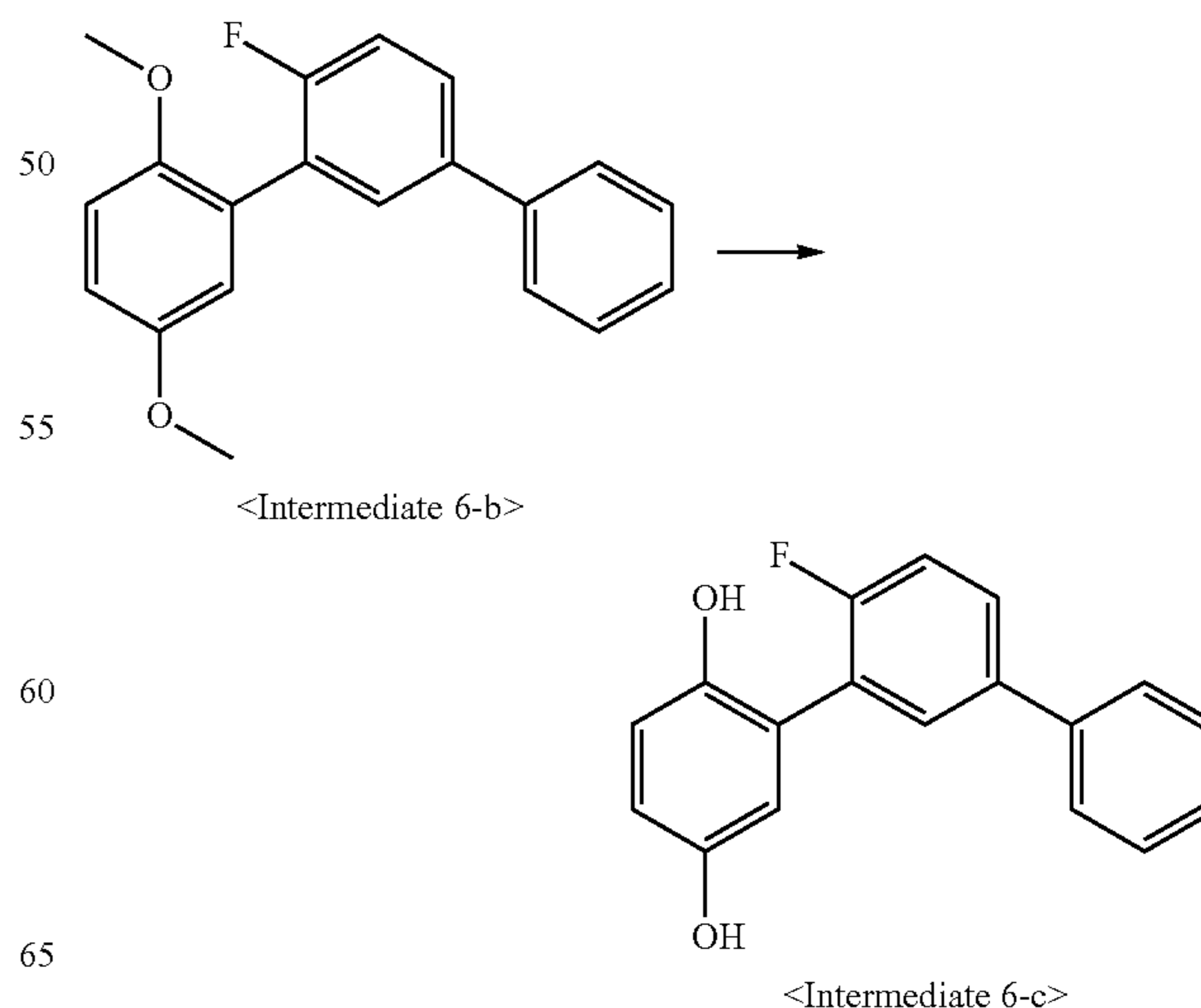
&lt;Reaction Scheme 32&gt;
