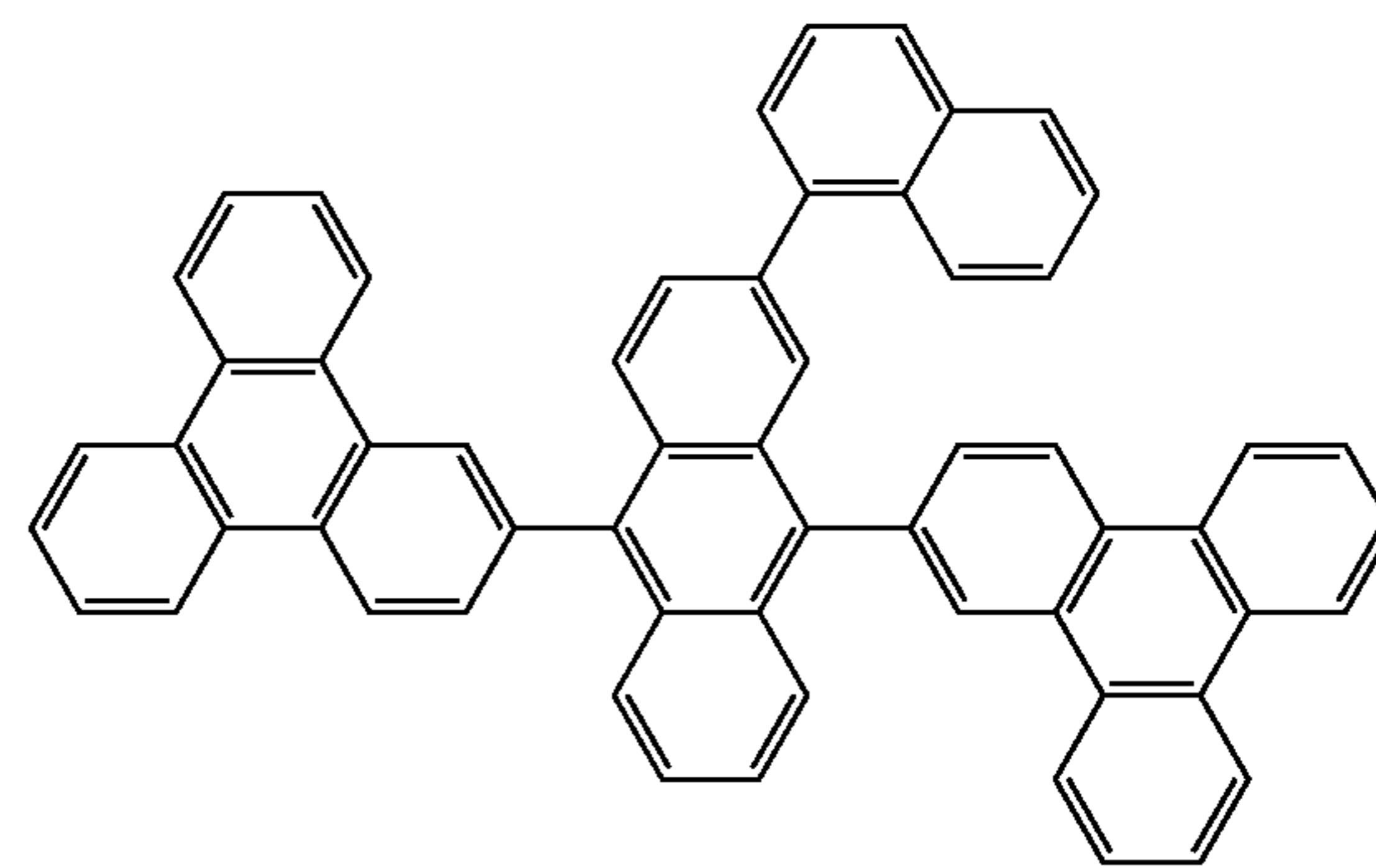
[Chemical Formula 277]
