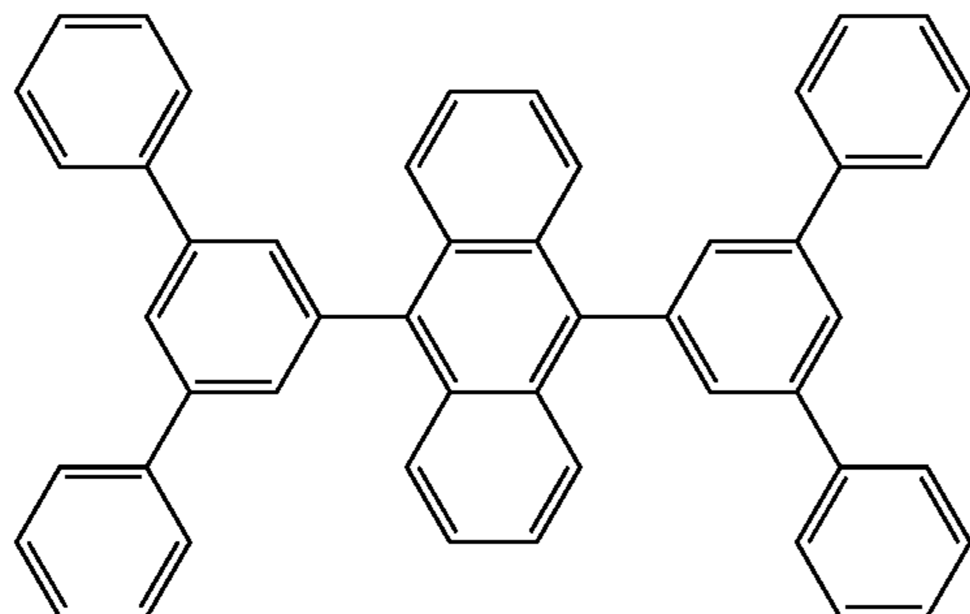
[Chemical Formula 114]
