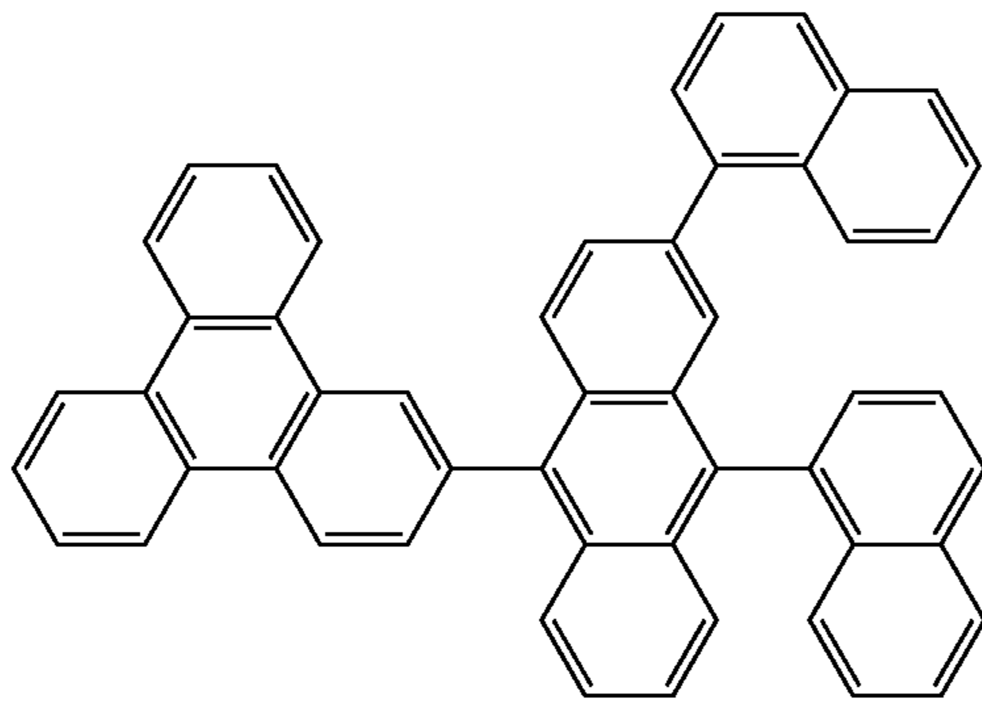
[Chemical Formula 274]
