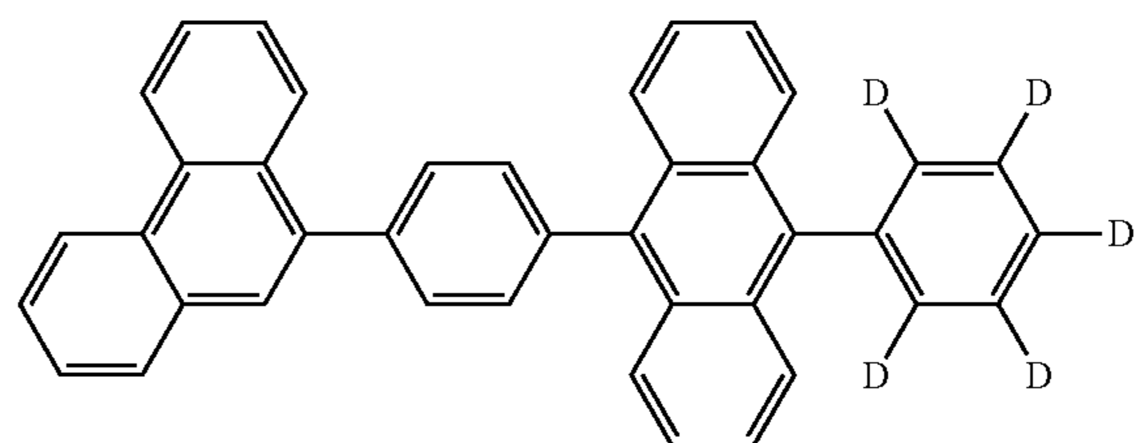
[Chemical Formula 131]
