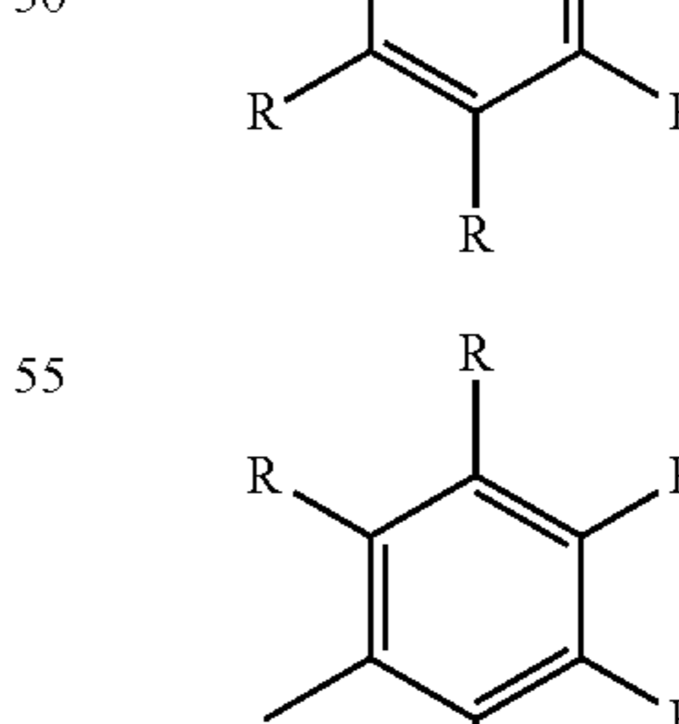
[Structural Formula C20]
