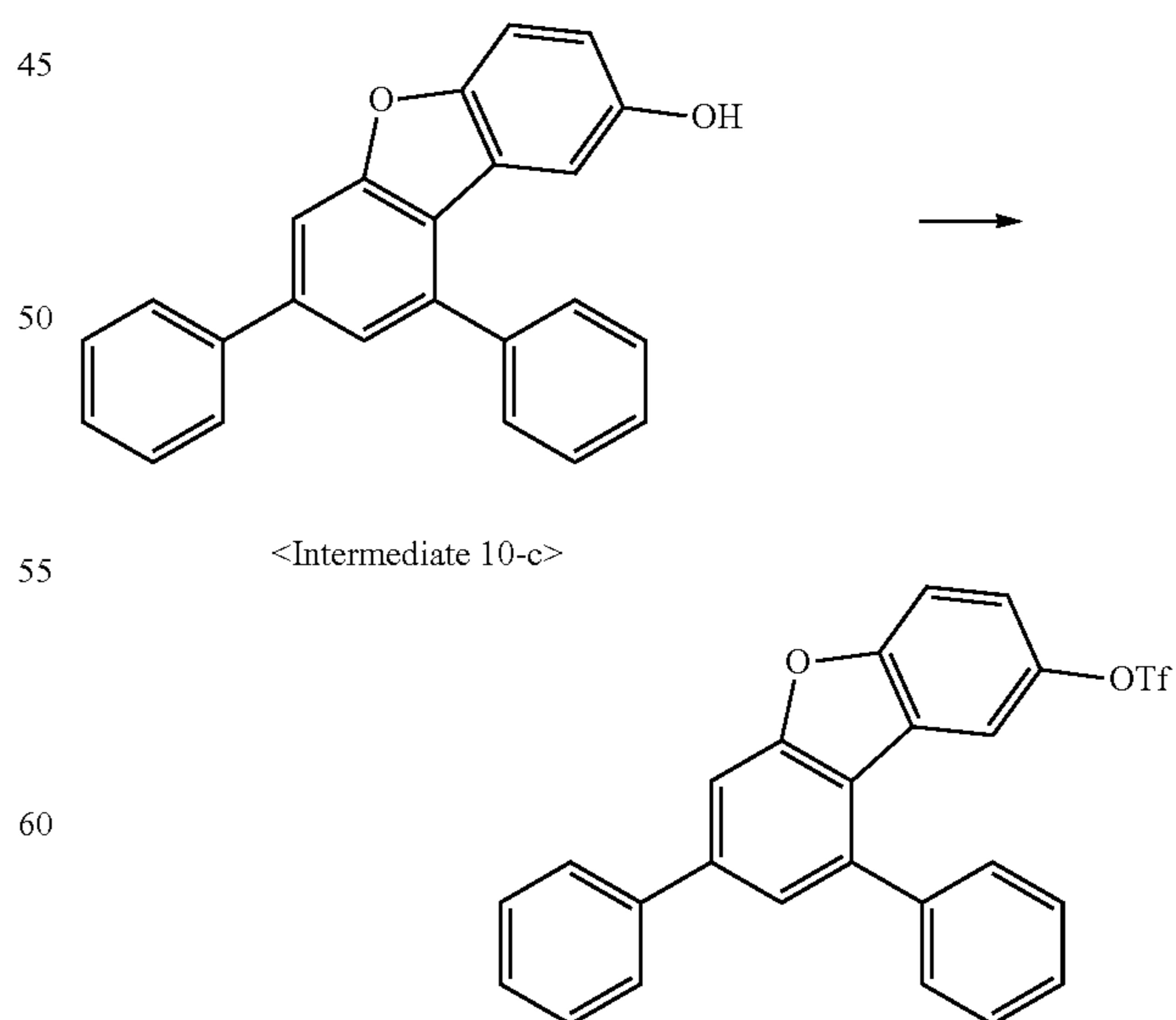
&lt;Reaction Scheme 60&gt;
