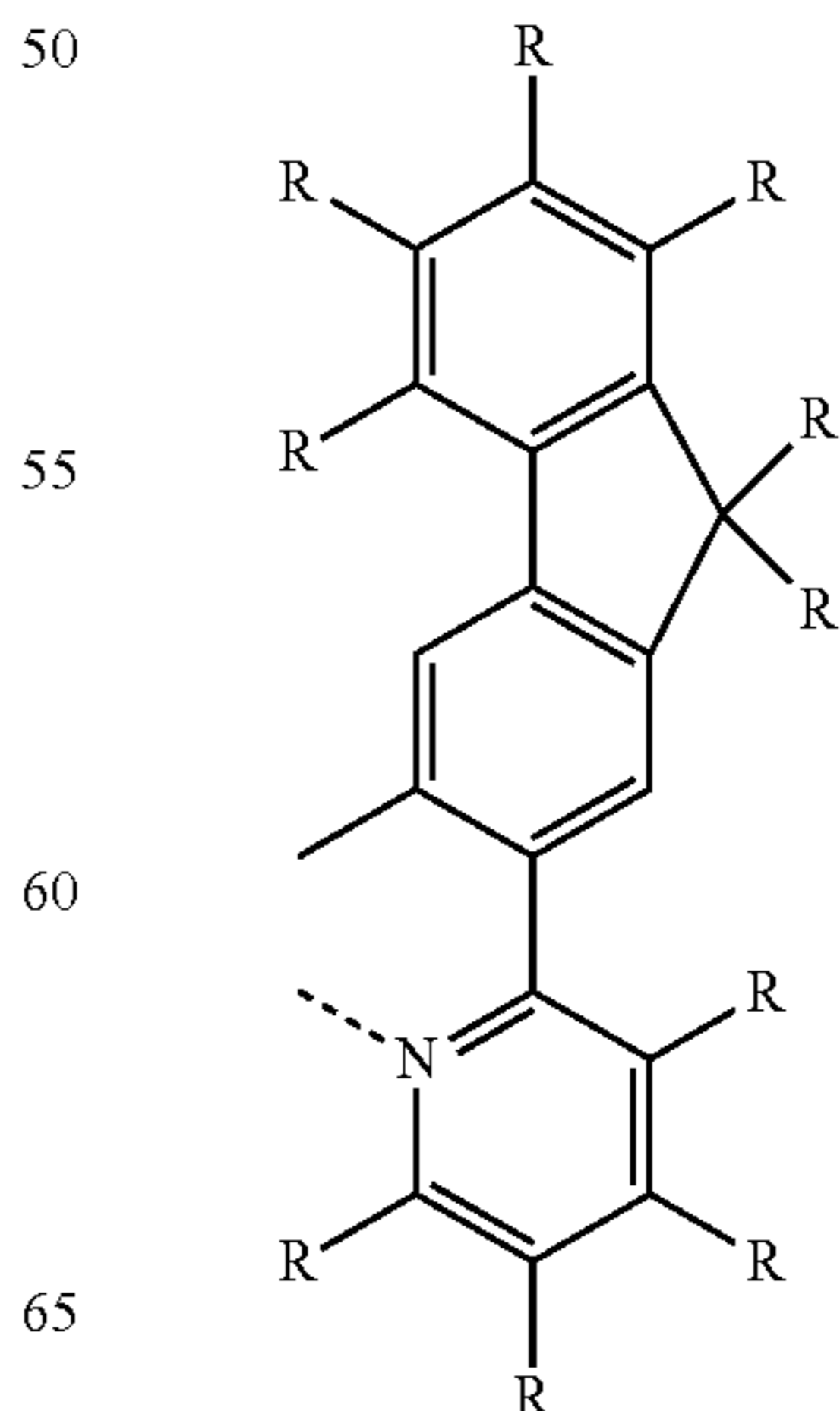
[Structural Formula C12]
