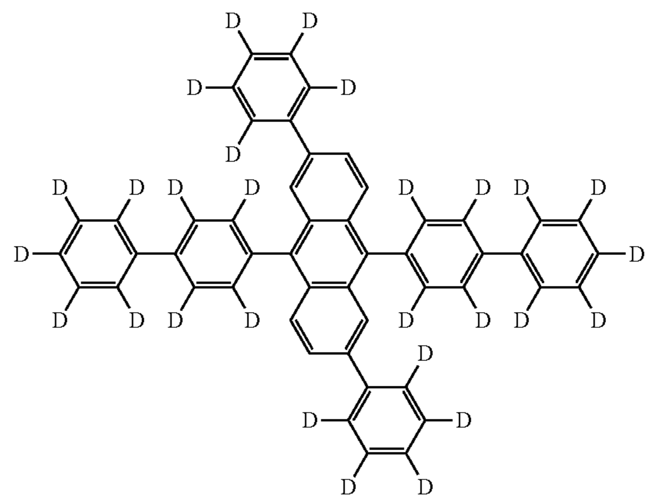
[Chemical Formula 189]
