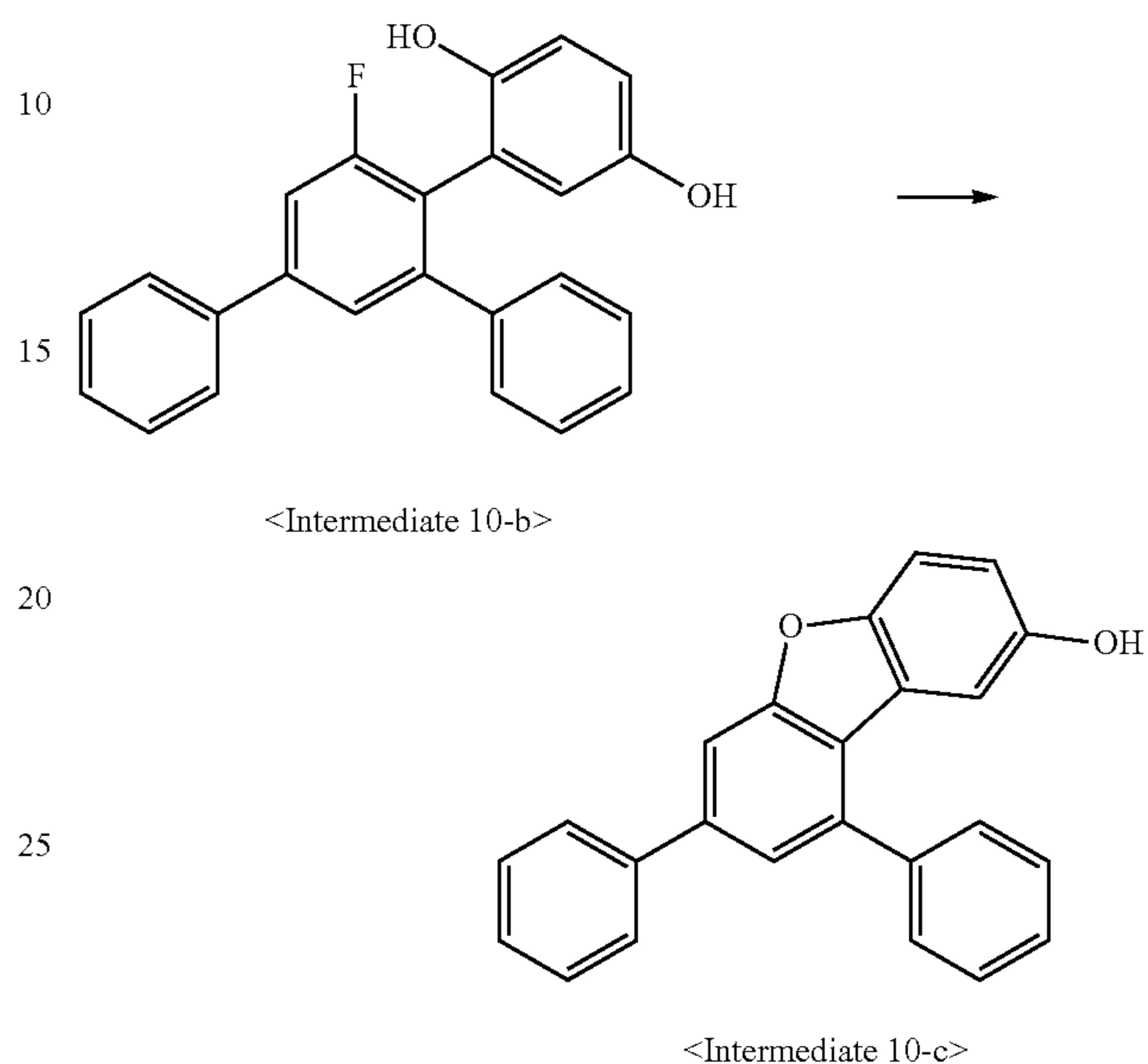
&lt;Reaction Scheme 59&gt;
