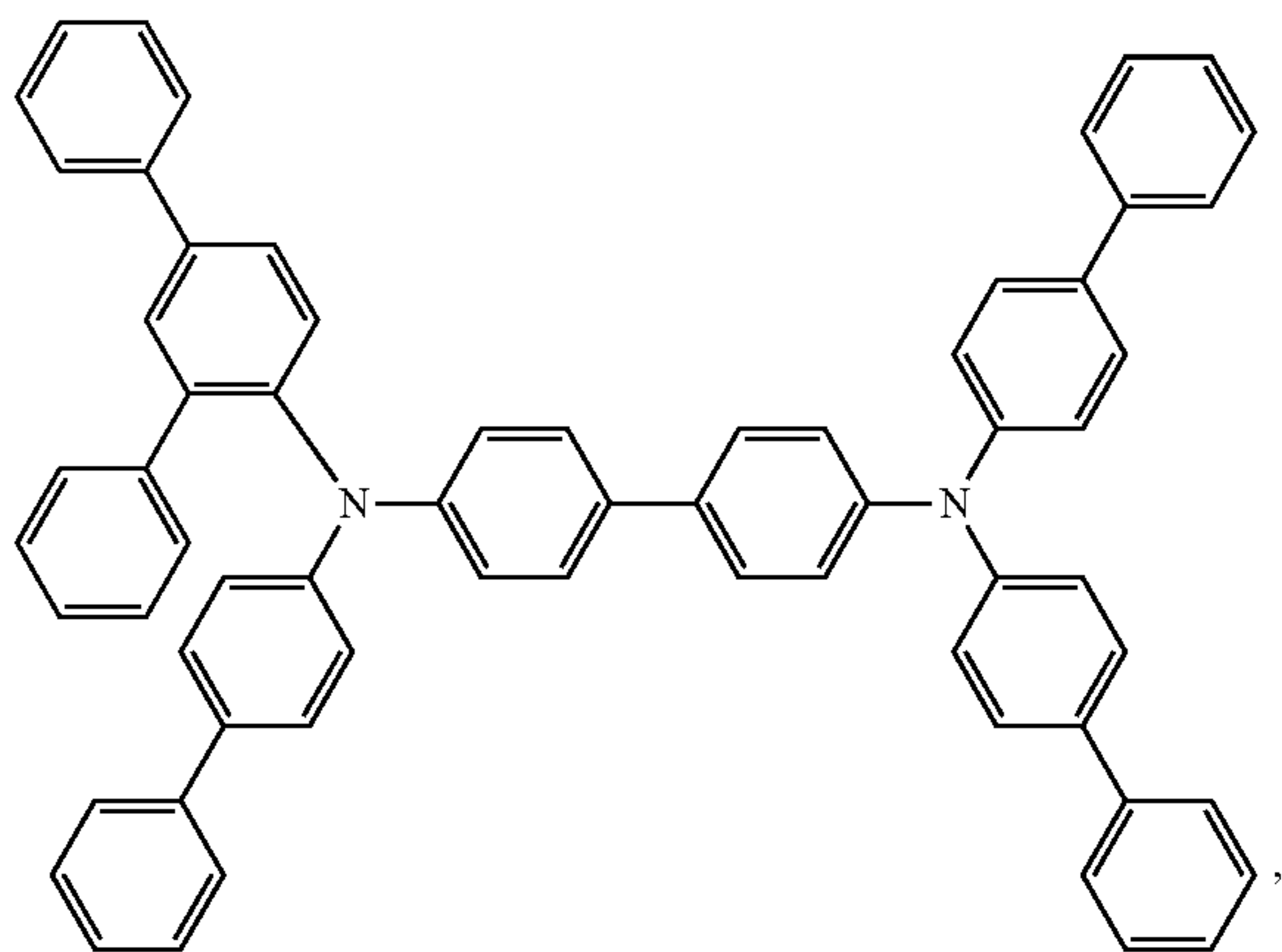
PPh-TPD
