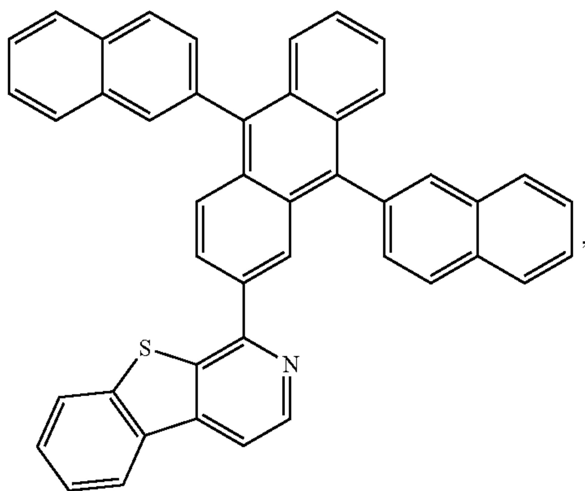
aDBT-ADN
