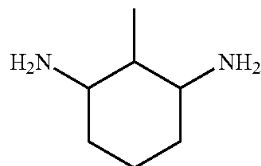
2-methylcyclohexane-1,3-diamine,
