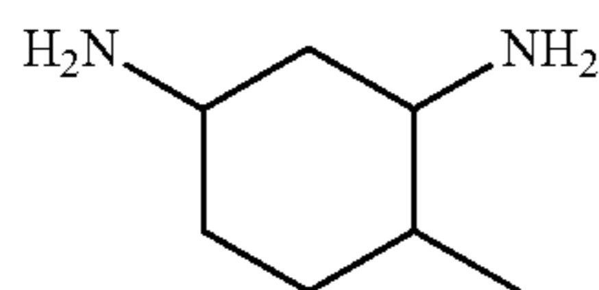
4-methylcyclohexane-1,3-diamine,
