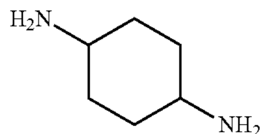
Cyclohexane-1,4-diamine,
