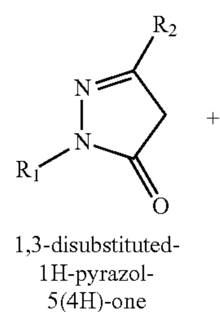
Scheme 2 General pathway to prepare Formula 2 related compounds
