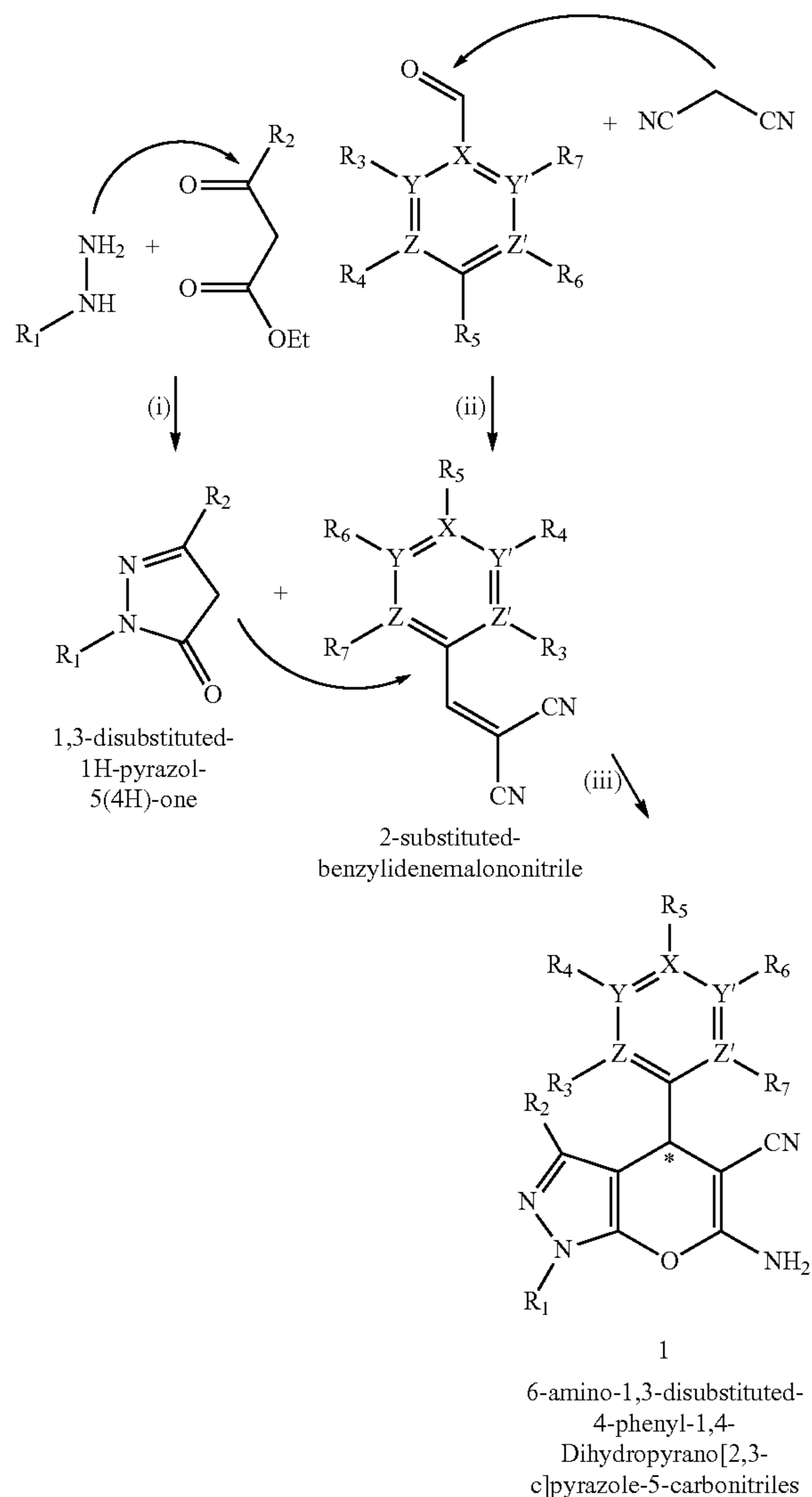
Scheme 1 General pathway to prepare Formula 1 related compounds
