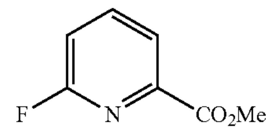
methyl 6-fluoropicolinate
