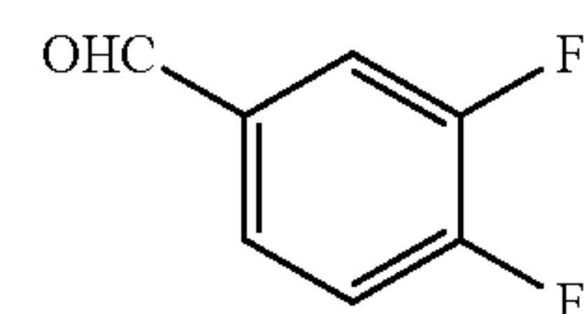
3,4-difluorobenzaldehyde
