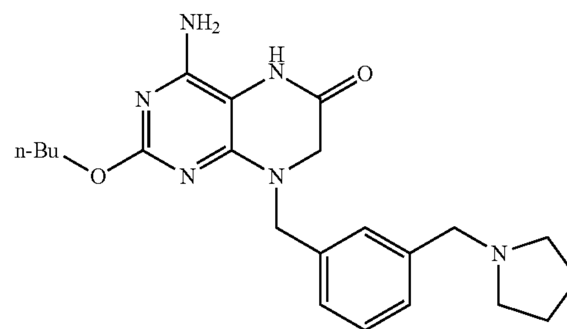
Vesatolimod
