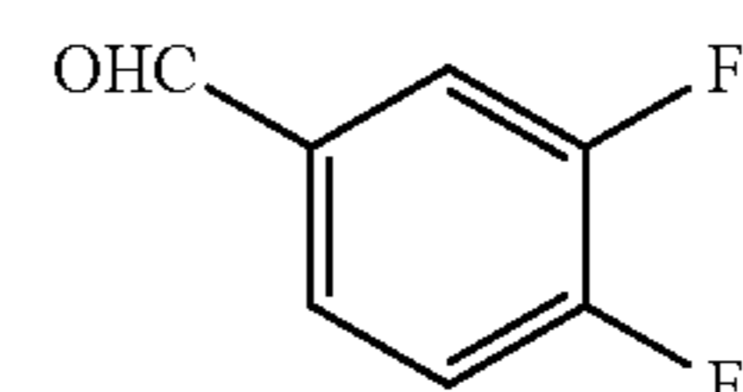
3,4-difluorobenzaldehyde
