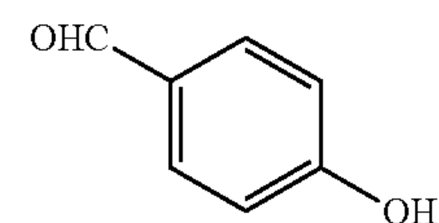
4-hydroxybenzaldehyde
