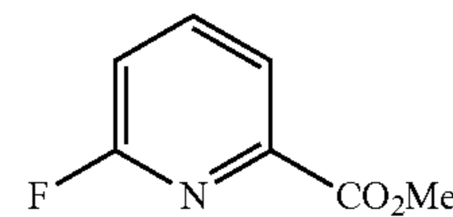
methyl 6-fluoropicolinate
