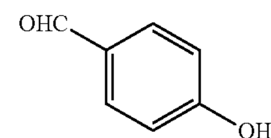
4-hydroxybenzaldehyde
