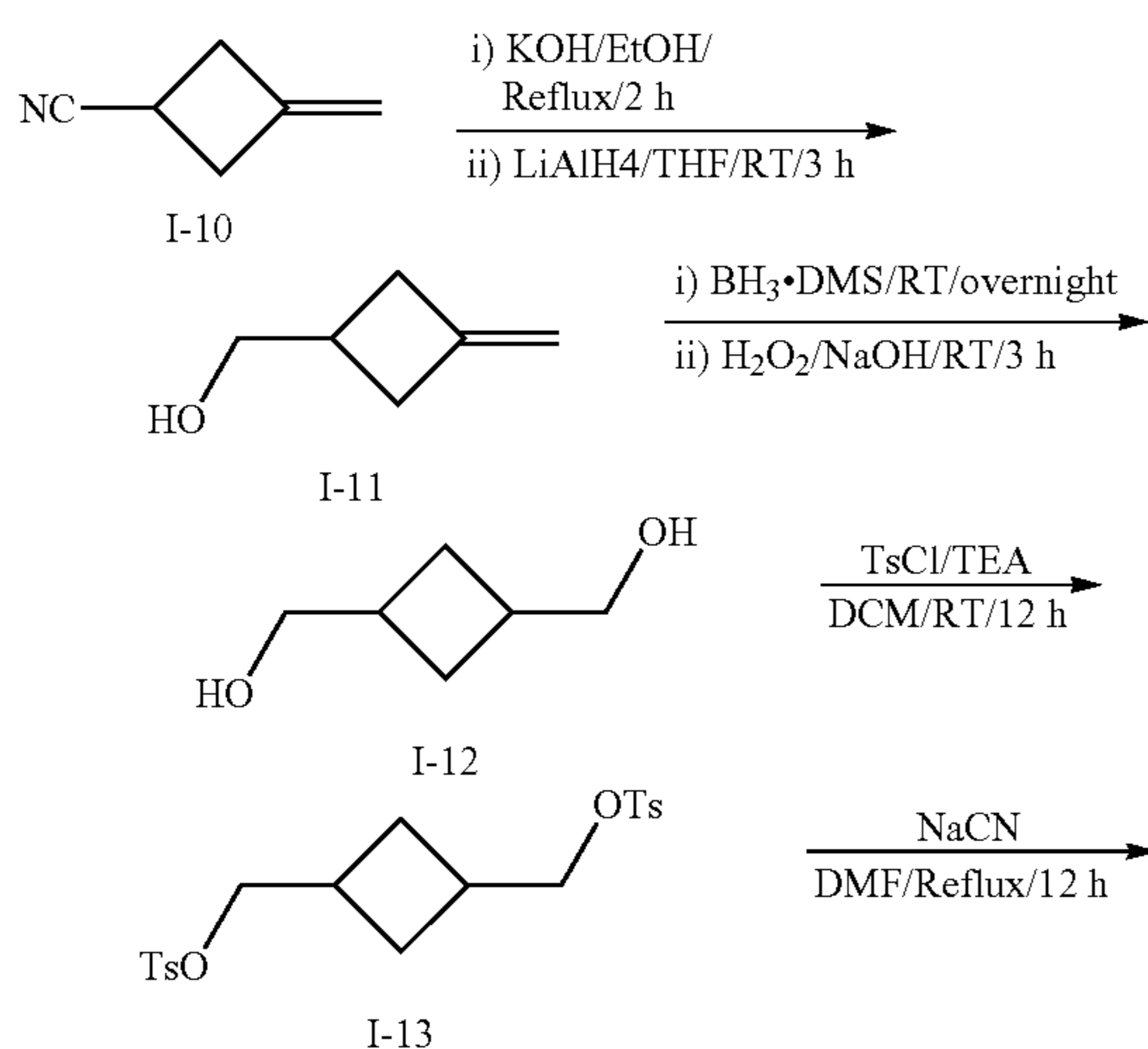
Scheme 12
