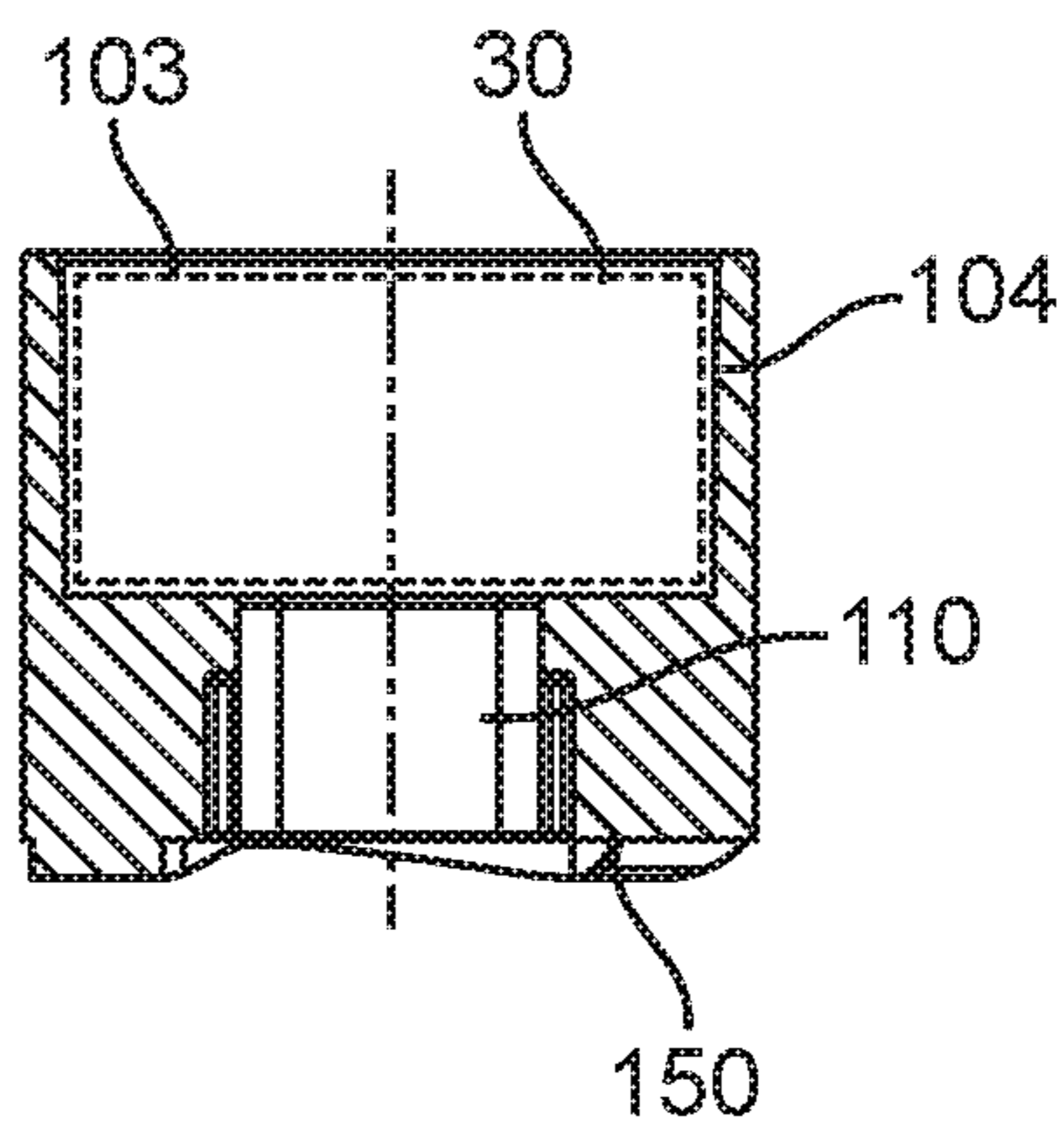
SECTION F-F
