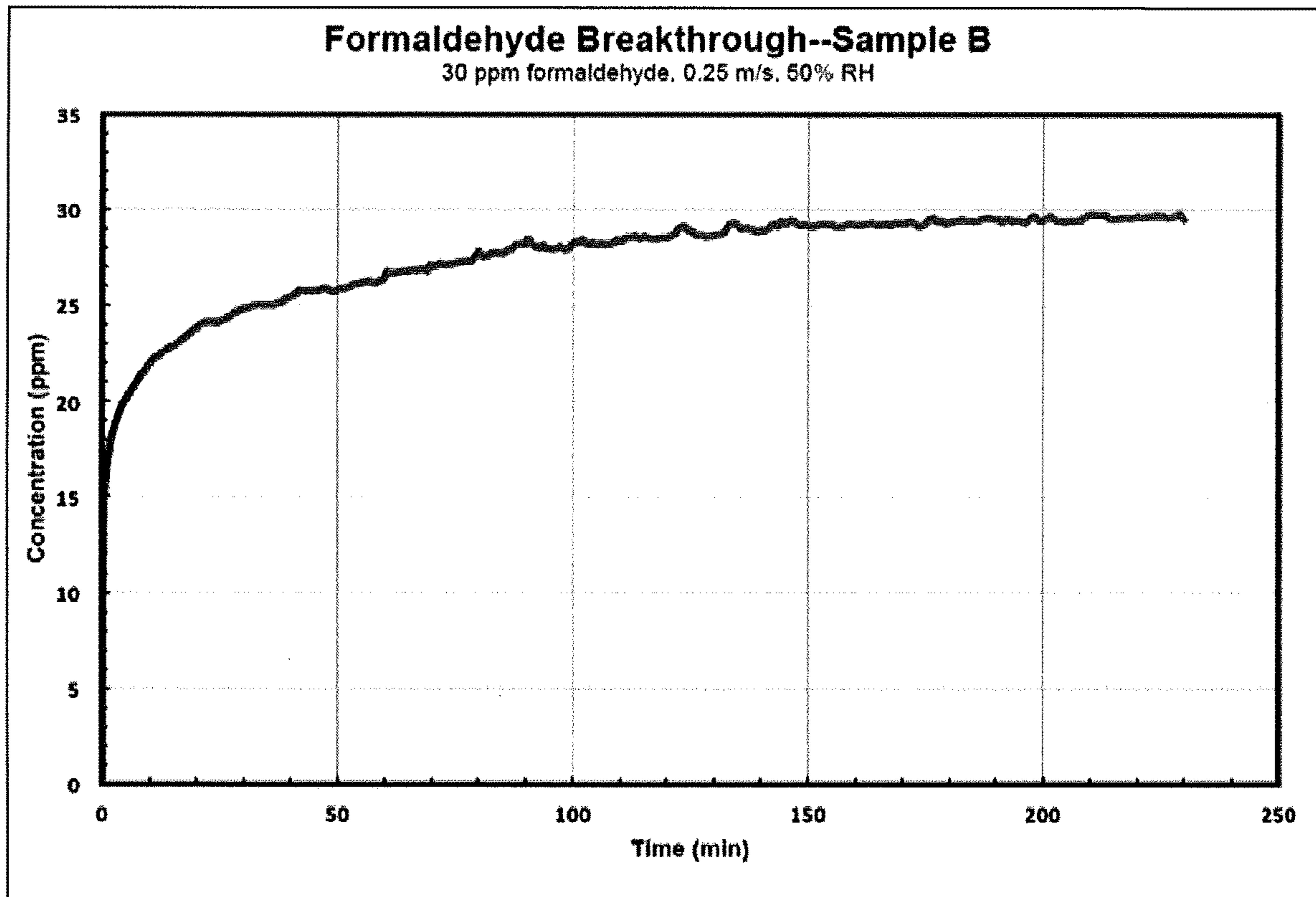
Concentration verses time for TRIS based impregnated carbon
