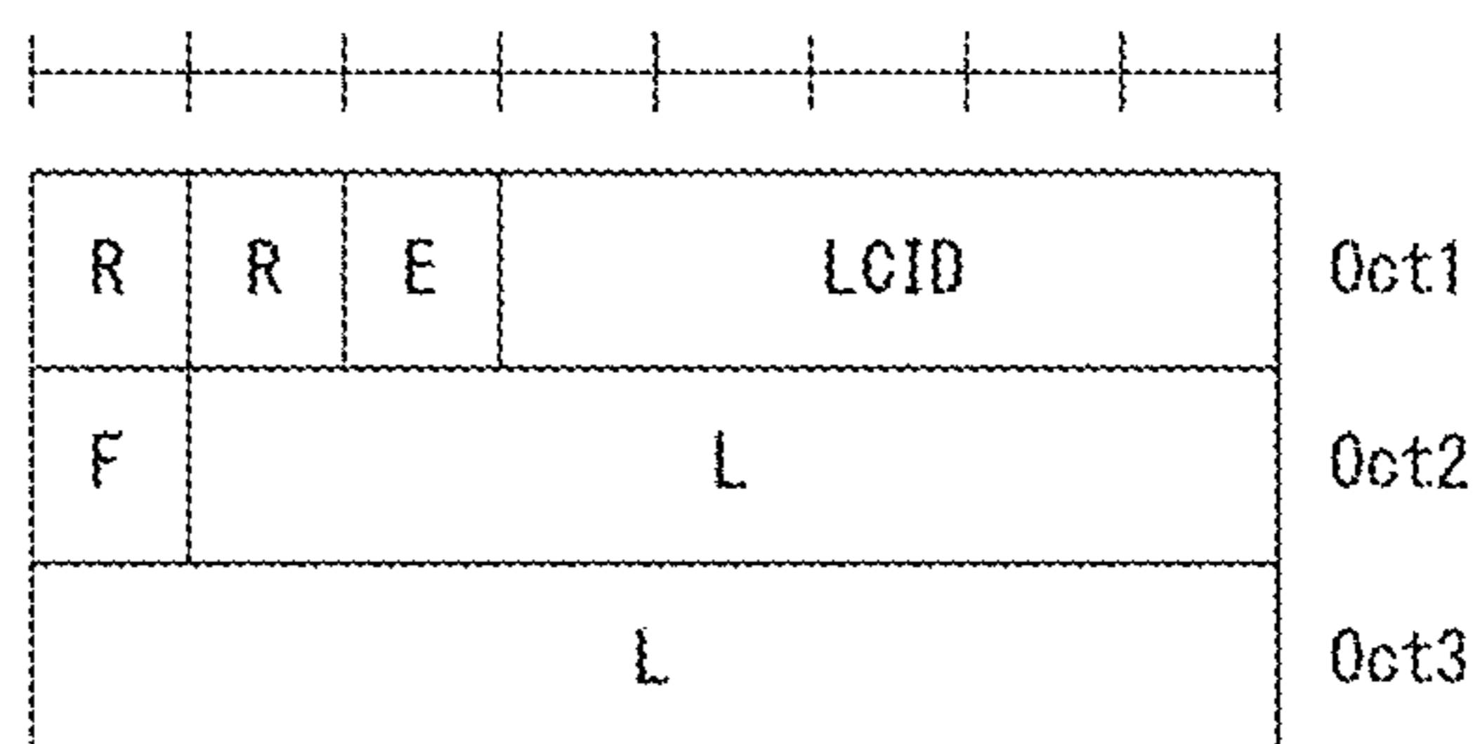
(b) R/R/E/LCID/F/L sub-header with 15-bit L field
