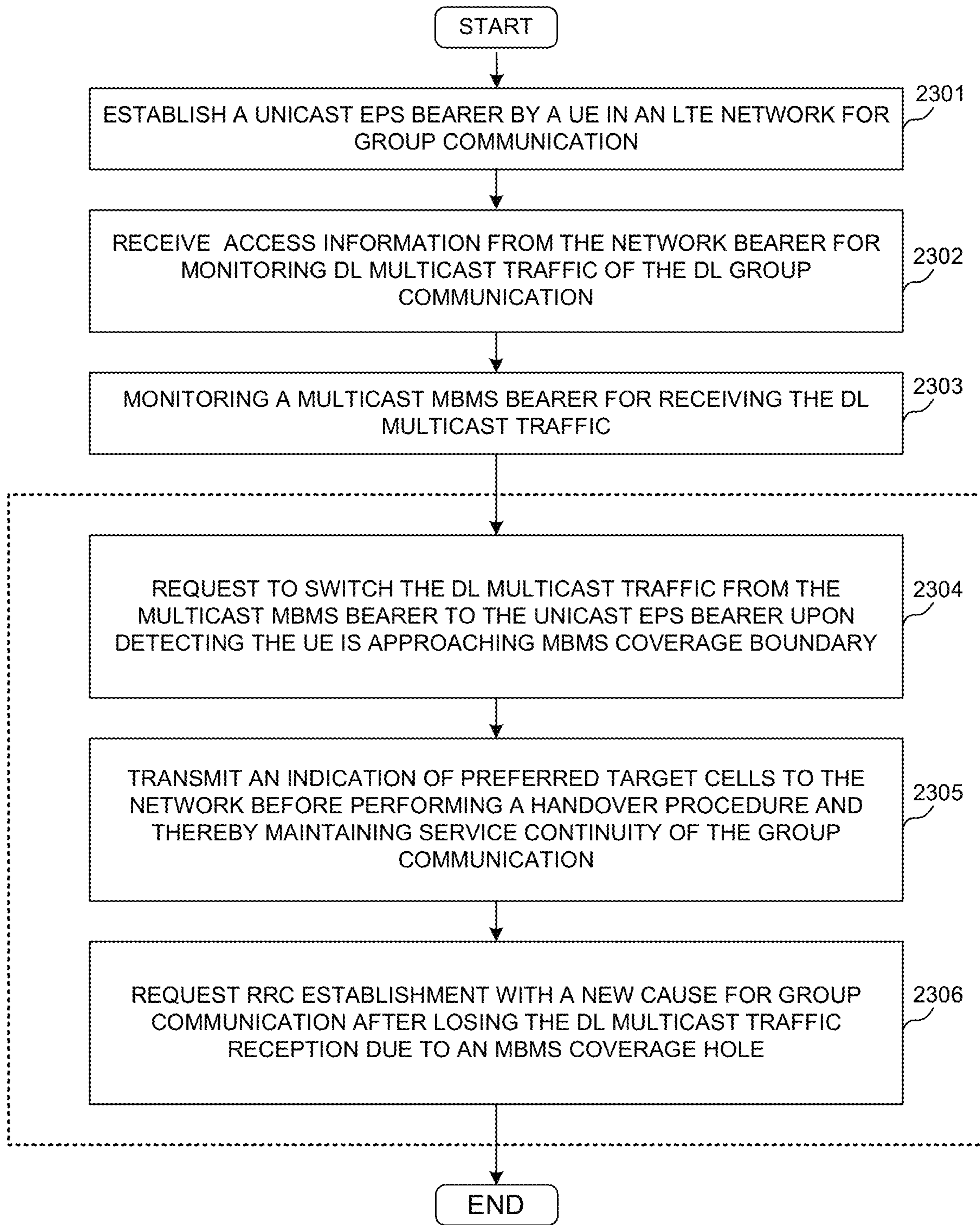
POC MULTICAST TRAFFIC SERVICE CONTINUITY
