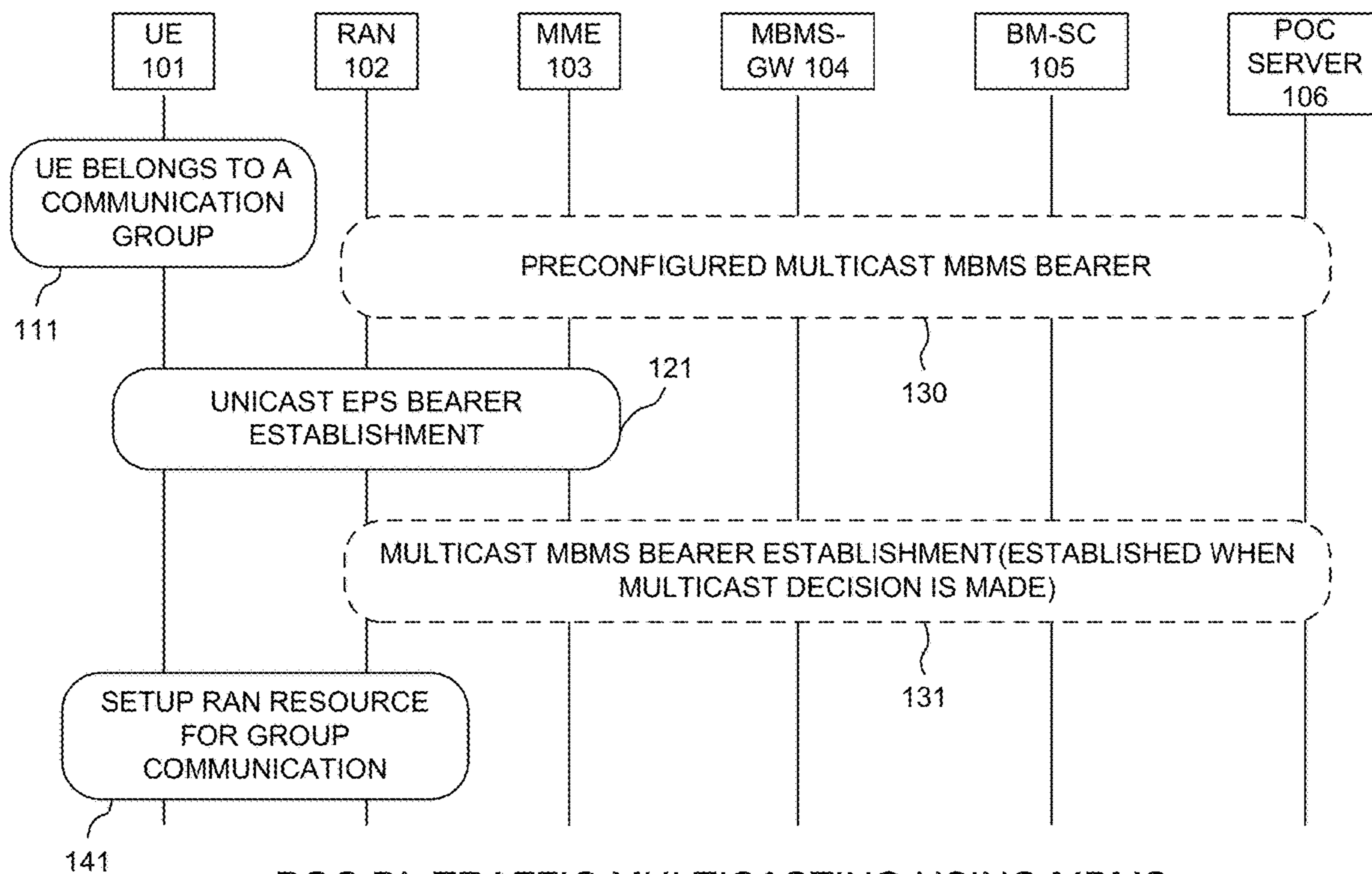
POC DL TRAFFIC MULTICASTING USING MBMS FIG. 1
