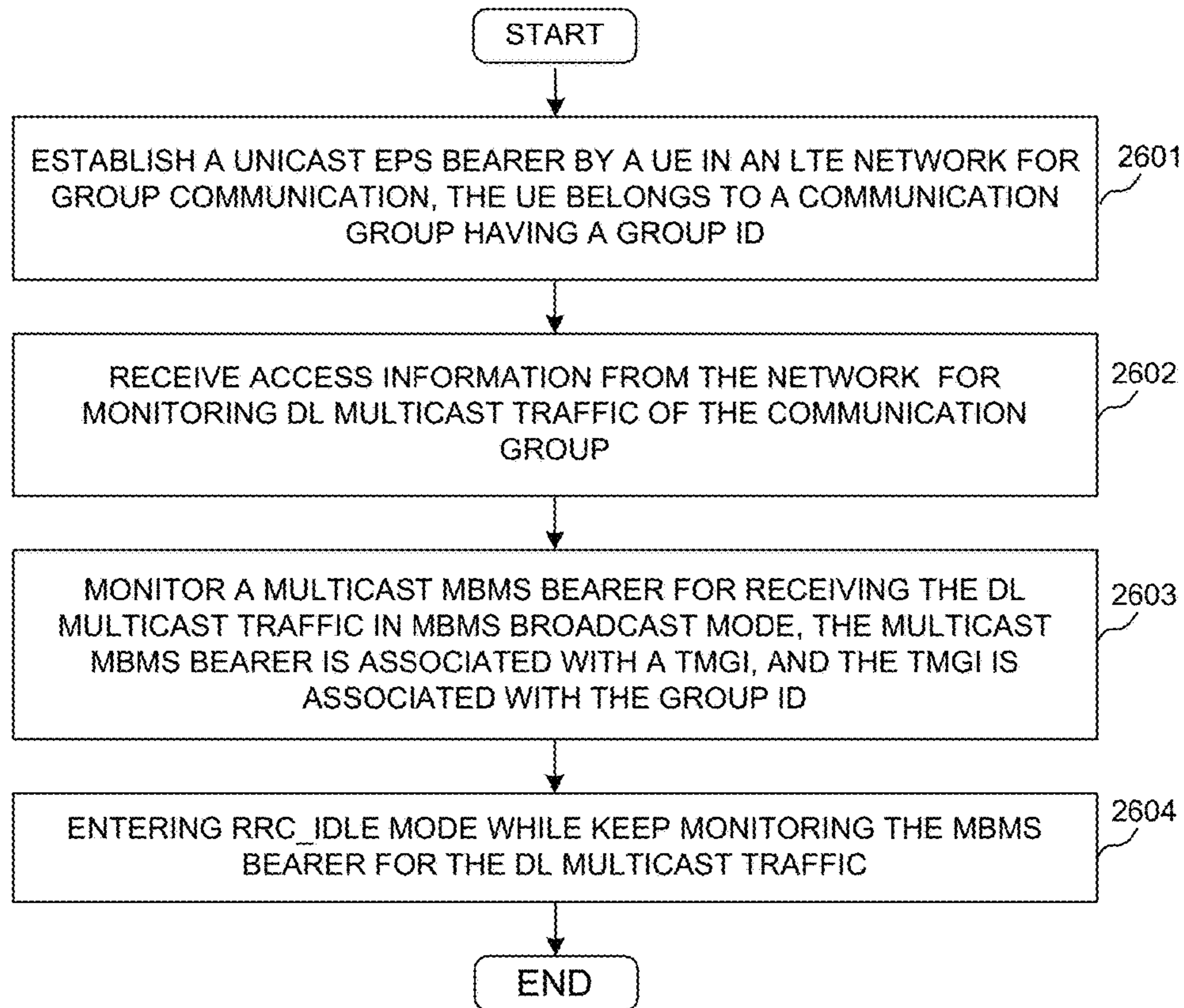
IDLE MODE RECEPTION FOR POC TRAFFIC FIG. 26
