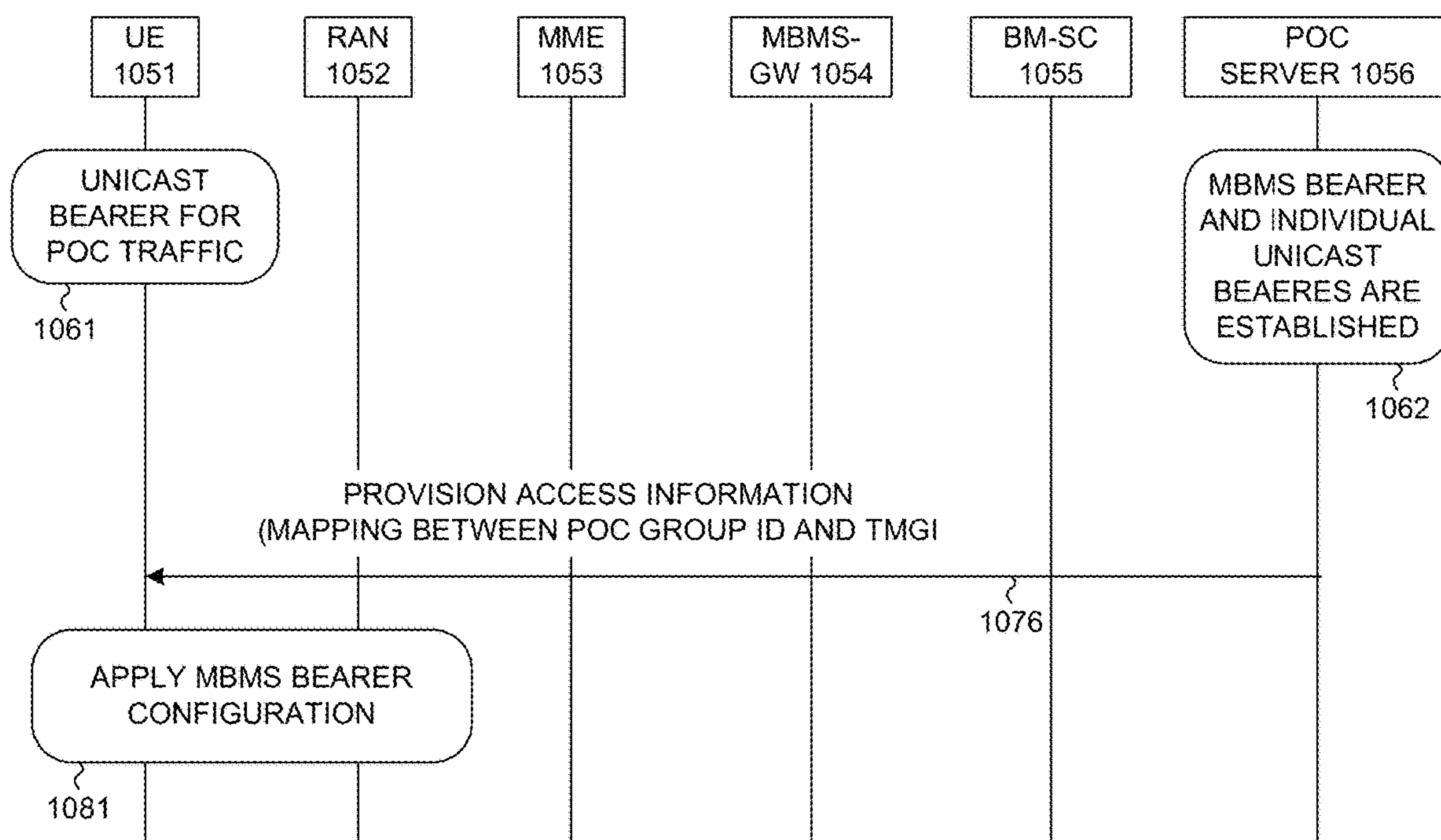
PROACTIVE MBMS BEARER ESTABLISHMENT BASED ON MBMS BROADCAST MODE FIG. 10B
