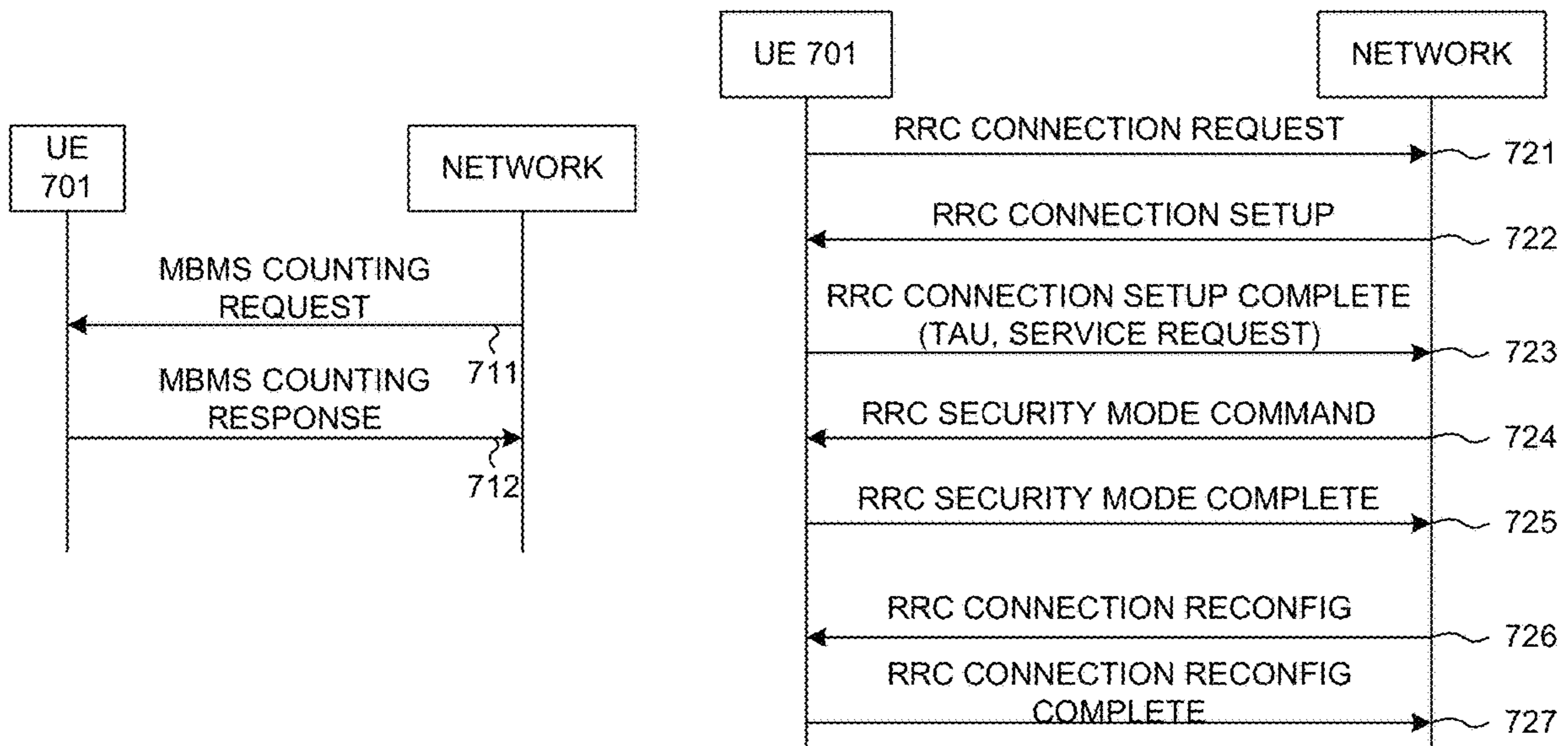
MBMS RECEPTION STATUS INDICATION FIG. 7
