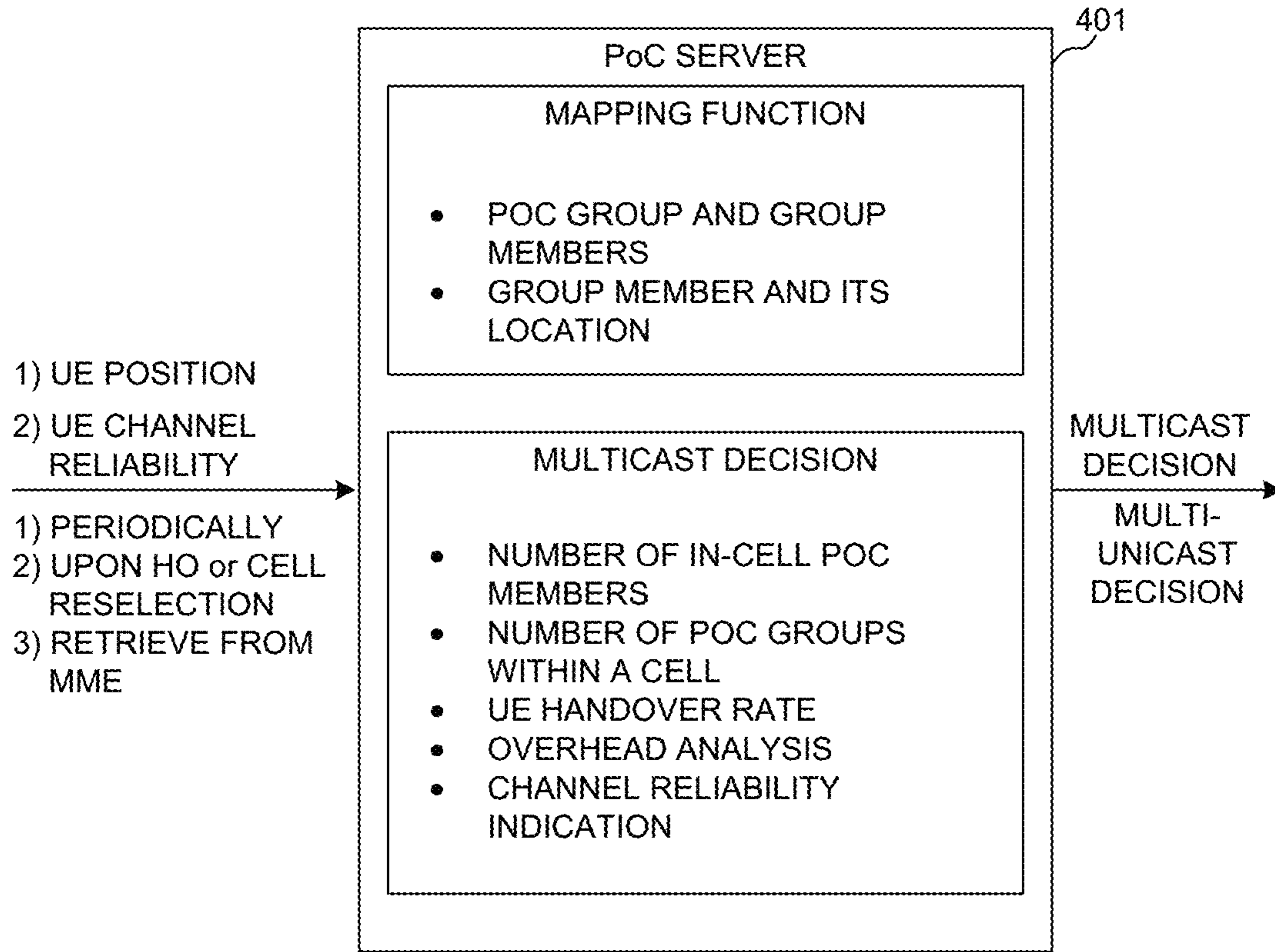
POC SERVER FOR GROUP MOBILITY MANAGEMENT FIG. 4
