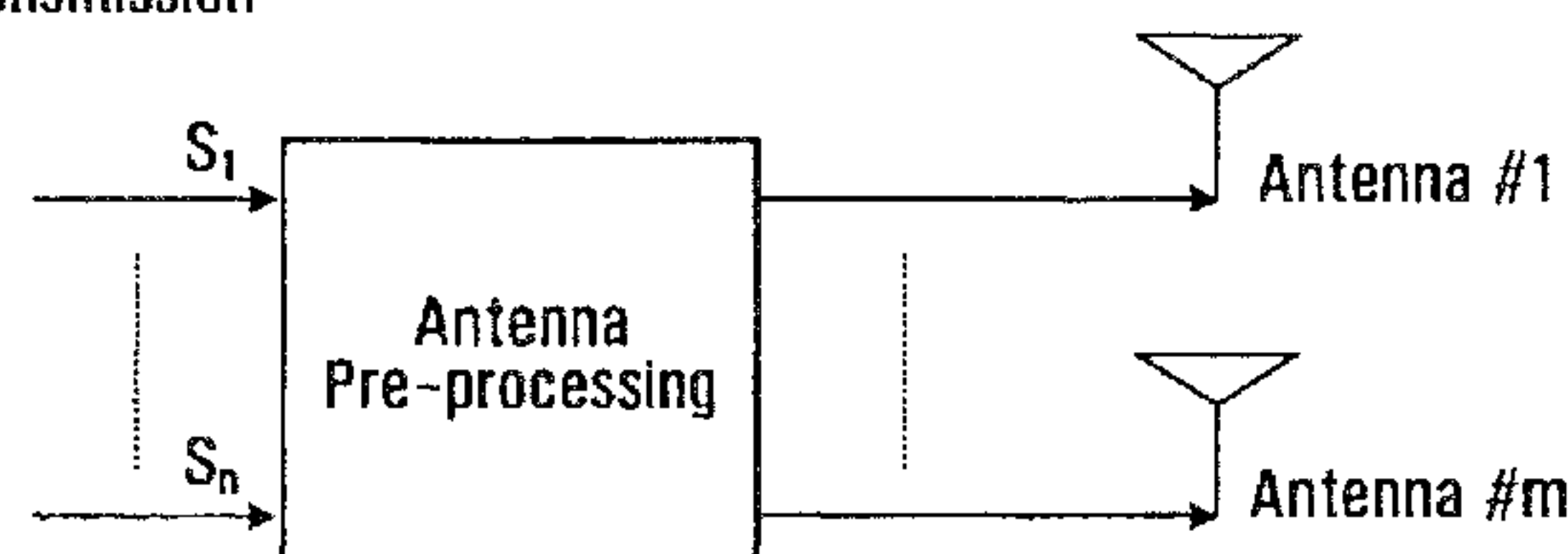
First transmission
