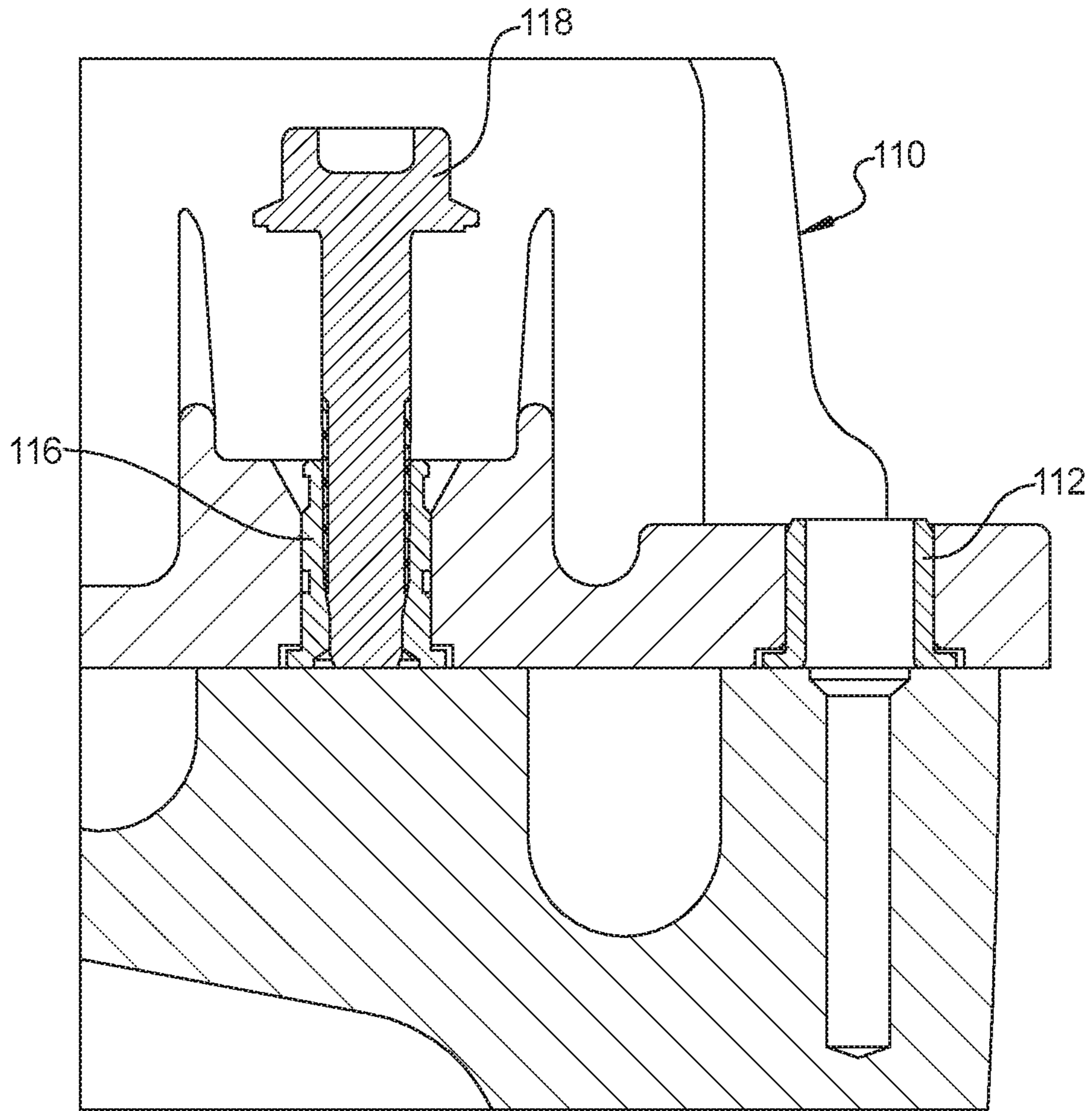
FIG 5 PRIOR ART
