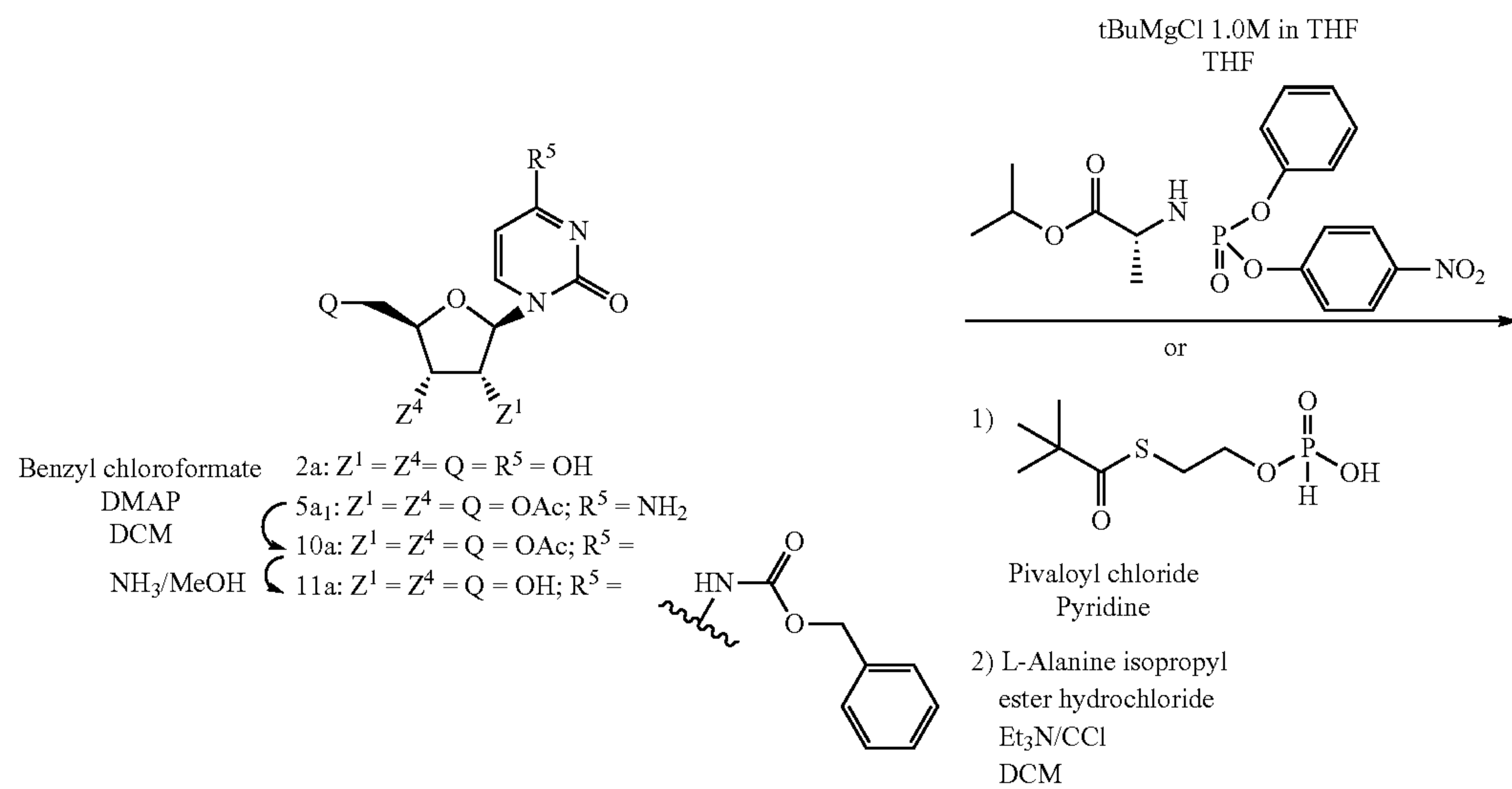
Scheme 4
