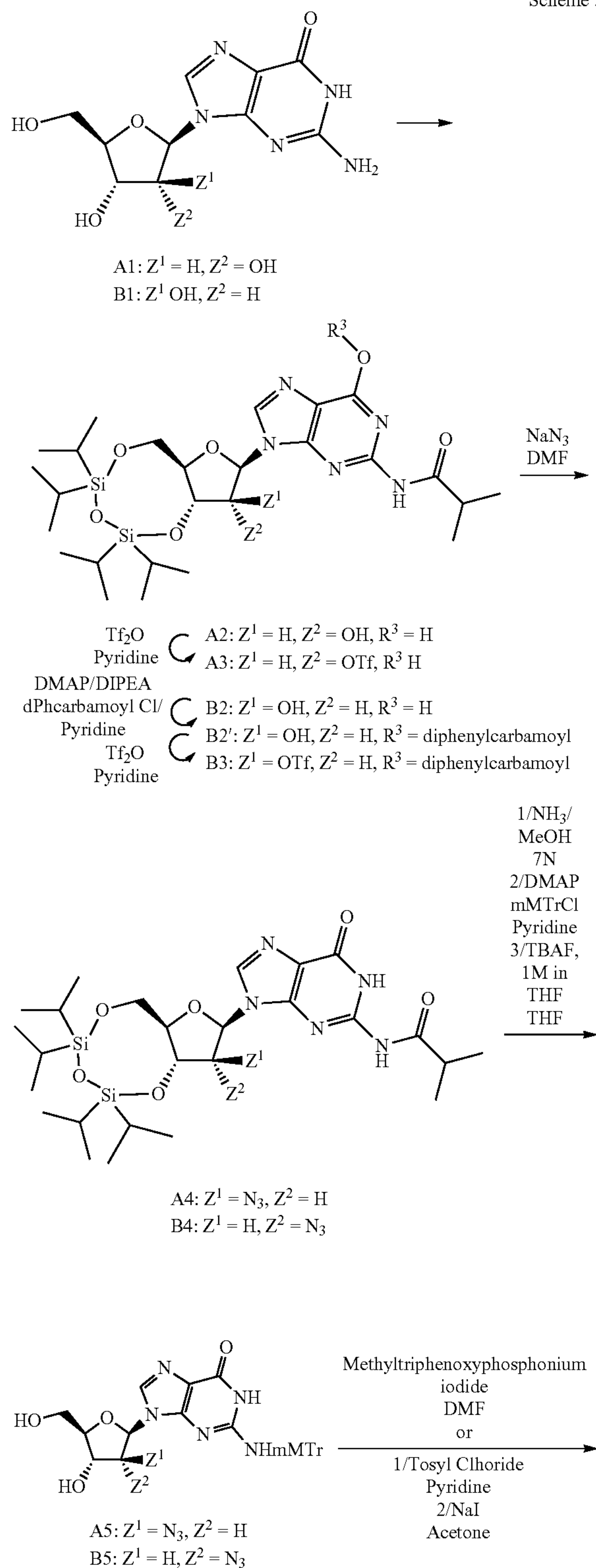
SCHEME 5
