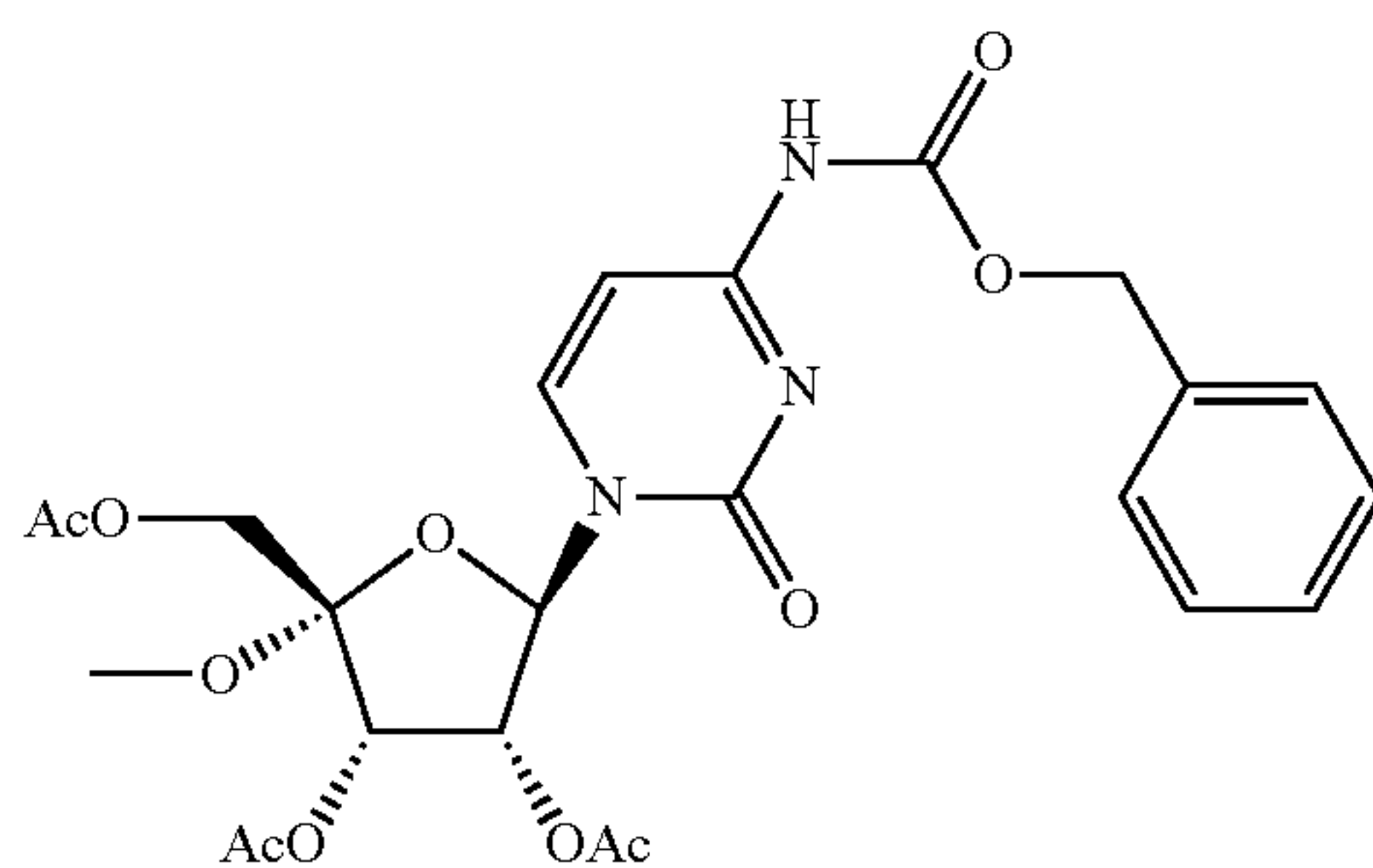
Compound (10a)
