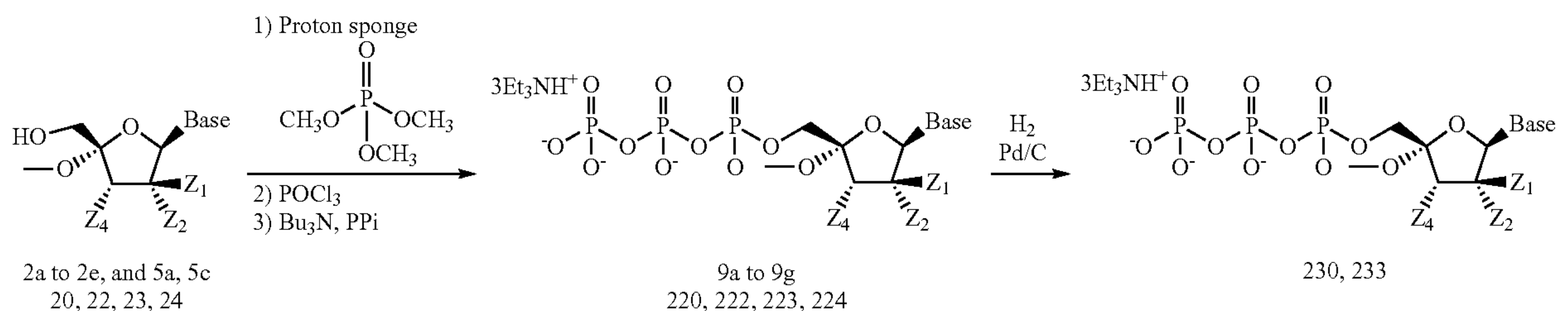
Scheme 3
