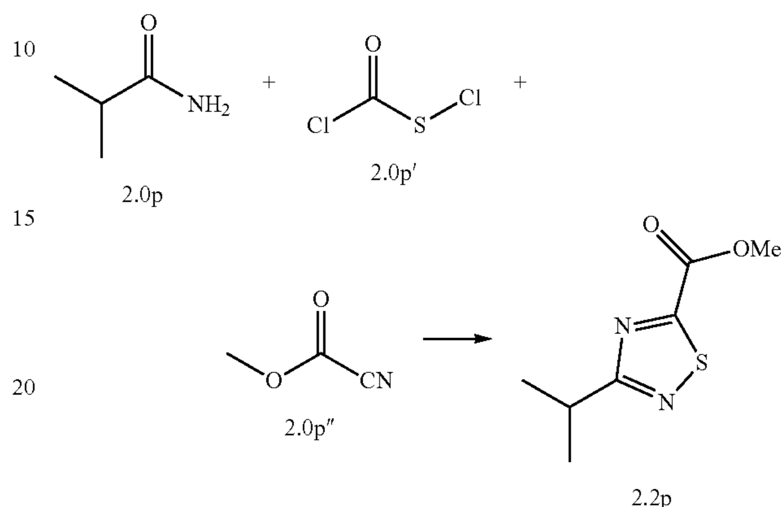
Scheme 14: Synthesis of methyl 3-isopropyl-1,2,4-thiadiazole-5-carboxylate 2.2p
