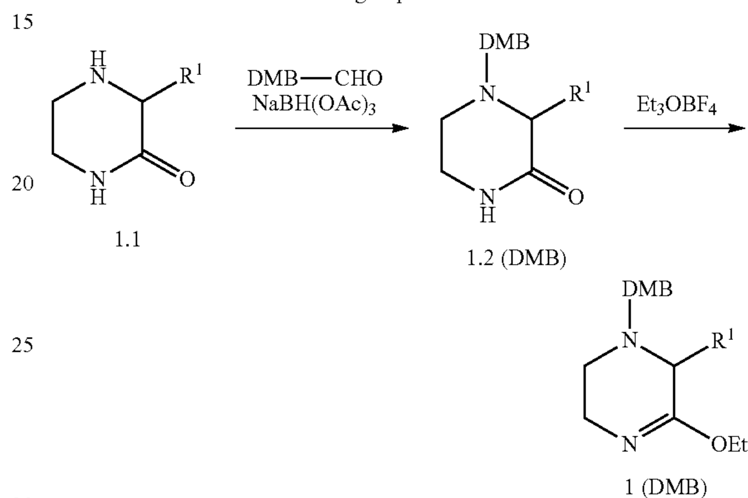
Scheme 5: Protection with DMB group and conversion to iminoether 1
