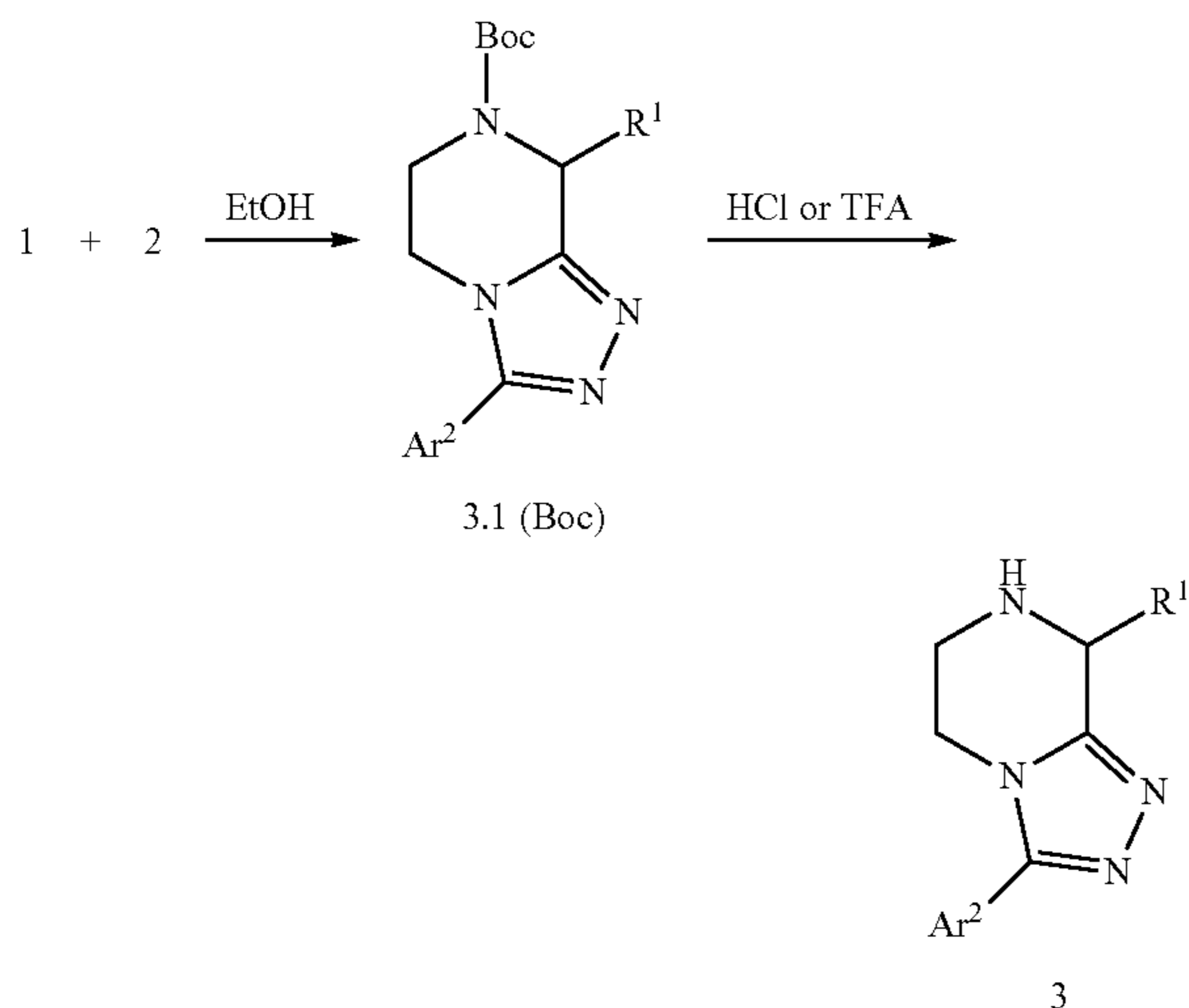
Scheme 16: Cyclodehydration leading to triazolopiperazine 3
