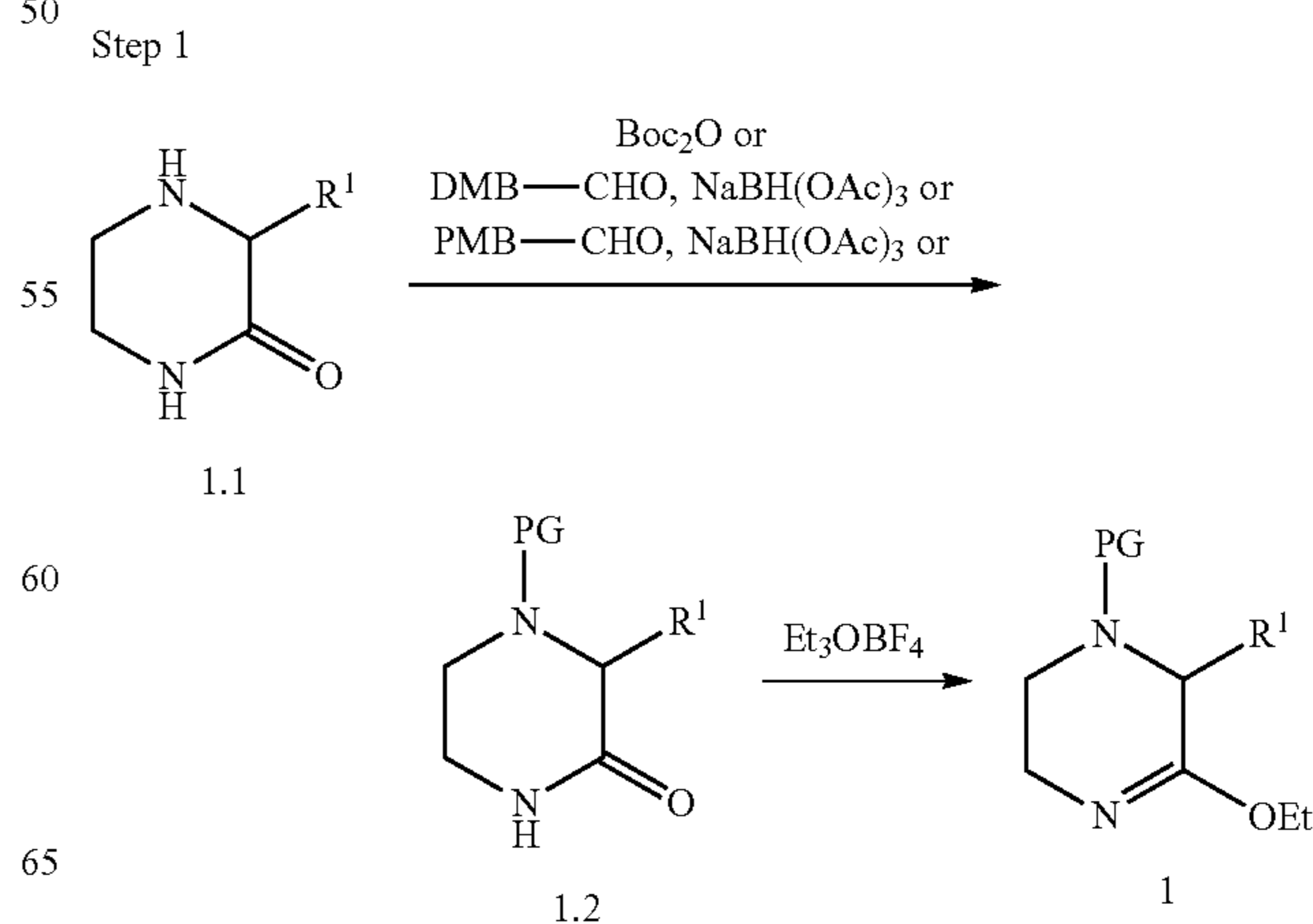
Scheme 1: General racemic synthetic scheme for the preparation of the compounds of the invention.
