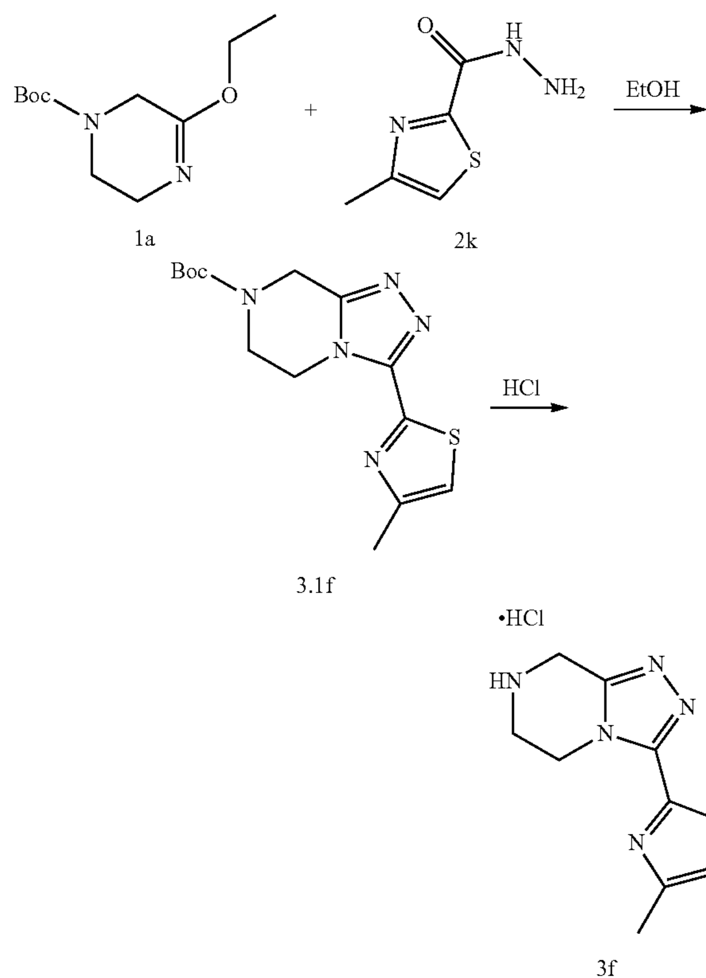
Scheme 18: Synthesis of 4-methyl-2-(5,6,7,8-tetrahydro-[1,2,4]triazolo[4,3-a]pyrazin-3-yl)thiazole 3f
