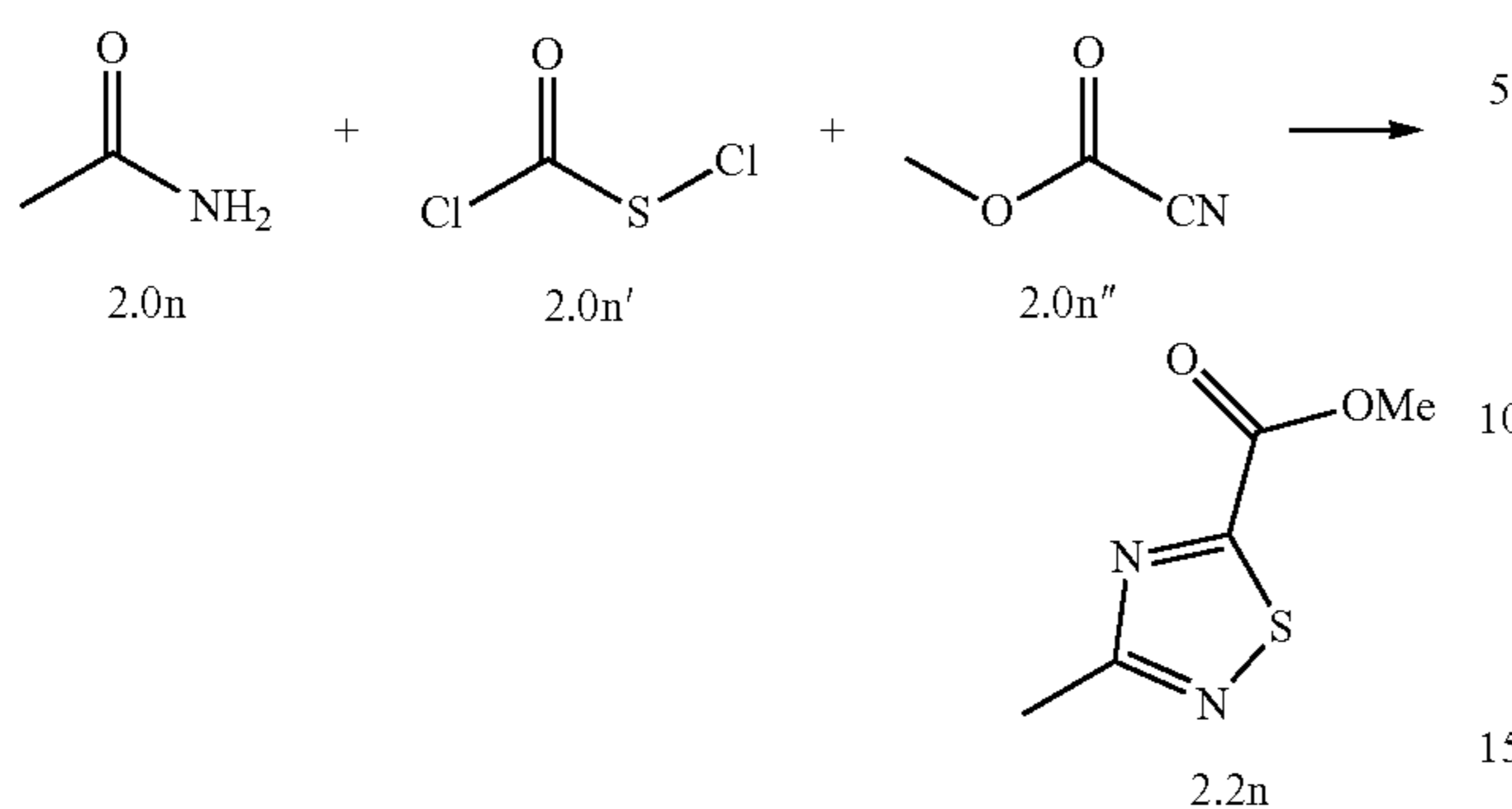
Scheme 12: Synthesis of methyl 3-methyl-1,2,4-thiadiazole-5-carboxylate 2.2n
