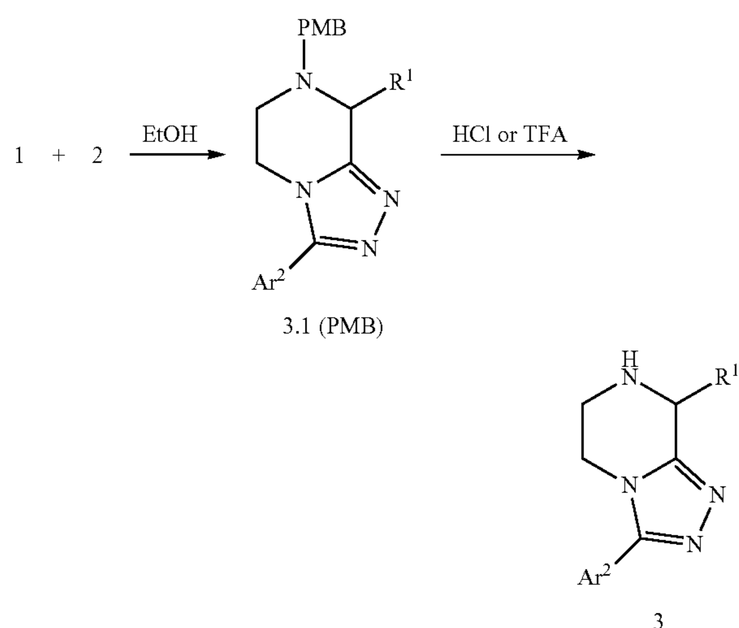
Scheme 23: Cyclodeshydration leading to triazolopiperazine 3
