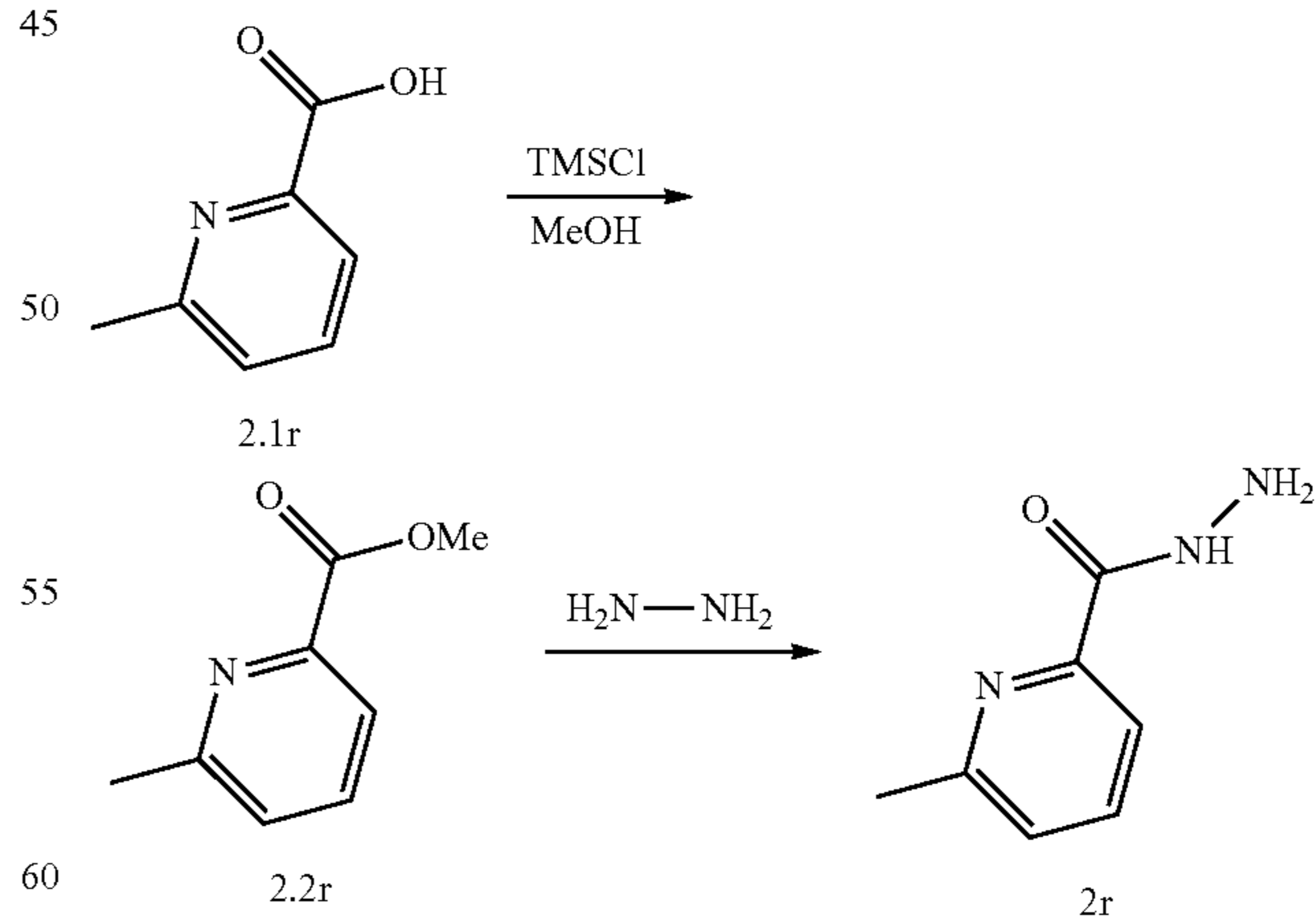
Scheme 15: Synthesis of 6-methylpicolinohydrazide 2r.
