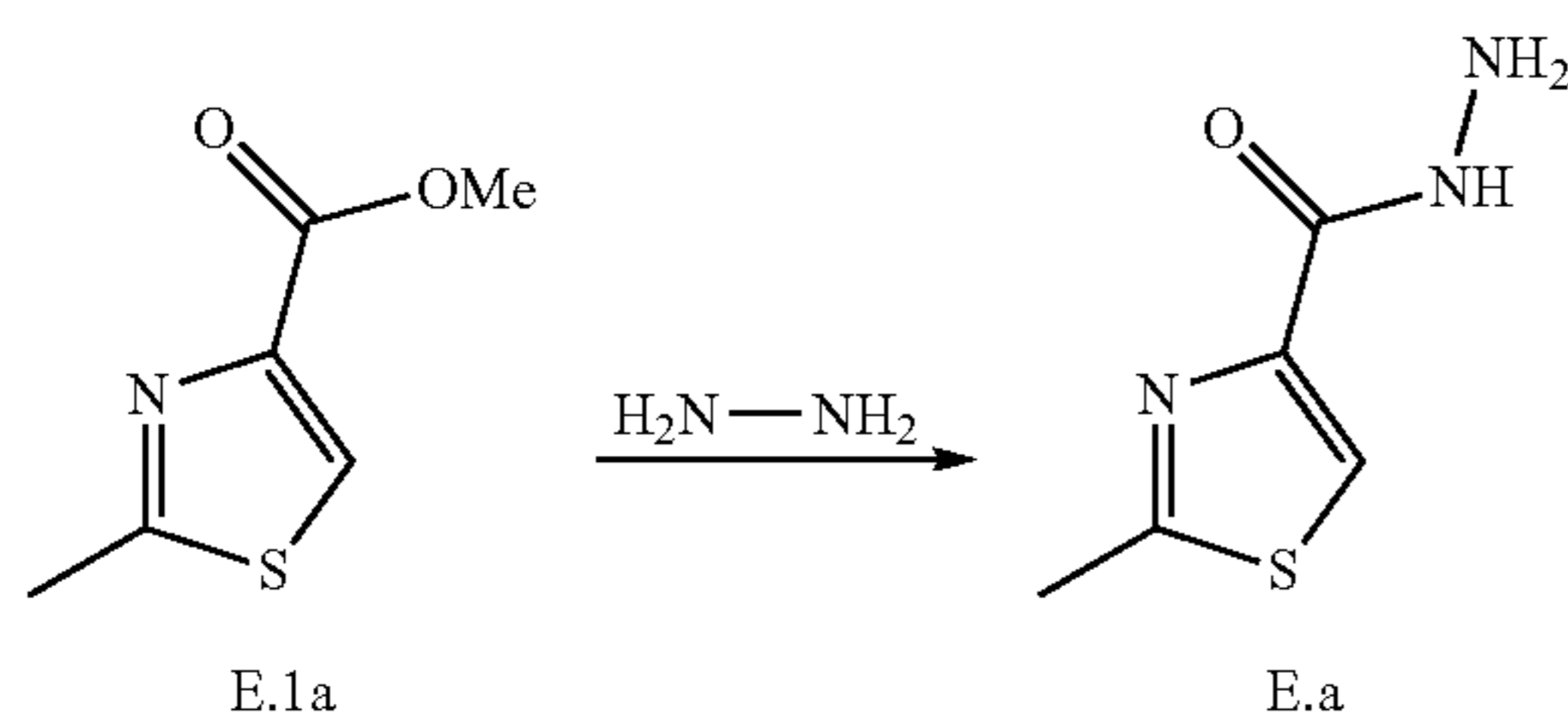
Scheme 31: Synthesis of 2-methylthiazole-4-carbohydrazide E.a
