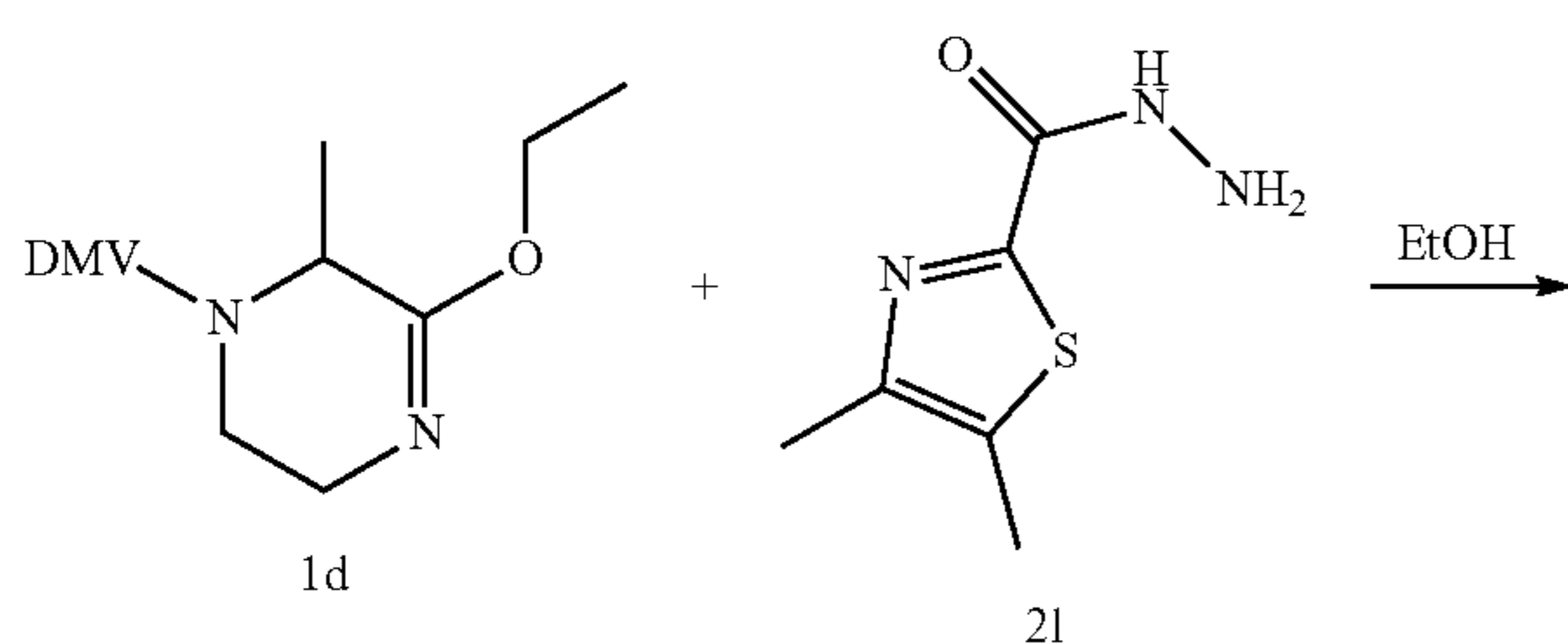
Scheme 22: Synthesis of 4,5-dimethyl-2-(8-methyl-5,6,7,8-tetrahydro-[1,2,4]triazolo[4,3-a]pyrazin-3-yl)thiazole hydrochloride 3q
