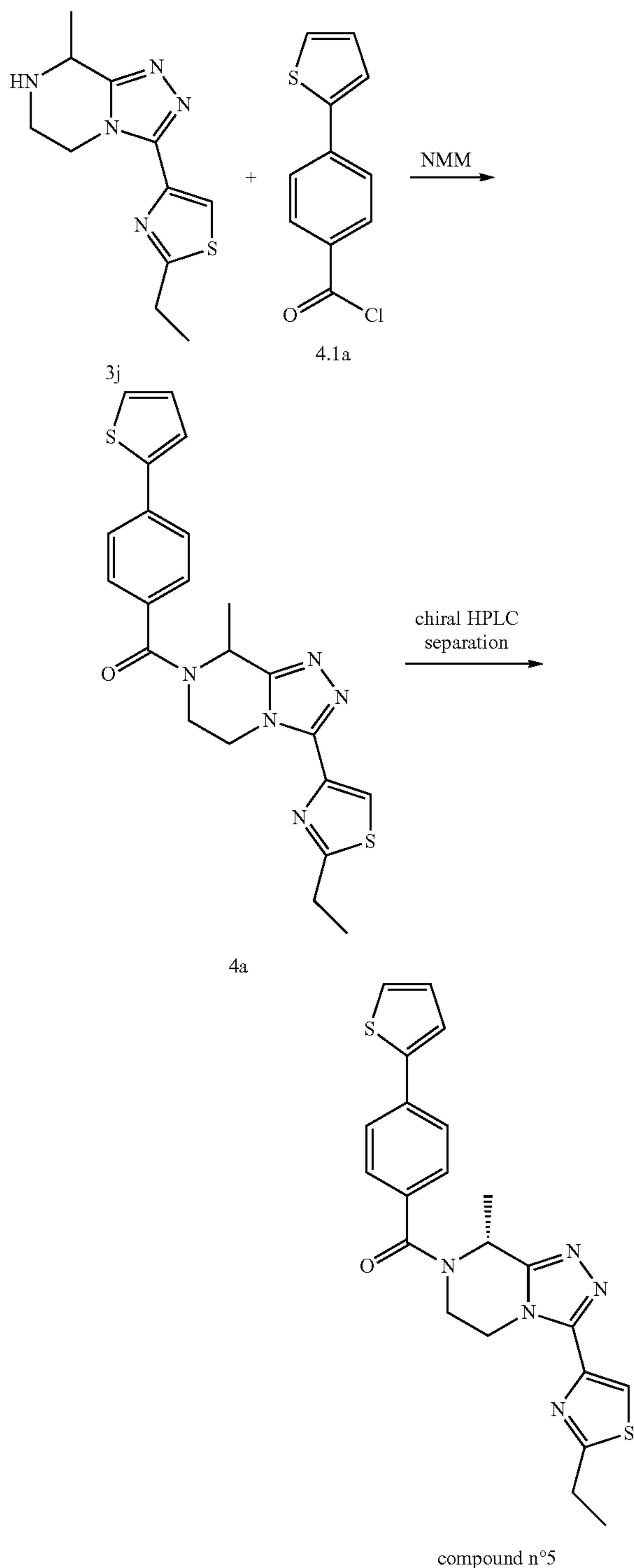
Scheme 26: Synthesis of compounds 4a and n o 5
