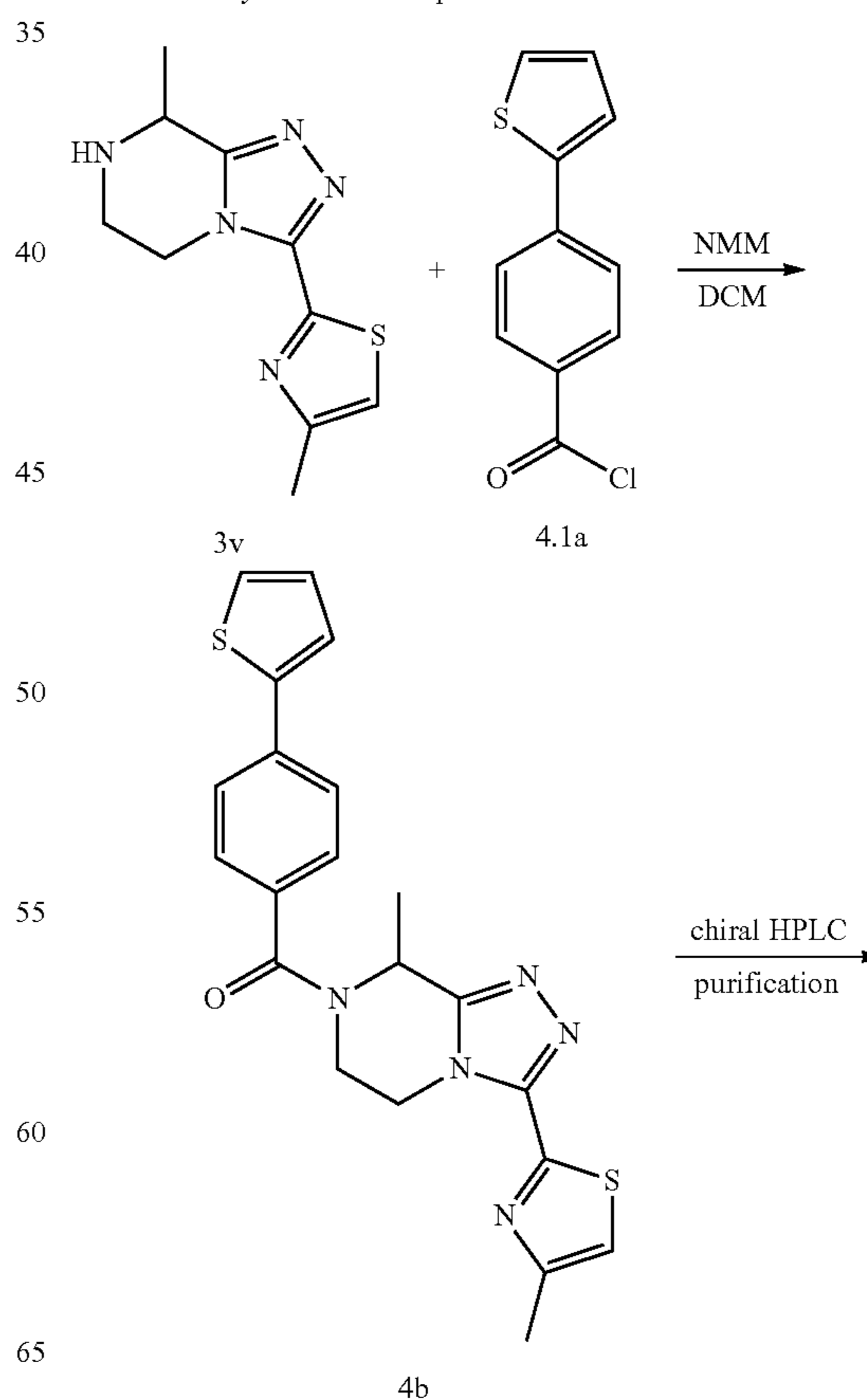
Scheme 27: Synthesis of compounds 4b and n o 19
