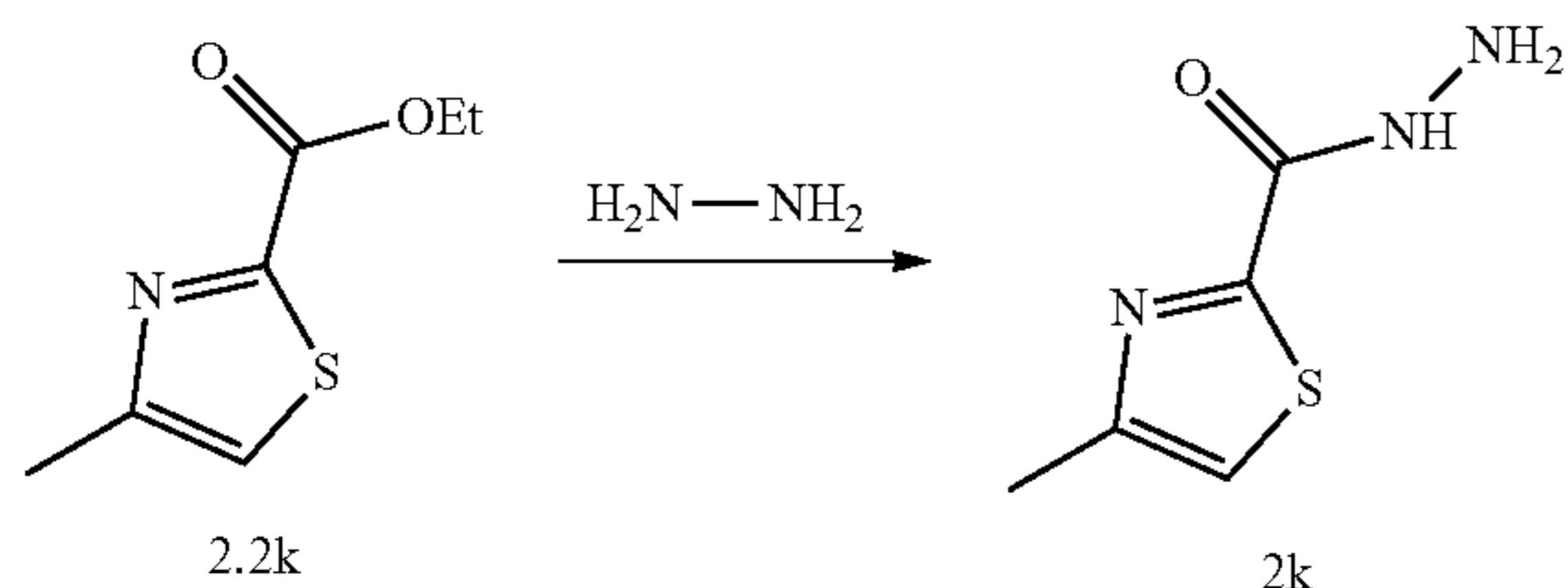
Scheme 9: Synthesis of 4-methylthiazole-2-carbohydrazide 2k
