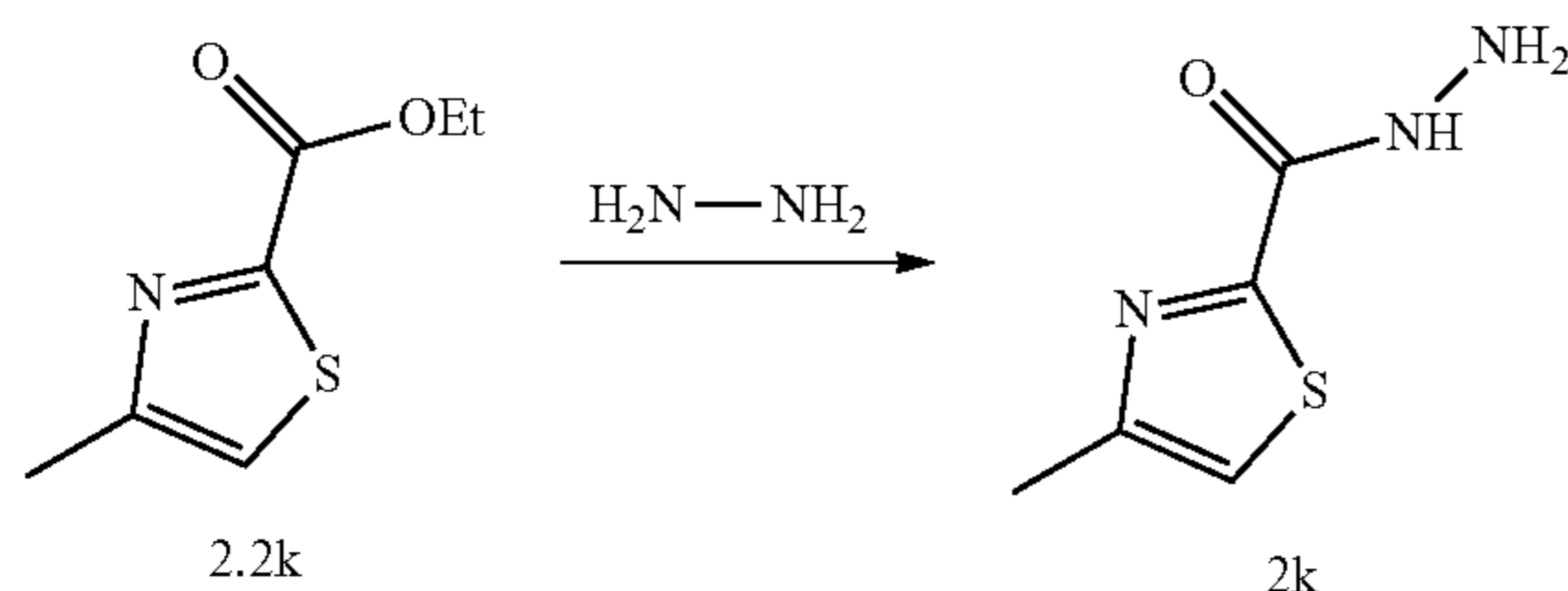
Scheme 9: Synthesis of 4-methylthiazole-2-carbohydrazide 2k
