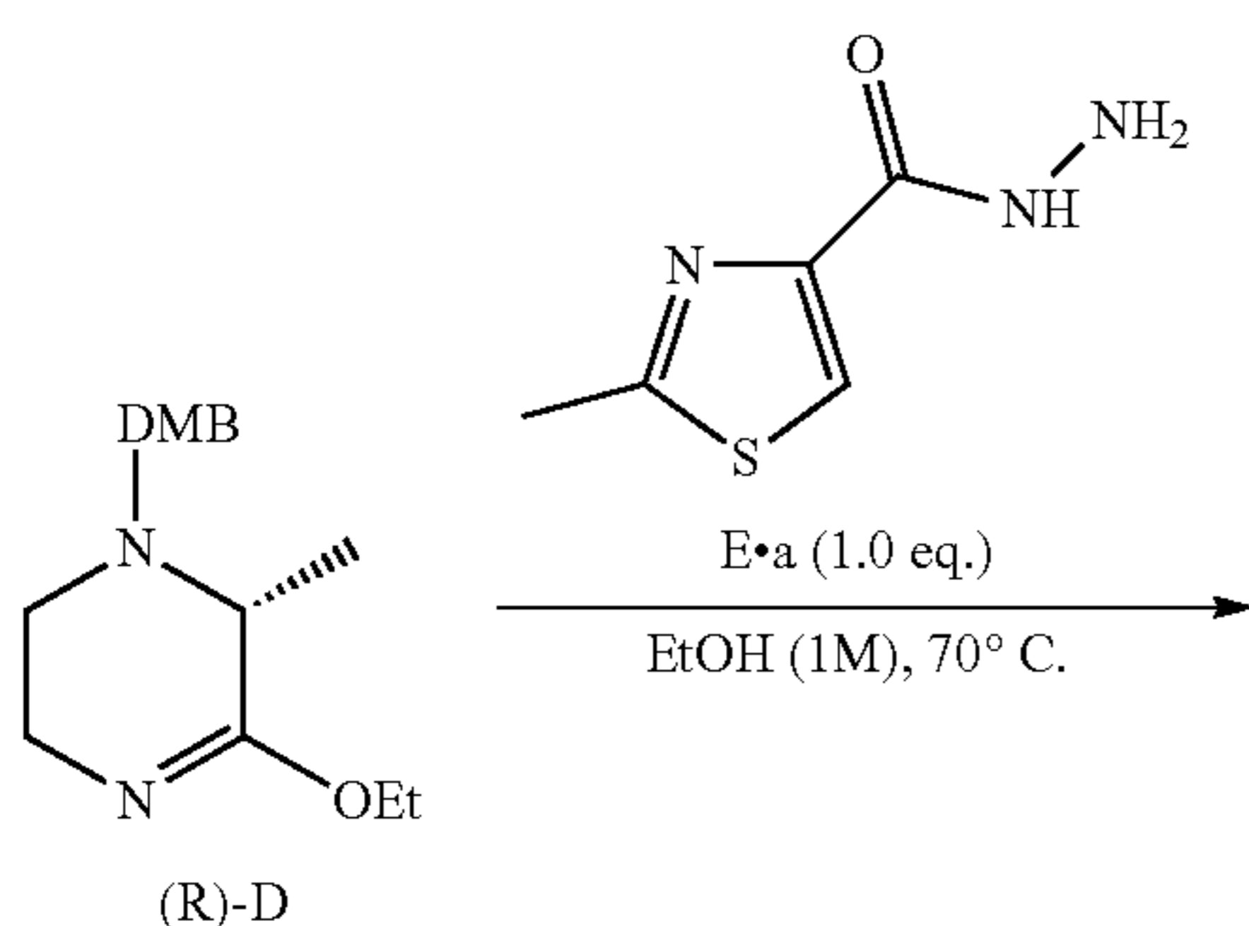
Scheme 32: Synthesis of (R)-4-(7-(2,4-dimethoxybenzyl)-8-methyl-5,6,7,8-tetrahydro-[1,2,4]triazolo[4,3-a]pyrazin-3-yl)-2-methylthiazole(R)-F.a
