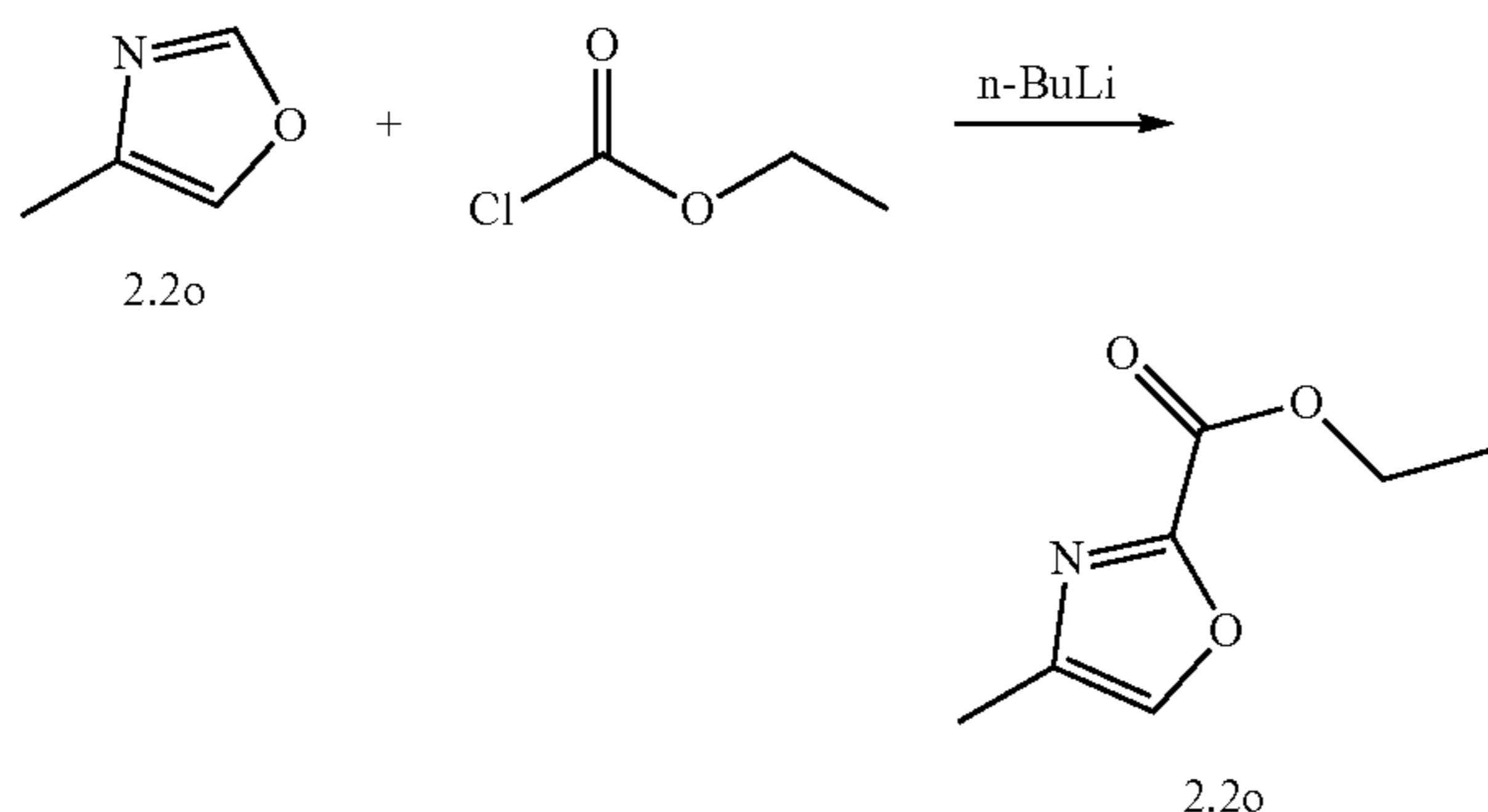
Scheme 13: Synthesis of methyl 4-methyloxazole-2-carboxylate 2.2o
