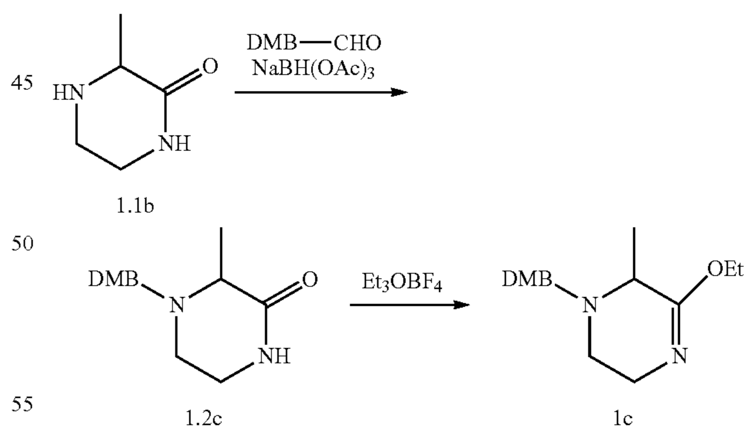
Scheme 6: Synthesis of 1-(2,4-dimethoxybenzyl)-5-ethoxy-6-methyl-1,2,3,6-tetrahydropyrazine 1c
