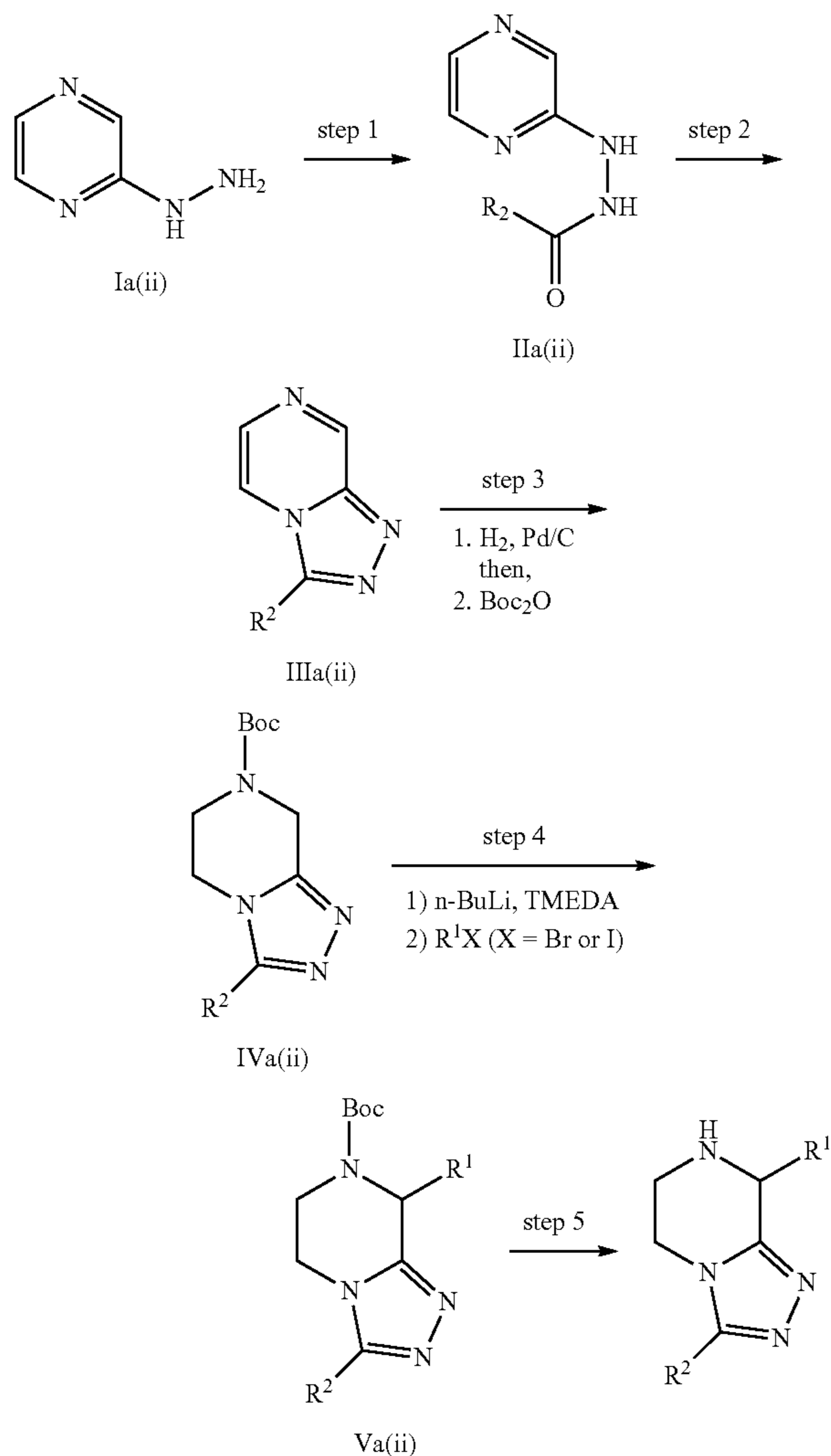
Scheme B: Method A(ii)
