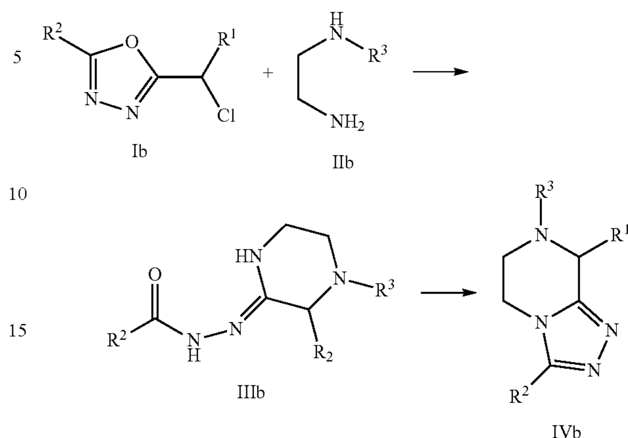
Scheme C: Method B
