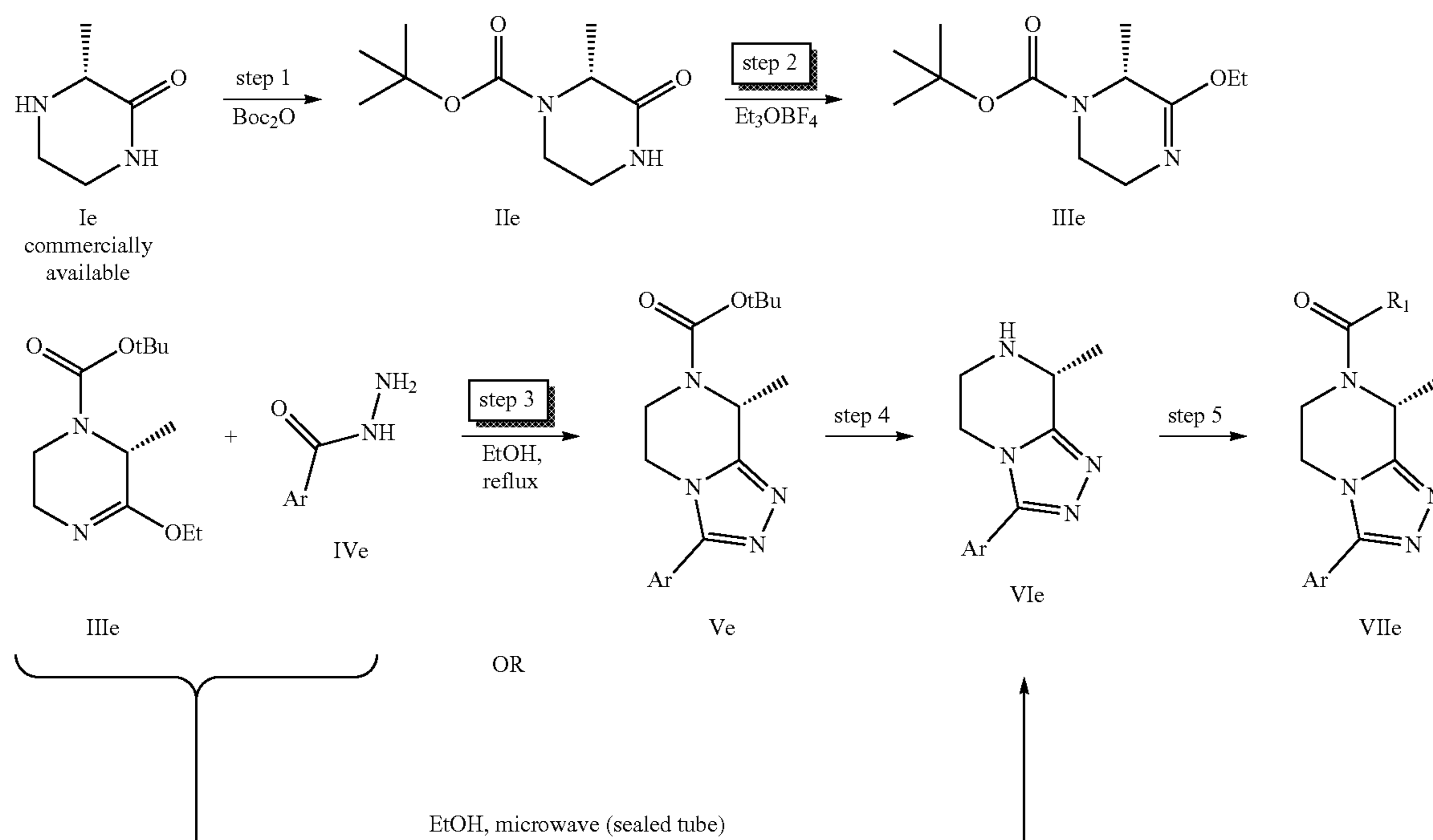
Scheme E: Synthesis of (R)-8-methyl-5,6,7,8-tetrahydro-[1,2,4]triazolo[4,3-a]pyrazine intermediates according to PCT/EP2011/055218.
