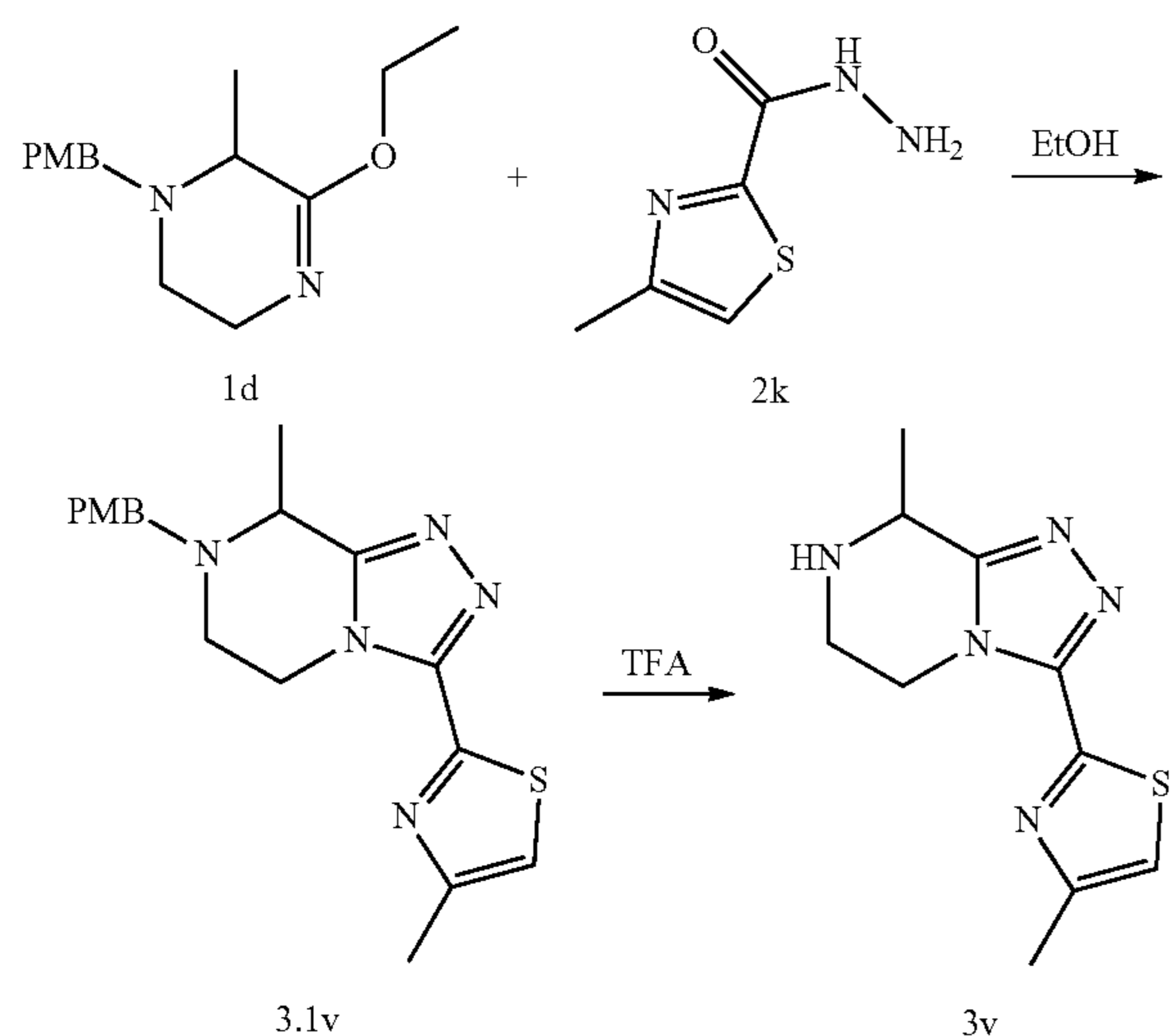
Scheme 24: Synthesis of 4-methyl-2-(8-methyl-5,6,7,8-tetrahydro-[1,2,4]triazolo[4,3-a]pyrazin-3-yl)thiazole 3v
