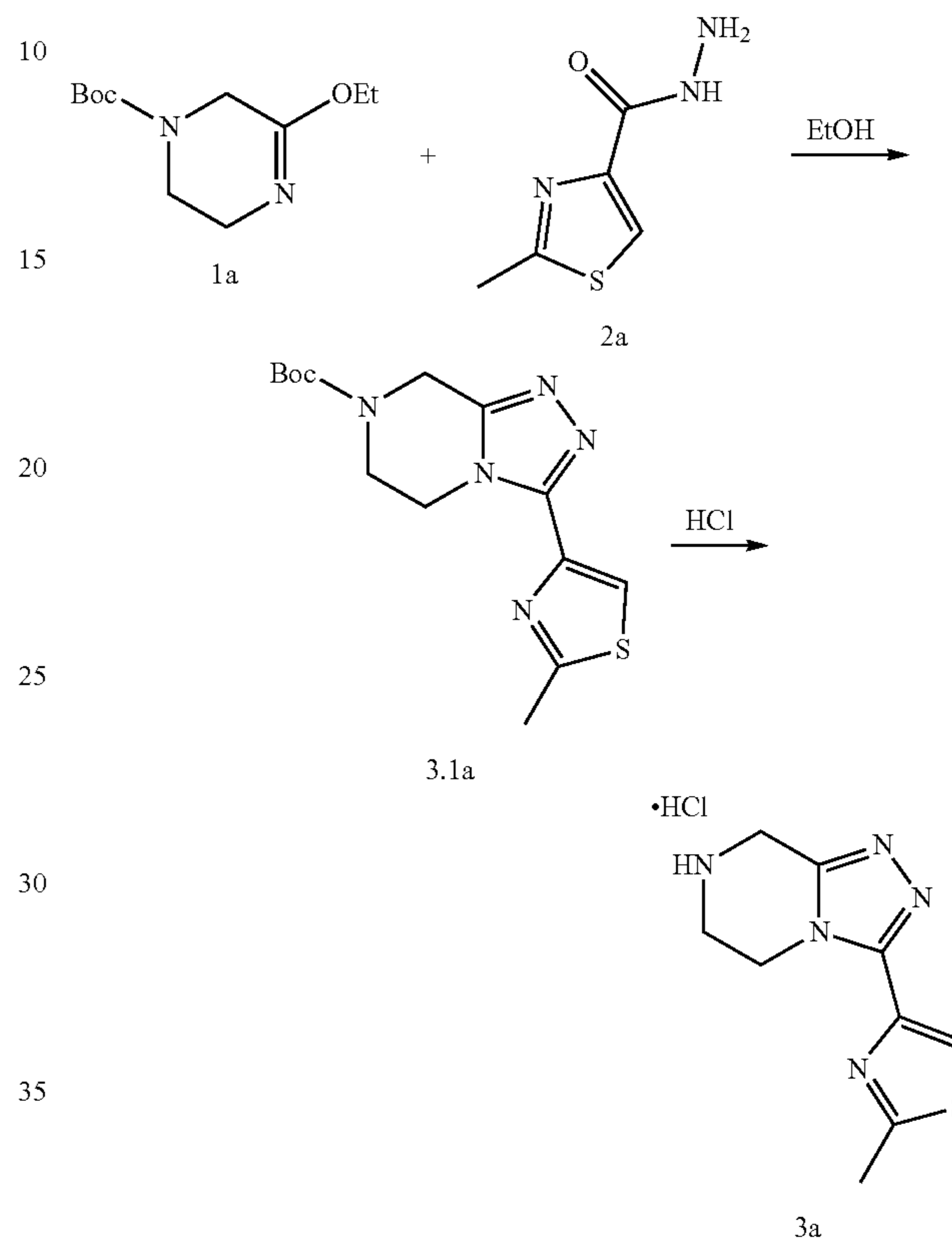
Scheme 17: Synthesis of 2-methyl-4-(5,6,7,8-tetrahydro-[1,2,4]triazolo[4,3-a]pyrazin-3-yl)thiazole hydrochloride 3a
