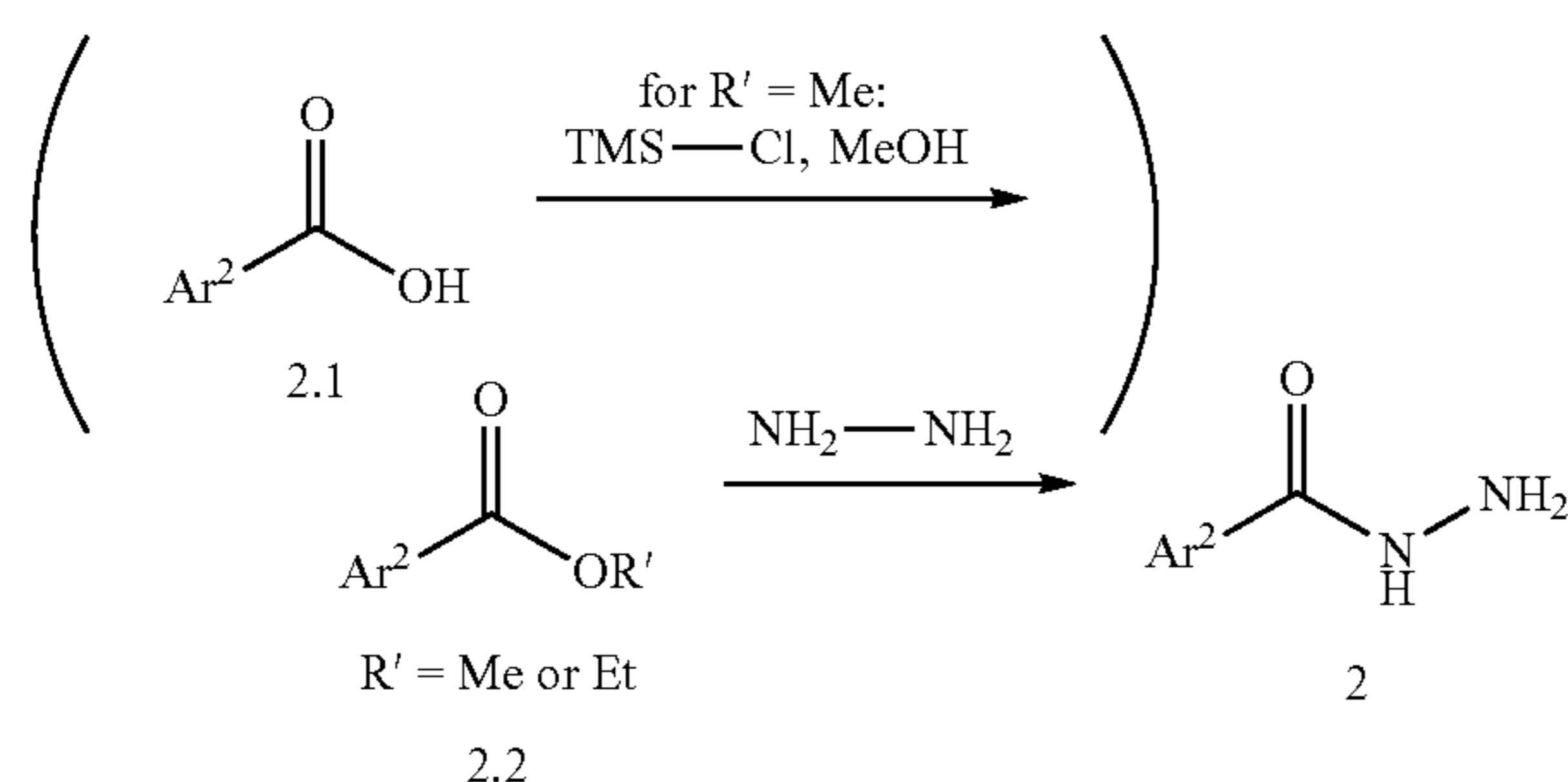
Scheme 7: Formation of acylhydrazide 2
