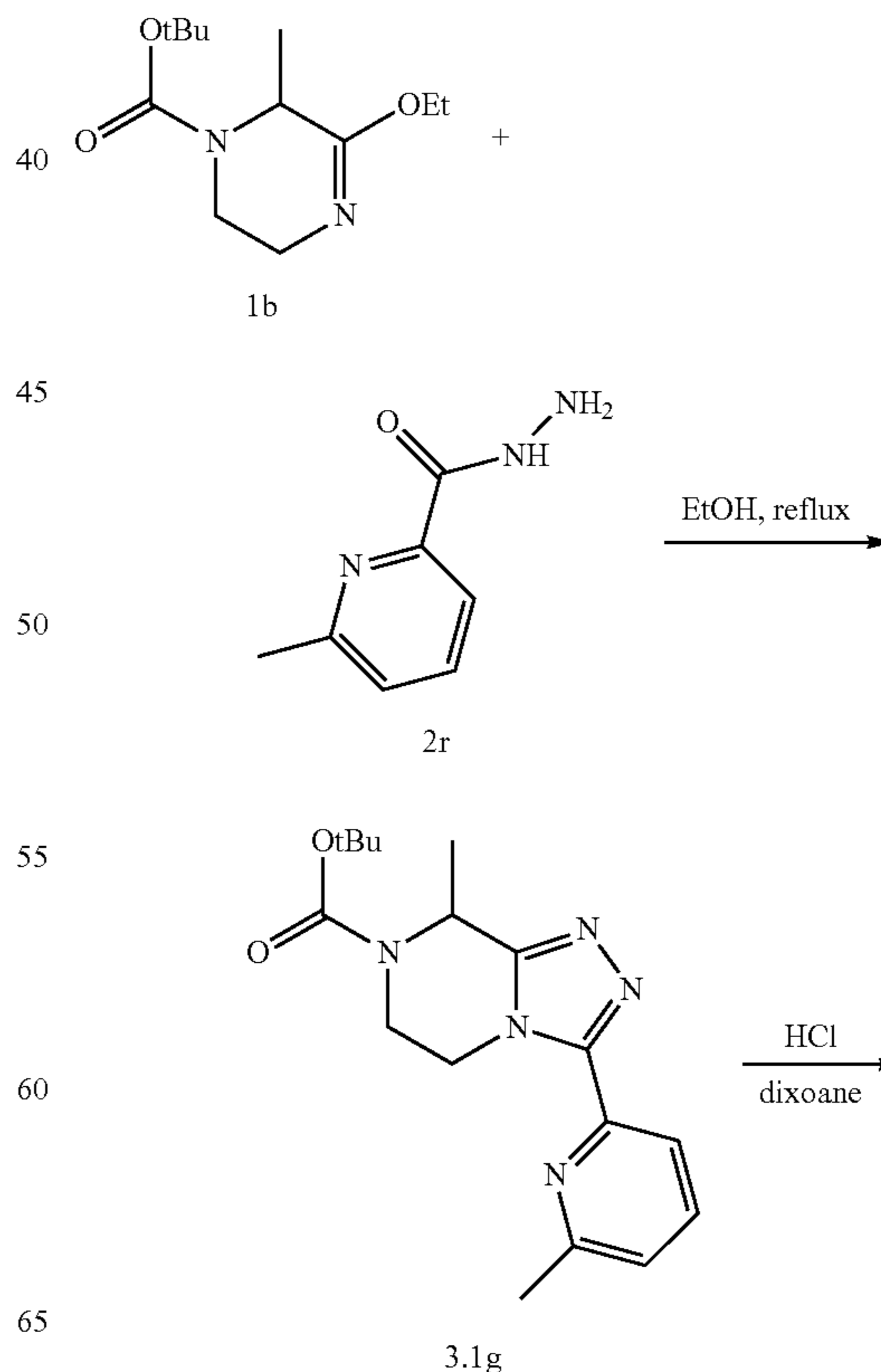
Scheme 19: Synthesis of 8-methyl-3-(6-methylpyridin-2-yl)-5,6,7,8-tetrahydro-[1,2,4]triazolo[4,3-a]pyrazine 3g
