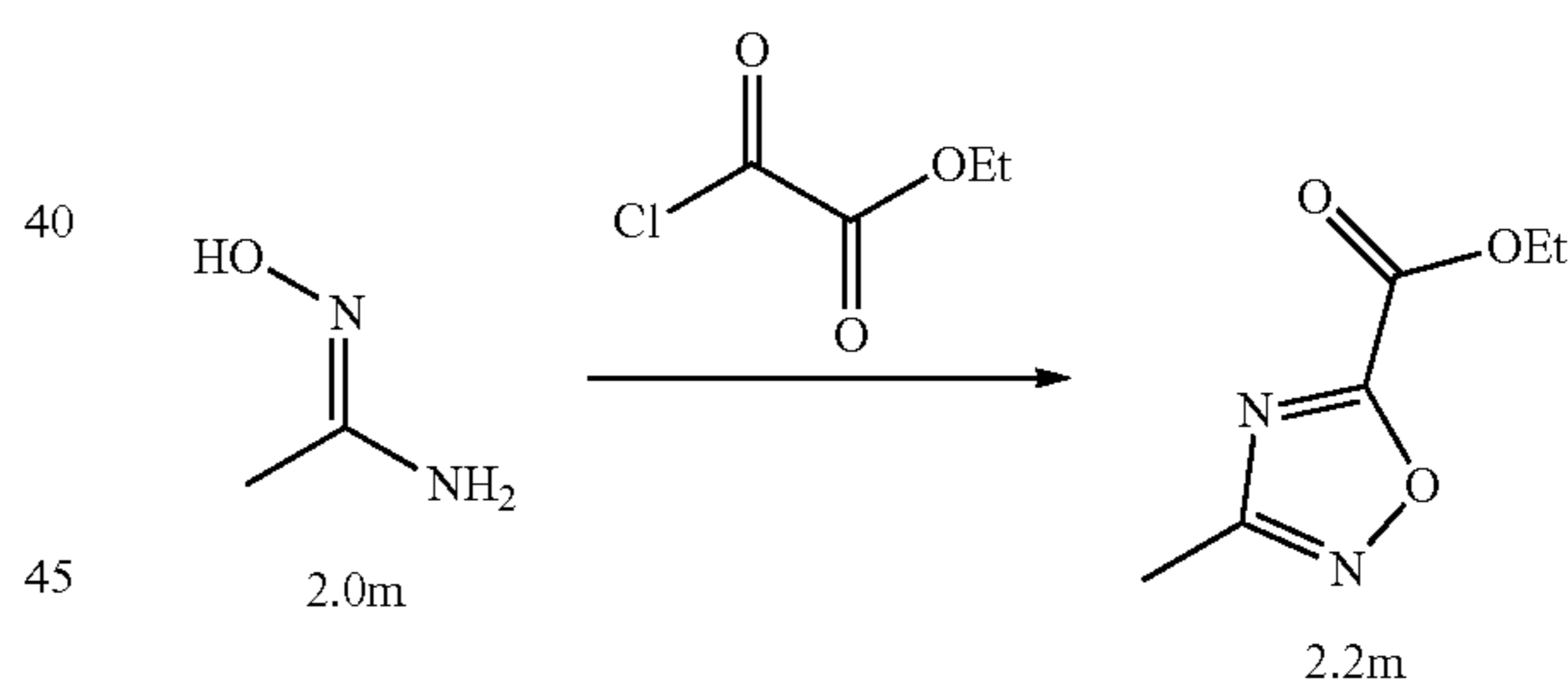
Scheme 11: Synthesis of ethyl 3-methyl-1,2,4-oxadiazole-5-carboxylate 2.2m
