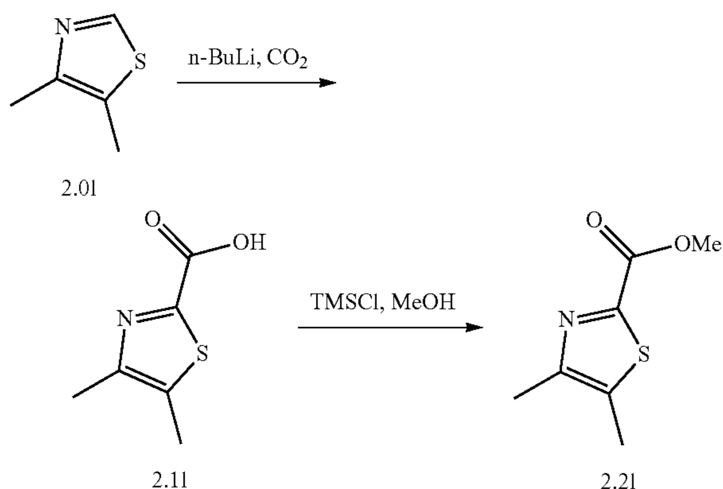
Scheme 10: Synthesis of methyl 4,5-dimethylthiazole-2-carboxylate 2.2l
