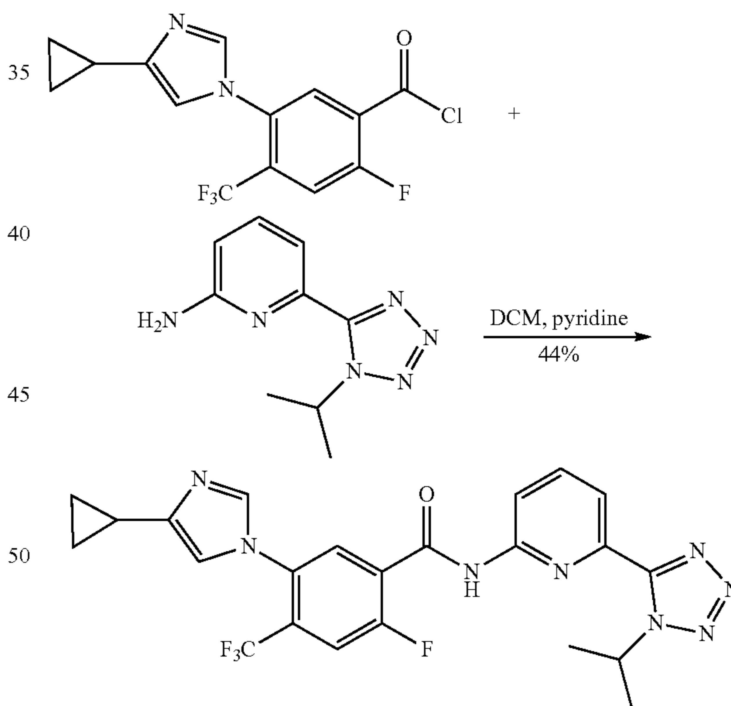
Example 37a
