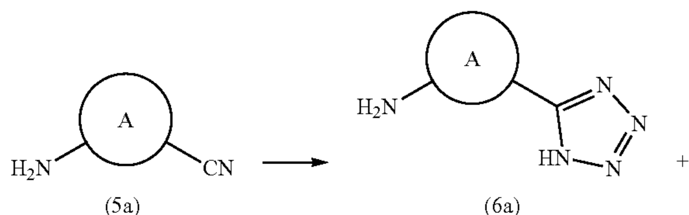
Scheme 4
