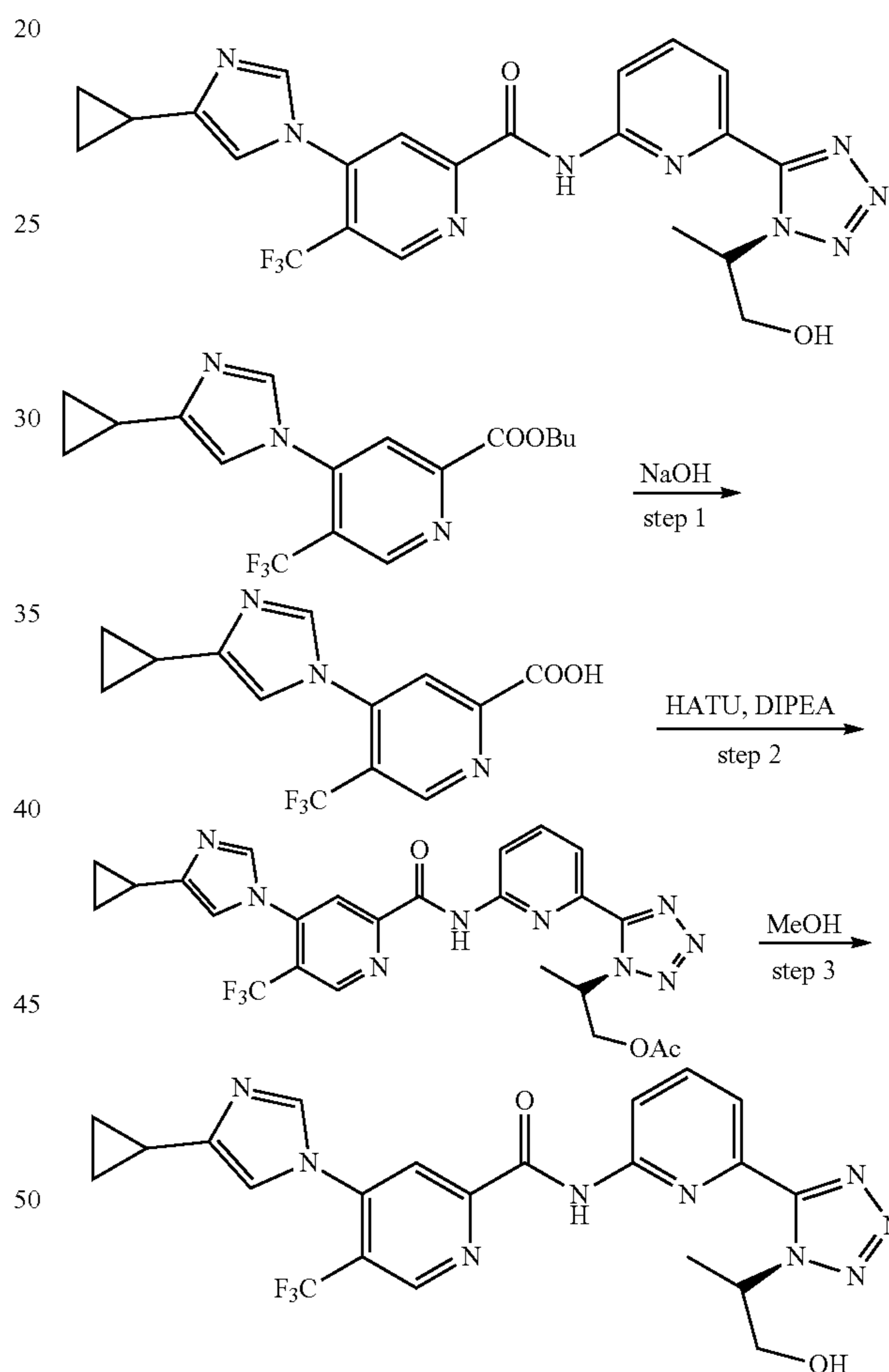
Example 58a
