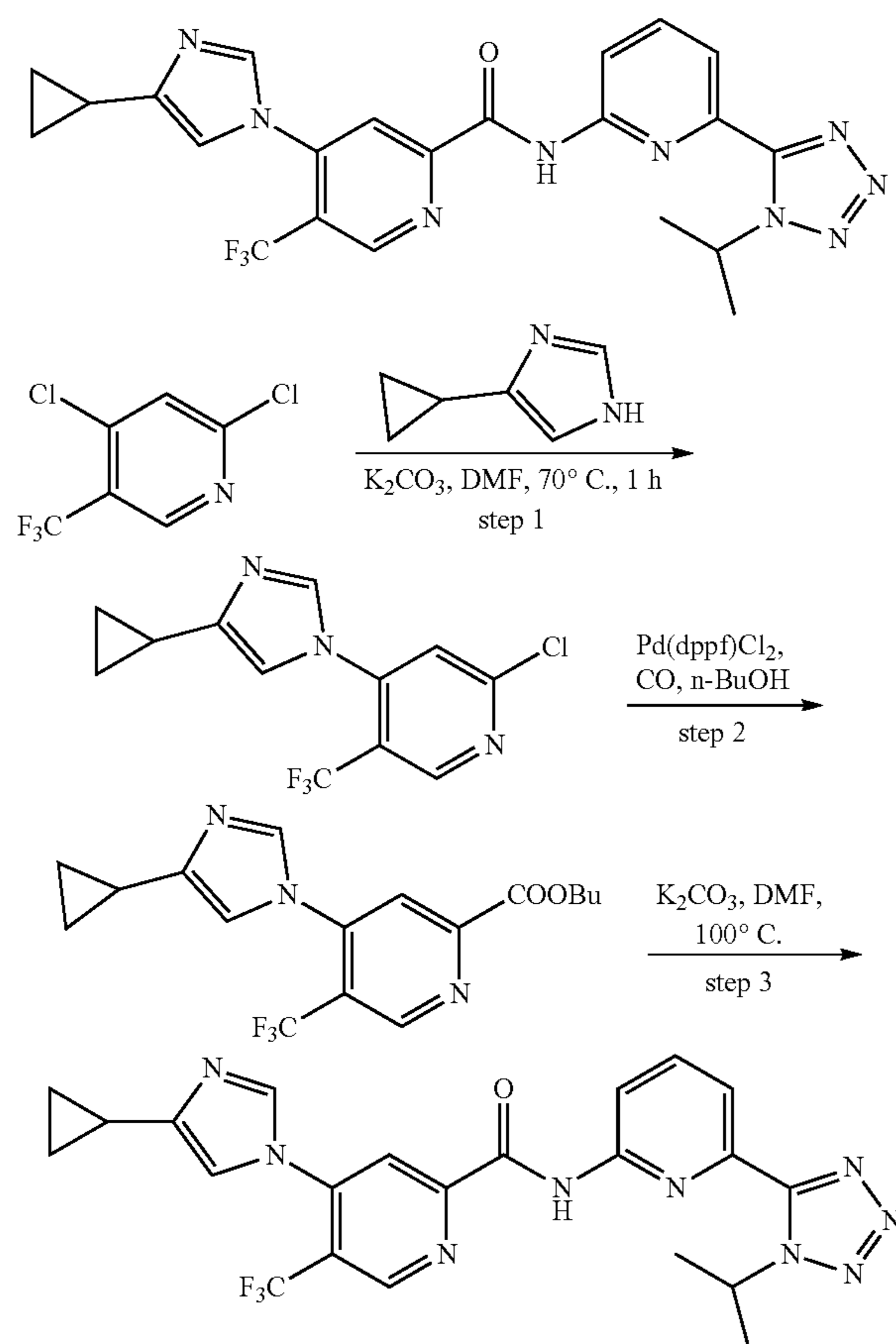
Example 57a
