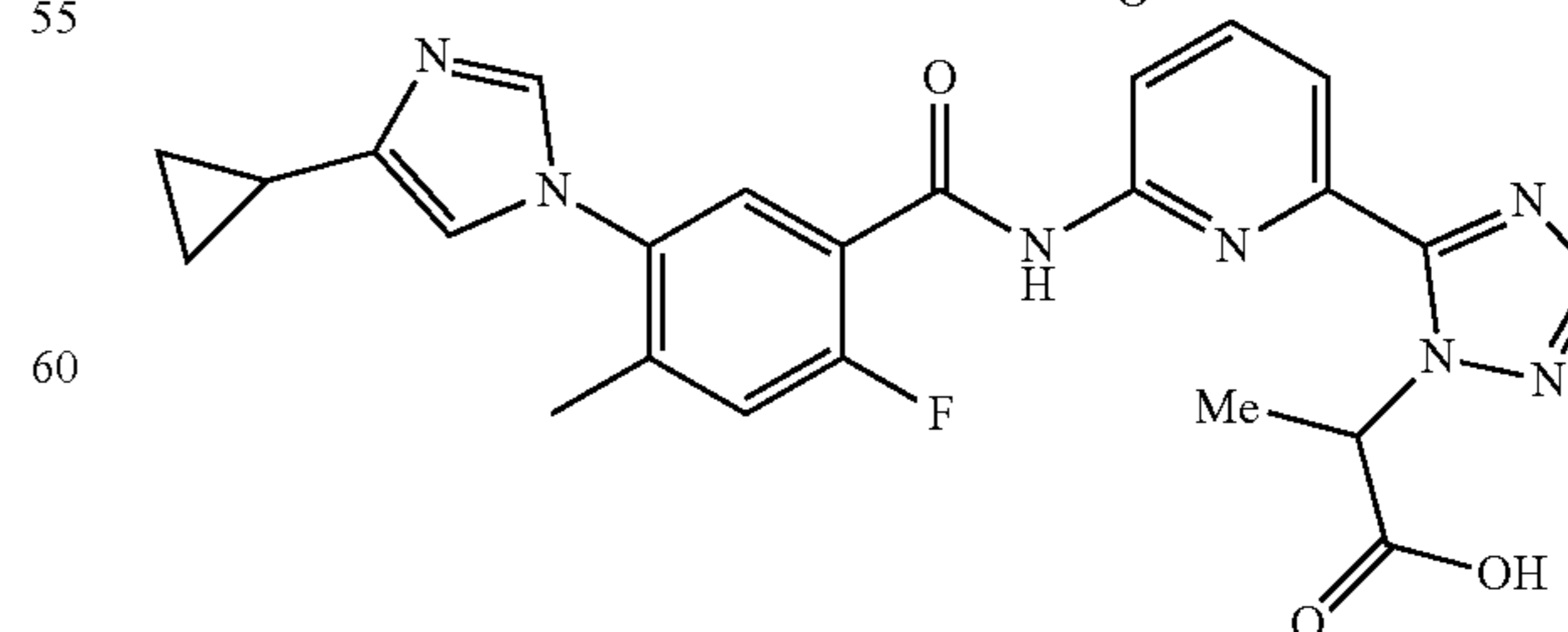
Example 19a
