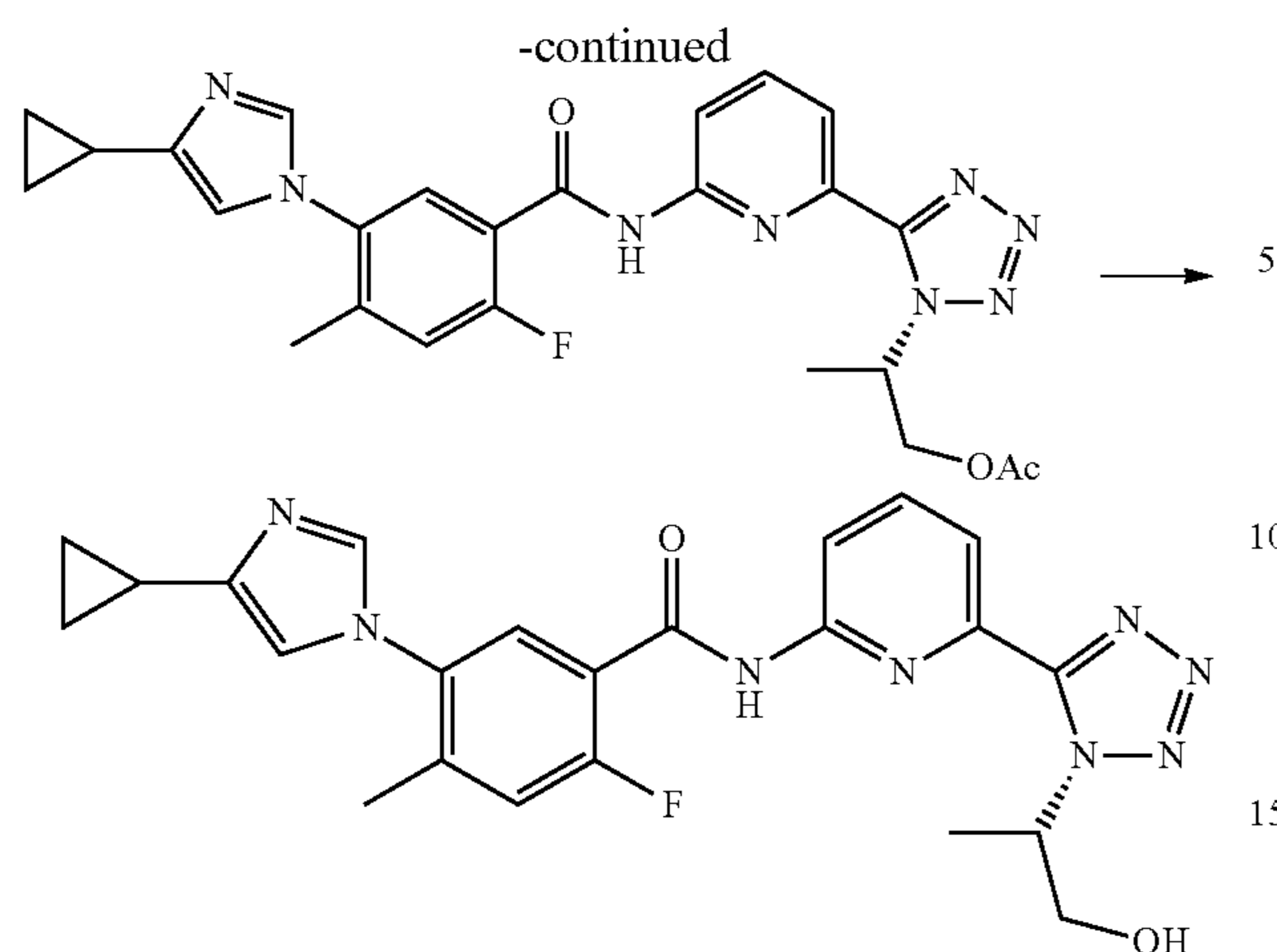
Example 5a
