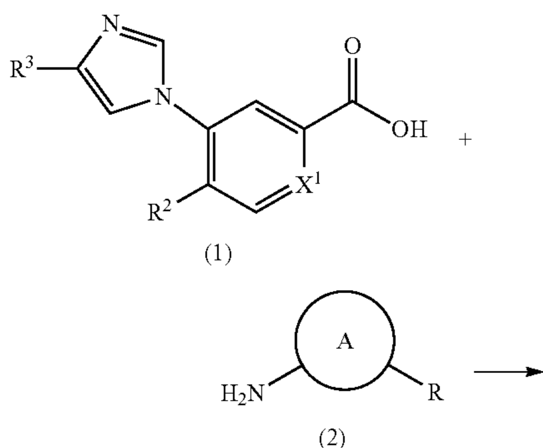
Scheme 1
