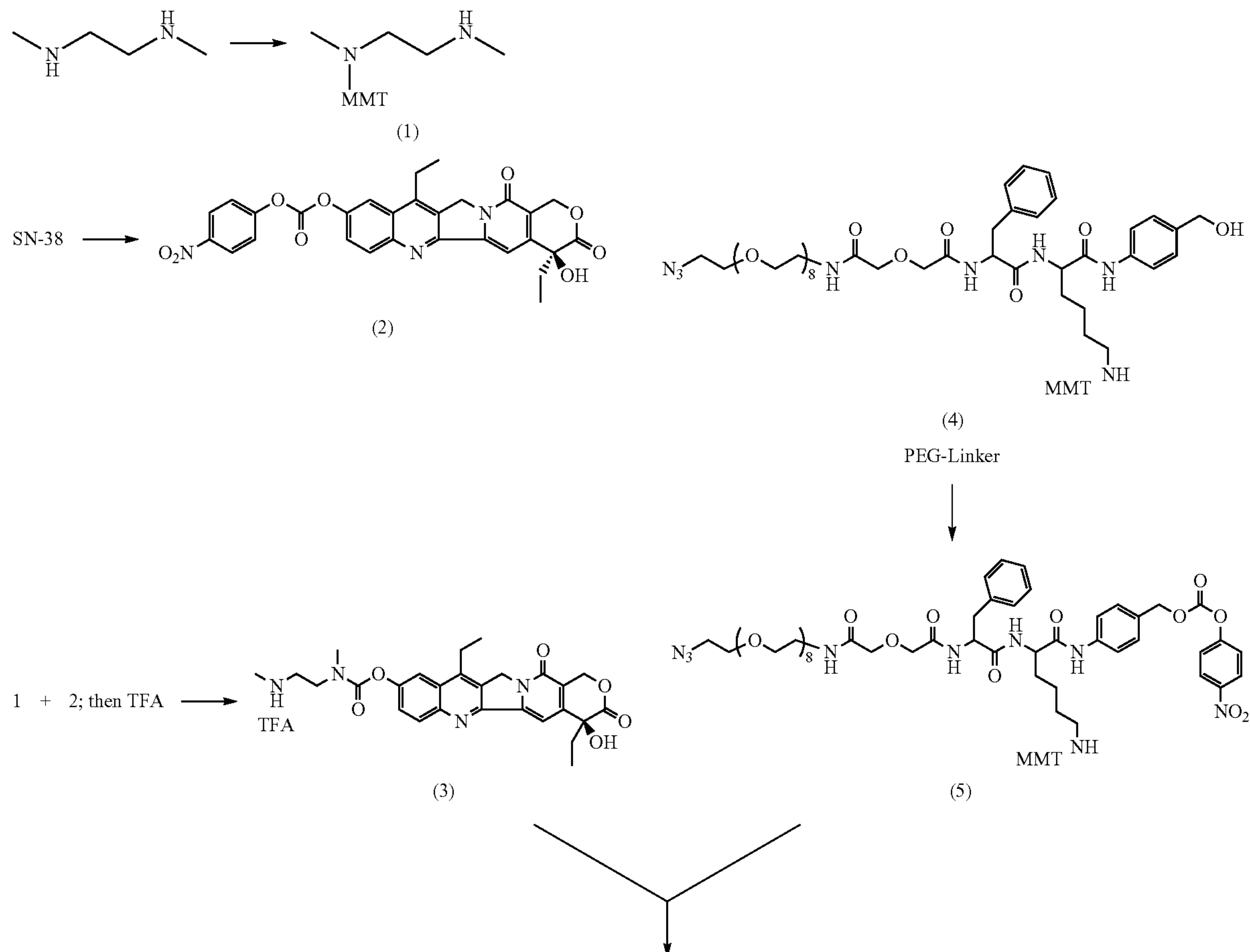
Scheme-4: Preparation of CL2E-SN-38
