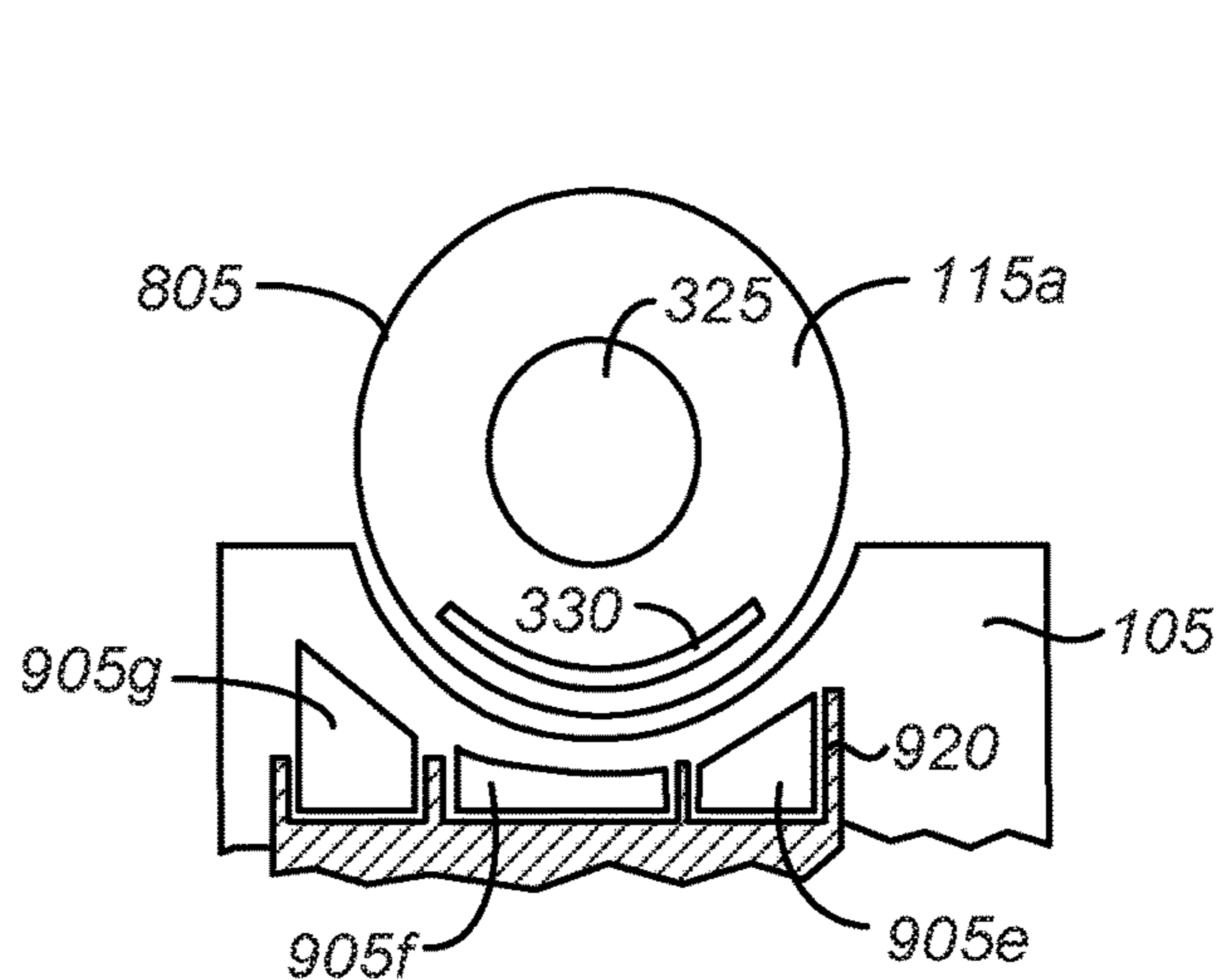
SECTION B-B
