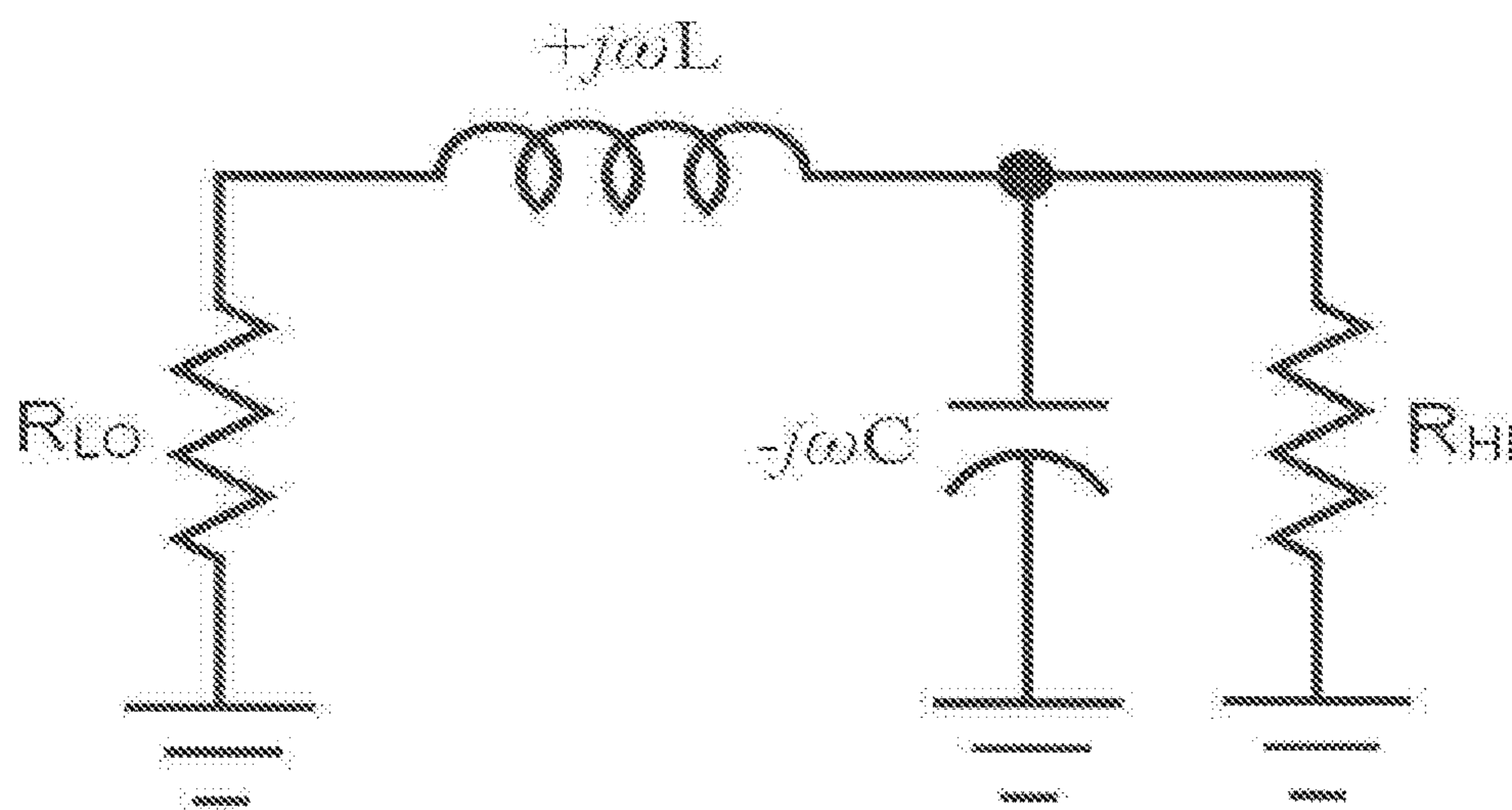
L-Matching network.
