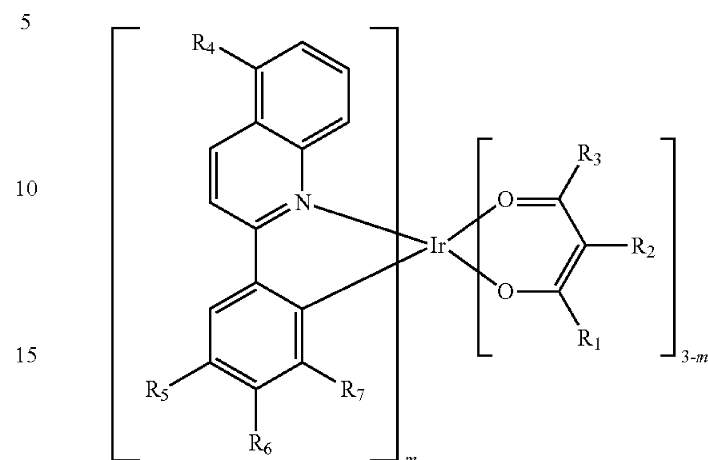
Formula III
