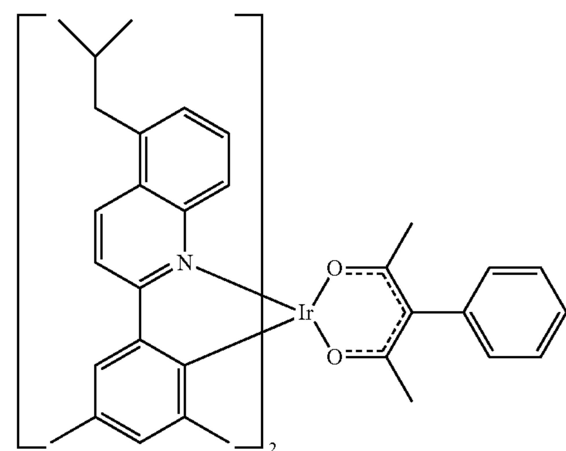
Compound 5
