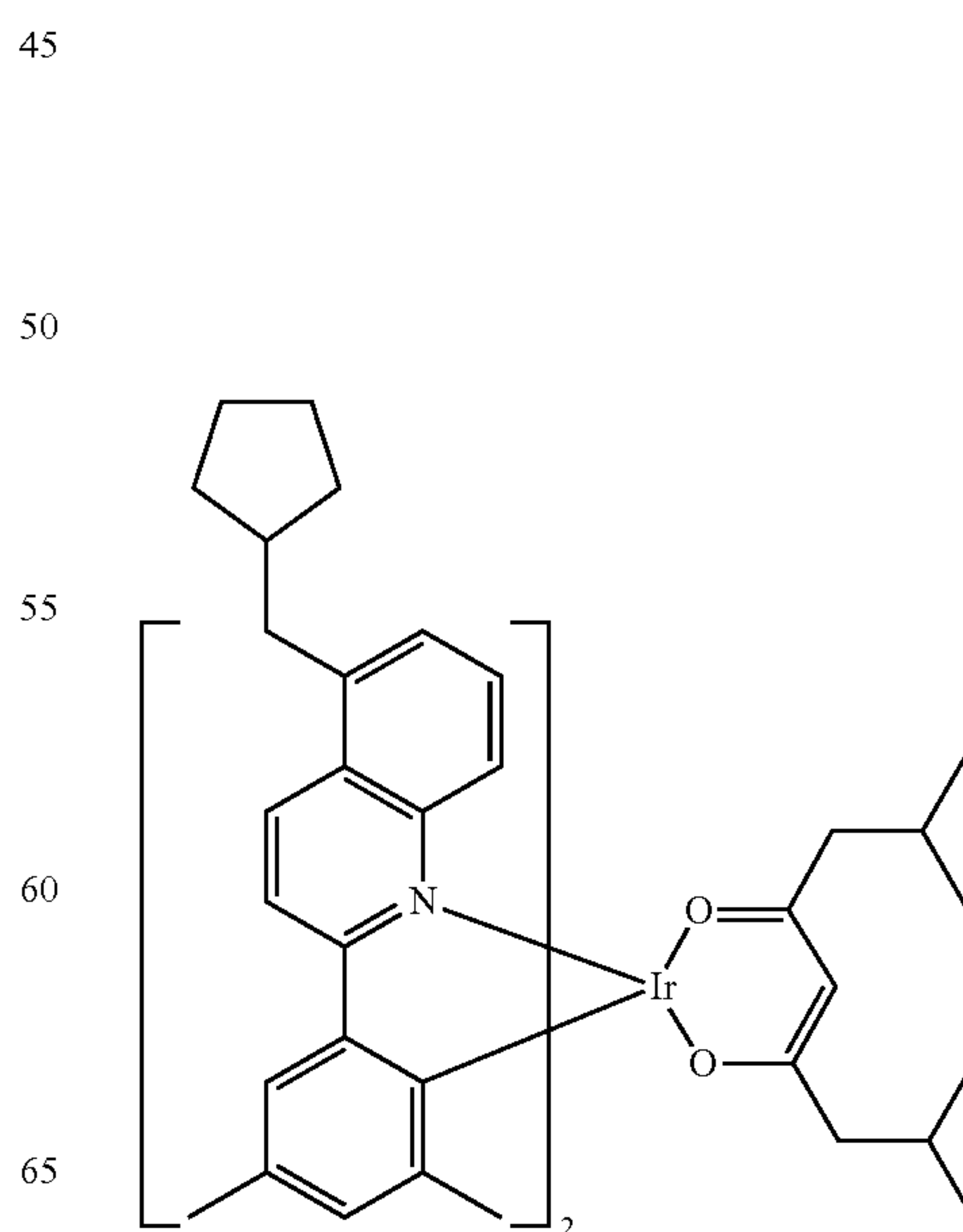
Compound II-26
