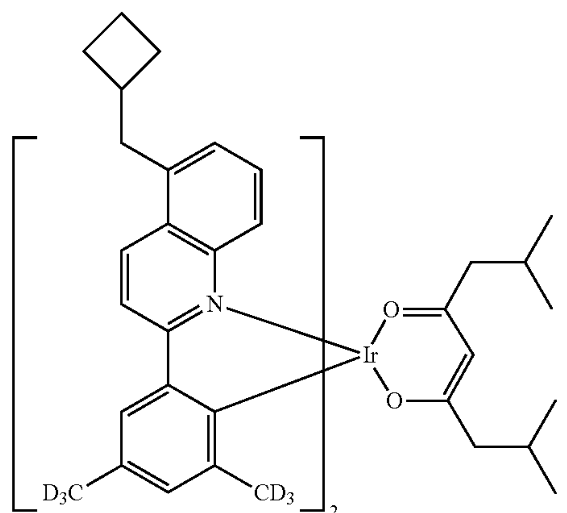
Compound II-61
