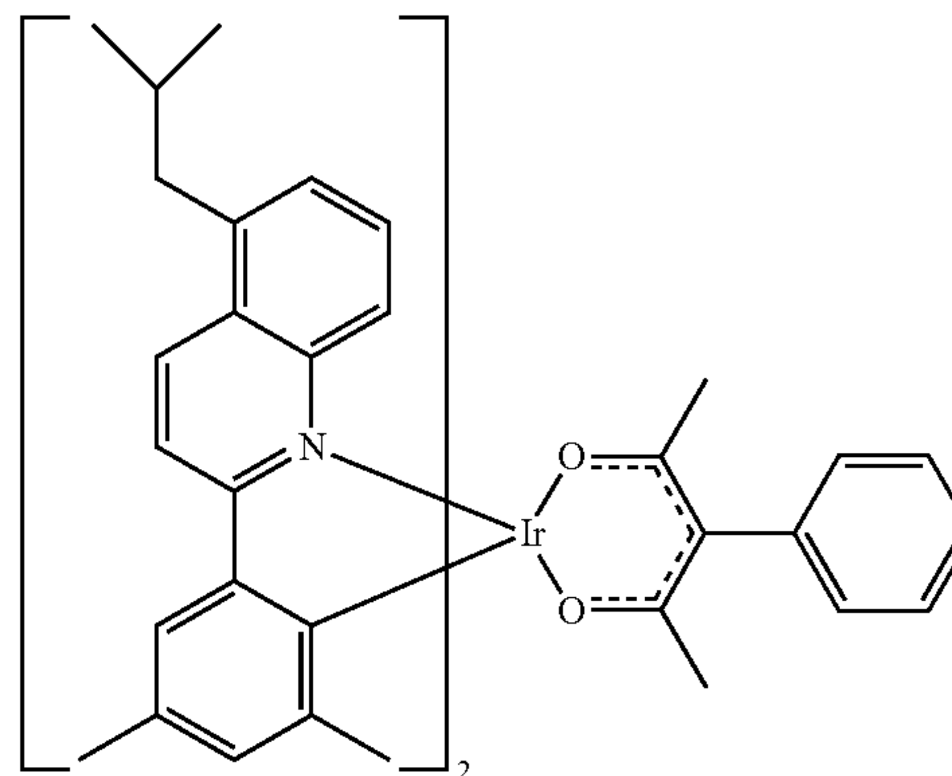
Compound 6
