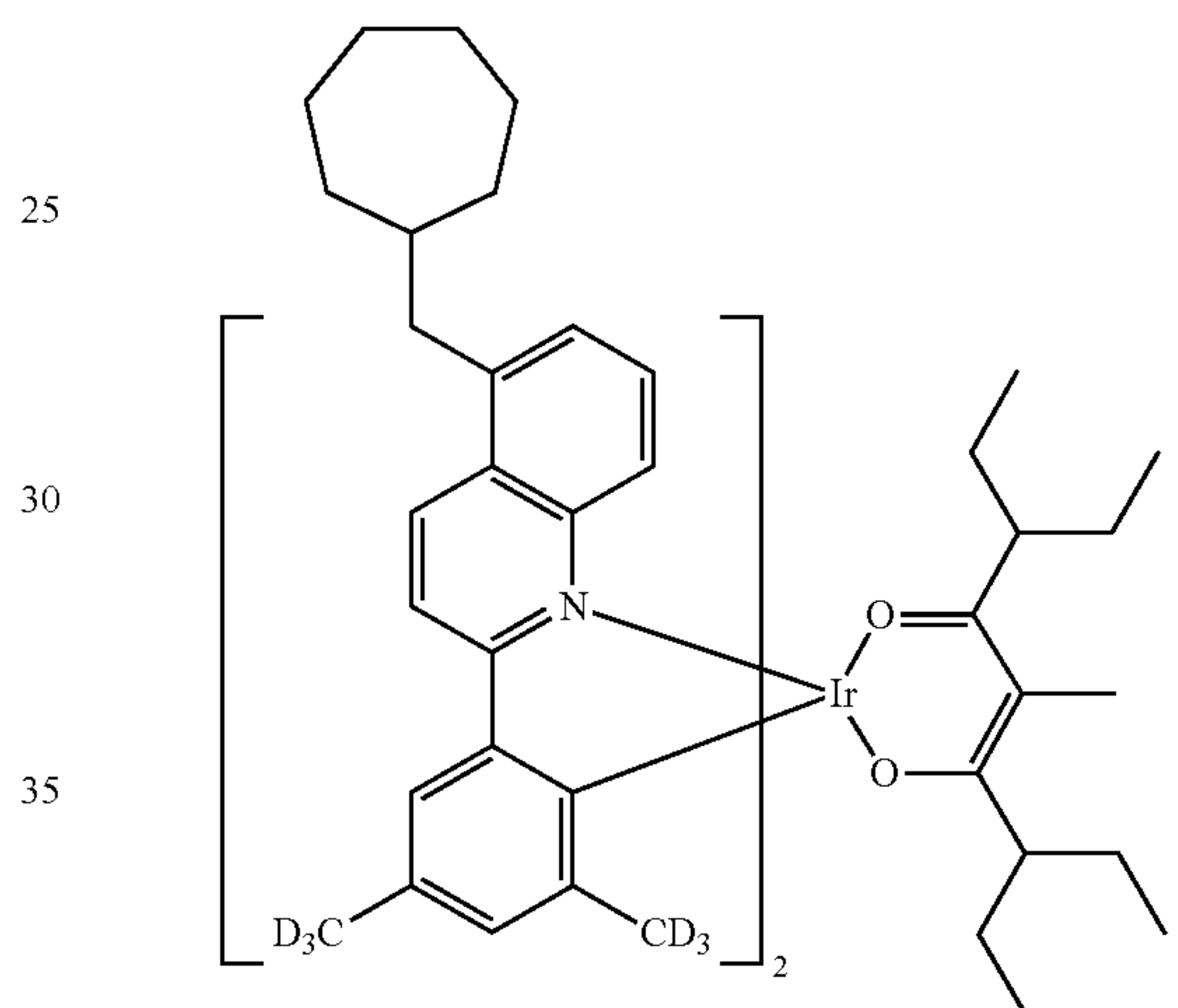
Compound II-72
