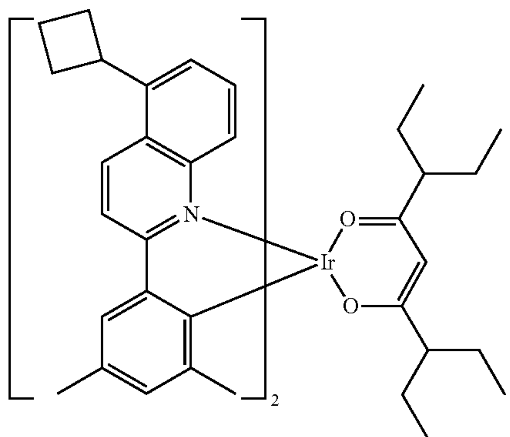
Compound II-14
