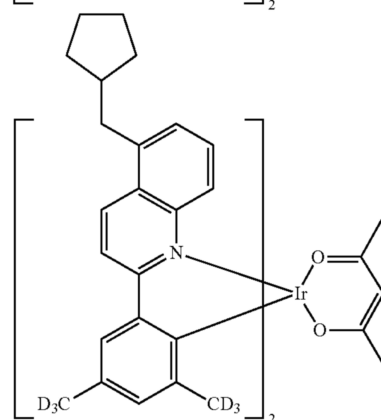
Compound II-55
