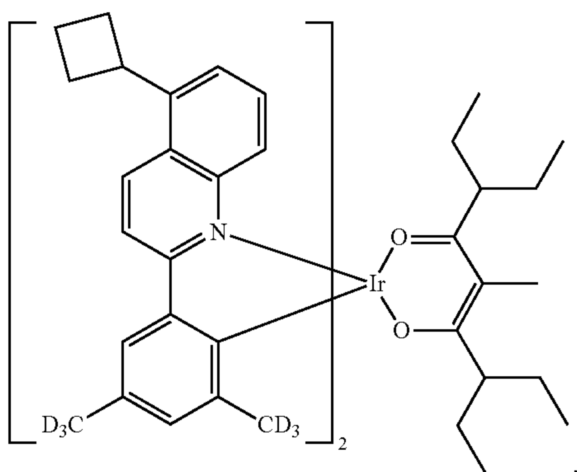
Compound II-51
