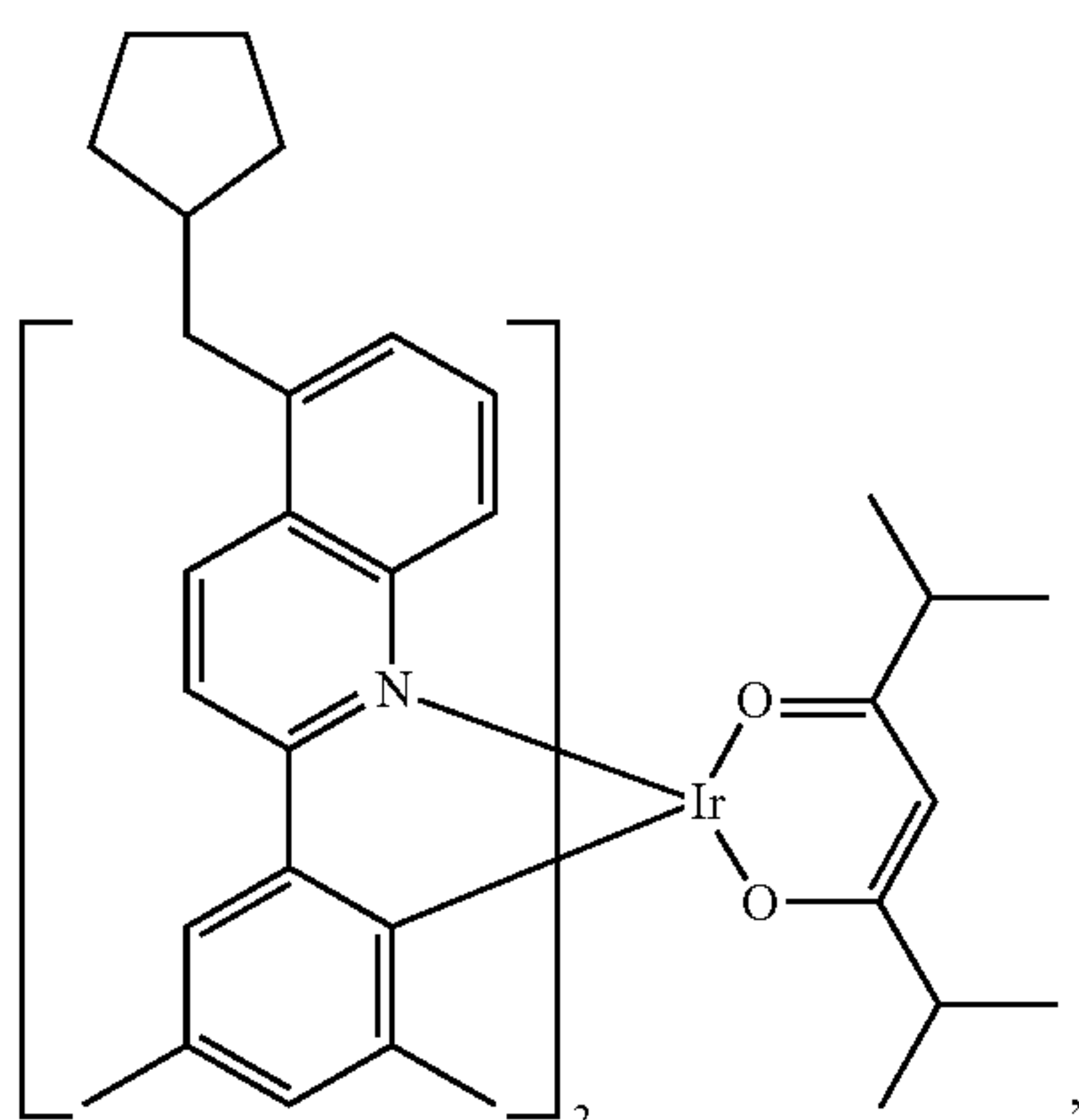
Compound II-23
