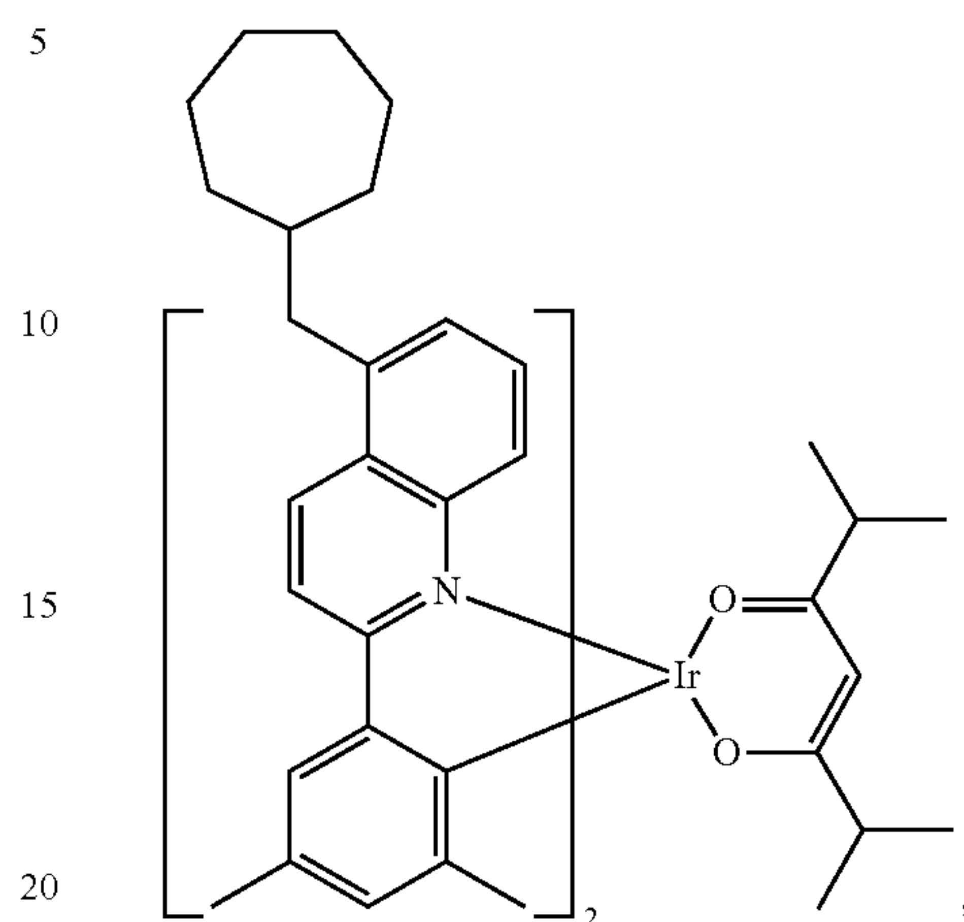
Compound II-21
