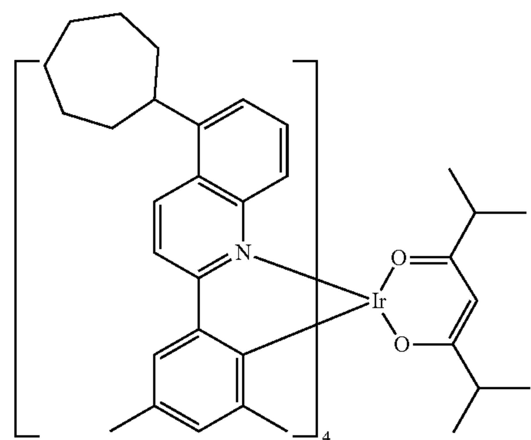
Compound II-9
