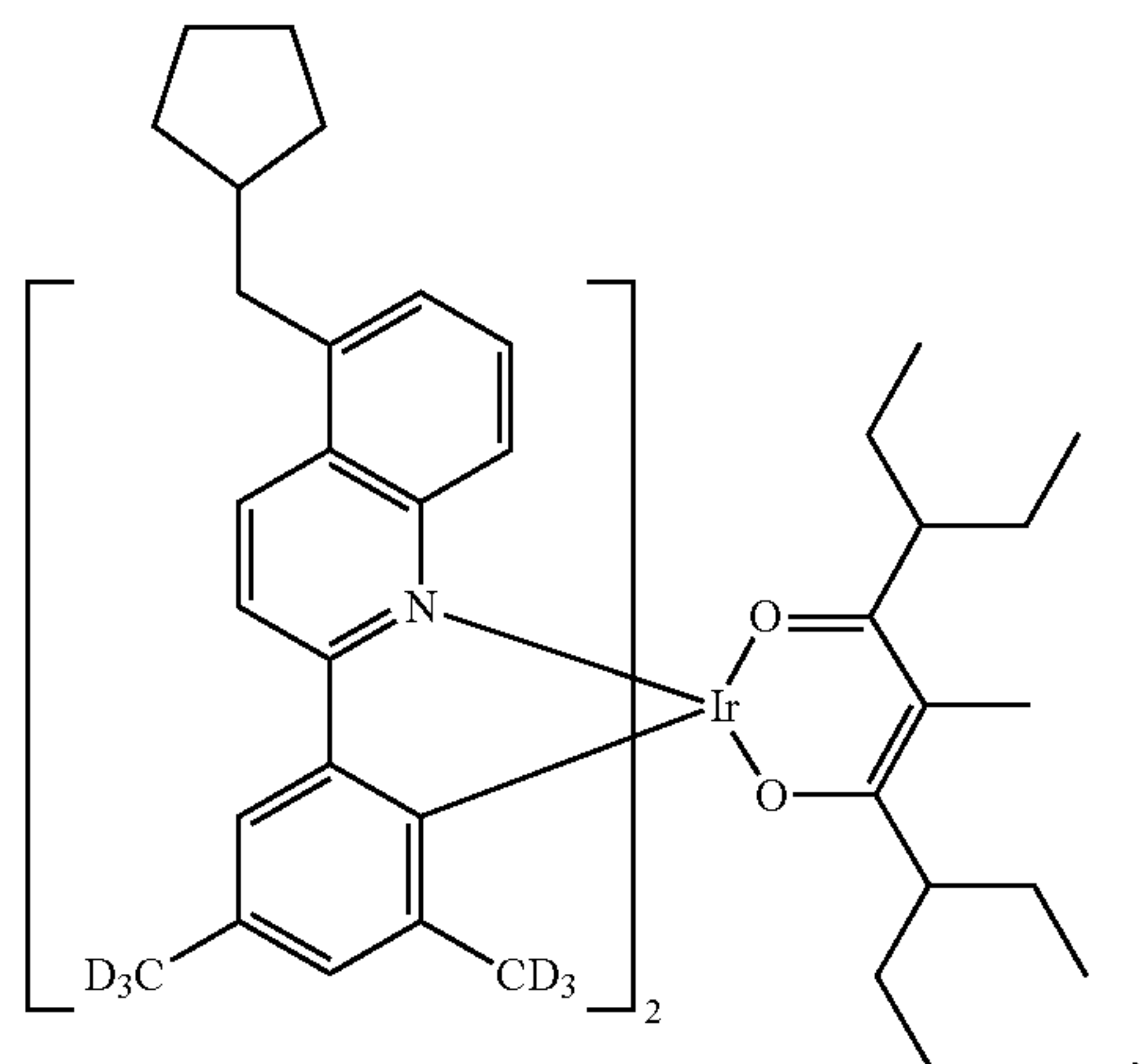
Compound II-70
