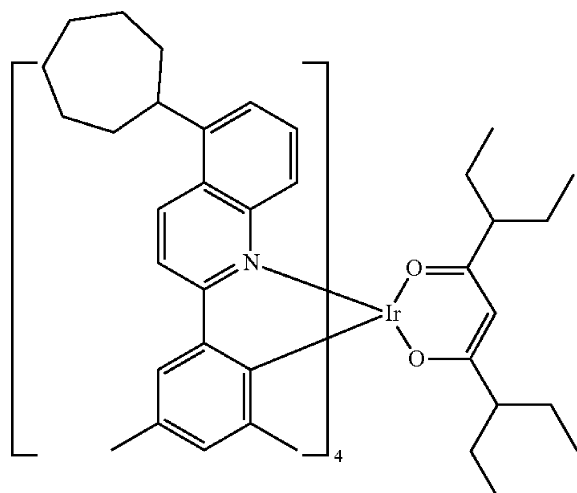
Compound II-15
