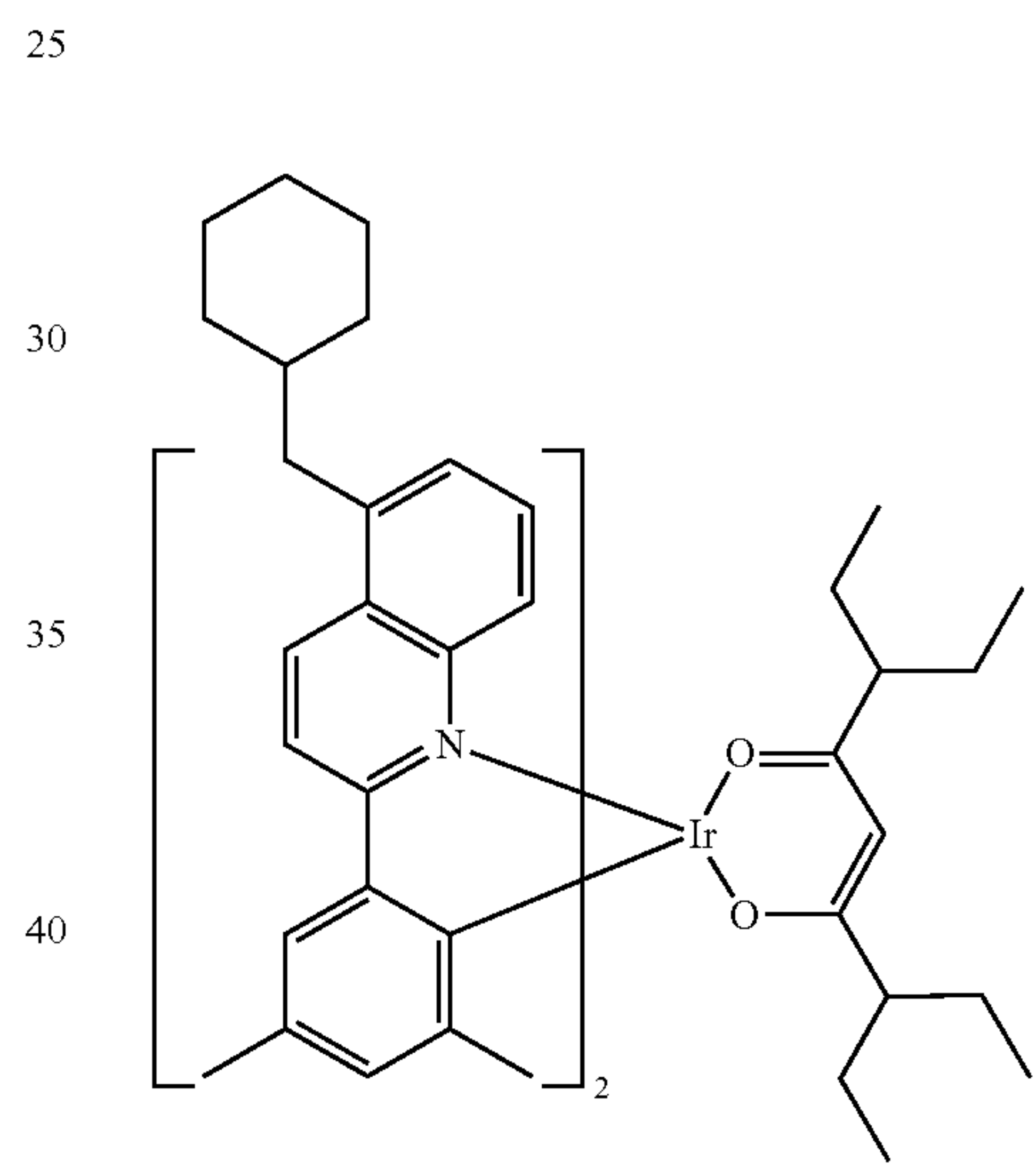
Compound II-28
