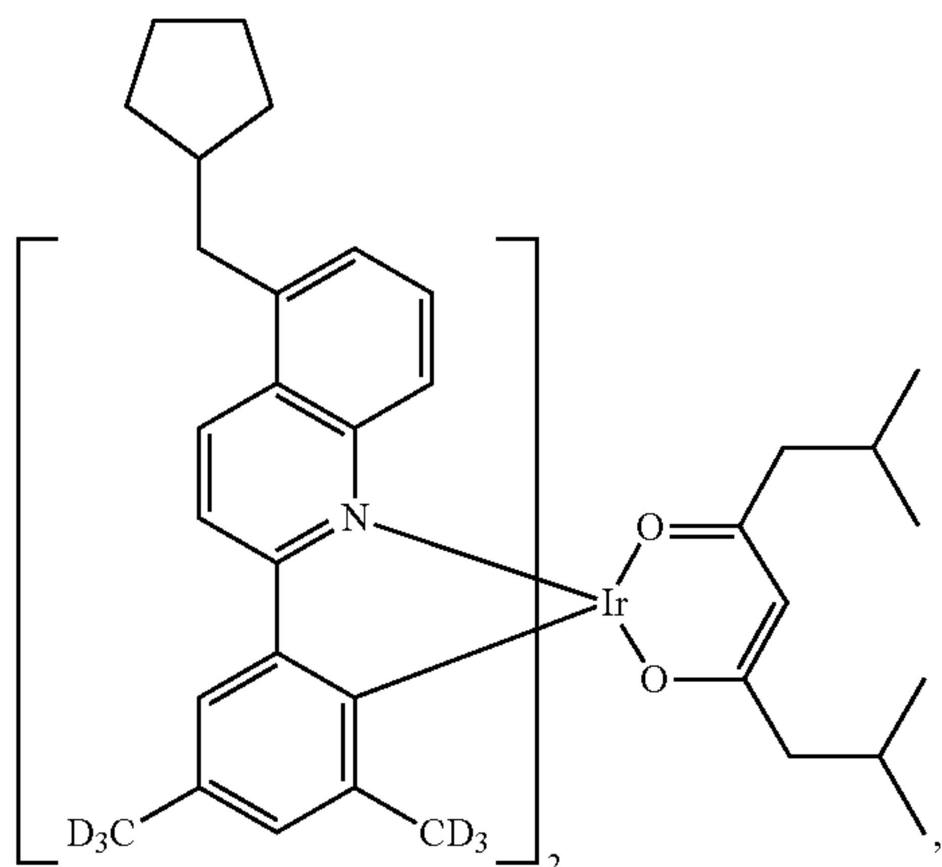
Compound II-62
