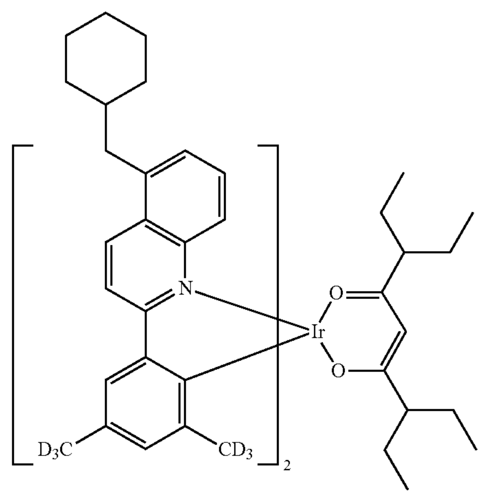
Compound II-67
