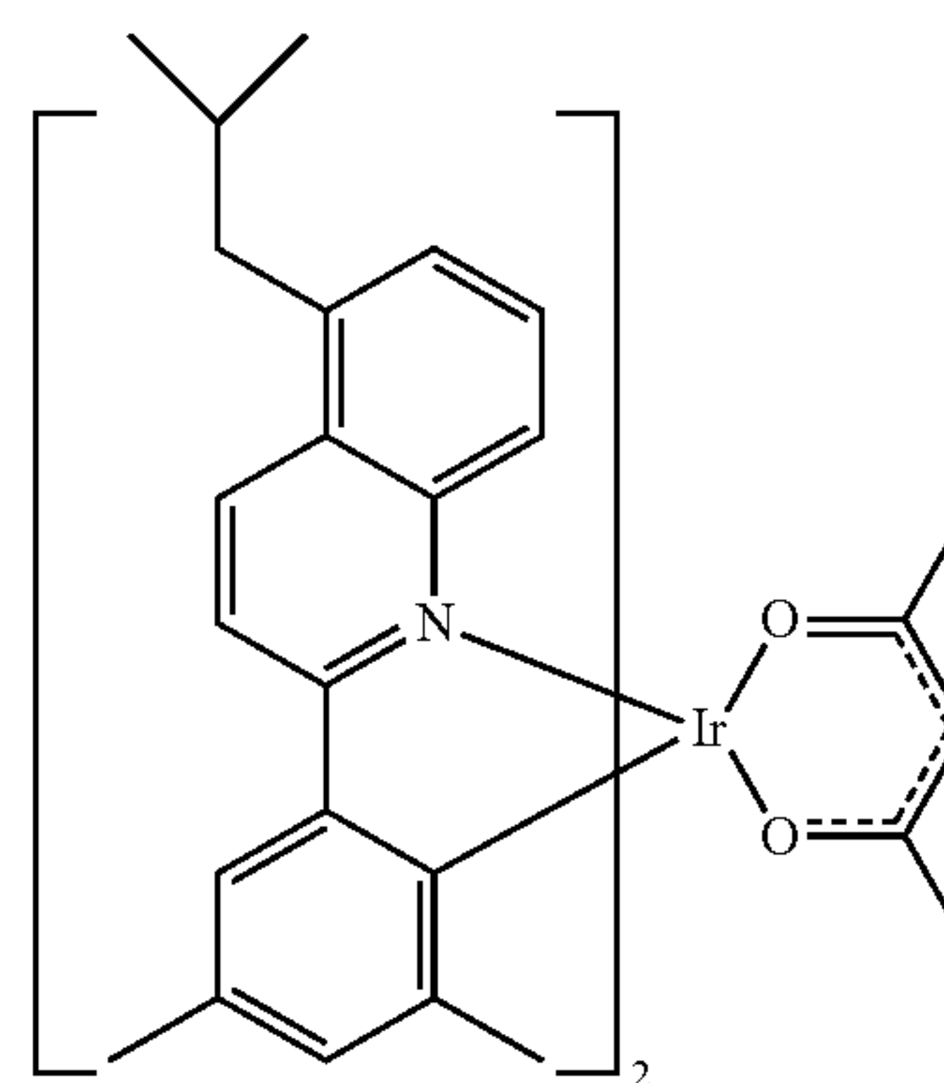
Compound 1
