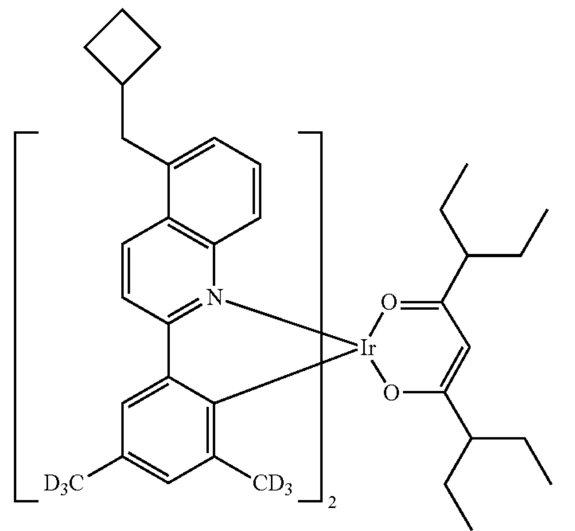
Compound II-65
