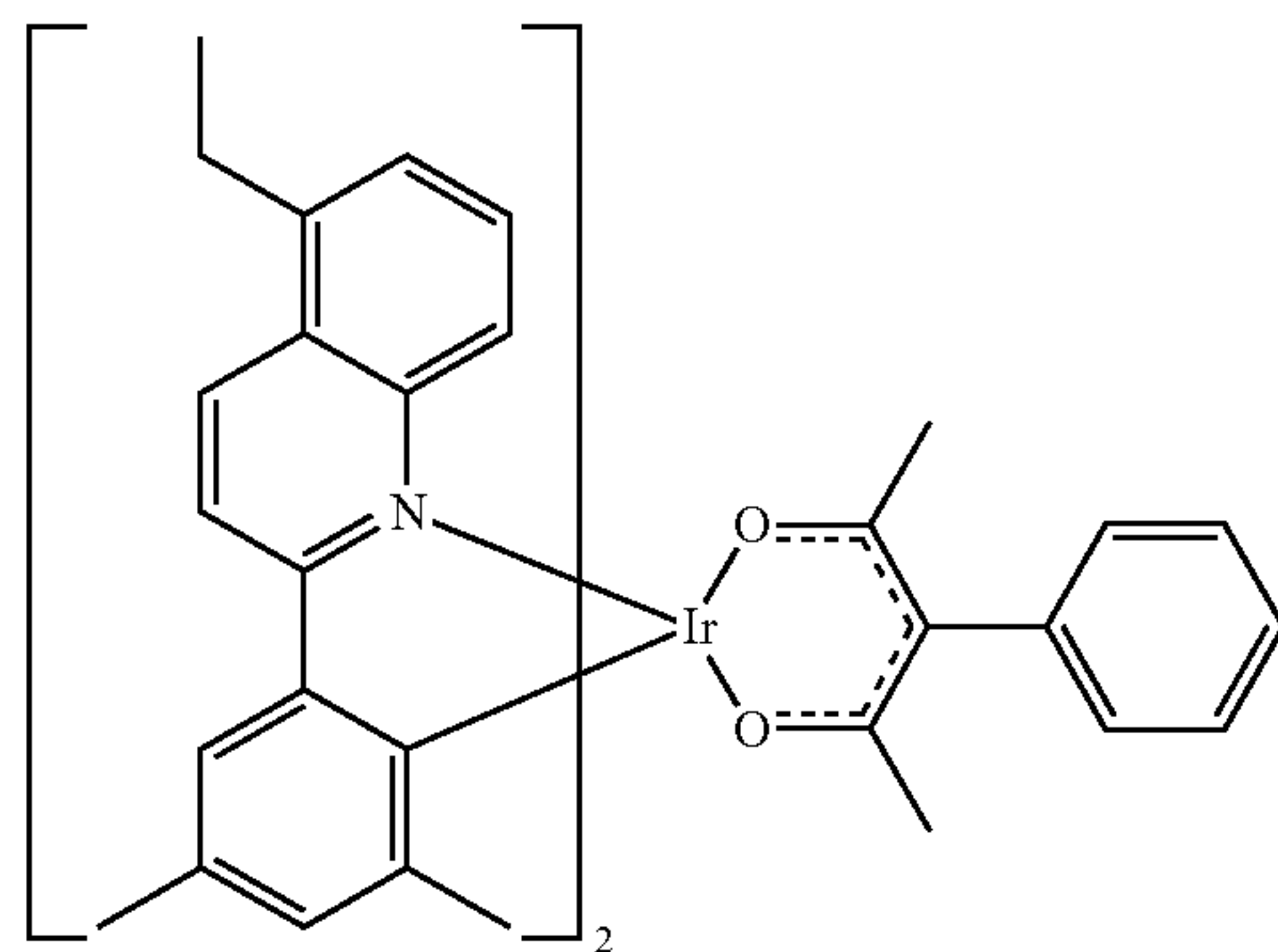
Compound 25
