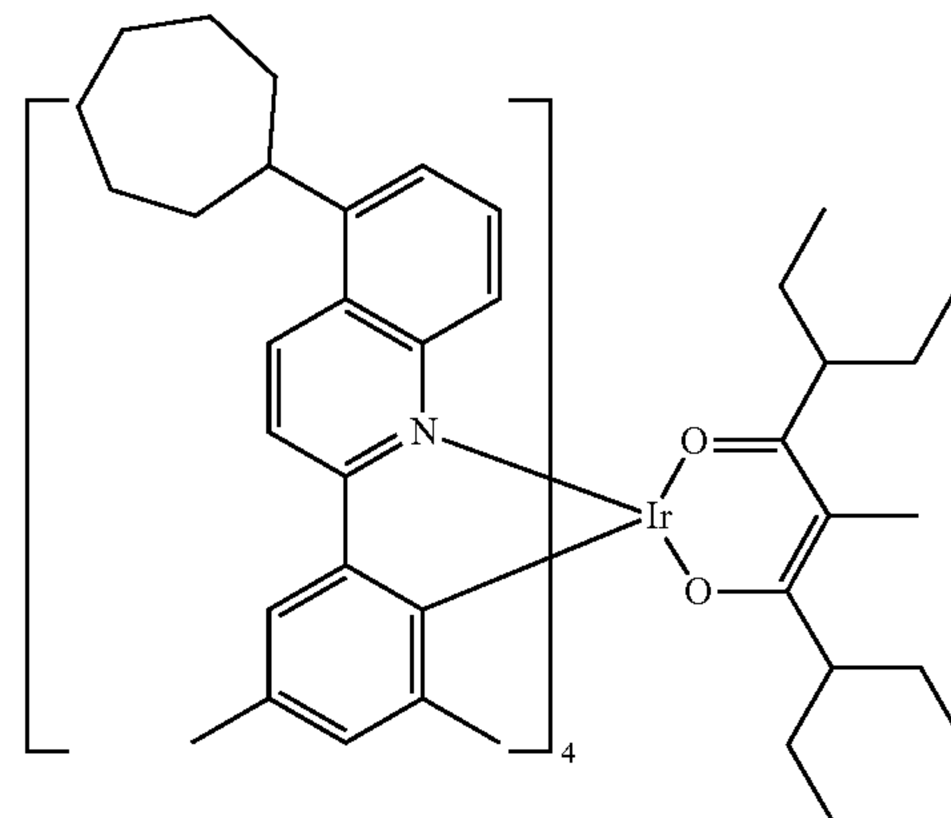
Compound II-17
