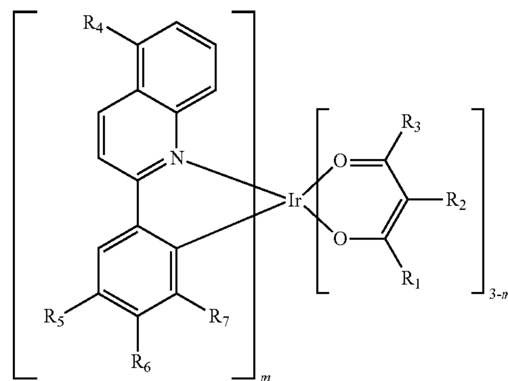
Formula III
