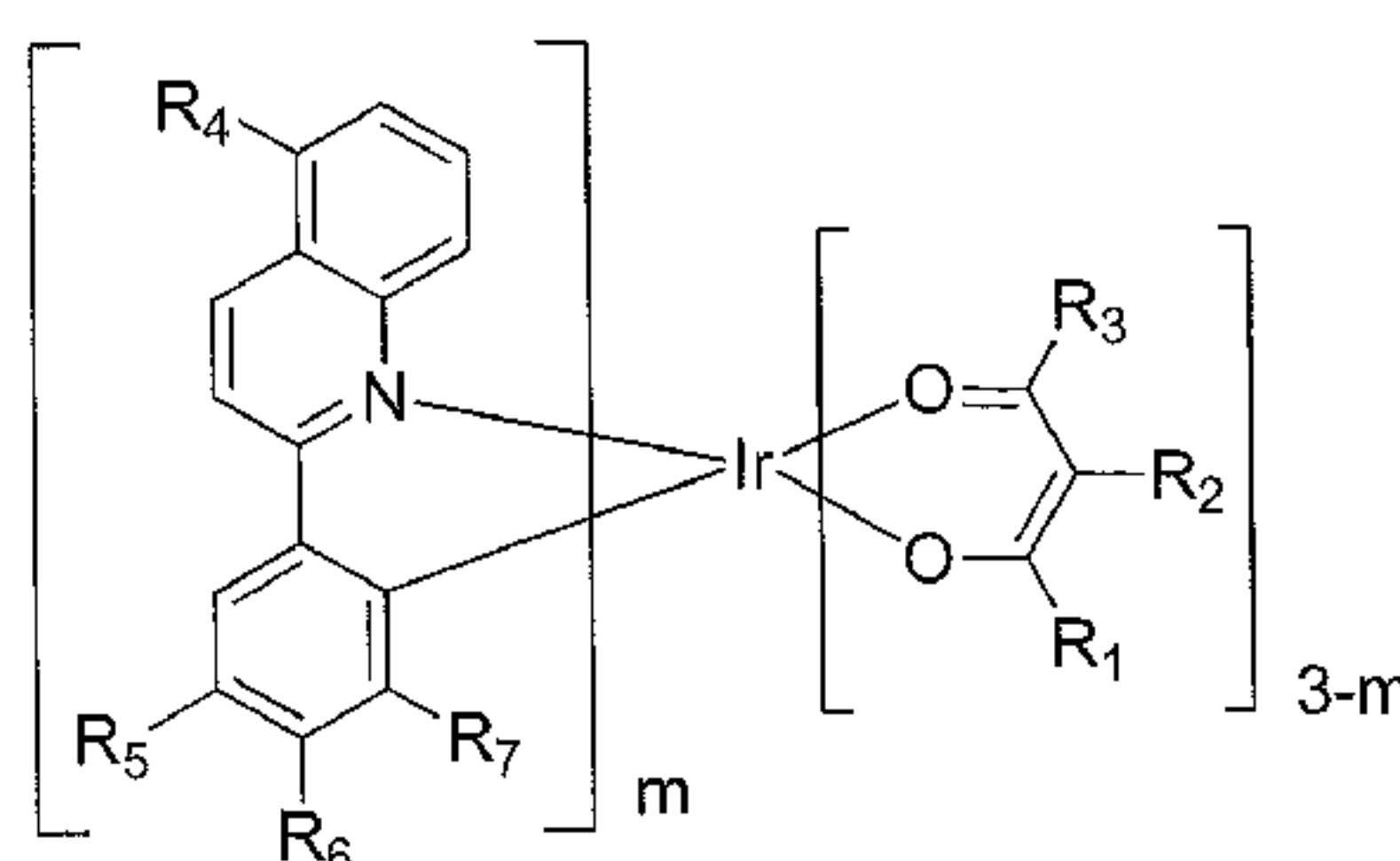
Formula III
