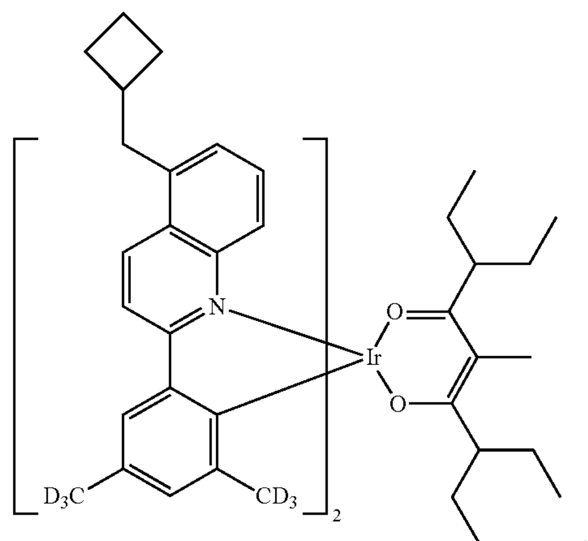
Compound II-69
