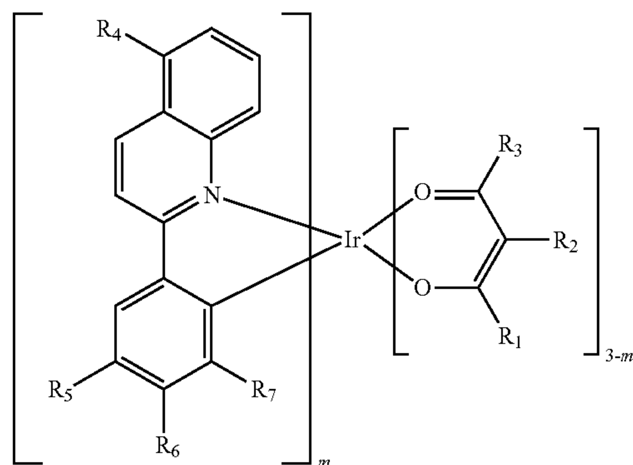
Formula III
