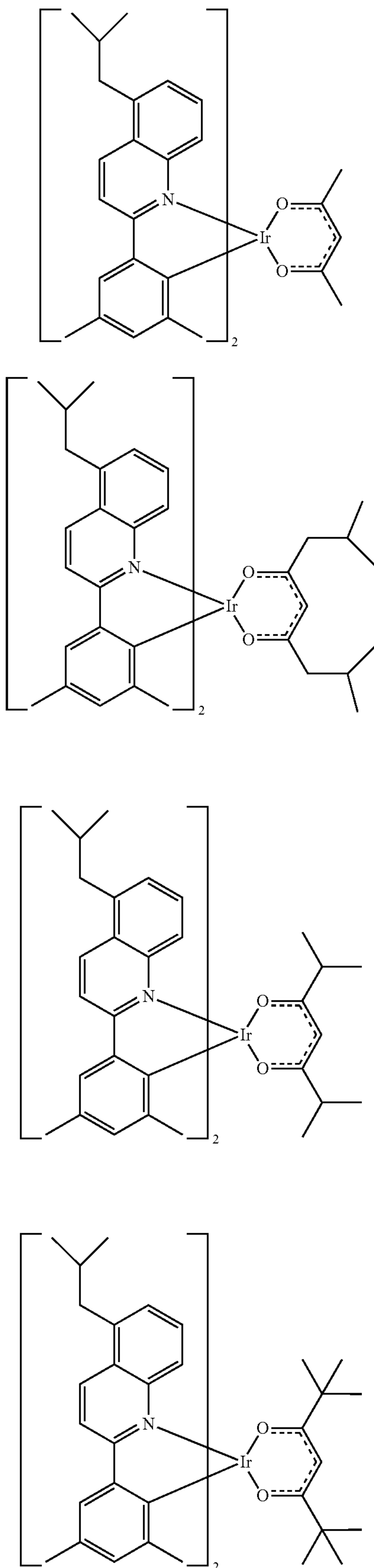
Compound 2
