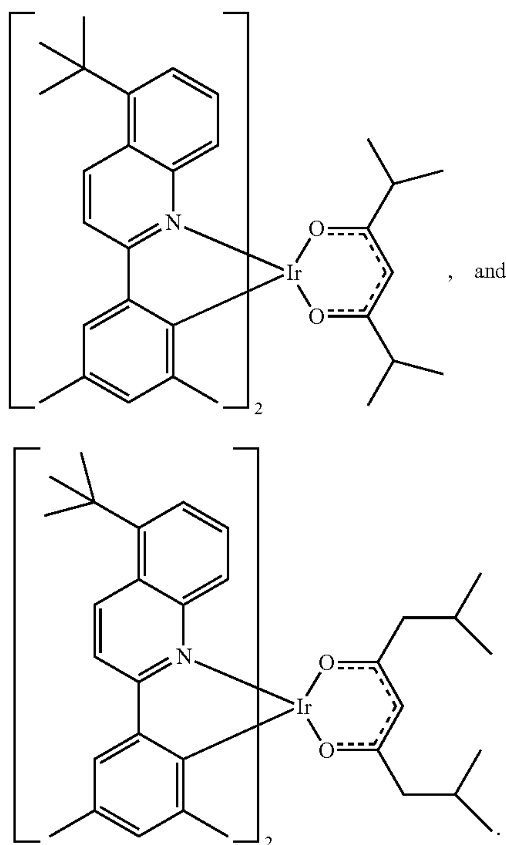
Compound 17
