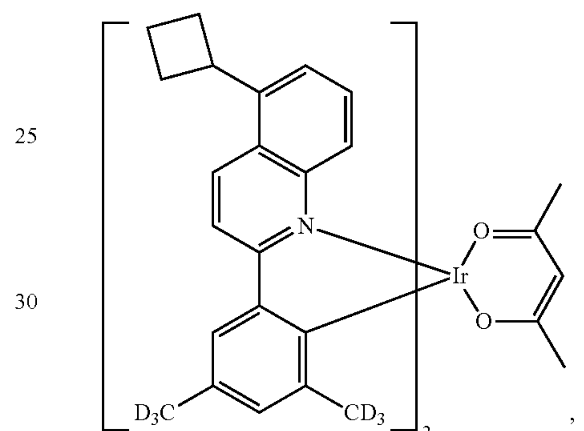
Compound II-34
