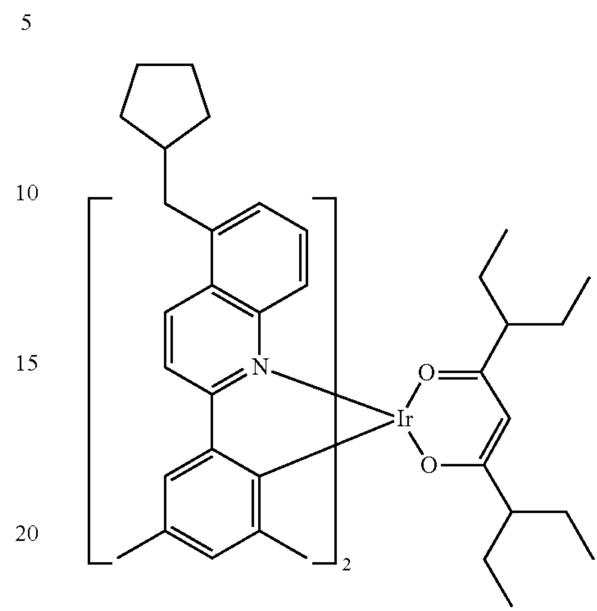
Compound II-27
