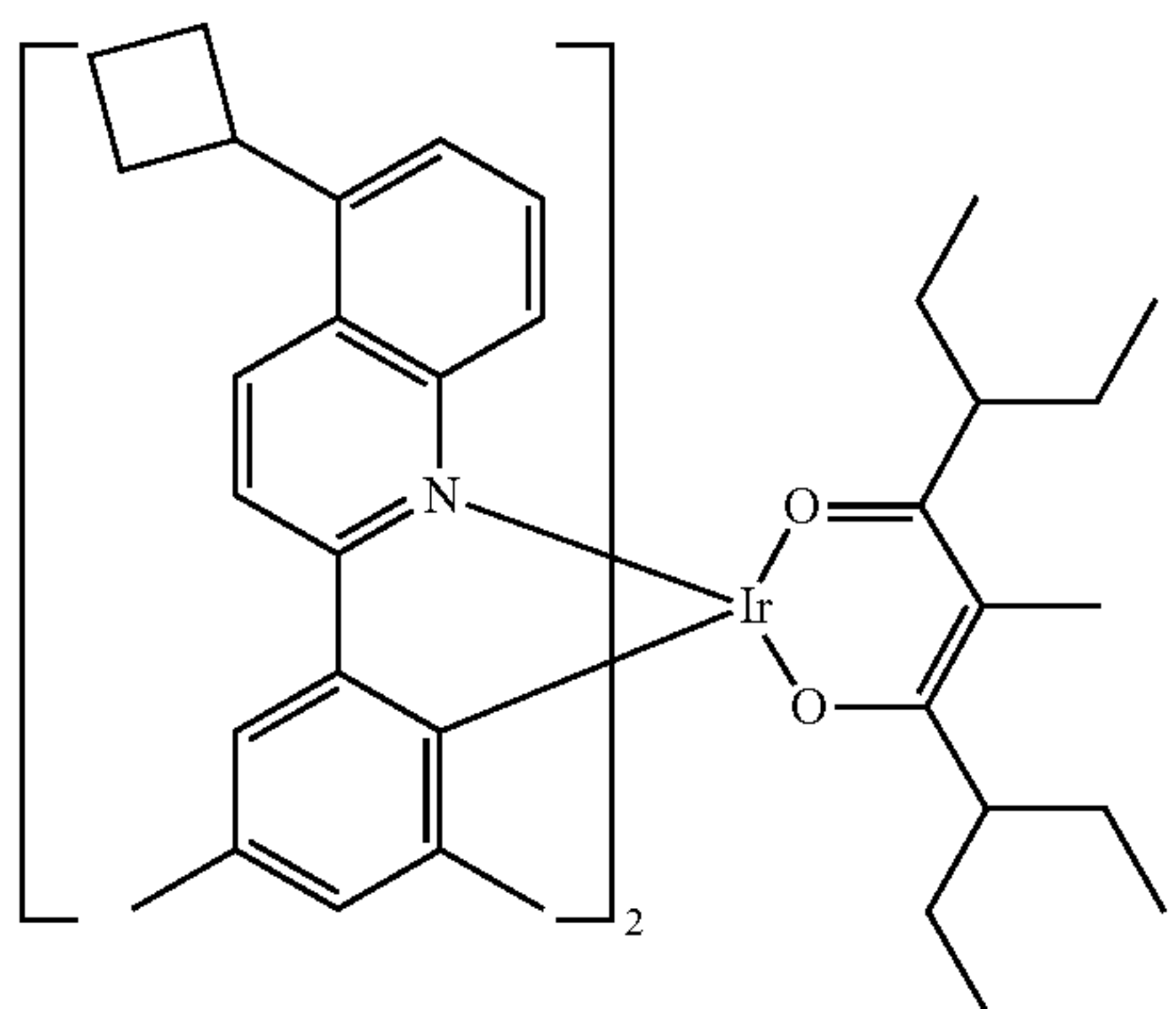
Compound II-15
