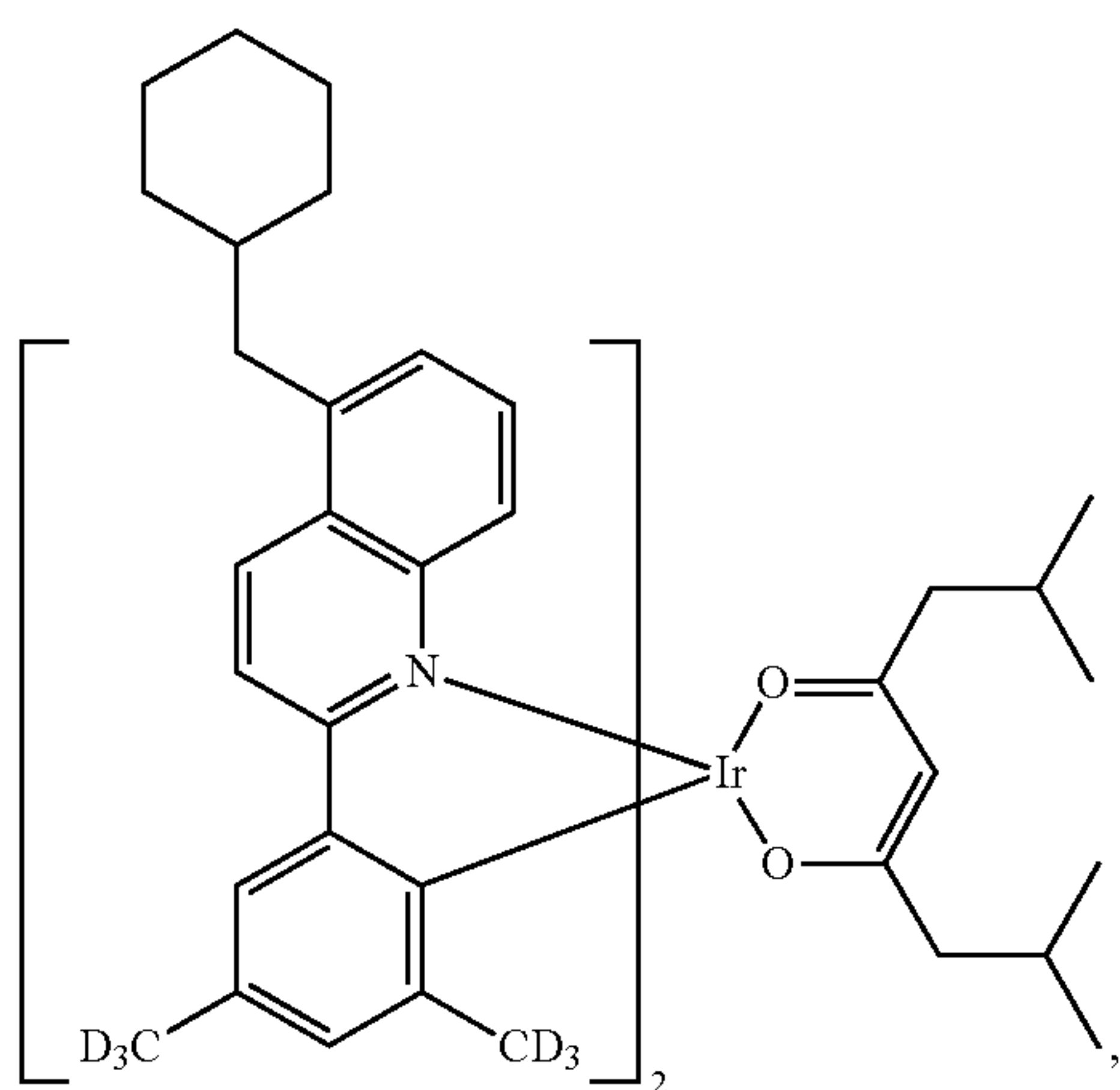
Compound II-63
