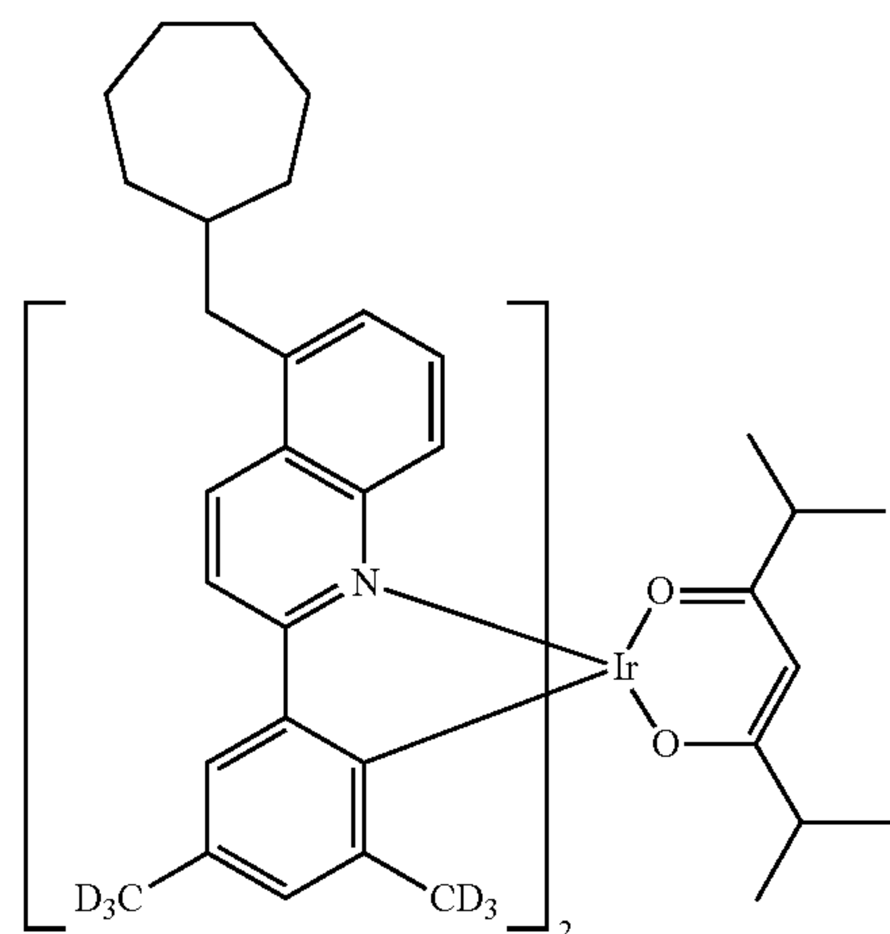
Compound II-60
