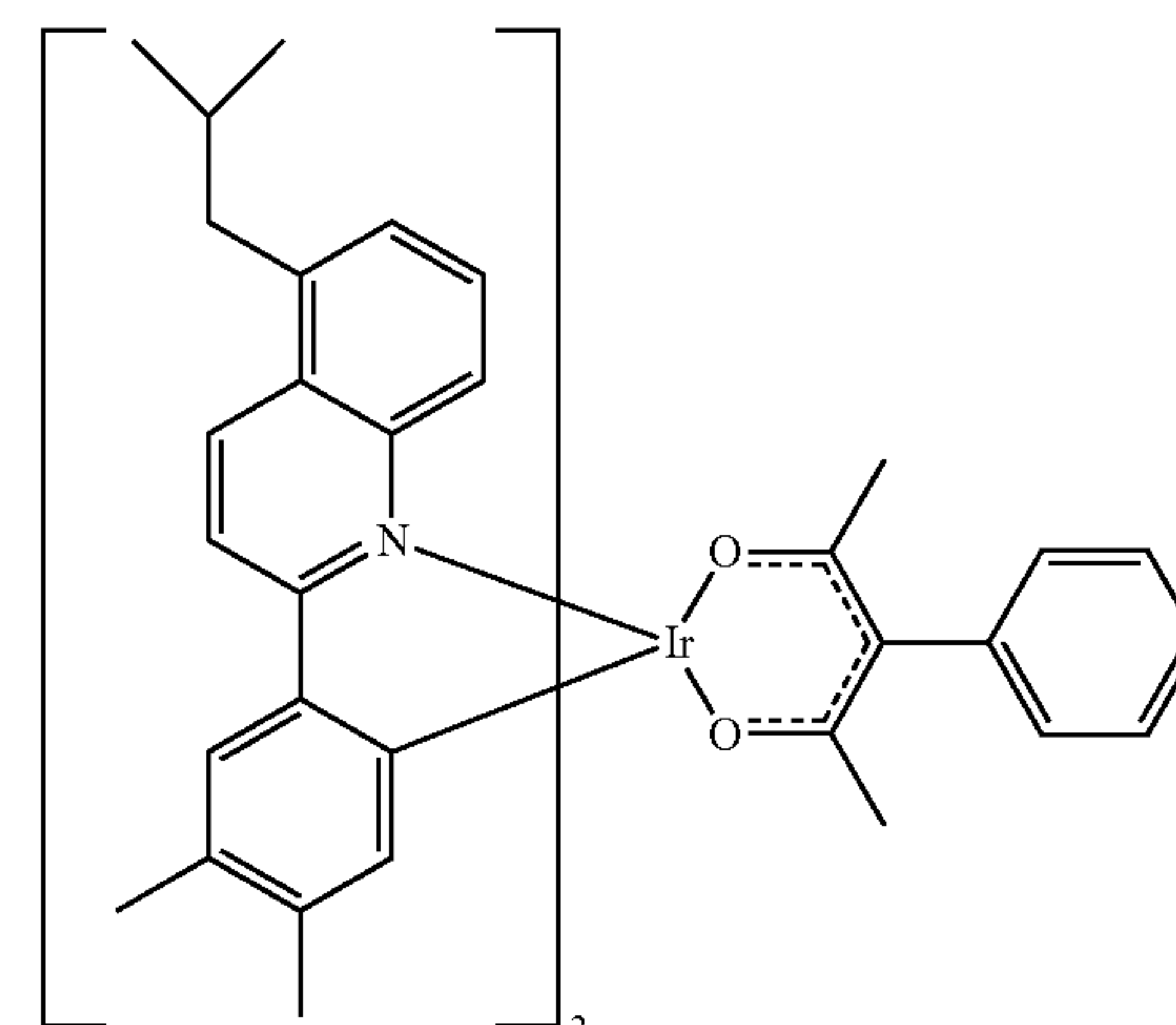
Compound 37
