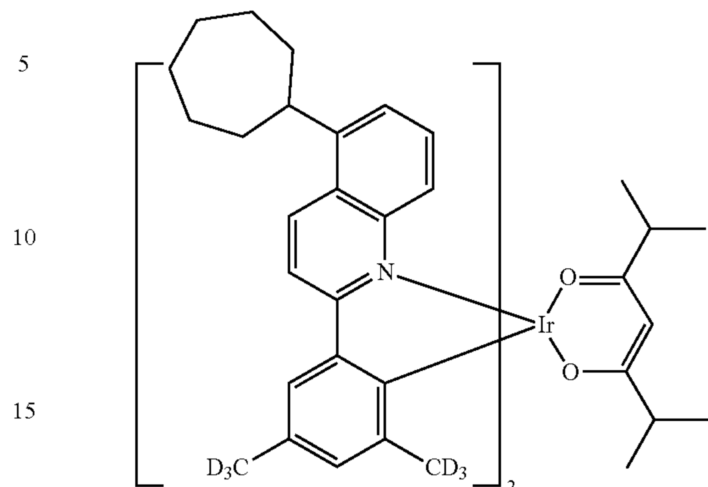
Compound II-44
