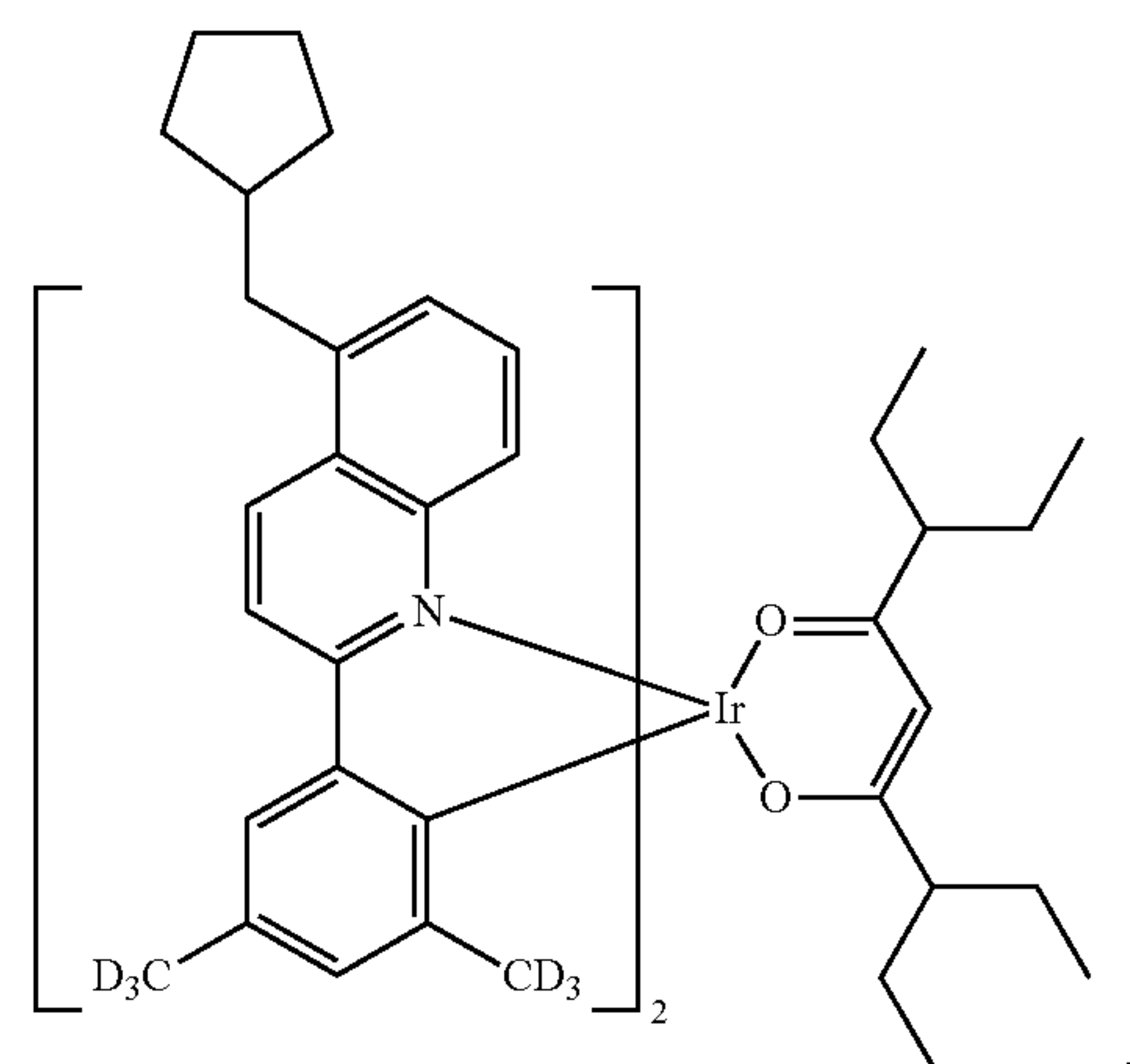
Compound II-66
