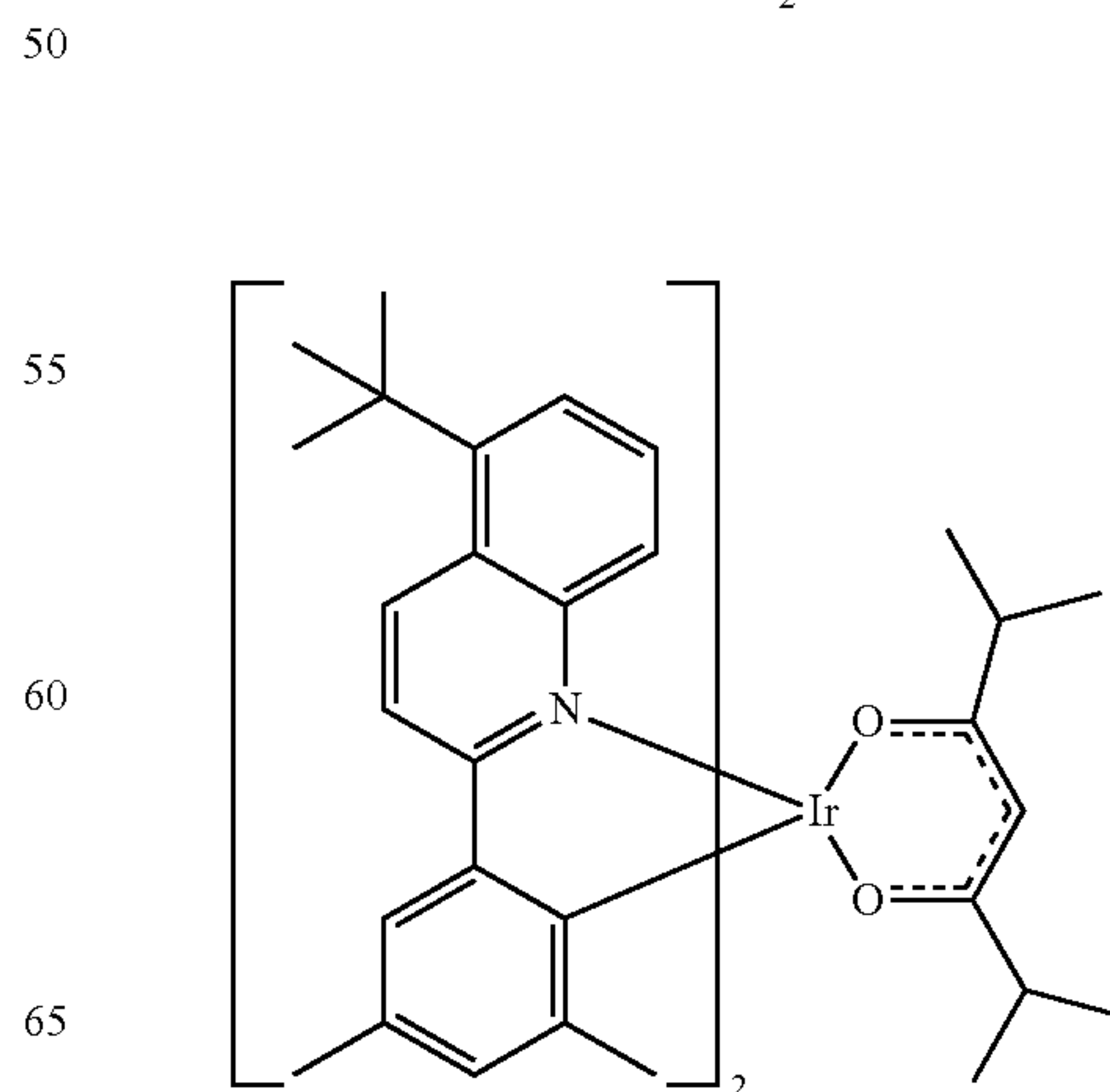
Compound 12
