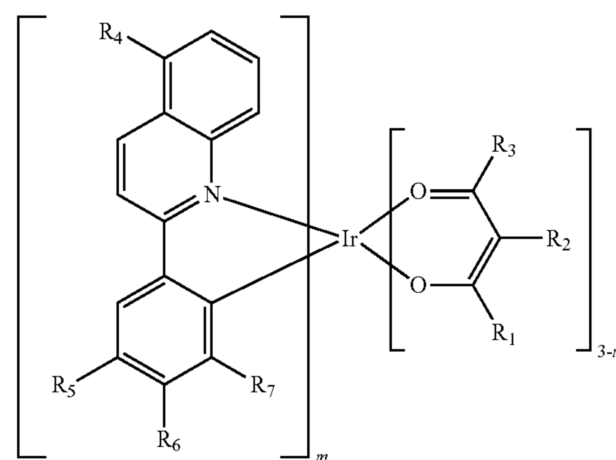
Formula III
