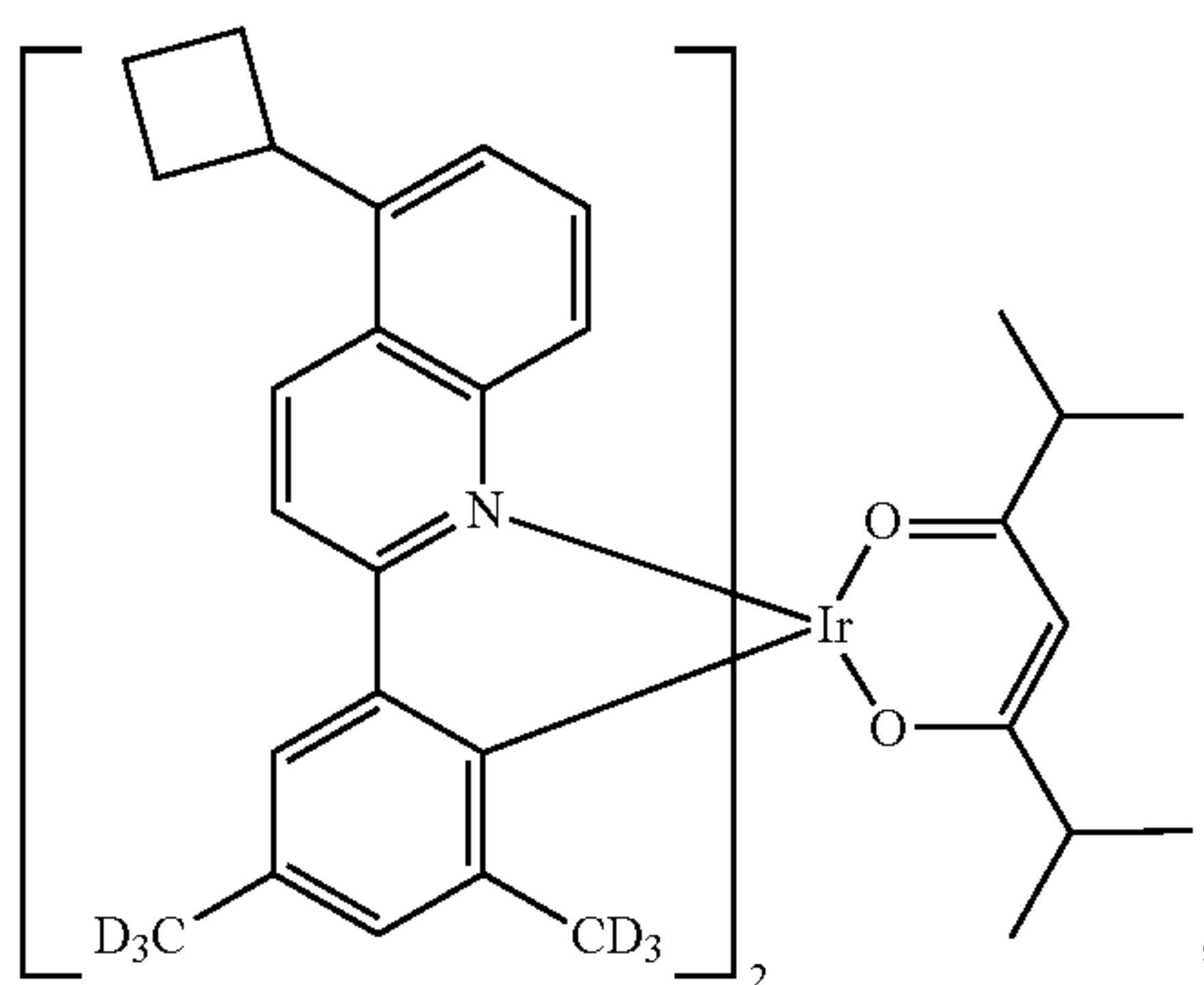
Compound II-42
