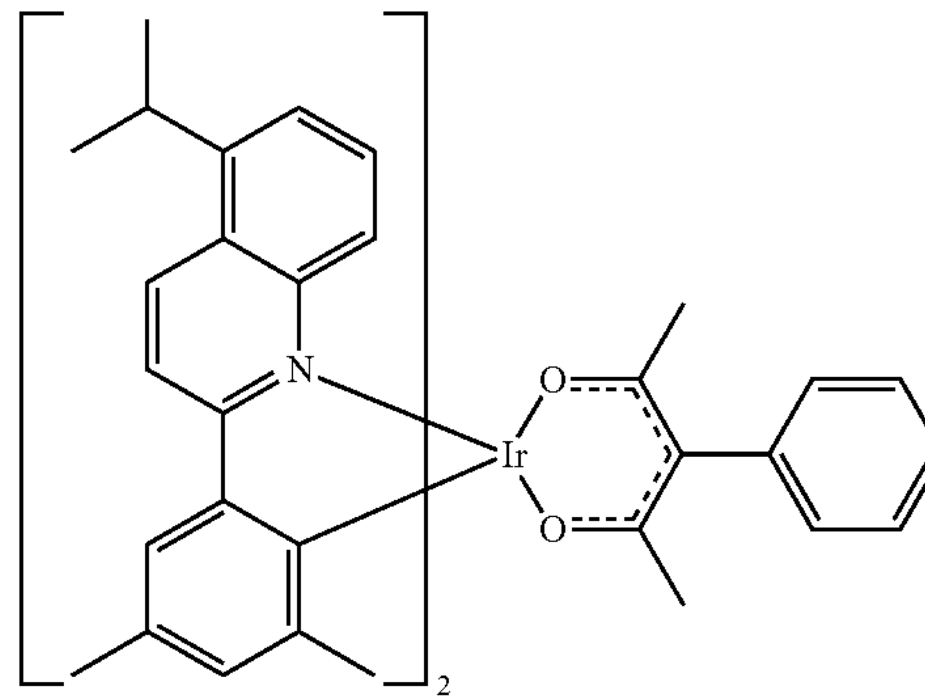
Compound 21
