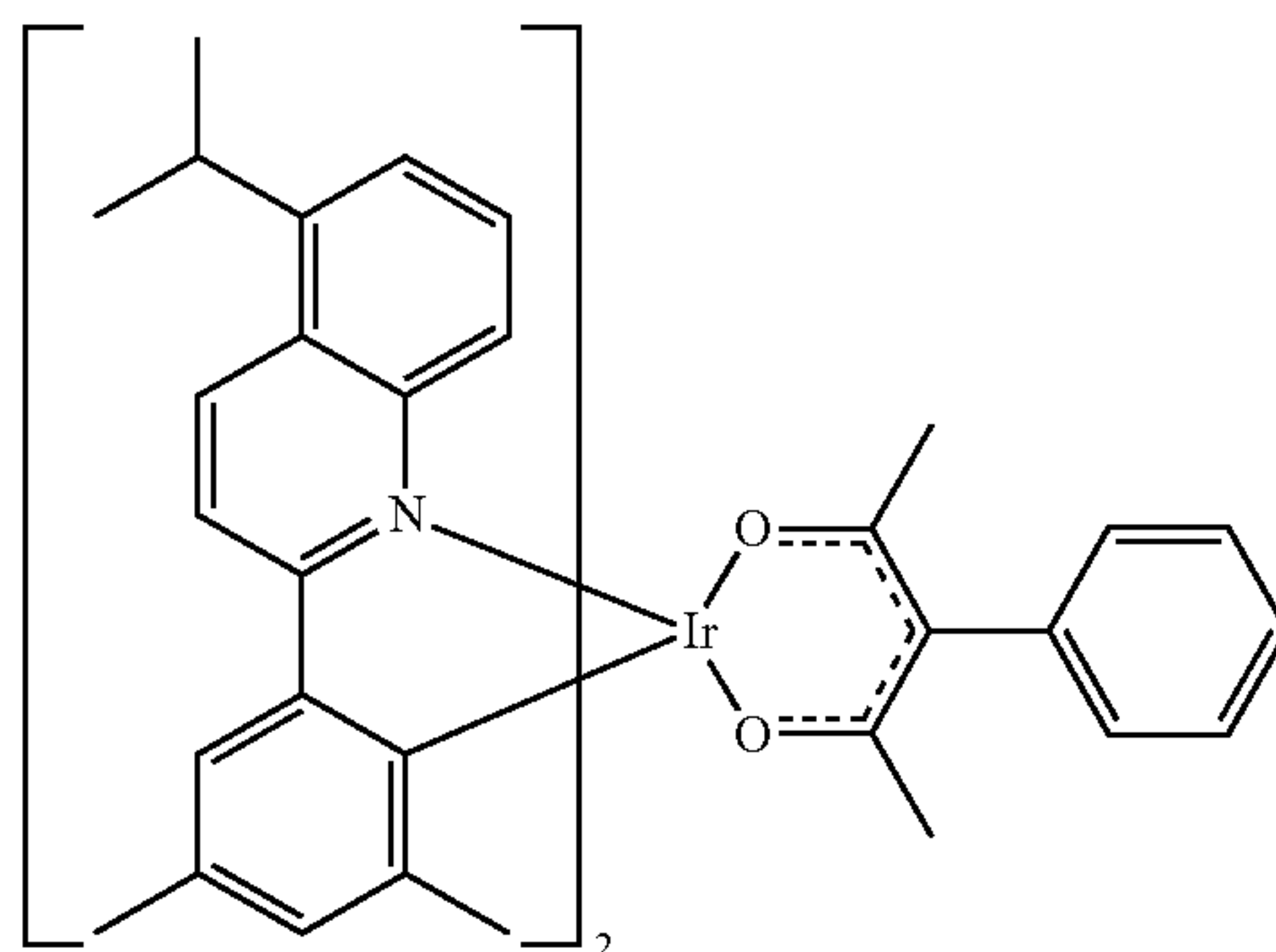
Compound 21
