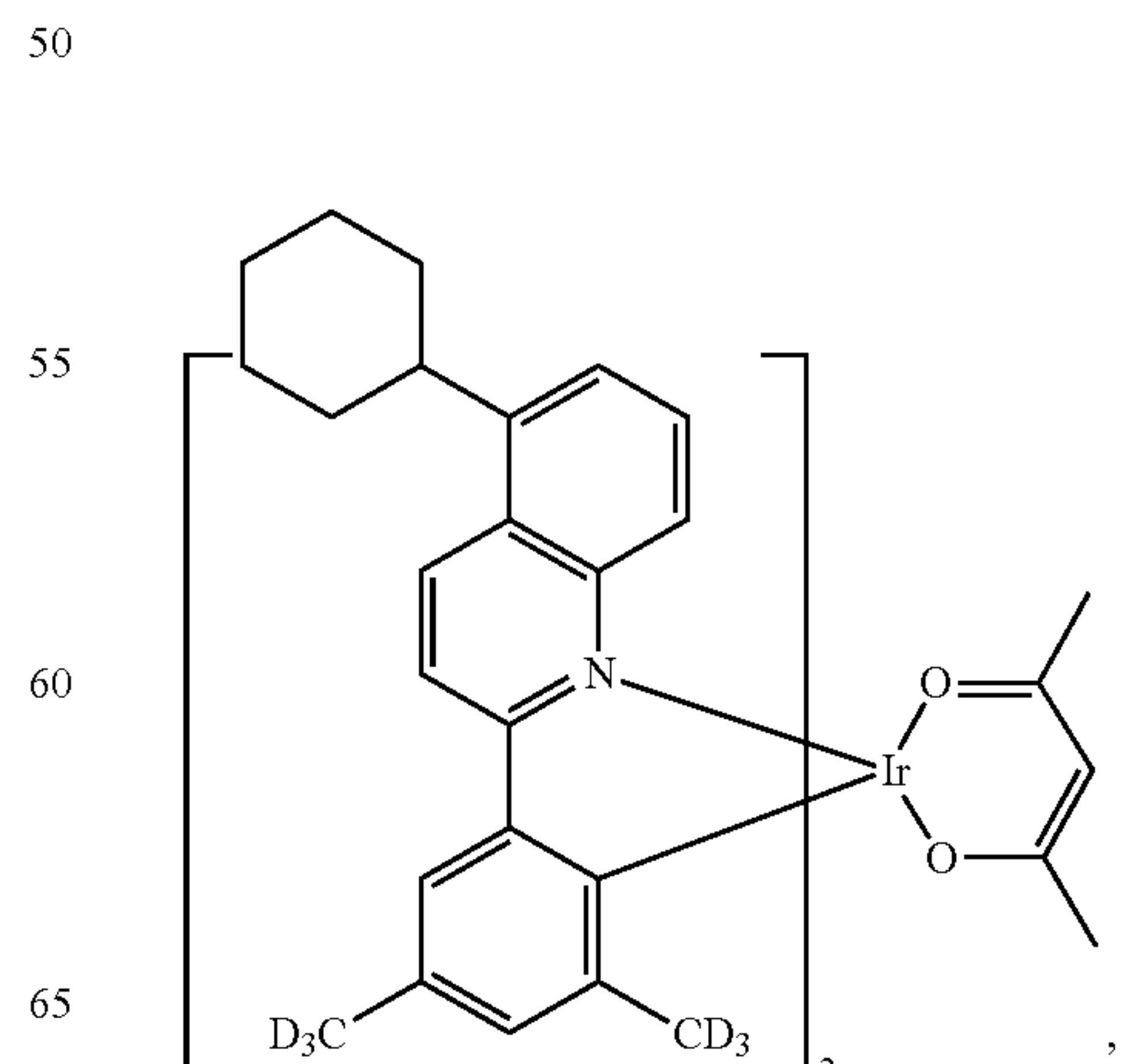
Compound II-39
