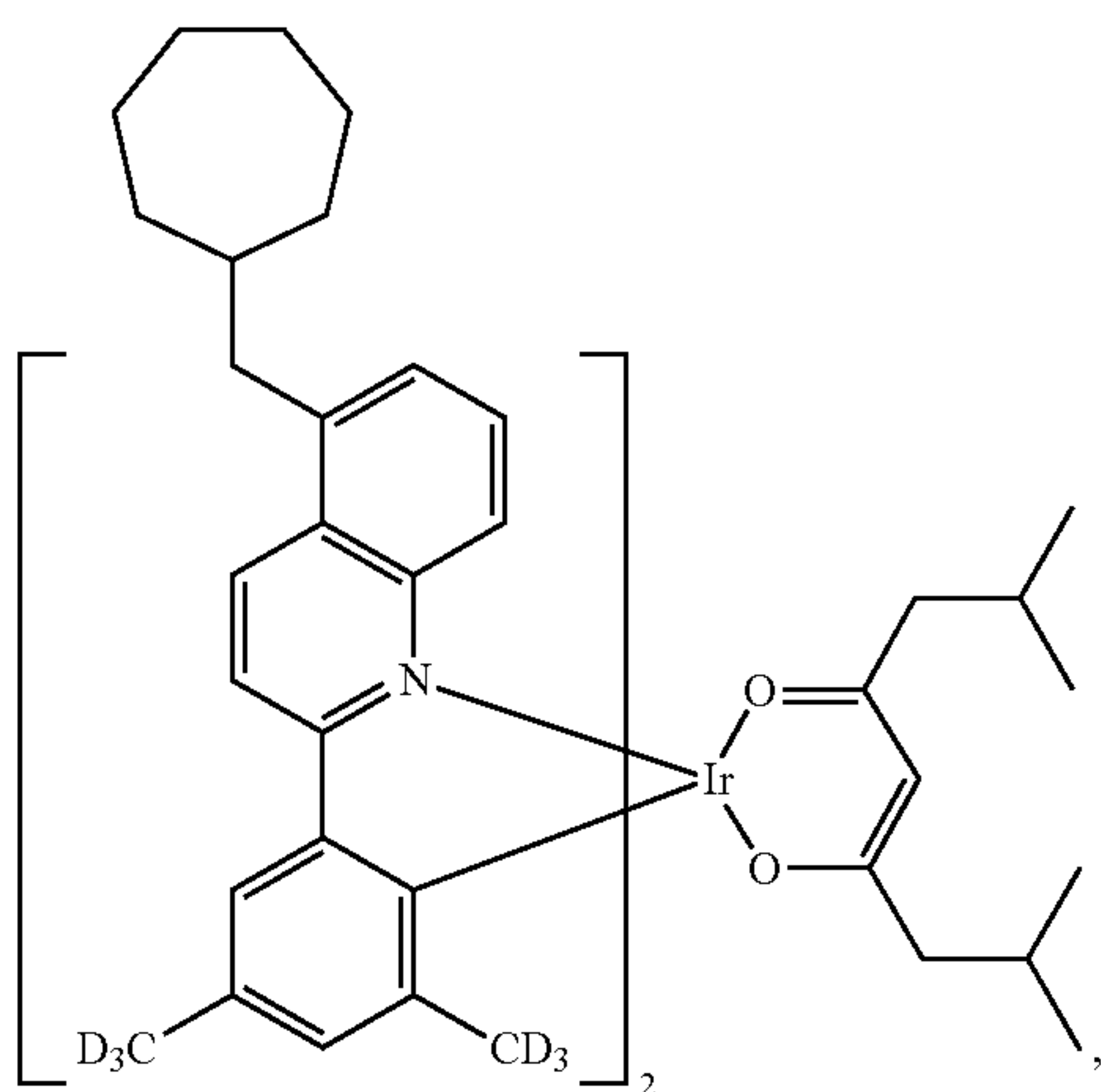
Compound II-64
