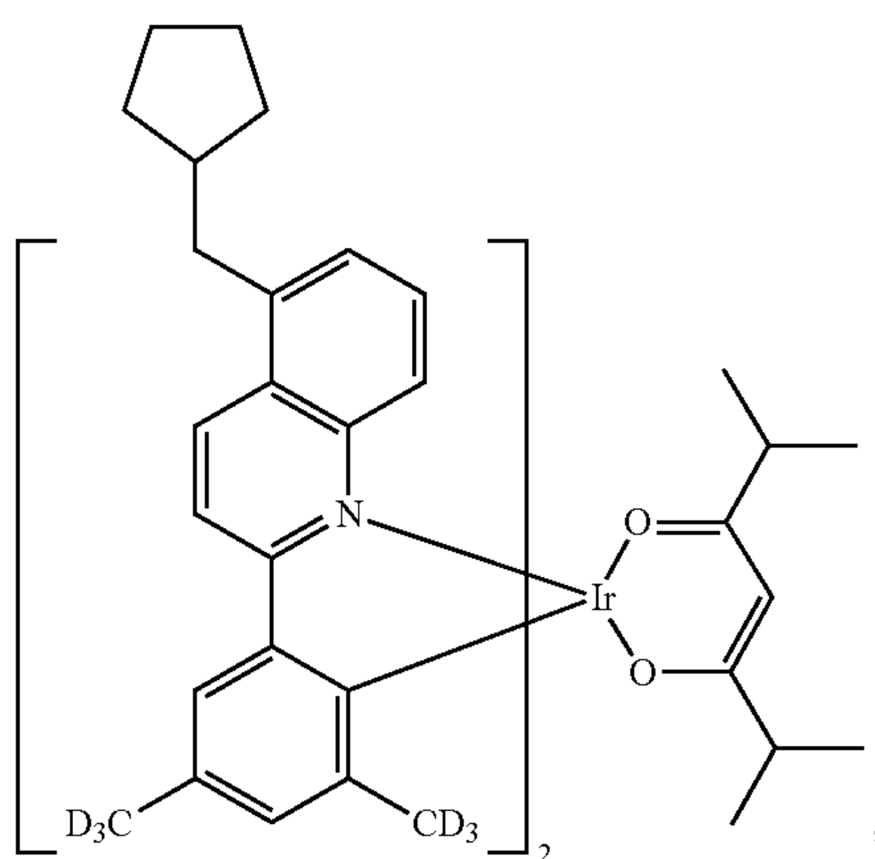
Compound II-58
