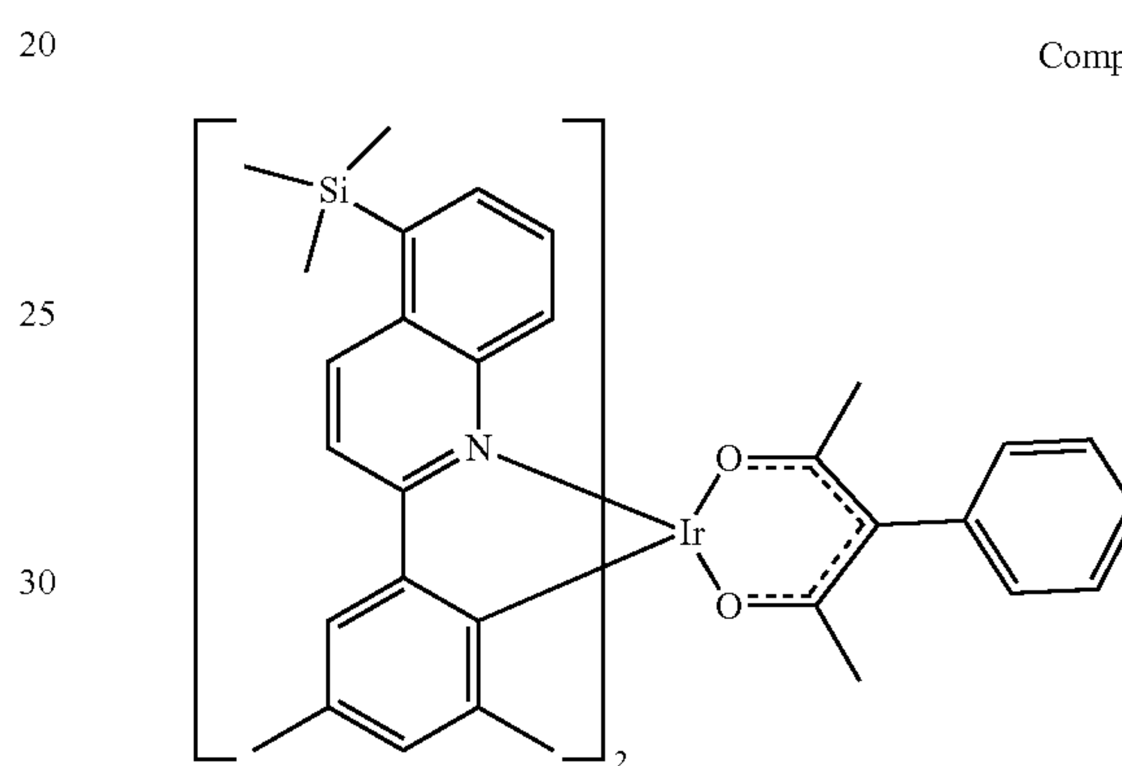
Compound 11
