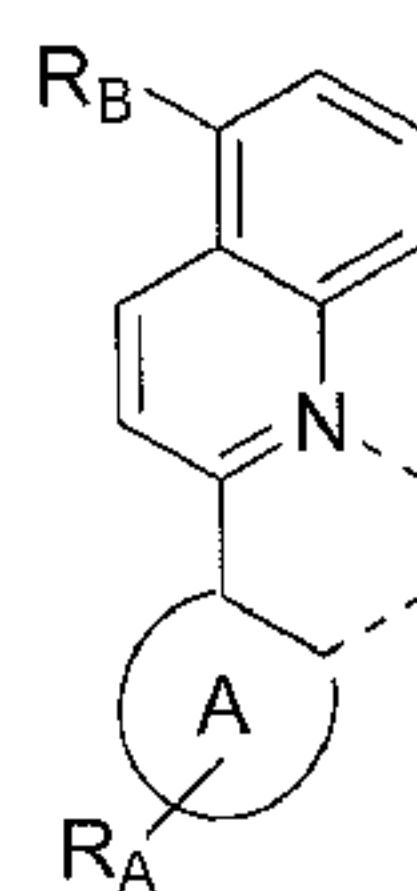
Formula I
