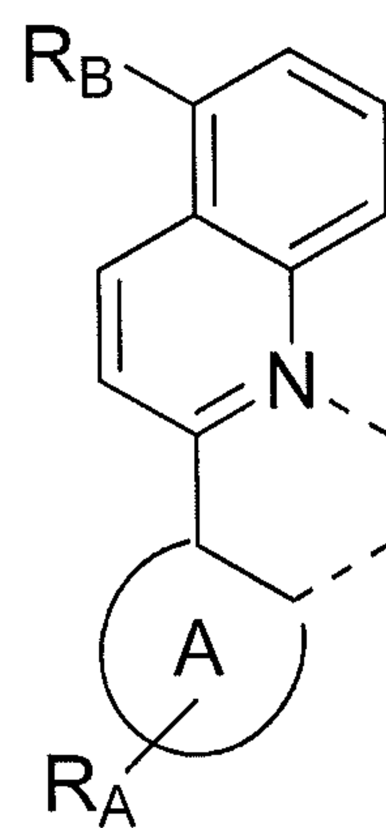
Formula I
