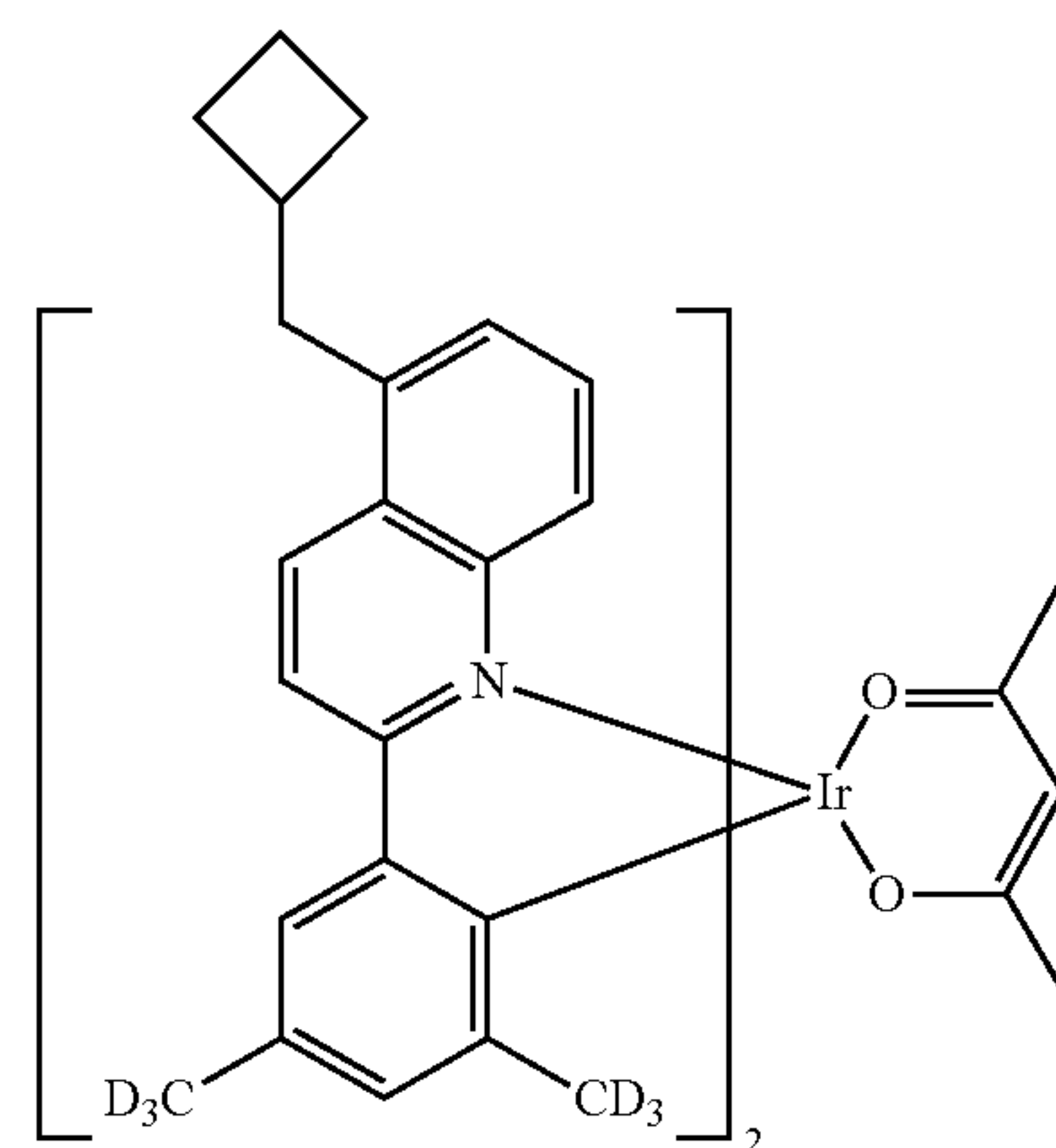
Compound II-54
