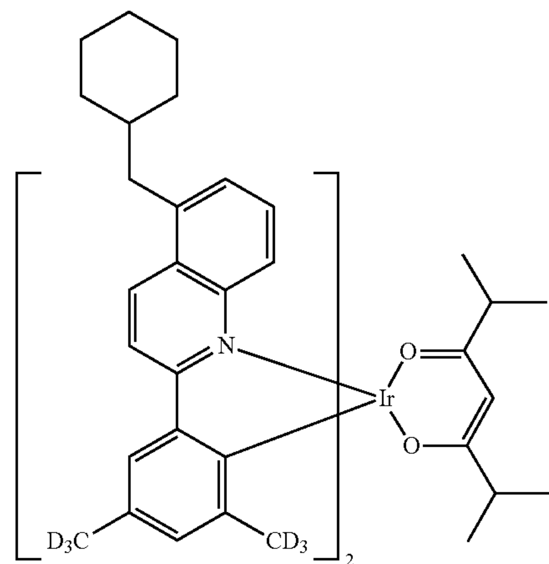
Compound II-59
