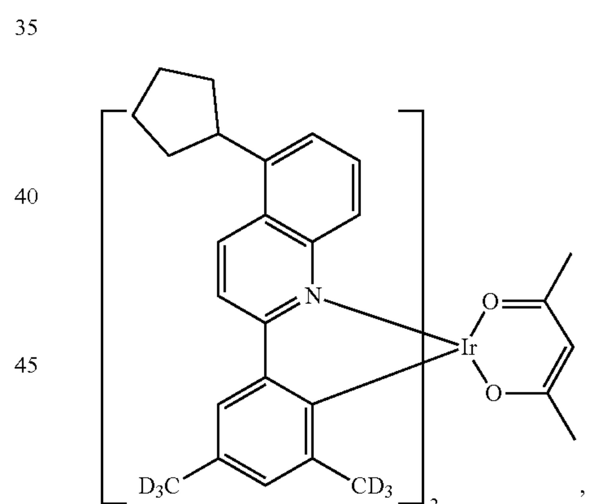
Compound II-35
