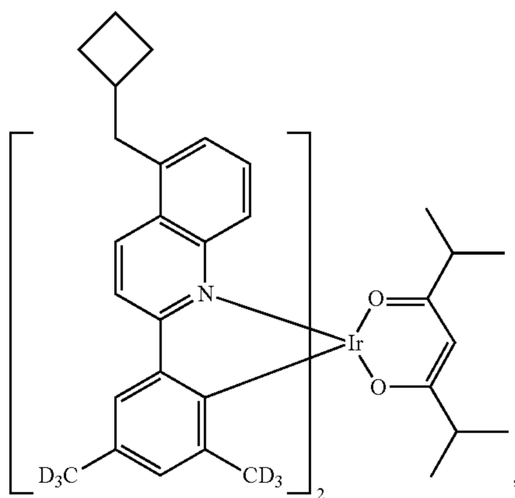
Compound II-57
