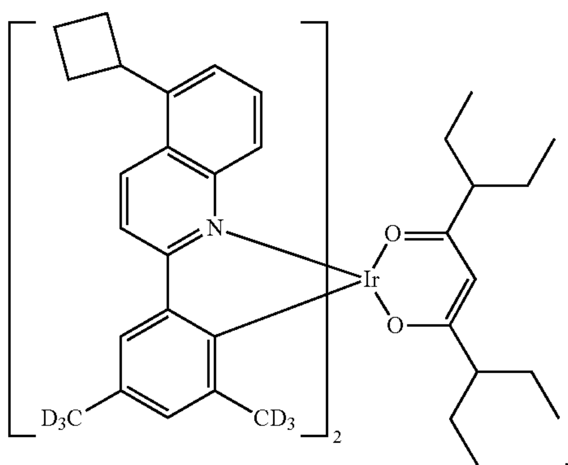
Compound II-50
