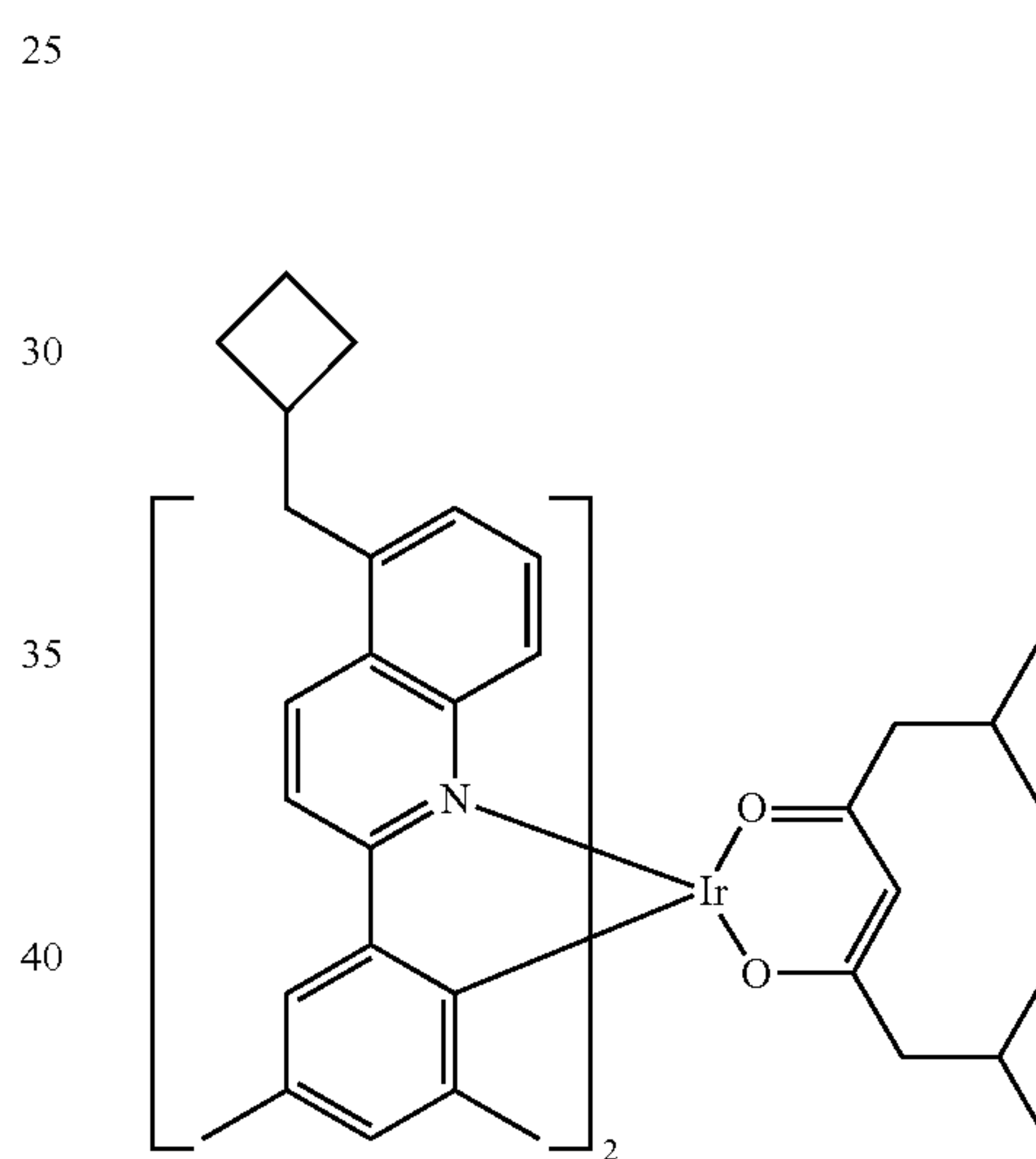
Compound II-22
