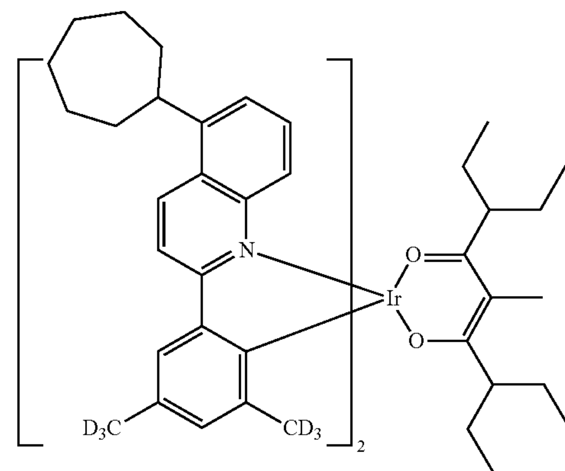
Compound II-53
