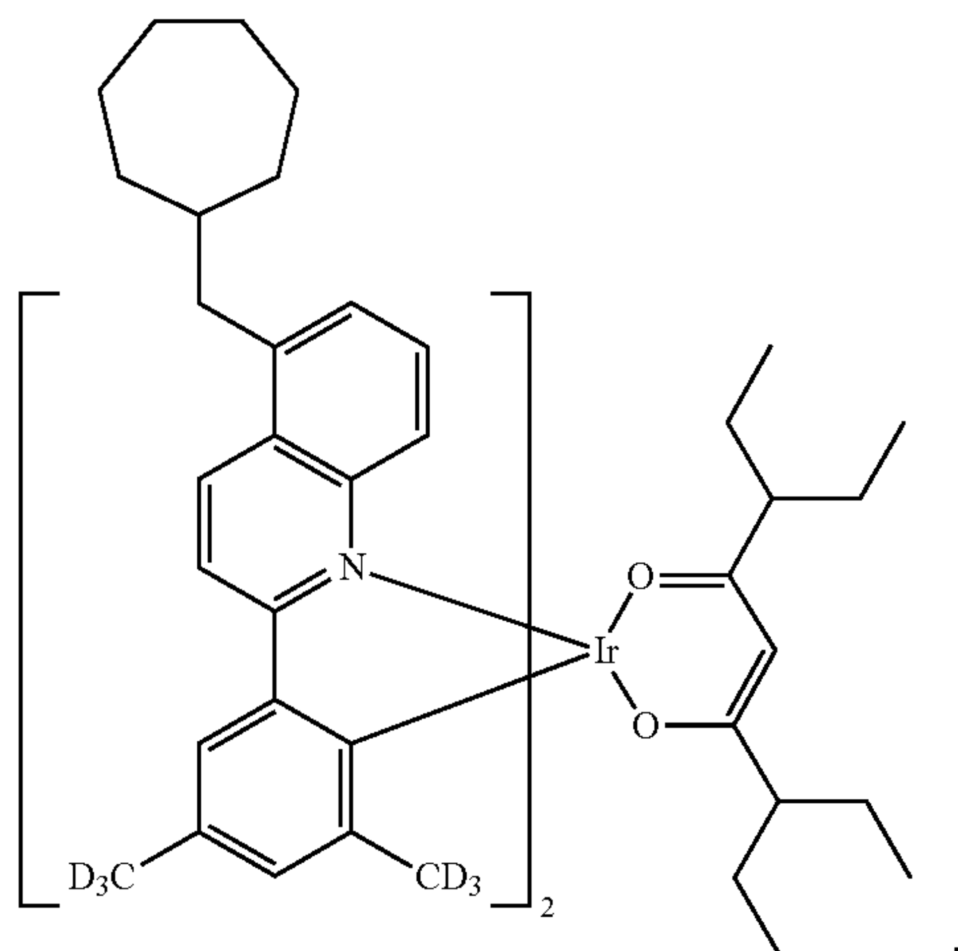
Compound II-68
