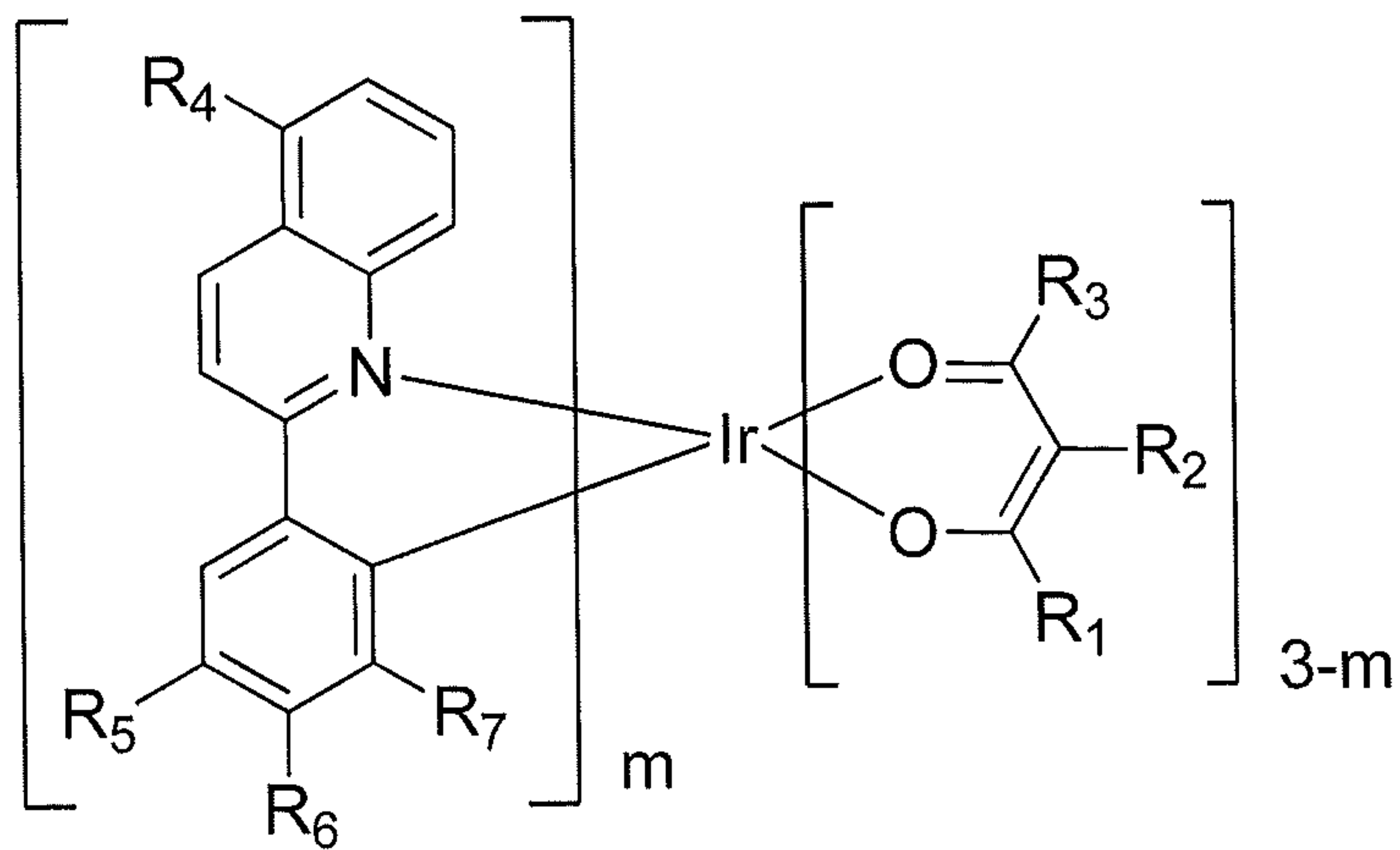
Formula III
