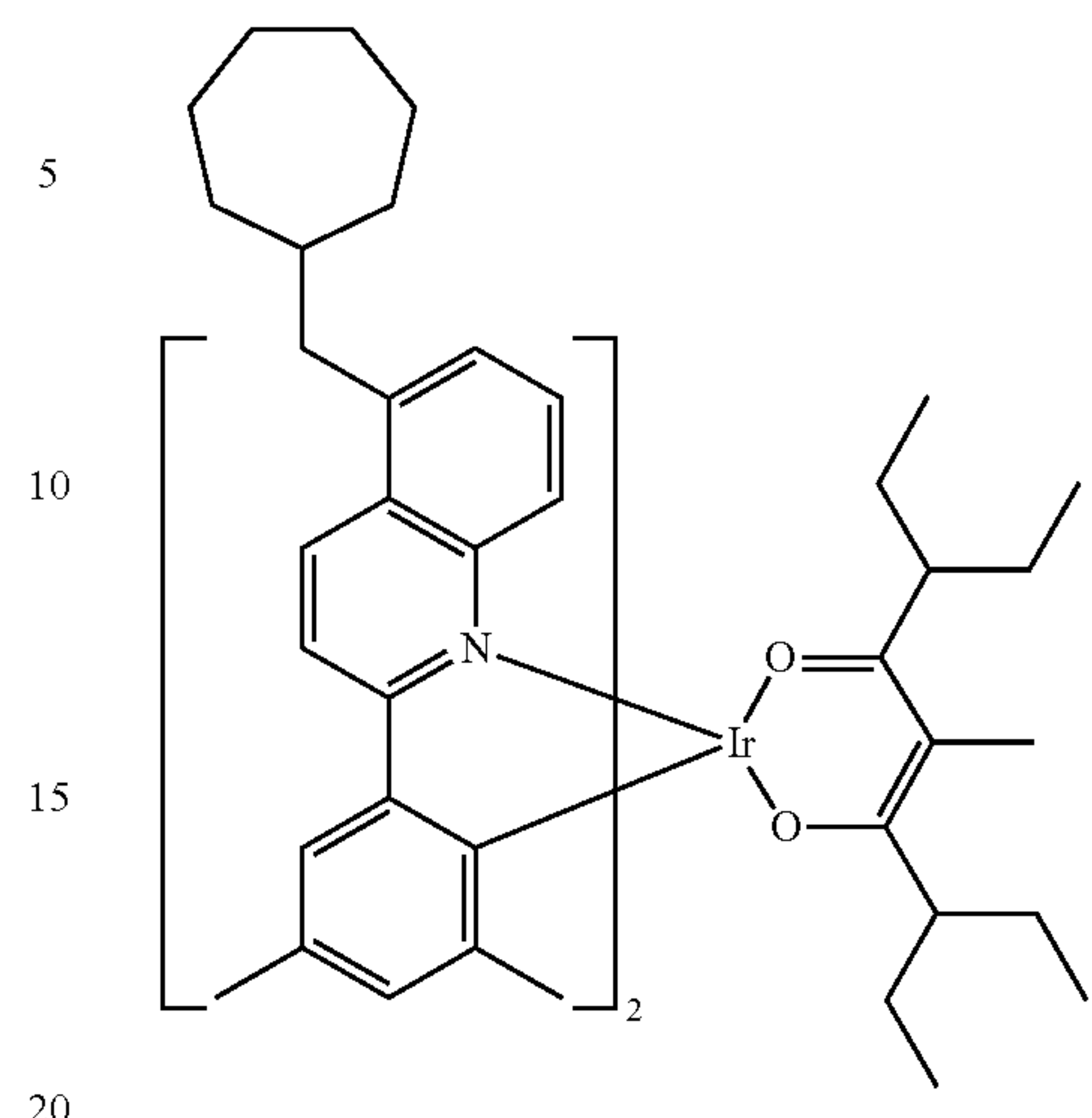
Compound II-33
