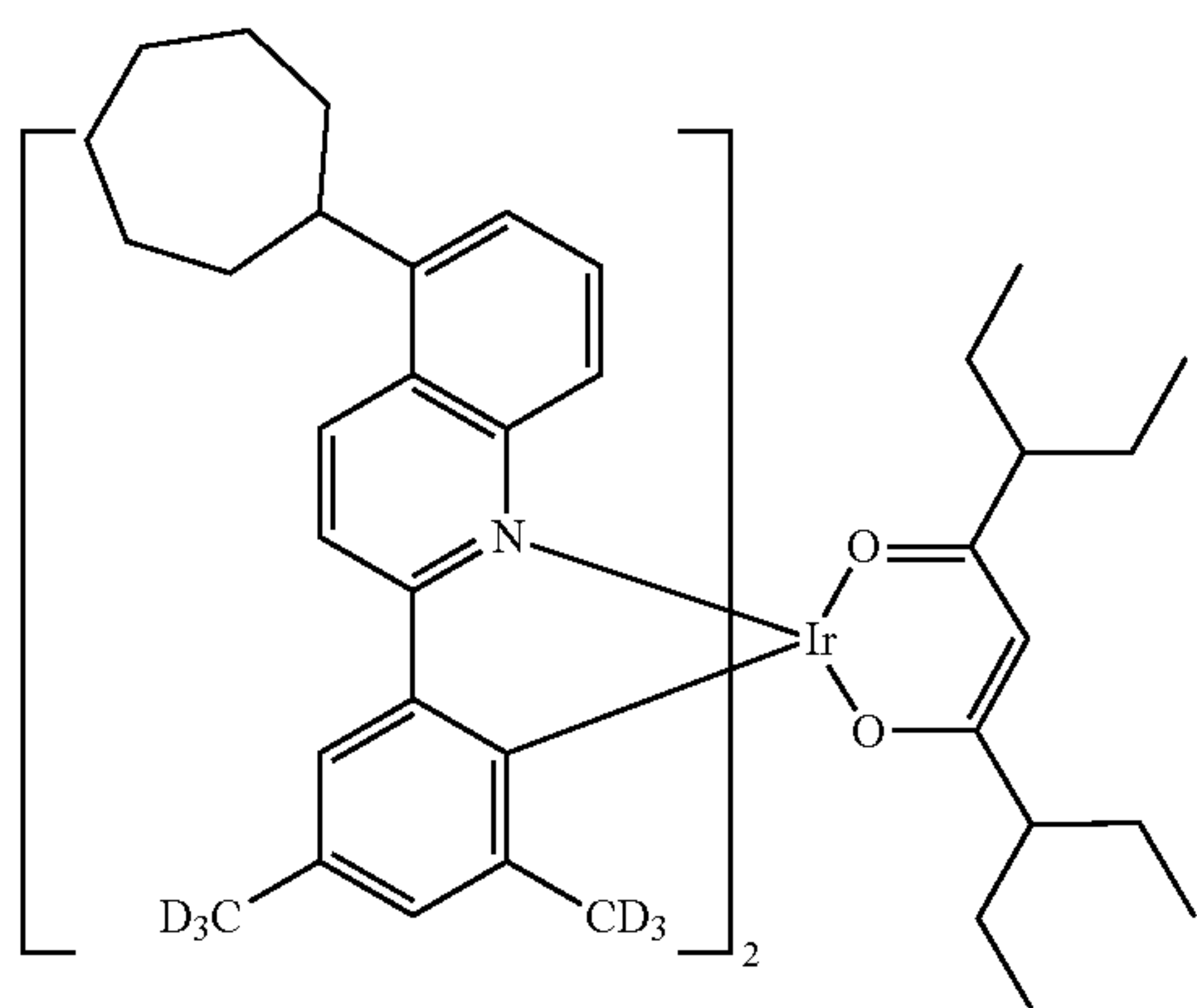
Compound II-51
