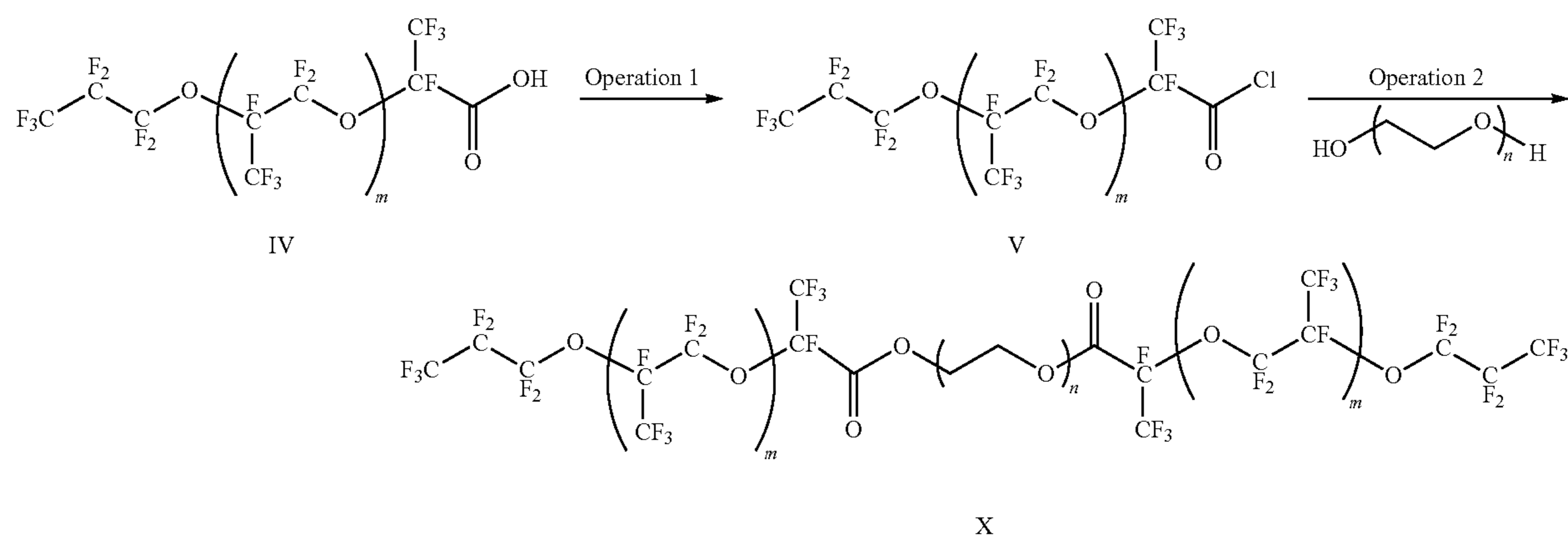
Scheme 2
