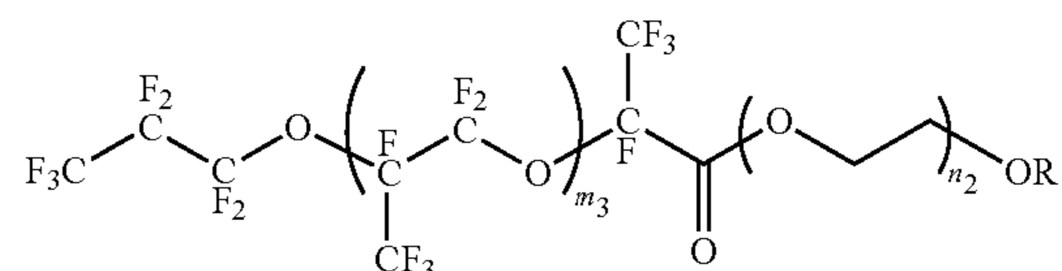
Formula II
